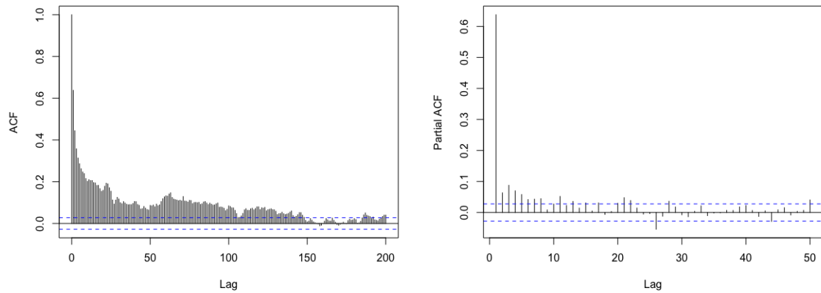
Figure 3.10 – Autocorrelation function (left) and partial autocorrelation function (right) of the residuals.
