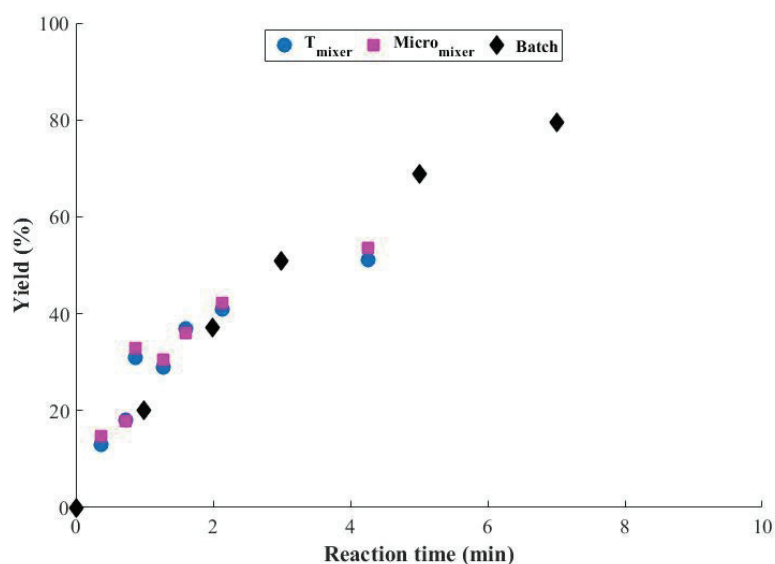
Figure 8 Verification that the reaction is not limited by micro-mixing or mass transfer
