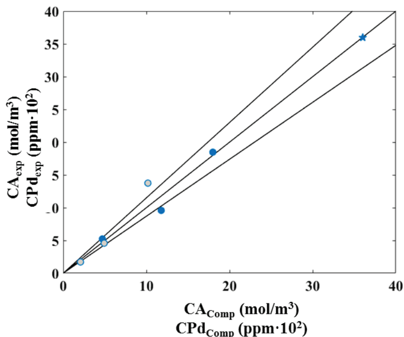
Figure 40 Parity plot of best fit for 4-odoacetophenone concentration at column and tube outlet and leached Pd concentration for Pd/C/Foam. Filled circles (column), empty circles (tube), Pd leaching (blue star) (ppm10 2 )
