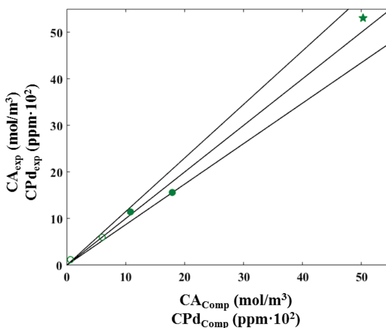
Figure 43 Parity plot of best fit for 4-iodoacetophenone concentration at column and tube outlet for Pd(II)-DPP-Siliacat. Filled circles (column), empty circles (tube), Pd leaching (green star) (ppm10 2 )
