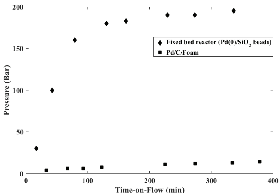
Figure 25 pressure variation inside the column for fixed bed and foam reactor.
