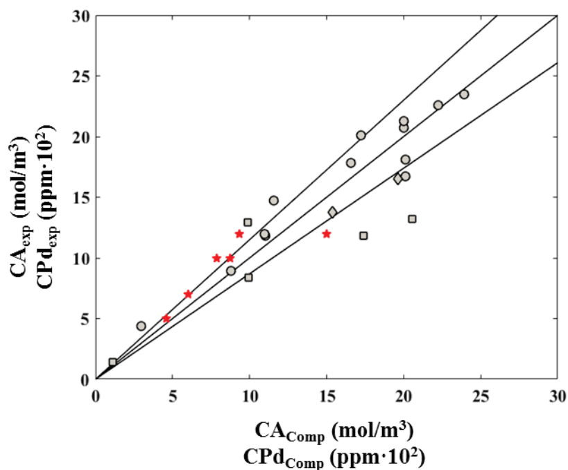
Figure 37 Parity plot of best fit for 4-iodoacetophenone and leached Pd concentrations at tube outlet for different Pd(0) catalysts (Pd(0)-Siliacat(black circles), Pd(0)-Strem (black squares), Pd(0)/alumina (diamonds), Pd leaching (red stars))
