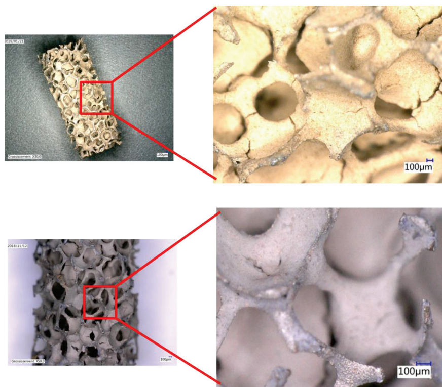
Figure 24 Optical microscopy for two different open cell foams before calcination
