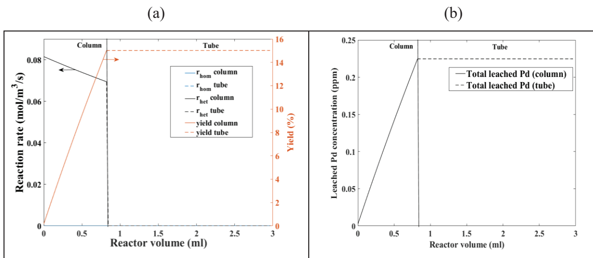
Figure 45 a) homogeneous vs. heterogeneous reaction rates and conversion inside the reactor for pure heterogeneous mechanism. b) homogeneous Pd concentration profiles inside column and empty tube continuous line (column), dashed line (tube).
