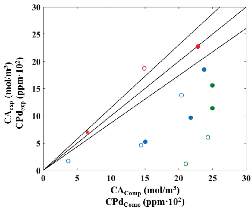
Figure 39 Parity plot of best fit for 4-iodoacetophenone at column and tube outlet for other Pd(0) catalysts ( \text{Ce}_{0.2}\text{Sn}_{0.79}\text{Pd}_{0.01}\text{O}_{2-\delta} (red circles), Pd/C/Foam (blue circles), Pd(II)-Siliacat/Foam (green circles) and \text{Pd}_{\text{leaching}} (stars)). Filled circles (column), empty circles (tube).
