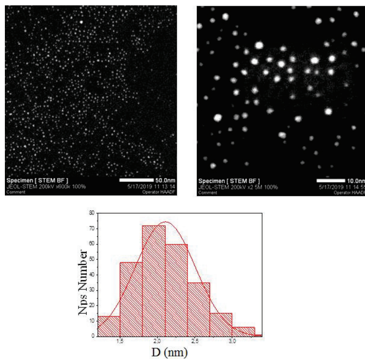
Figure 26 Pd Nps STEM images with the histogram of size distribution (C2P2 images)
