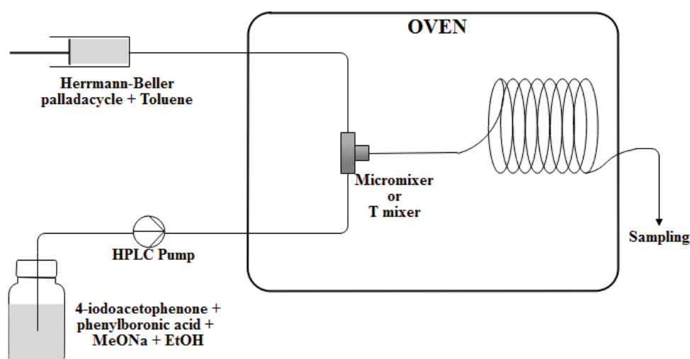
Figure 5 Flow test experimental set-up
