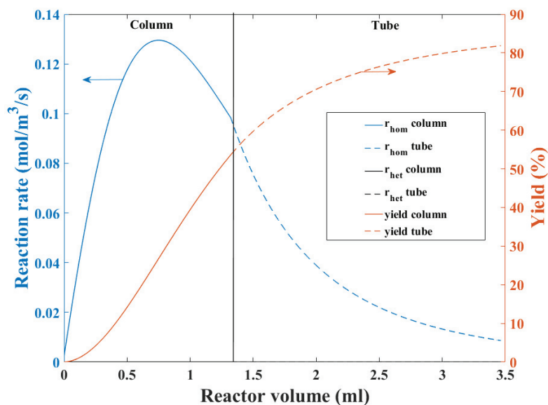
Figure 41 Simulated homogeneous vs. heterogeneous reaction rates and conversion inside the reactor for 4-iodoacetophenone. Continuous line (column), dashed line (tube).
