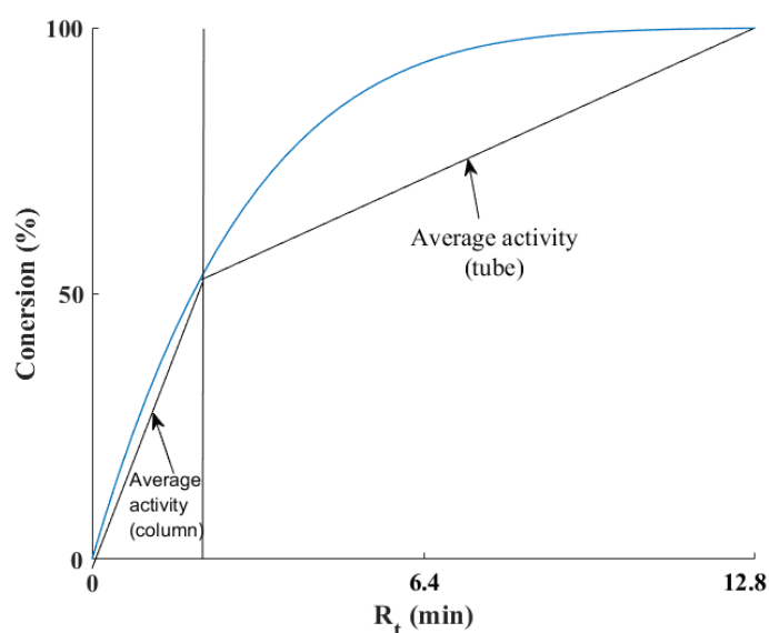
Figure 21 Average activity inside column and tube with conversion
