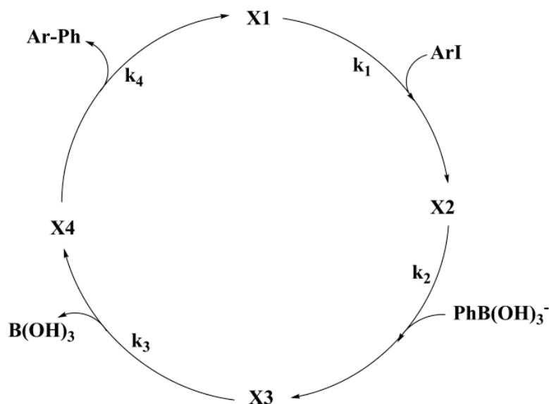
Figure 16 Homogeneous mechanism for Suzuki-Miyaura reaction
