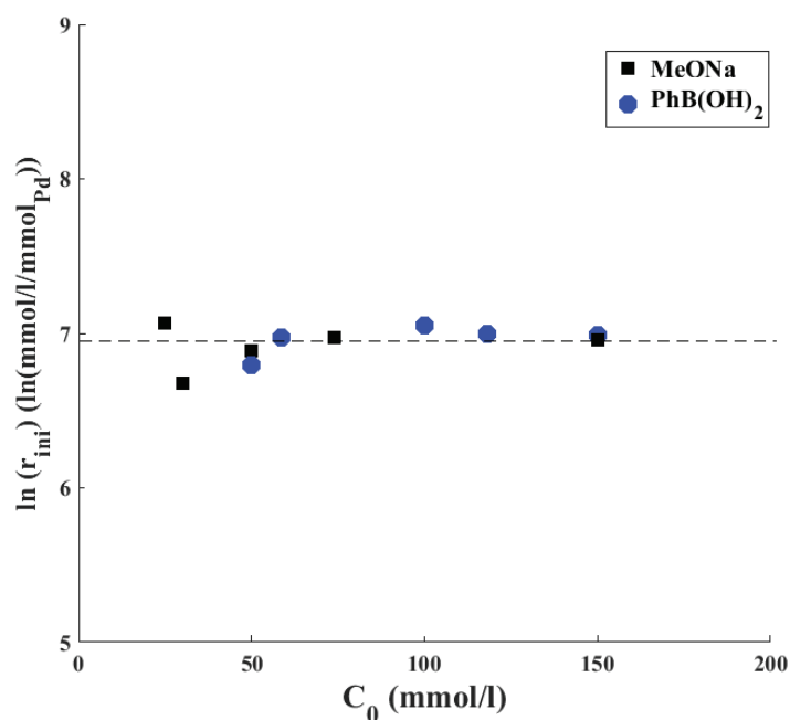
Figure 12 Phenylboronic acid and sodium methylate effect on SM initial reaction rate
