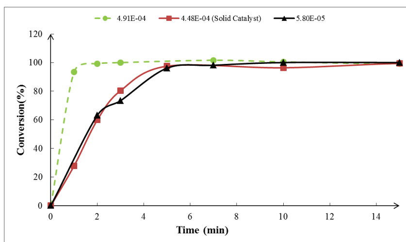
Figure 7 Effect of palladacycle pre-dissolution in toluene. (a) brown squares: use of crystalline catalyst directly ( 2.5 \cdot 10^{-4} \text{ mol}_\text{I}/\text{l} ); (b) green circles pre-dissolution of the catalyst in toluene ( 2.5 \cdot 10^{-4} \text{ mol}_\text{I}/\text{l} ) and the (c) black triangles with pre-dissolution of the catalyst in toluene ( 2.5 \cdot 10^{-5} \text{ mol}_\text{I}/\text{l} ). Conditions: 4-iodoacetophenone (0.05 M, 1 eq.), phenylboronic acid (0.06 M, 1.2 eq.), MeONa (0.075 M, 1.5 eq.), I ( 2.5 \cdot 10^{-5} \text{ mol}_\text{I}/\text{l} , 0.0005 eq.) or I ( 2.5 \cdot 10^{-4} \text{ mol}_\text{I}/\text{l} , 0.005 eq.), T=60^\circ\text{C} , 20 ml of ethanol.
