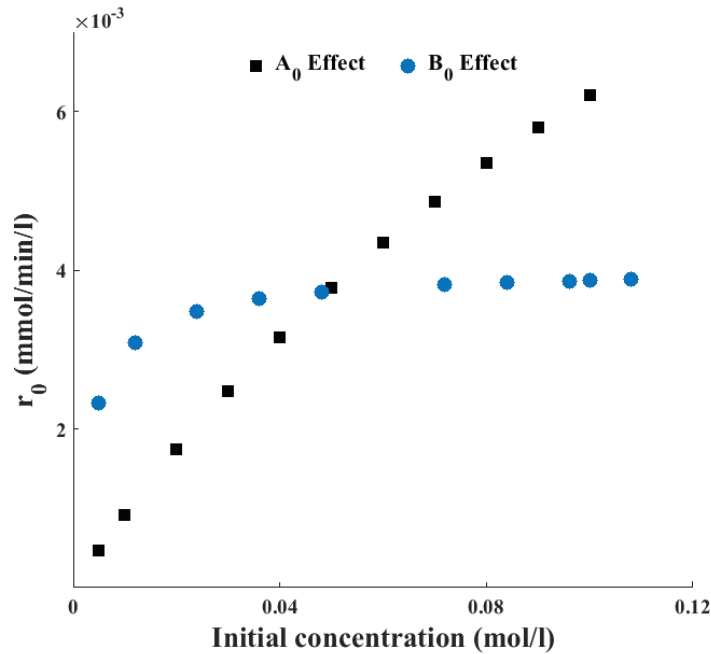
Figure 17 Effect of A_0 and B_0 on the reaction initial rate
