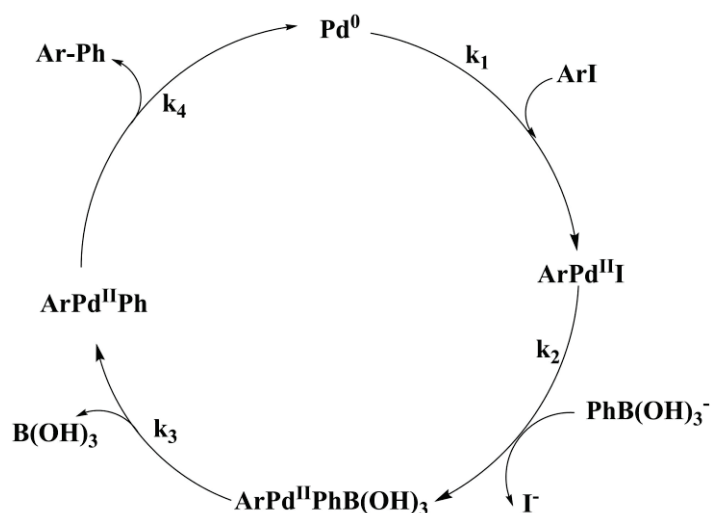
Figure 14 The final mechanism used for the simulation process
