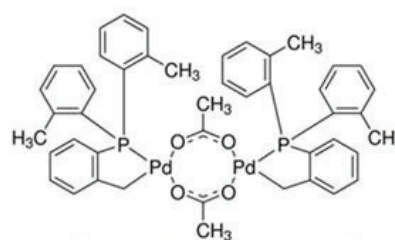
Palladacycle
