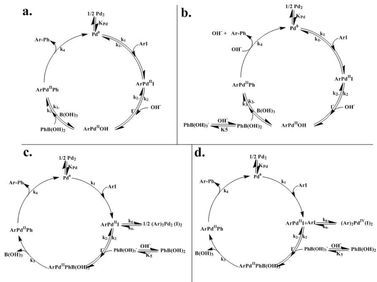
Appendix 11 Possible mechanisms for Suzuki-Miyaura reaction
