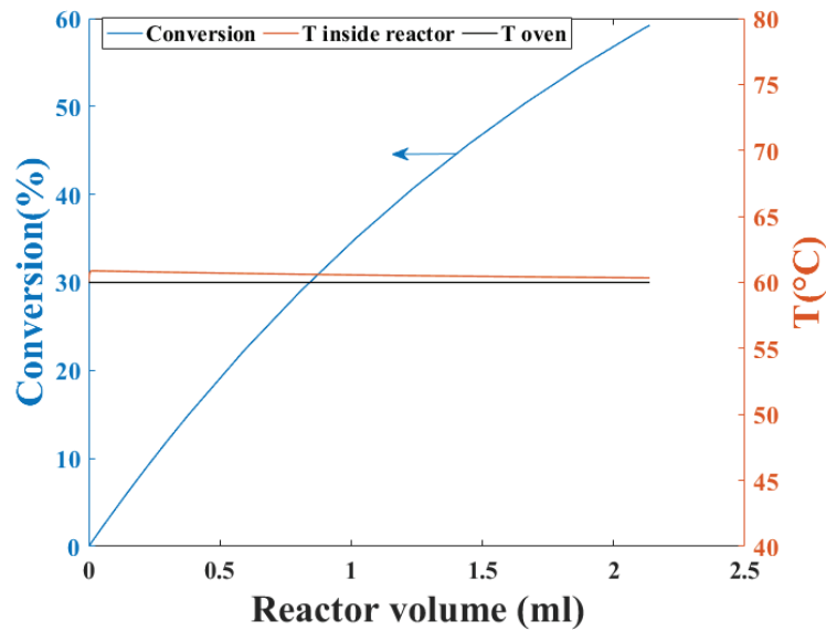
Appendix 13 Isothermal behavior of the reactor
