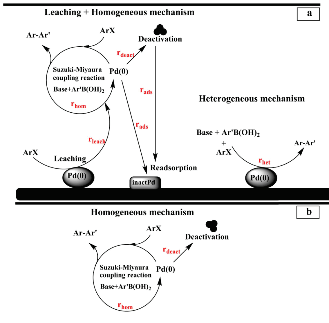
Figure 35 Homogeneous vs. heterogeneous catalysis a): inside column and b): inside tube
