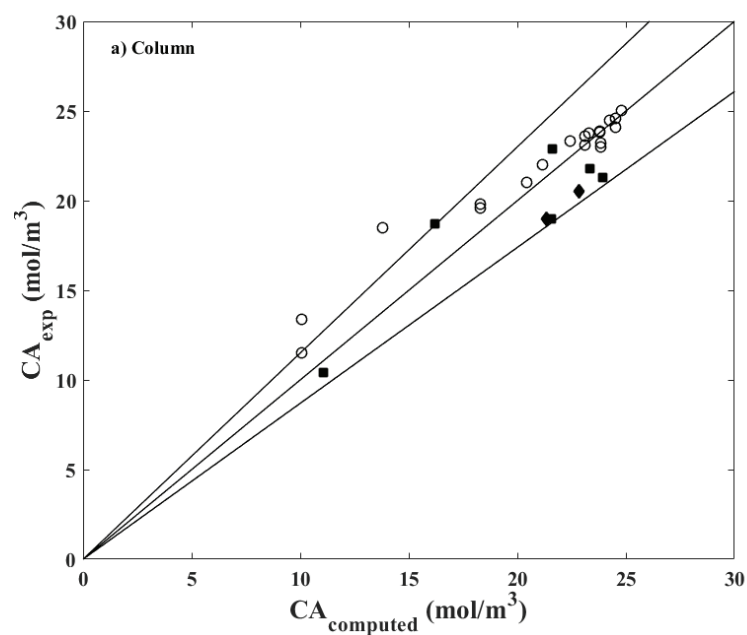
Figure 36 Parity plot of best fit for 4-iodoacetophenone and leached Pd concentrations at column outlet for different Pd(0) catalysts (Pd(0)-Siliacat(empty circles), Pd(0)-Strem (black squares), Pd(0)/alumina (diamonds)).
