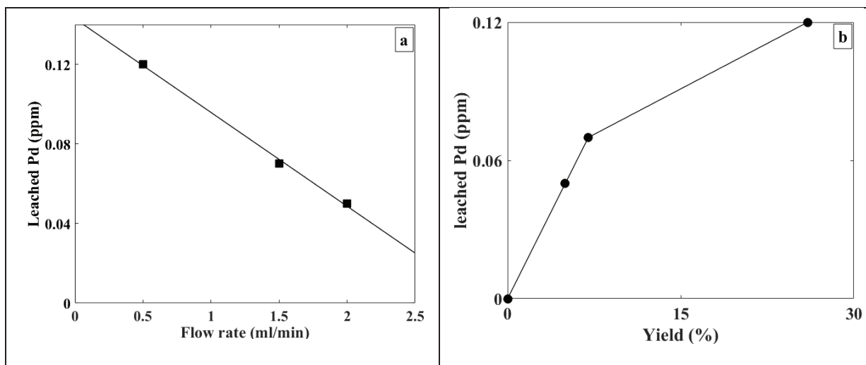
Figure 22 Pd leaching vs. flow rate (a) and Pd leaching vs. yield (b).
