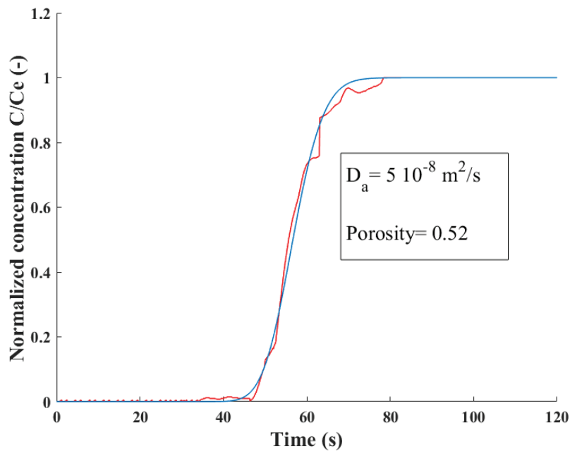
Appendix 12 Experimental vs. Optimized step response profile of normalized concentration at column outlet
