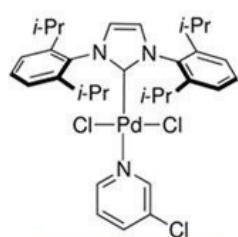
PEPPSI
