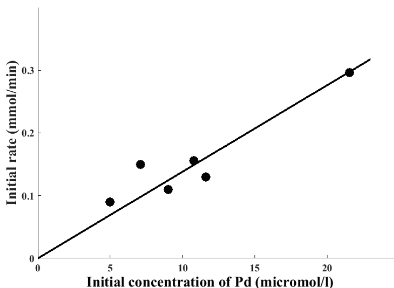
Figure 10 Effect of the initial concentration of Pd on the reaction rate. Conditions: 4-iodoacetophenone (0.05 M, 1 eq.), phenylboronic acid (0.06 M, 1.2 eq.), MeONa (0.075 M, 1.5 eq.), I from 2.5 \cdot 10^{-6} M to 2.5 \cdot 10^{-4} M, 20 ml of ethanol and 60 °C.
