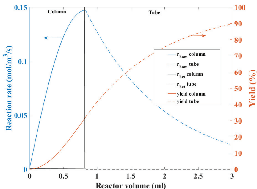
Figure 38 Simulated homogeneous vs. heterogeneous reaction rates and conversion inside the reactor for 4-iodoacetophenone. Continuous line (column), dashed line (tube).
