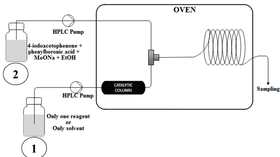
Figure 23 Experimental set-up to identify the reactant responsible for leaching
