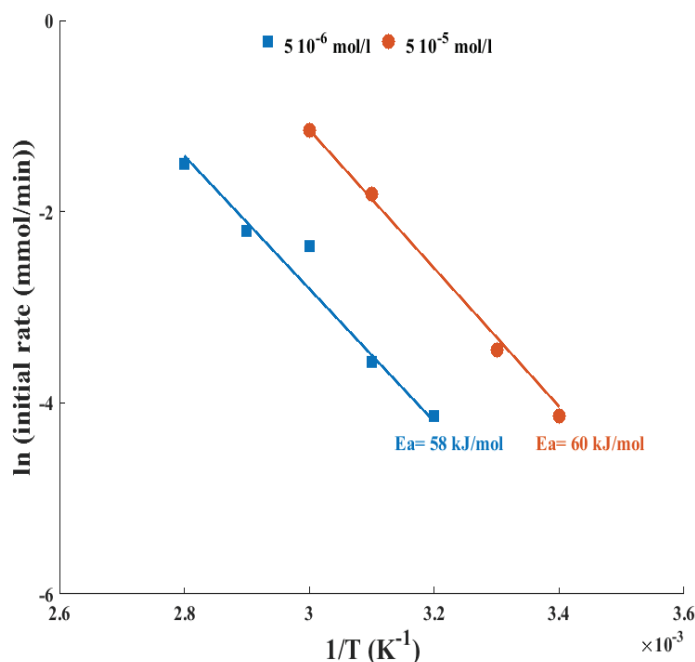
Figure 9 Effect of temperature on Suzuki-coupling of 4-iodoacetophenone and phenylboronic acid using two different concentrations of Pd (Arrhenius Plot).
