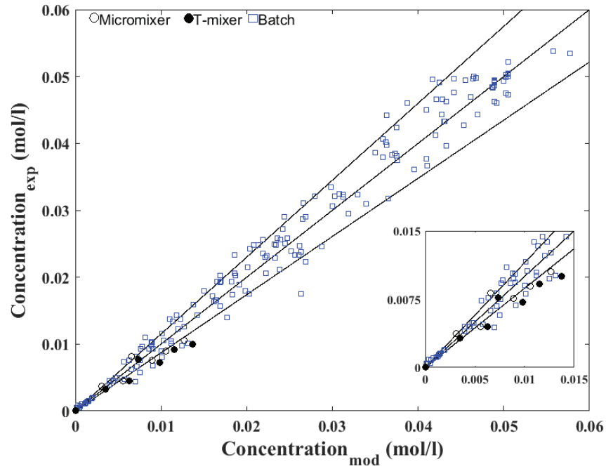
Figure 15 parity plot between experimental and modeled concentrations
