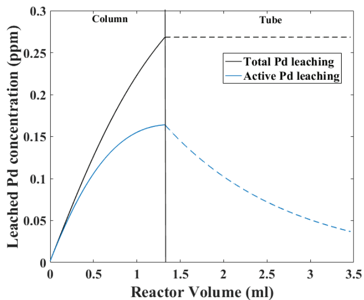
Figure 42 total and active leached Pd for Pd/C/Foam. Conditions: see Figure 41
