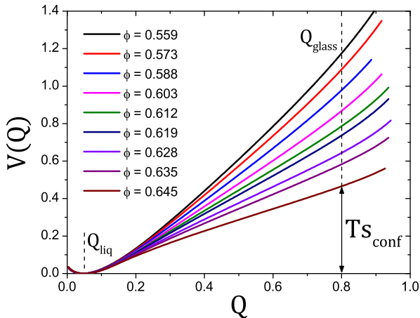
Figure 9: Franz-Parisi free energy in three dimensional polydisperse hard spheres, using a combination of swap Monte Carlo, parallel tempering, and umbrella sampling techniques. [136] V(Q_{\text{glass}}) decreases progressively with increasing the volume fraction \phi . The vertical arrow indicates the estimate of S_{\text{conf}} as the free energy difference between the low-overlap ( Q_{\text{liq}} ) and large-overlap ( Q_{\text{glass}} ) phases. Estimated Kauzmann transition volume fraction, \phi_K , at which S_{\text{conf}} vanishes is \phi_K \approx 0.68 . The system shows jamming transition by rapid compression of dilute configurations at \phi_J \approx 0.655 . [221]
