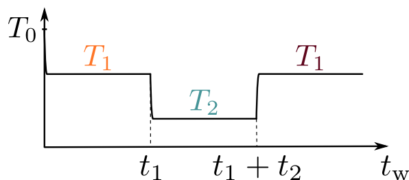
Figure 2: Protocol: Sketch of the temperature cycle, where T_1 and T_2 are both in the glass phase while T_0 is in the fluid.
