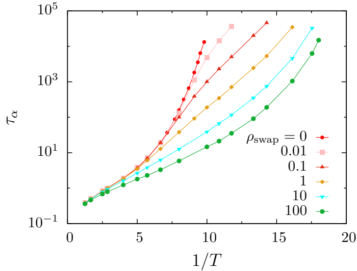
Figure 2: Evolution of the equilibration time \tau_\alpha with inverse temperature 1/T in hybrid MD/MC simulations of the three-dimensional soft polydisperse model of Sec. II.1 at number density 1. The swap density \rho_{\text{swap}} is varied between \rho_{\text{swap}} = 0 (ordinary molecular dynamics) and \rho_{\text{swap}} = 100 . The dynamics at intermediate \rho_{\text{swap}} smoothly interpolates between these two limits.
