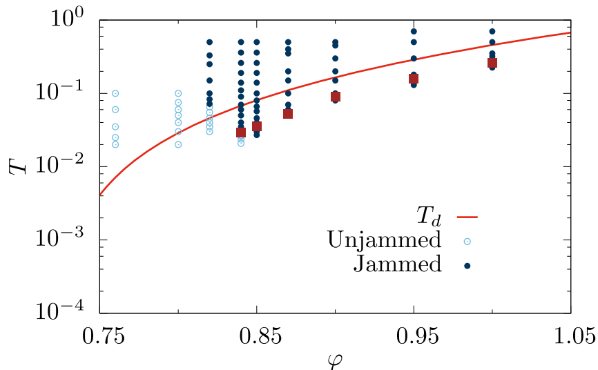
Figure 1: Equilibrium phase diagram of the WCA model. The red line corresponds to the computer glass transition, below which conventional molecular dynamics simulations fail to reach equilibrium over accessible time scales. State points are studied in equilibrium conditions with the hybrid swap method (circles). After energy minimization, their potential energy is either zero (open circles, unjammed), or positive (full circles, jammed). The equilibrium glassy states analyzed in more detail are indicated with red squares.
