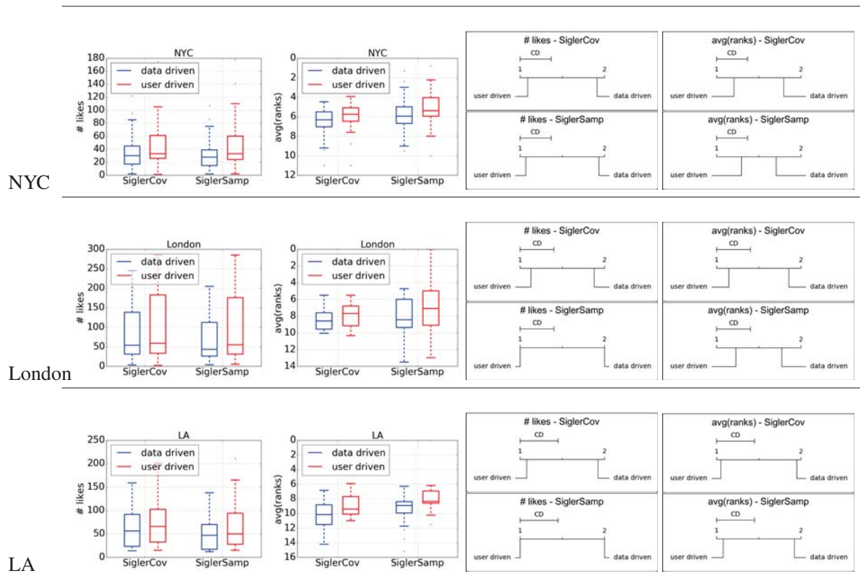
Figure 5.12: Virtual user-driven geo-spatial event detection with SIGLER-Cov and SIGLER-Samp. Number of likes (1st column) and average ranks of events liked by both data and user-driven settings (2nd column), Nemenyi tests on number of likes and average ranks (3rd and 4th columns).
