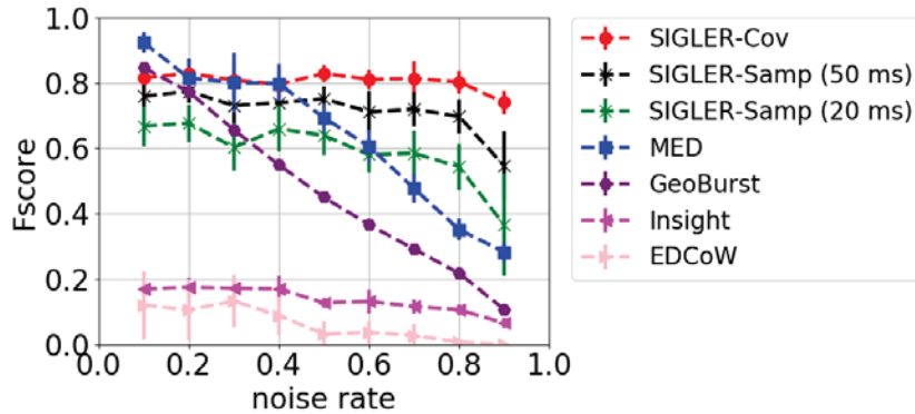
Figure 5.5: Average and error bars of Fscore values obtained over 10 generated datasets for a given noise rate value ( \delta = 5 and \text{minCov} = 0.8 ). Non location-aware event detection approaches are not able to detect geolocated events. MED fails in presence of noise. Runtime of SIGLER-Cov increases from 10ms to 2.5s when the noise rate increases.
