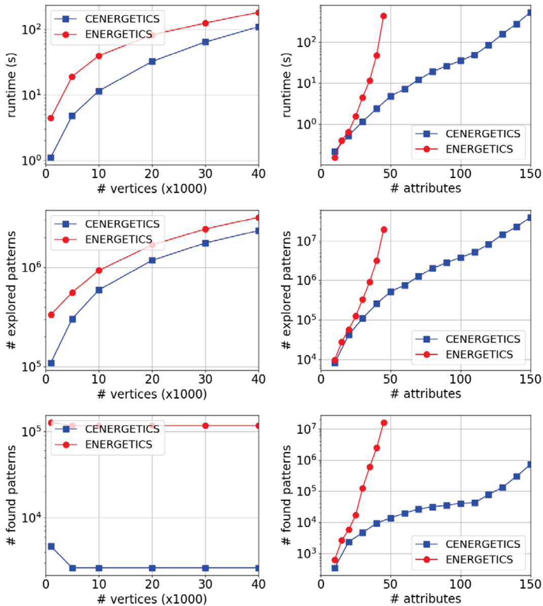
Figure 3.4: Comparison (i.e., runtime, number of explored patterns and number of returned patterns) between \text{CENERGETICS} and \text{ENERGETICS} according to the number of vertices and attributes (default values: number of vertices = 1000, number of attributes = 30).
