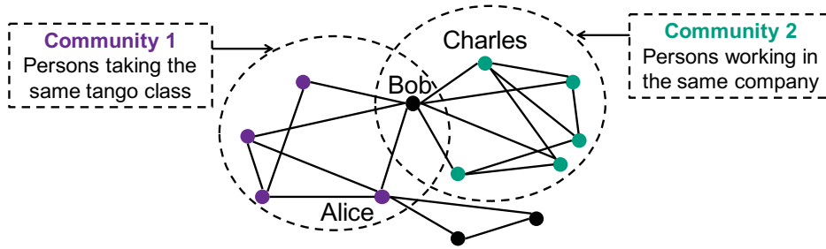
Figure 2.7: Example for the community search problem. Results for this task would be the community 1 if the query vertices are \{\text{Bob}, \text{Alice}\} , and the community 2 if the query vertices are \{\text{Bob}, \text{Charles}\} .
