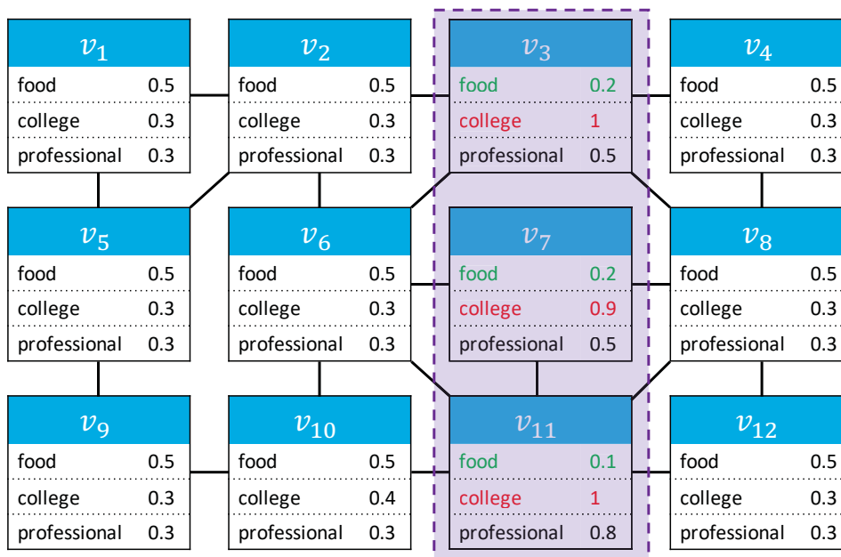
Figure 4.5: The toy graph of Fig. 4.3 with normalized attribute values ( p -values indicating how over-represented the value is as compared to a MaxEnt model with category and vertex size constraints, see Section 4.3.2).
