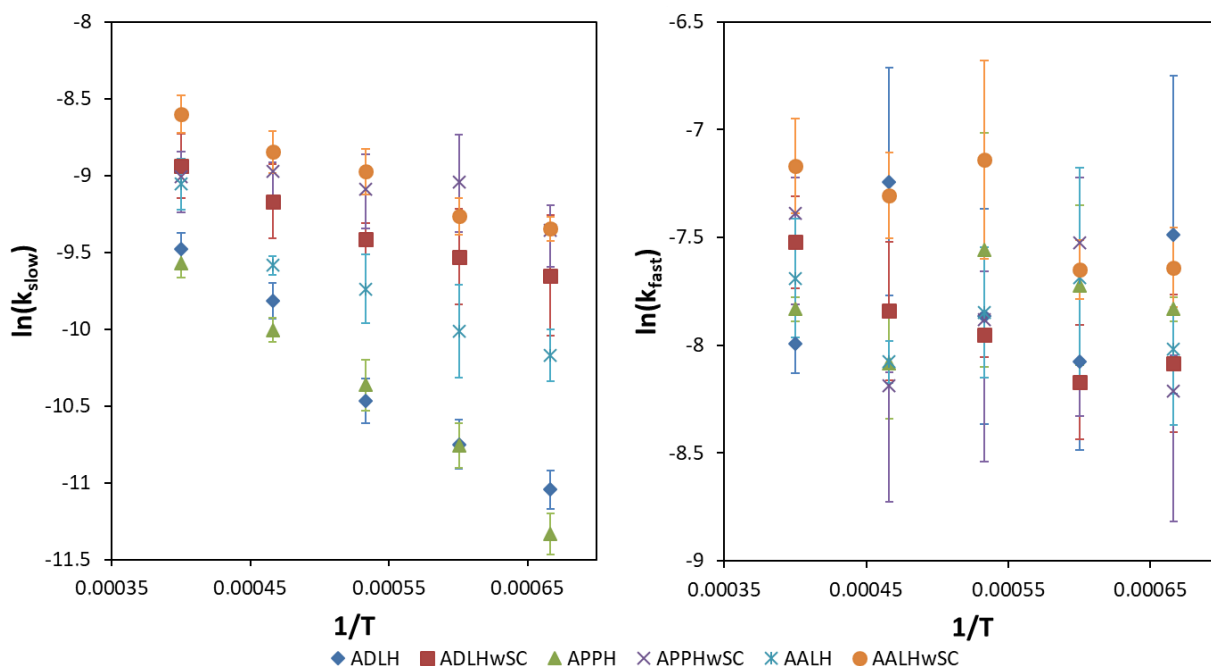
Figure 57. Natural logarithm of the fitted kinetic rate constant of the atomic oxygen consumption of the first exponential function of the double exponential fits (left) and the second exponential function of the double exponential fit (right) over the inverse temperature, for all differentiated species and a temperature range between 1500 K and 2500 K. The addition of “wSC” to the different structural groups denotes the presence of sidechains in the species of the structural group.
