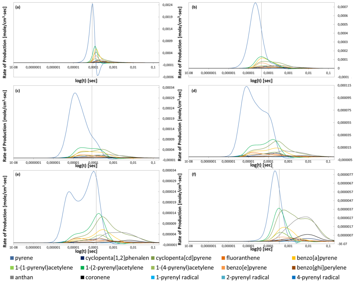
Figure 7. Rates of production of the extracted PAH (shown in Figure 9) over the simulation time for the Chemkin calculations performed with an equivalence ratio of 3.5, a temperature of 1600K and fuel mixtures of (a) 0 mol% n-decane and 100 mol% toluene, (b) 20 mol% n-decane and 80 mol% toluene, (c) 40 mol% n-decane and 60 mol% toluene, (d) 60 mol% n-decane and 40 mol% toluene, (e) 80 mol% n-decane and 20 mol% toluene, and (f) 100 mol% n-decane and 0 mol% toluene.
