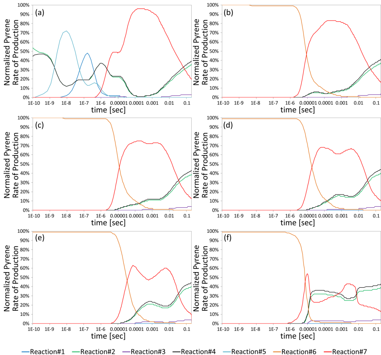
Figure 15. Percentage contribution to the positive ROP of pyrene by each reaction detected to contribute to the growth of pyrene. The numbering of the reactions follows the numbering shown in Table 12. The chosen conditions depicted are taken at an equivalence ratio for 3.5, a temperature of 1600K and a fuel mixture of (a) 100 mol% n-decane, (b) 80 mol% n-decane and 20 mol% toluene, (c) 60 mol% n-decane and 40 mol% toluene, (d) 40 mol% n-decane and 60 mol% toluene, (e) 20 mol% n-decane and 80 mol% toluene, and (f) 100 mol% toluene, to show the impact of fuel composition on the percentage contribution of each reaction. Reactions not shown in one of the graphs did not exceed 1% with respect to the total pyrene ROP.
