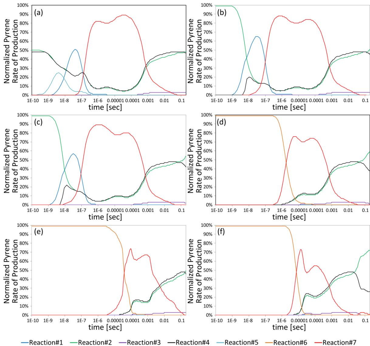
Figure 16. Percentage contribution to the positive ROP of pyrene by each reaction detected to contribute to the growth of pyrene. The numbering of the reactions follows the numbering shown in Table 12. The chosen conditions depicted are taken at an equivalence ratio for 3.5, a temperature of 1800K and a fuel mixture of (a) 100 mol% n-decane, (b) 80 mol% n-decane and 20 mol% toluene, (c) 60 mol% n-decane and 40 mol% toluene, (d) 40 mol% n-decane and 60 mol% toluene, (e) 20 mol% n-decane and 80 mol% toluene, and (f) 100 mol% toluene, to show the impact of fuel composition on the percentage contribution of each reaction. Reactions not shown in one of the graphs did not exceed 1% with respect to the total pyrene ROP.
