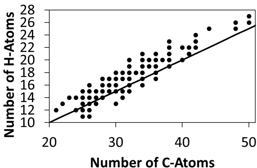
Figure 27. Number of H-atoms over the number of C-atoms found for all detected structures grown from soot precursors for all fuel mixtures, equivalence ratios and temperatures. The solid line depicts the values for an H/C ratio of 0.5.
