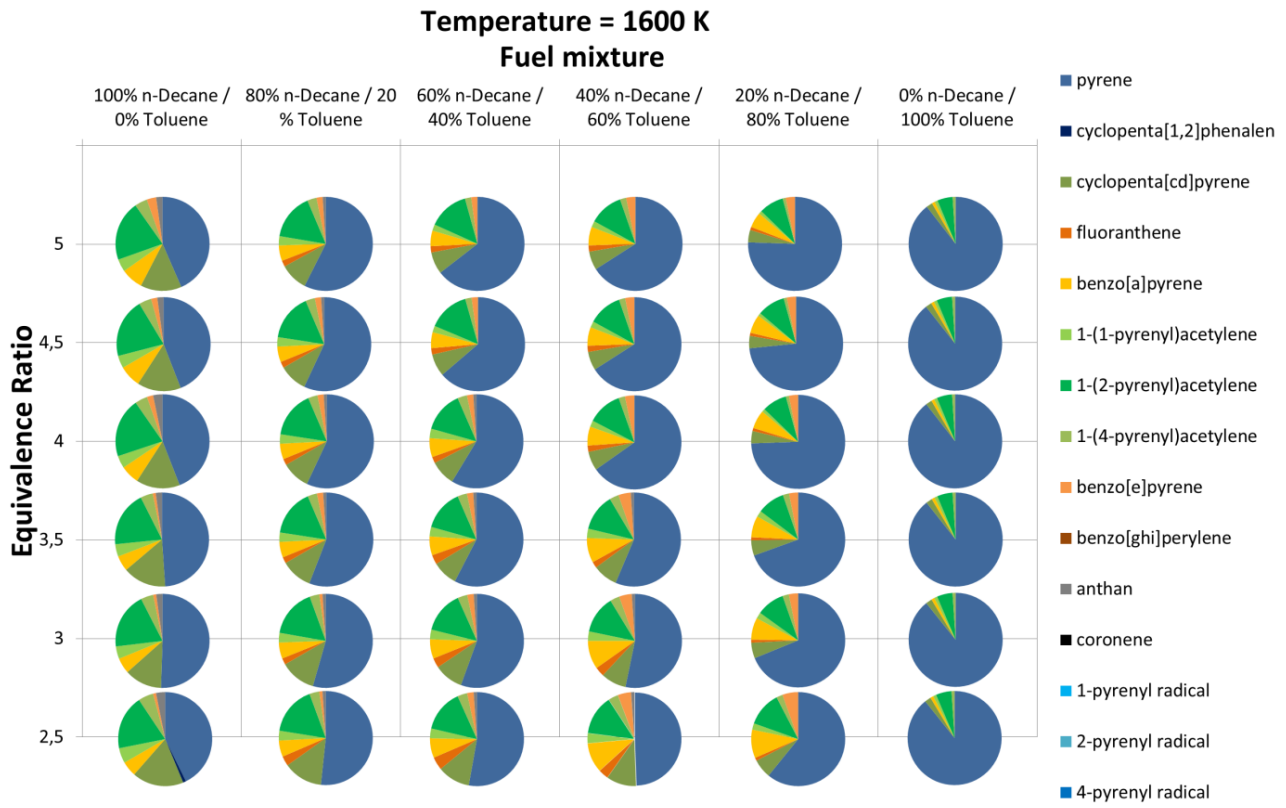
Figure 11. Pie chart of the soot precursor pool compositions at all equivalence ratios and fuel mixtures for a temperature of 1600 K in the Chemkin calculation. The color scheme of the soot precursors included in the compositions is given on the right-hand side. The size of each slice in the pie chart depicts the numerical proportion of the soot precursor of equal color in the composition.
