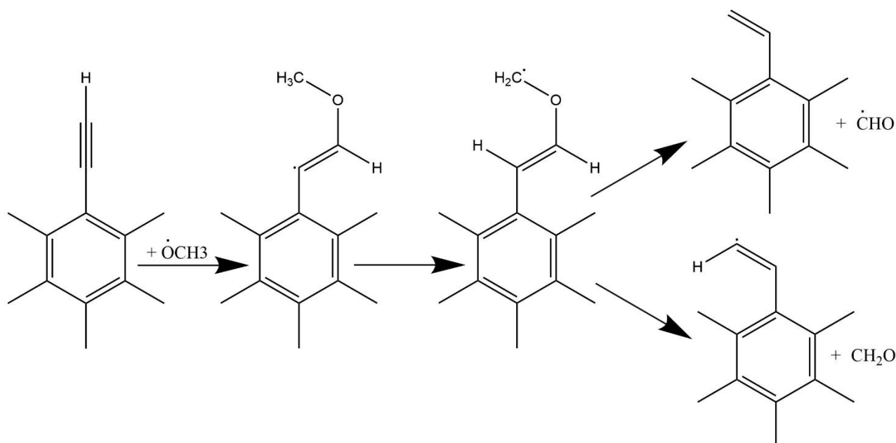
Figure 51. Detected reaction pathways of the addition of methoxyl radicals to a terminal sidechain carbon.
