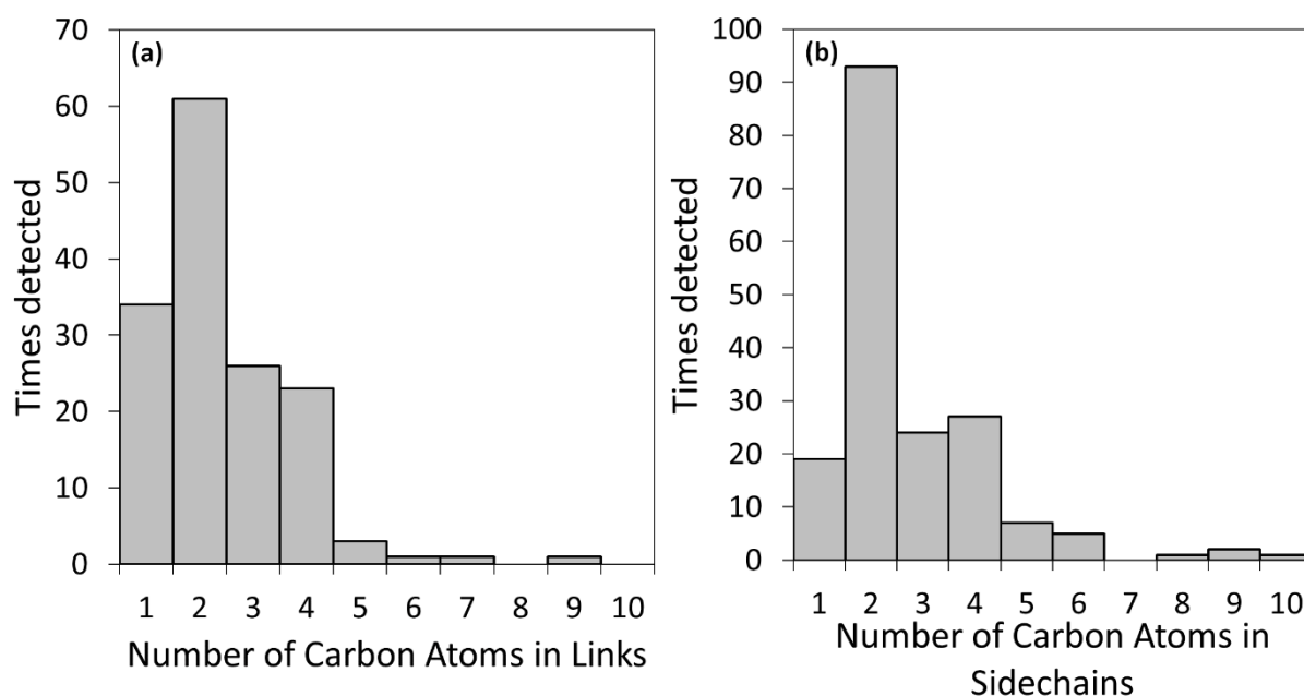
Figure 41. Bar diagram of the number of carbon atoms found in (a) links between aromatic moieties of the detected growth structures and (b) in sidechains attached to the detected growth structures.
