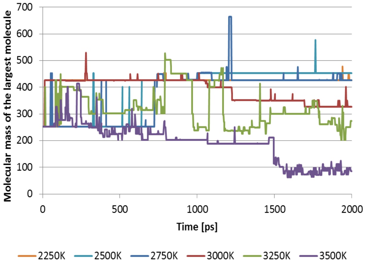
Figure 21. Molecular mass of the largest molecule found during ReaxFF calculations over the simulation time at different temperatures. The molecular composition used for simulation is the precursor pool composition extracted from the Chemkin simulated at a temperature of 1400 K, an equivalence ratio of 2.5 and a fuel composition of 60% n-decane and 40% toluene. While the reactivity is initially accelerated with increasing temperatures for temperatures >3000 K, fragmentation of the molecules takes over for temperatures <3000 K.
