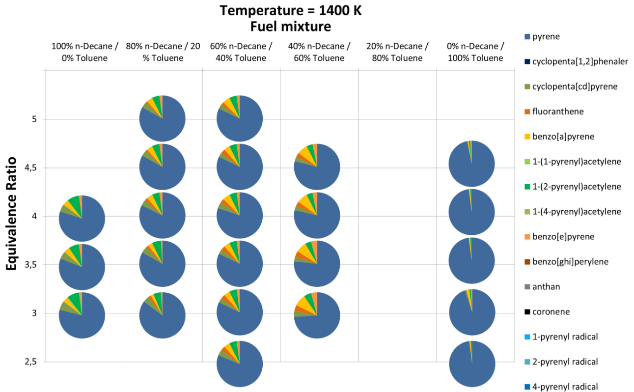
Figure 10. Pie chart of the soot precursor pool compositions at all equivalence ratios and fuel mixtures for a temperature of 1400 K in the Chemkin calculation. The color scheme of the soot precursors included in the compositions is given on the right-hand side. The size of each slice in the pie chart depicts the numerical proportion of the soot precursor of equal color in the composition.
