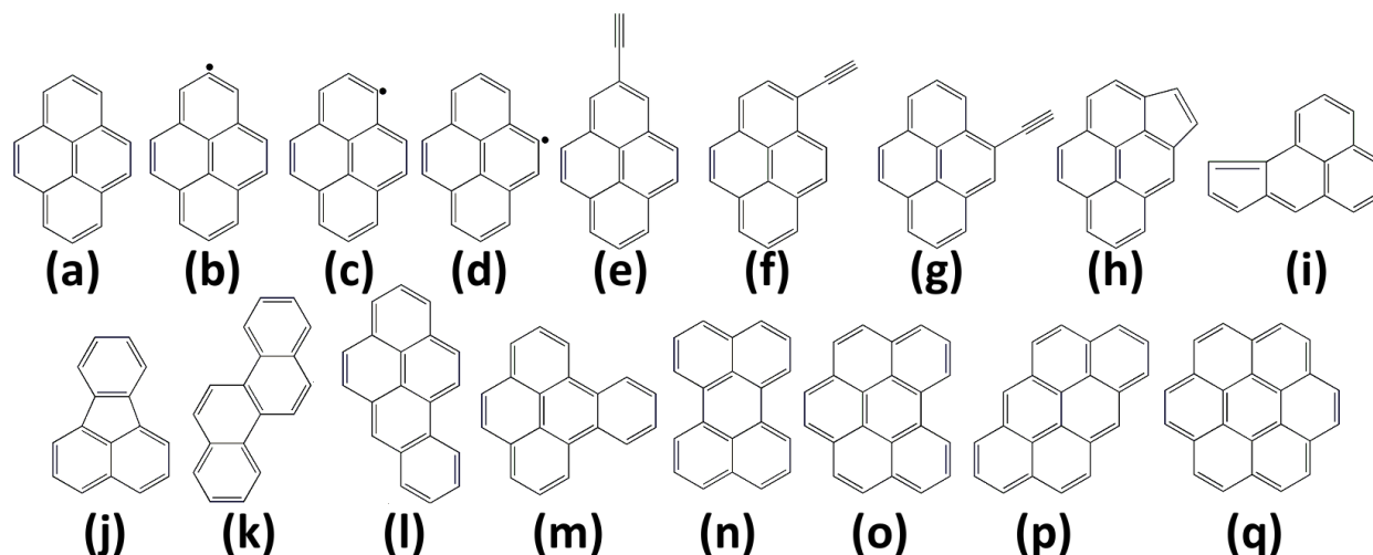
Figure 9. PAH considered for the generation of the precursor pool for the ReaxFF simulations from the Chemkin calculations. (a) pyrene, (b) 1-pyrenyl radical, (c) 2-pyrenyl radical (d) 3-pyrenyl radical, (e) 1-(1-pyrenyl)acetylene, (f) 1-(2-pyrenyl)acetylene, (g) 1-(4-pyrenyl)acetylene, (h) cyclopenta[cd]pyrene, (i) cyclopenta[1,2]phenalen, (j) fluoranthene, (k) chrysene, (l) benzo[a]pyrene, (m) benzo[e]pyrene, (n) perylene, (o) benzo[ghi]perylene, (p) anthanthrene, (q) coronene.
