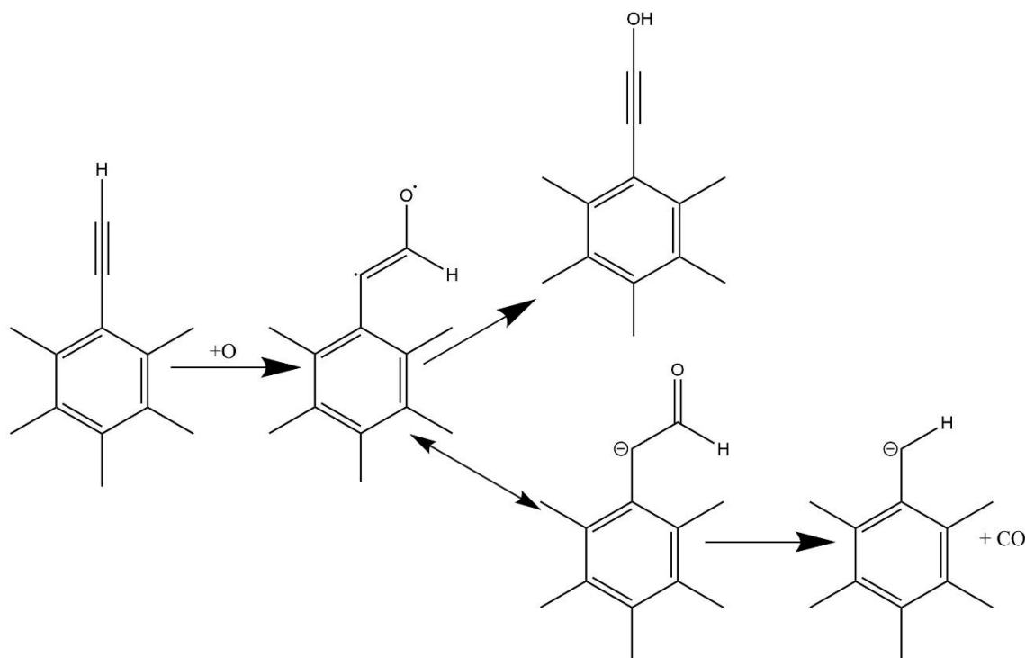
Figure 44. Detected reaction pathways for the addition of atomic oxygen to terminal sidechain carbon.
