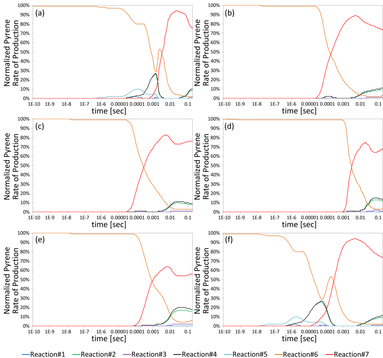
Figure 14. Percentage contribution to the positive ROP of pyrene by each reaction detected to contribute to the growth of pyrene. The numbering of the reactions follows the numbering shown in Table 12. The chosen conditions depicted are taken at an equivalence ratio for 3.5, a temperature of 1400K and a fuel mixture of (a) 100 mol% n-decane, (b) 80 mol% n-decane and 20 mol% toluene, (c) 60 mol% n-decane and 40 mol% toluene, (d) 40 mol% n-decane and 60 mol% toluene, (e) 20 mol% n-decane and 80 mol% toluene, and (f) 100 mol% toluene, to show the impact of fuel composition on the percentage contribution of each reaction. Reactions not shown in one of the graphs did not exceed 1% with respect to the total pyrene ROP.
