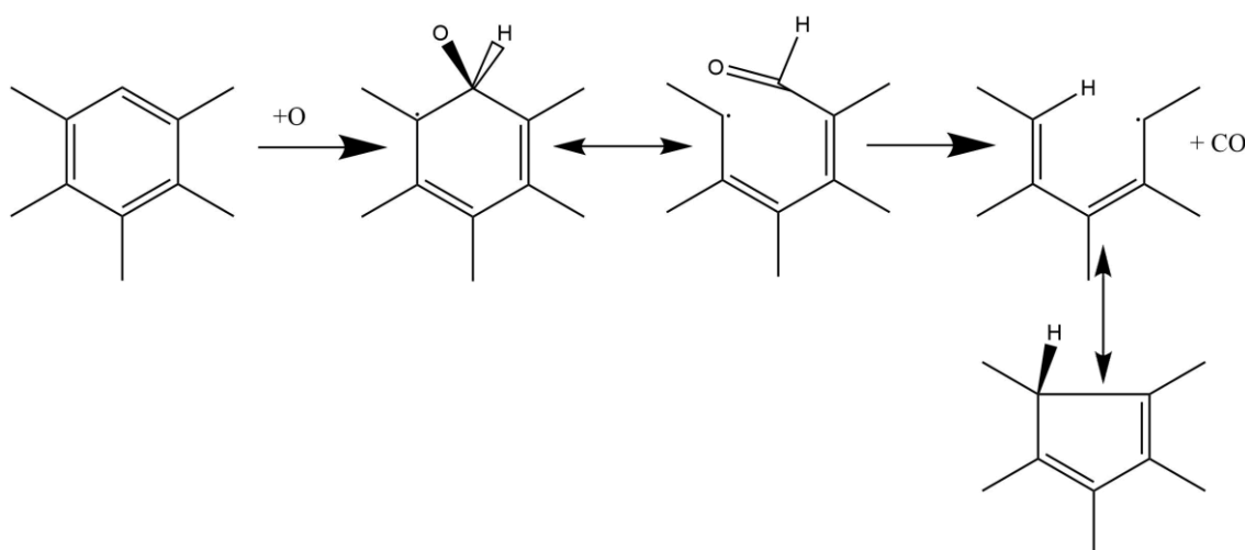
Figure 46. Detected reaction pathways for the addition of atomic oxygen to zigzag sites of aromatic hydrocarbons.
