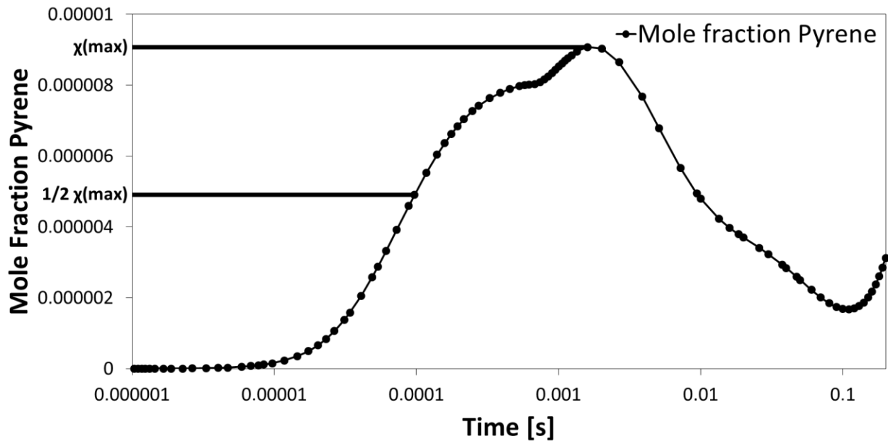
Figure 5. Mole fraction of pyrene for the Chemkin calculation at an equivalence ratio of 3, temperature of 1800 K and a fuel composition of pure n-decane as a function of time. At the time step where 1/2 \chi(\max) is reached the gas-phase composition is taken for the extraction of the soot precursor pool for the MD simulations.
