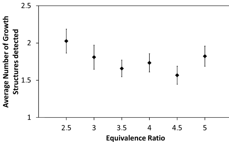
Figure 31. Number of all detected growth structures through bond formation as a function of equivalence ratio. The number of structures is averaged for all temperatures and fuel mixtures and distinguished by equivalence ratio. The vertical bars represent error bars.
