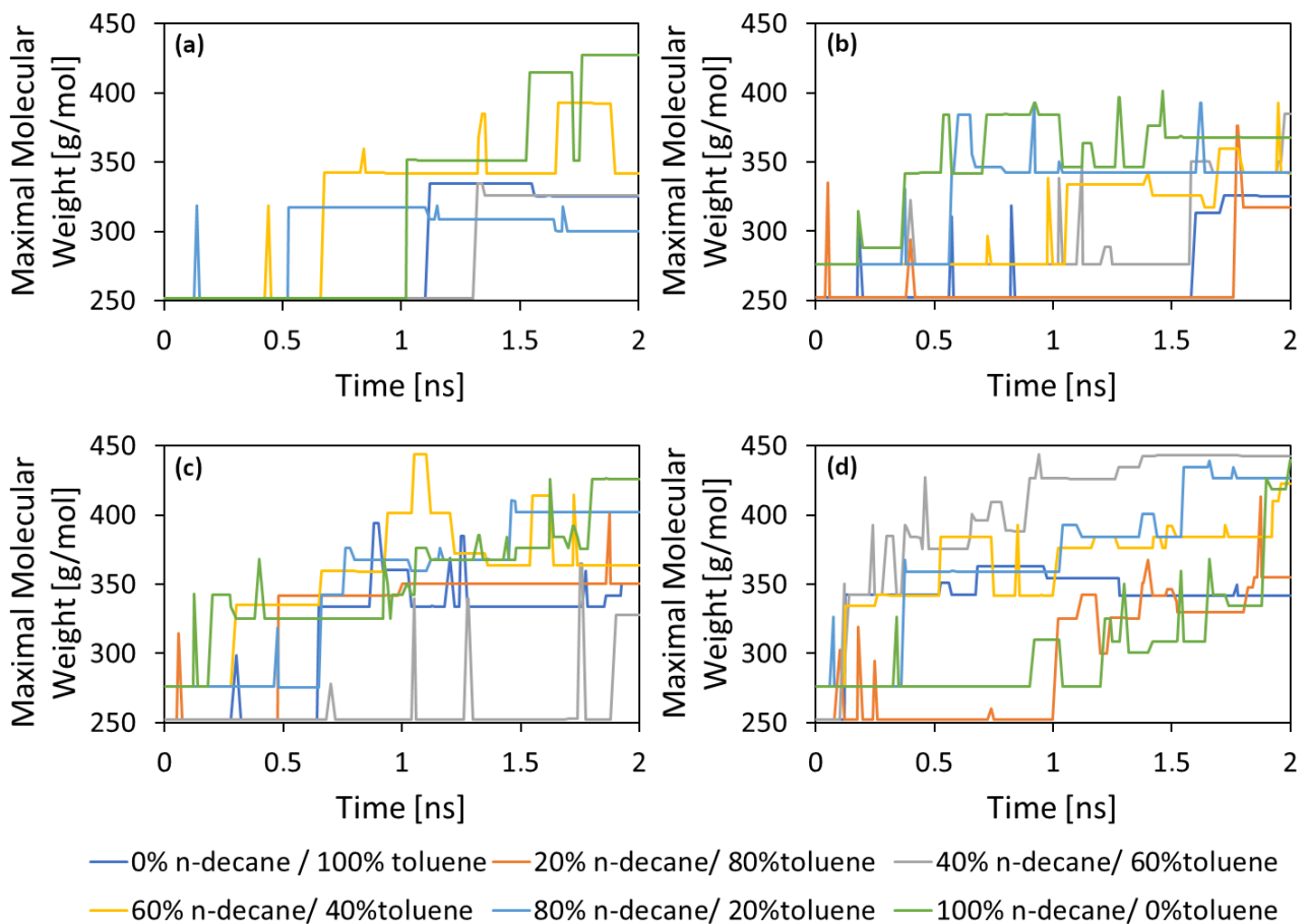
Figure 24. Molecular weight of the largest molecule detected during the ReaxFF simulation averaged over all simulations of one condition and plotted over the calculation time. The soot precursor compositions correspond to the Chemkin calculations performed with an equivalence ratio of 3.5, all fuel mixtures and (a) 1400K, (b) 1600K, (c) 1800K and (d) 2000K.
