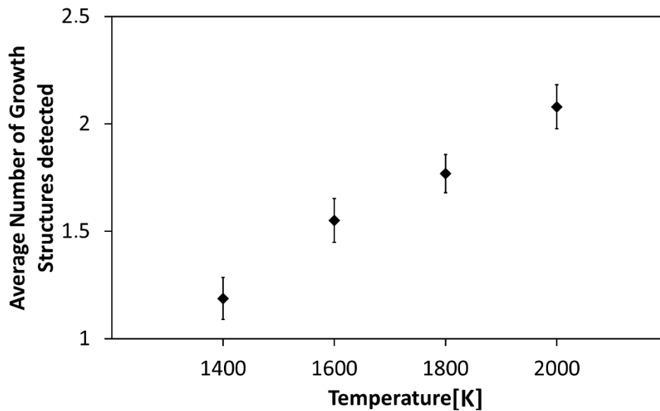
Figure 30. Number of all detected growth structures through bond formation as a function of temperature. The number of structures is averaged for all equivalence ratios and fuel mixtures and distinguished by temperature. The vertical bars represent error bars.
