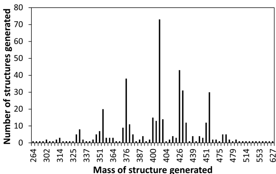
Figure 26. Mass distribution of all detected structures grown from soot precursors for all fuel mixtures, equivalence ratios and temperatures. The main peaks correspond to the following sum formula: C_{26}H_{15} = 327 g/mol; C_{28}H_{16} = 352 ; C_{30}H_{16} = 376 g/mol; C_{32}H_{18} = 402 g/mol; C_{34}H_{18} = 426 g/mol; C_{36}H_{20} = 452 g/mol.
