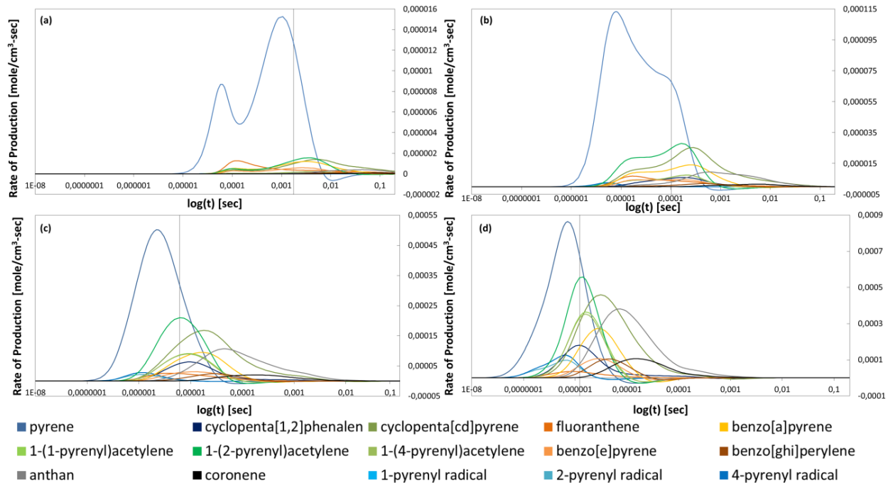
Figure 8. Rates of production of the extracted PAHs (shown in Figure 9) over the simulation time for the Chemkin calculations performed with an equivalence ratio of 3.5, a fuel mixture of 60 mol% n -decane and 40 mol% toluene, and temperatures of (a) 1400 K, (b) 1600 K, (c) 1800 K, and (d) 2000 K.
