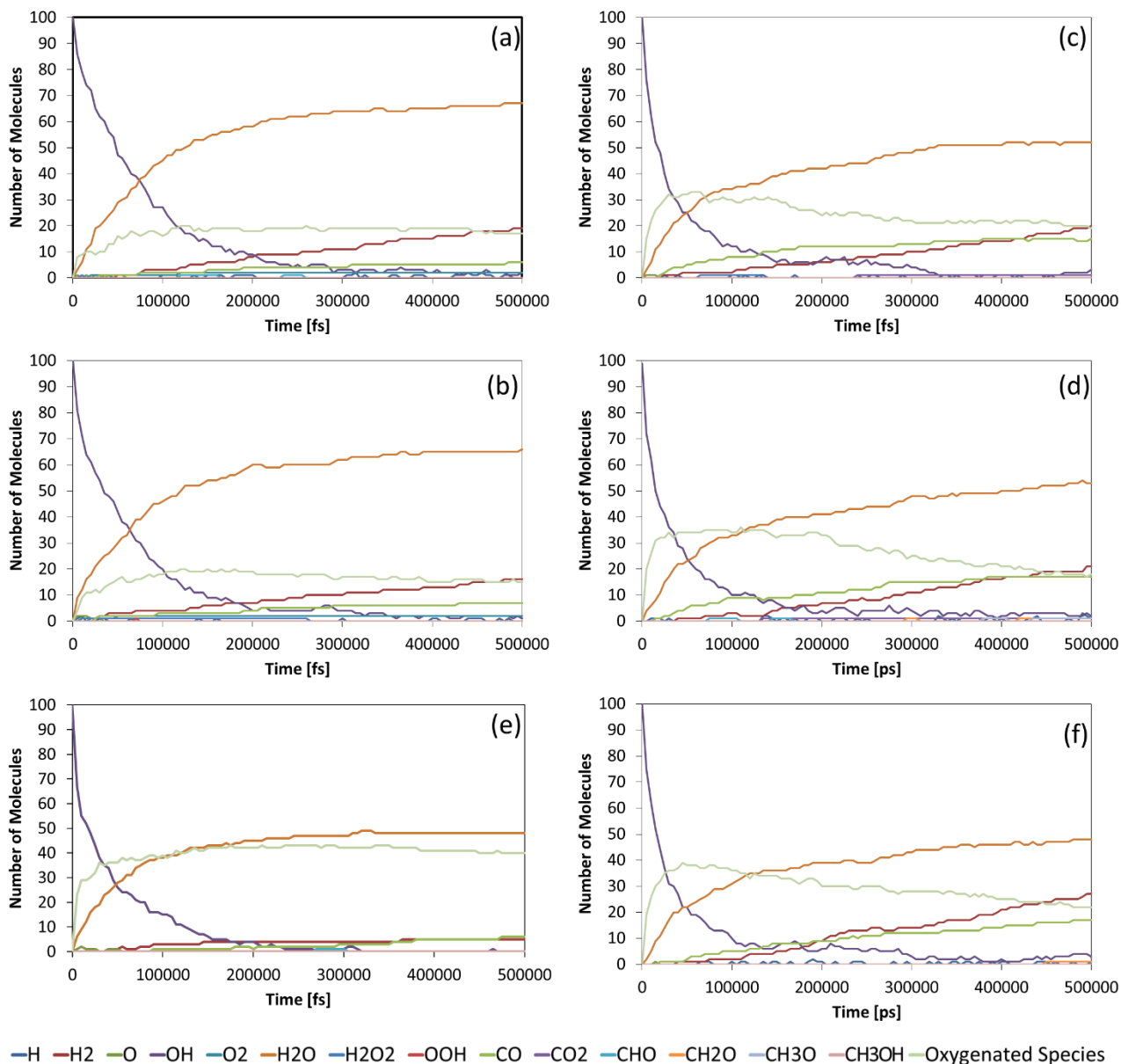
Figure 47. Number of oxygen containing molecules over time for the reactions of the nascent soot structures and hydroxyl radicals. The results have been averaged over the three calculations performed at each condition. The corresponding calculations contain 100 hydroxyl radicals and (a) all ADLH species without sidechains, (b) all ADLH species with sidechains, (c) all APPH species without sidechains, (d) all APPH species with sidechains, (e) all AALH species without sidechains and (f) all AALH species with sidechains.
