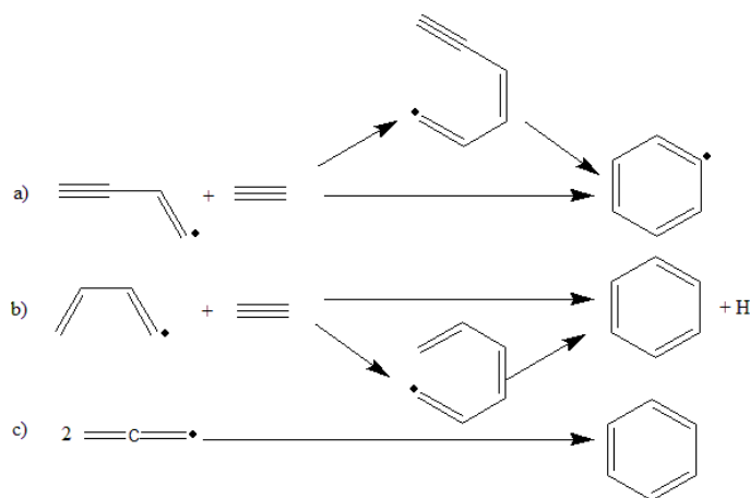
Figure 1. Three major pathways to the formation of the first aromatic ring
