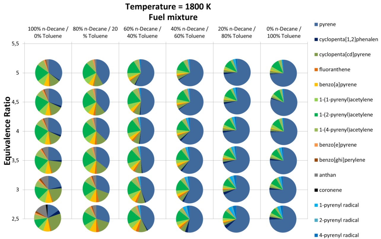
Figure 12. Pie chart of the soot precursor pool compositions at all equivalence ratios and fuel mixtures for a temperature of 1800 K in the Chemkin calculation. The color scheme of the soot precursors included in the compositions is given on the right-hand side. The size of each slice in the pie chart depicts the numerical proportion of the soot precursor of equal color in the composition.
