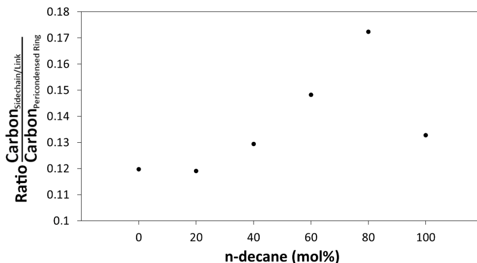
Figure 40. The ratio of carbon atoms found in a sidechain or ring of the growth structures detected to carbon atoms found in pericondensed rings of the growth structures detected as a function of the n-decane mol fraction.
