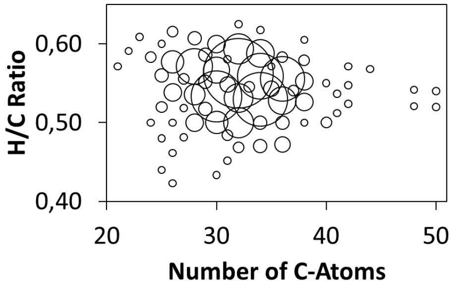
Figure 28. Number of species with a certain H/C-ratio over the number of C-atoms found for all generated structures grown from soot precursors for all fuel mixtures, equivalence ratios and temperatures. The size of the circles gives the amount of species found for a H/C-ratio and a number of carbon atoms. The smallest circles stand for a count of one species, while the biggest circle represents the amount of 73 species found with that H/C-ratio and that number of carbon atoms.
