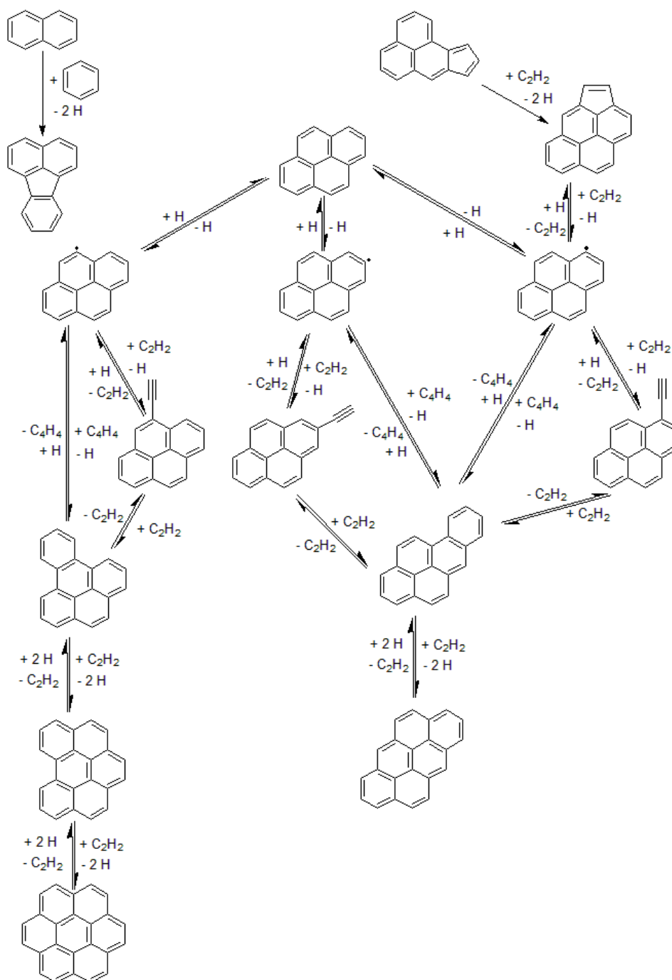
Figure 4. Reaction Pathway scheme for the growth of the PAHs in Raj's mechanism for all PAHs considered in the precursor pool.
