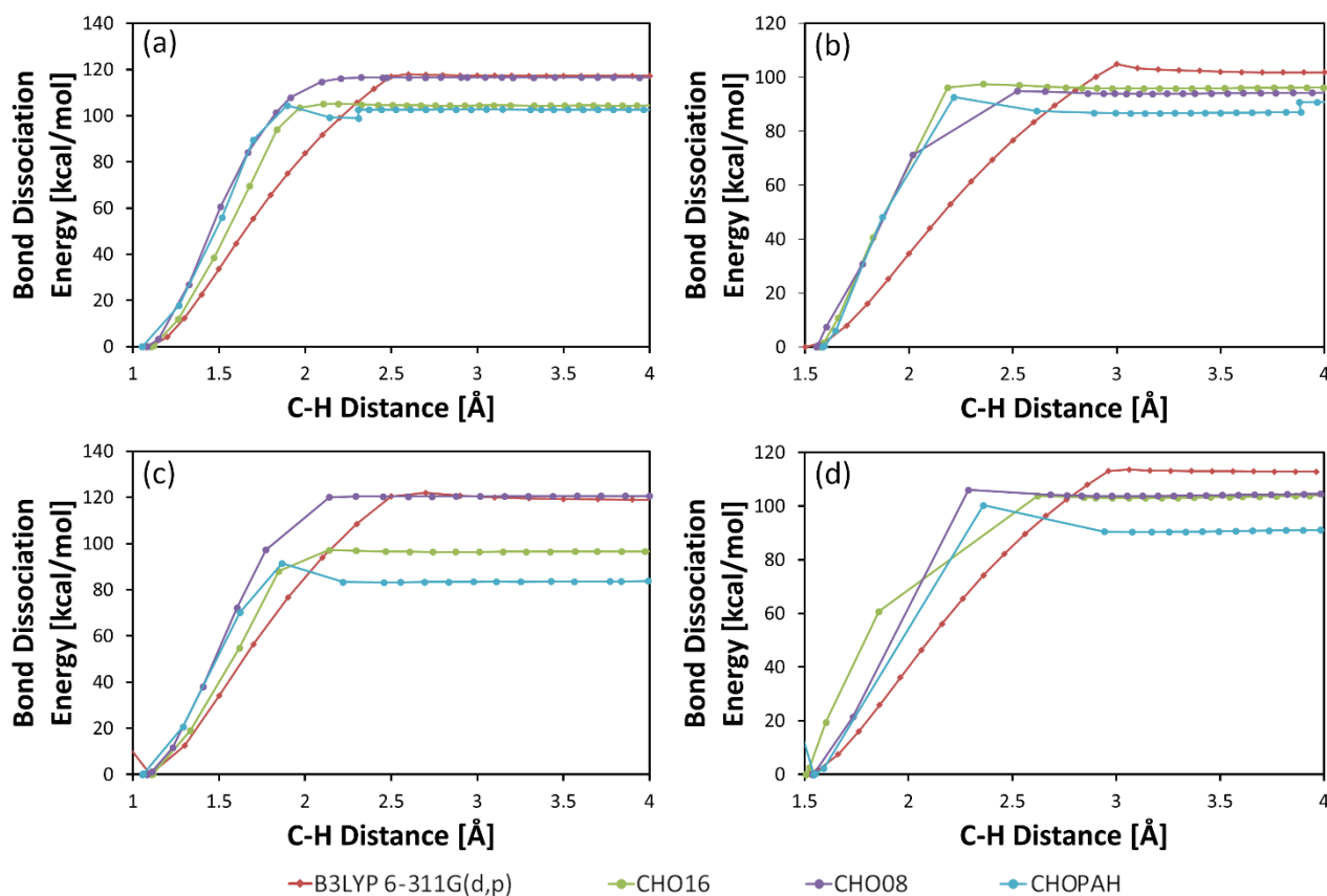
Figure 18. Bond dissociation energy calculations utilizing DFT and ReaxFF calculations for (a) hydrogen dissociation from benzene, (b) methyl dissociation from toluene, (c) hydrogen dissociation from pyrene, and (d) dissociation of biphenyl into two phenyl radicals. The energy of the relaxed bond distance has been normalized to 0 kcal/mol for all calculations.
