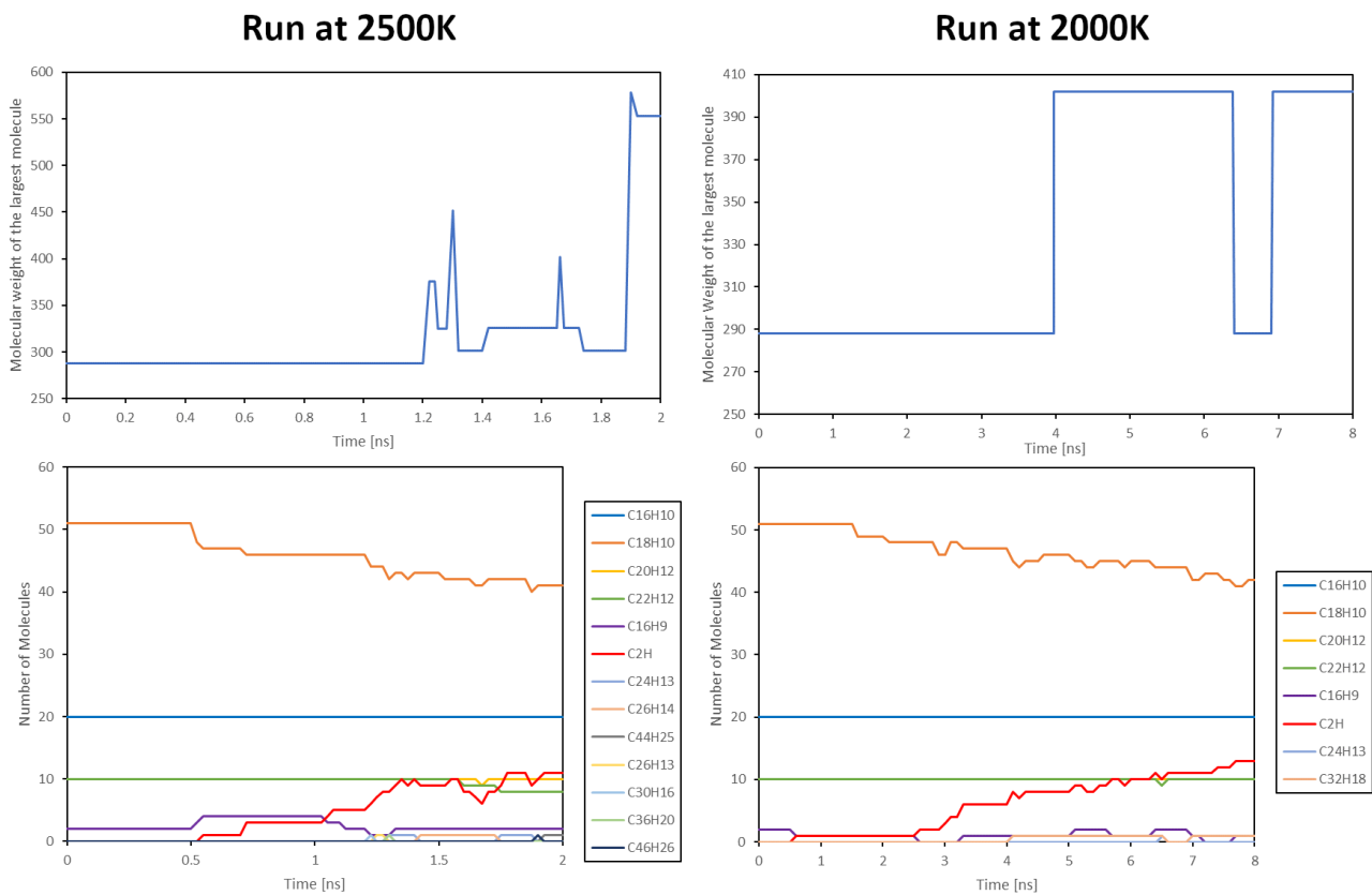
Figure 20. Graphs of the molecular weight of the largest molecule and the number of relevant molecular species found during the ReaxFF calculations over the simulation time. The calculations are performed with the precursor pools generated with Chemkin for a temperature of 2000 K, an equivalence ratio of 3.5 and a fuel mixture of pure n -decane. The ReaxFF calculation is performed at 2500 K (left side) and 2000 K (right side) to show the impact of temperature on the reactivity in the ReaxFF calculations.
