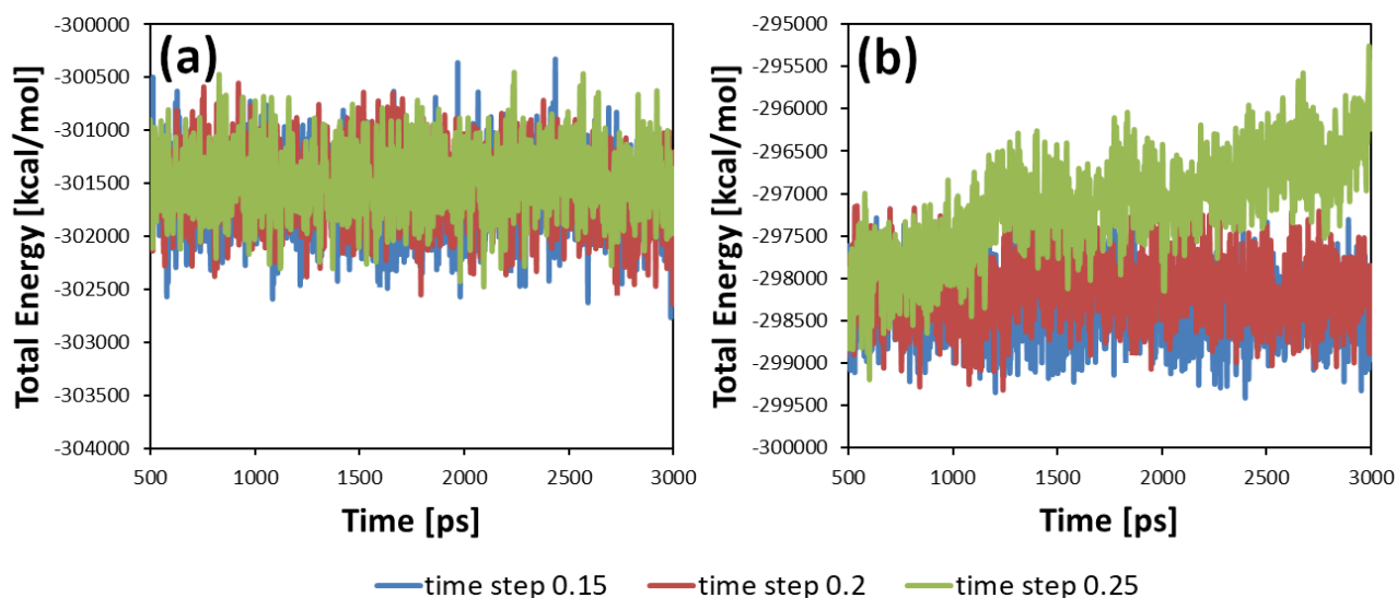
Figure 23. The total energy of the ReaxFF calculations over time for different time steps employed during the calculation for temperatures of (a) 1800 K and (b) 2000 K simulated in the ReaxFF calculations.
