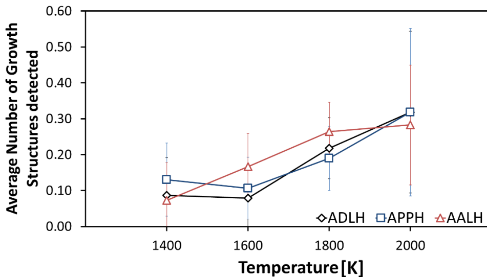
Figure 35. Number of detected growth structures through bond formation with different structural features plotted as a function of the temperature. The number of structures of each structural group are averaged for all equivalence ratios and fuel mixtures and distinguished by temperature. The vertical bars represent error bars.
