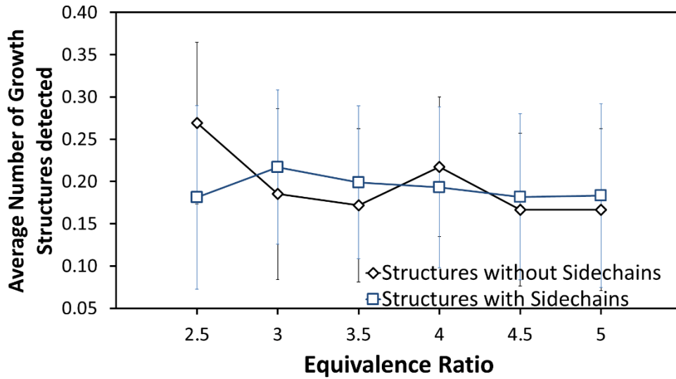
Figure 37. Number of detected growth structures through bond formation with and without sidechains plotted as a function of the equivalence ratio. The number of structures of each structural group are averaged for all temperatures and fuel mixtures and distinguished by equivalence ratio. The vertical bars represent error bars.
