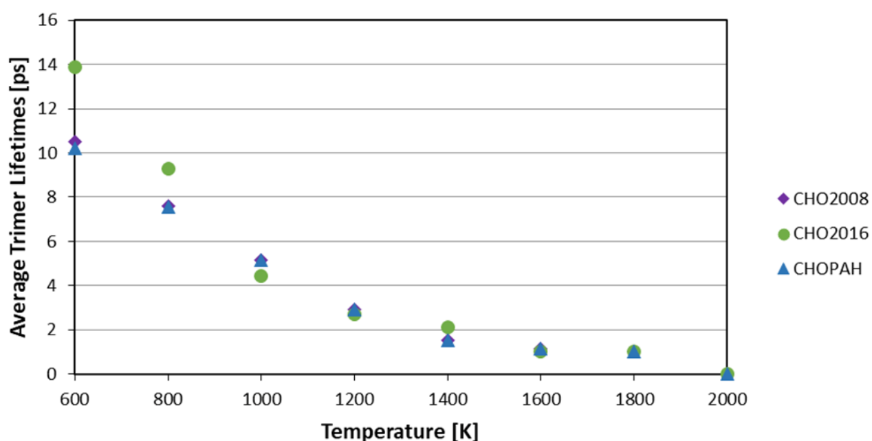
Figure 19. Average lifetimes of trimer structures detected during ReaxFF calculation performed for 2 ns at different temperatures for the three force fields investigated.
