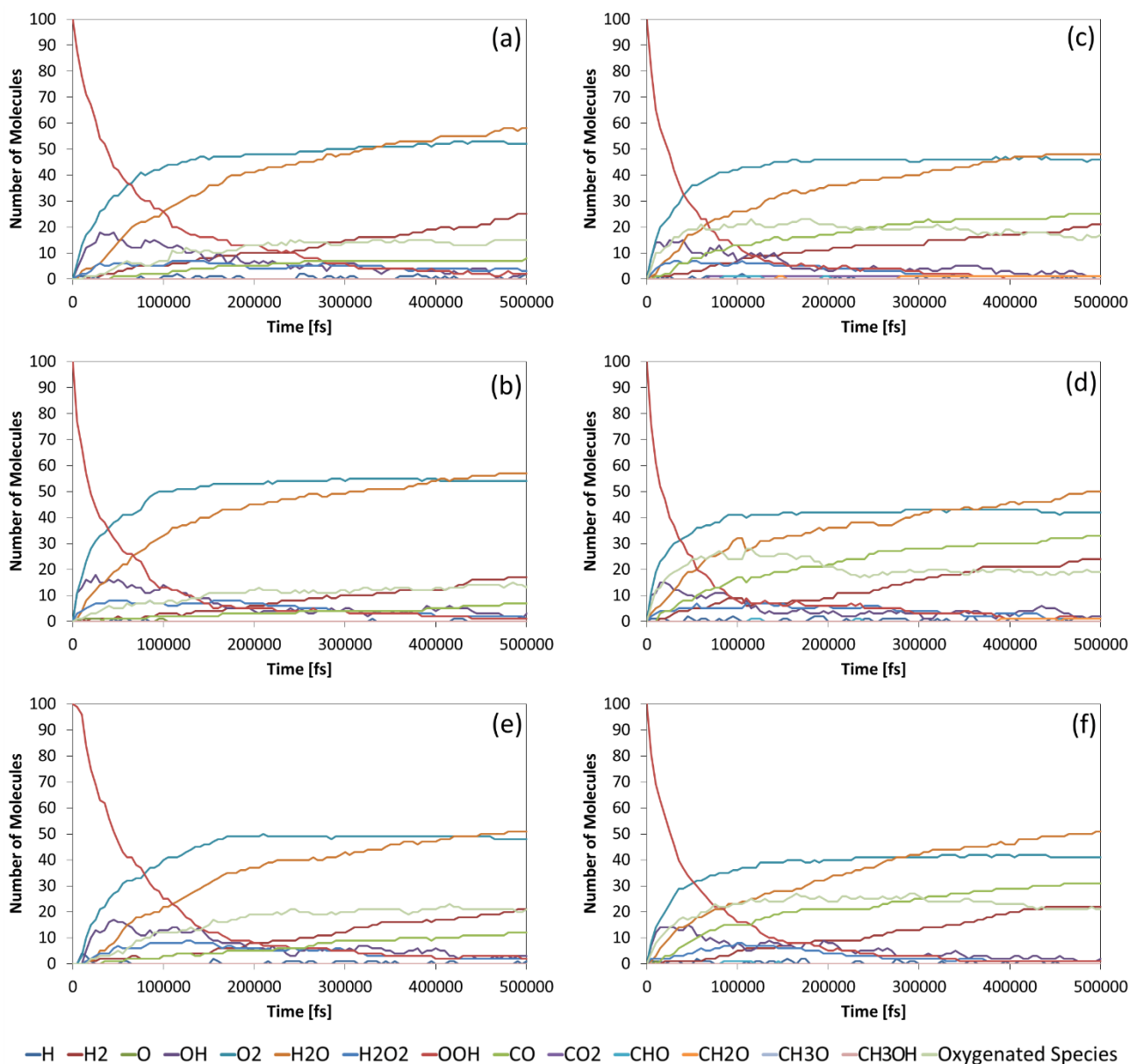
Figure 49. Number of oxygen containing molecules over time for the reactions of the nascent soot structures and hydroperoxyl. The results have been averaged over the three calculations performed at each condition. The corresponding calculations contain 100 hydroperoxyl radicals and (a) all ADLH species without sidechains, (b) all ADLH species with sidechains, (c) all APPH species without sidechains, (d) all APPH species with sidechains, (e) all AALH species without sidechains and (f) all AALH species with sidechains.
