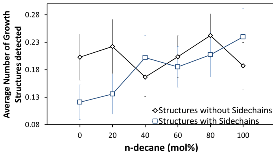
Figure 39. Number of detected growth structures through bond formation with and without sidechains plotted as a function of the n -decane mol fraction in the fuel mixture. The number of structures of each structural group are averaged for all equivalence ratios and temperatures and distinguished by fuel mixture. The vertical bars represent error bars.
