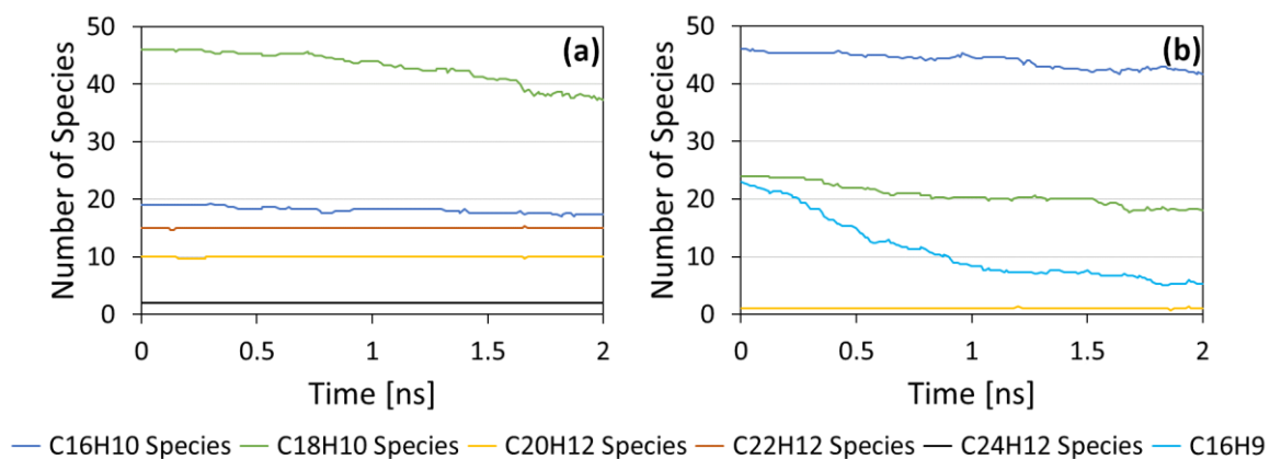
Figure 25. Consumption of the initial species present in the ReaxFF calculations plotted over the calculation time. The precursor pool compositions depicted represent the Chemkin calculations at (a) an equivalence ratio of 2.5, temperature of 1800K and a fuel mixture of pure-n-decane and (b) an equivalence ratio of 2.5, temperature of 2000K and a fuel mixture of 60 mol% n-decane and 40 mol% toluene.
