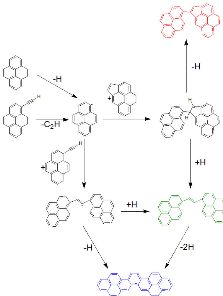
Figure 42. A schematic depiction of the most representative reaction pathways for the three structural groups found. The product for each structural group is highlighted in color. In order to help comprehension only forward reactions are shown.
