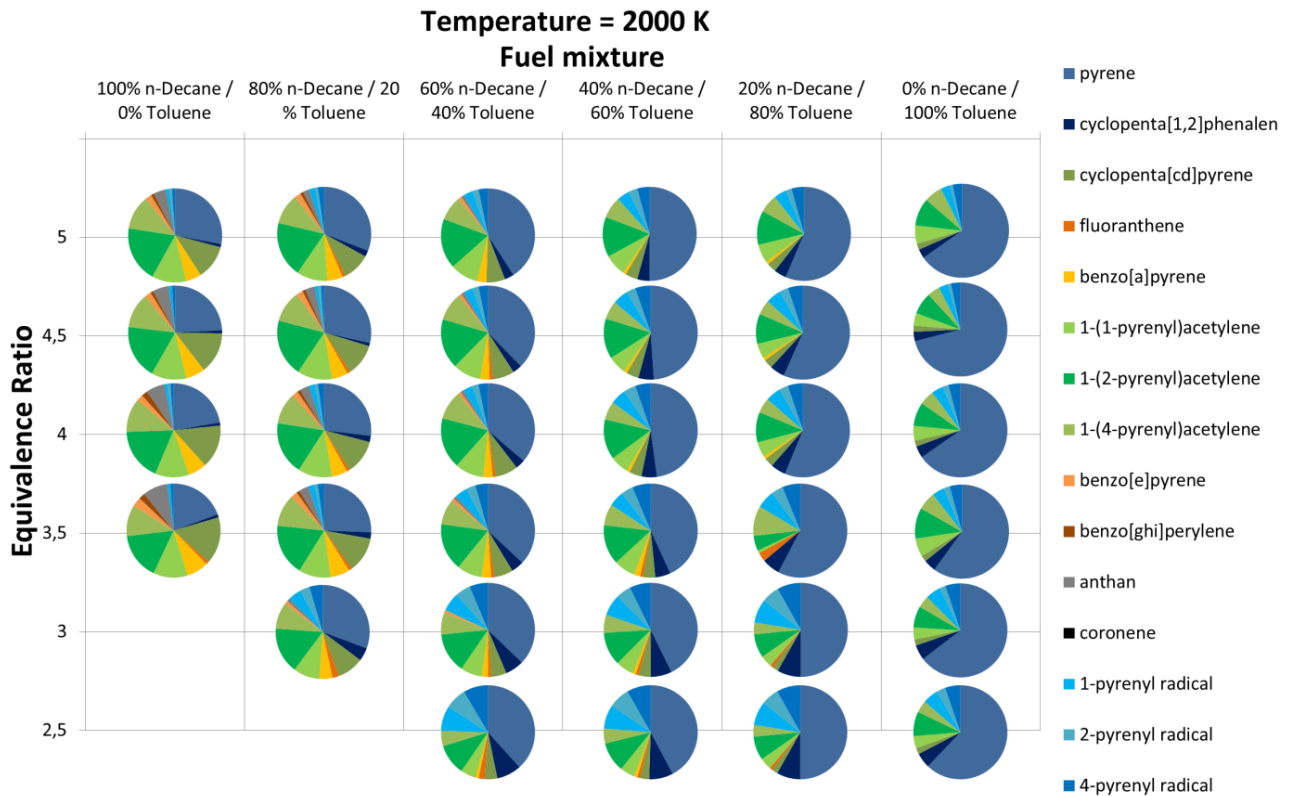
Figure 13. Pie chart of the soot precursor pool compositions at all equivalence ratios and fuel mixtures for a temperature of 2000 K in the Chemkin calculation. The color scheme of the soot precursors included in the compositions is given on the right-hand side. The size of each slice in the pie chart depicts the numerical proportion of the soot precursor of equal color in the composition.
