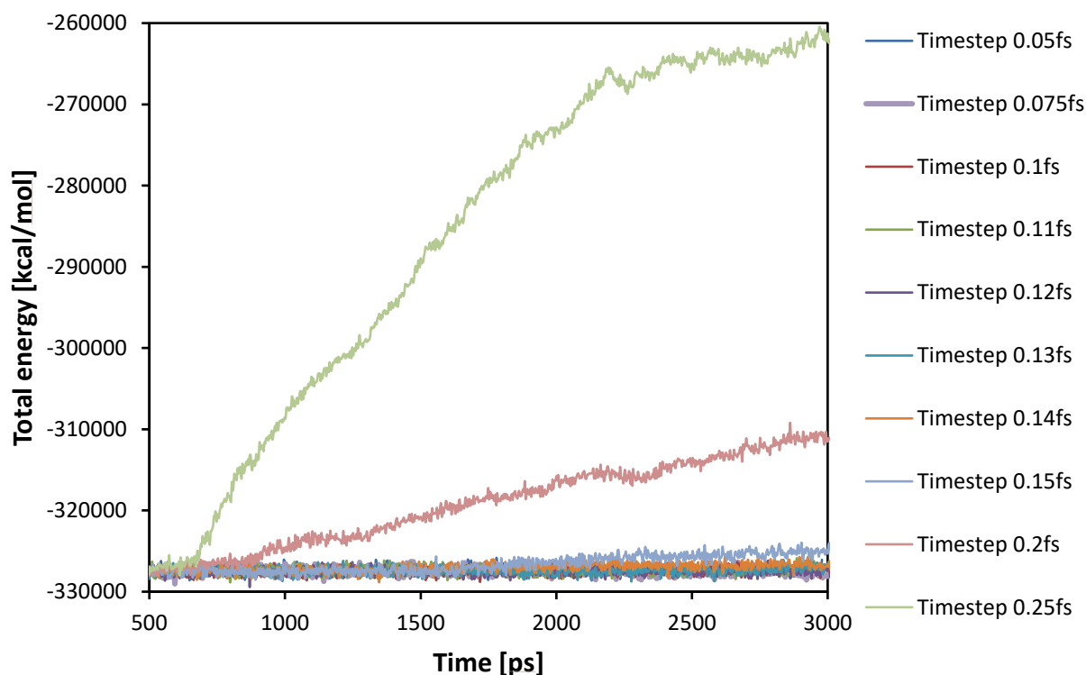
Figure 22. The total energy of the ReaxFF calculations over time for different time steps employed during the calculation for a simulated temperature of 2500 K. Failing to reproduce the results of smaller time steps indicates that the time step chosen is too large.
