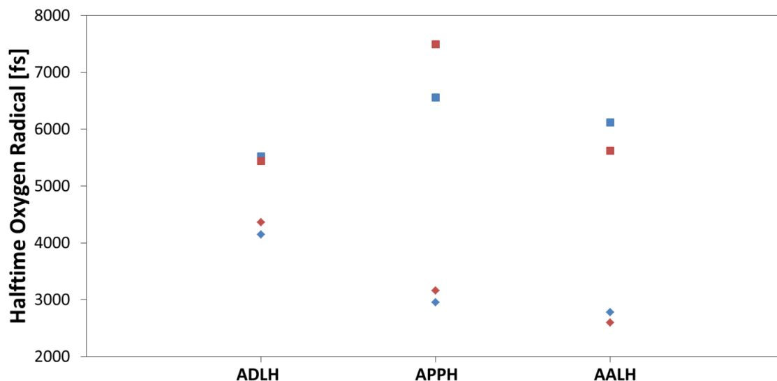
Figure 52. Average halftime of the atomic oxygen radicals for all calculations including all detected structures for one species (red) and the average halftime found for all calculations using representative species (blue), differentiated by species structural features and the species of one structural group with sidechains (diamonds) or without sidechains (square).
