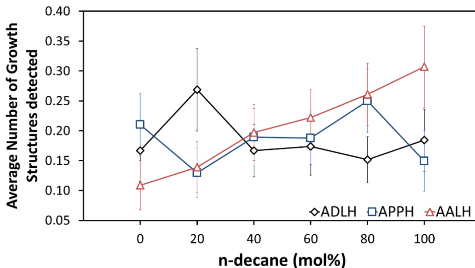
Figure 36. Number of detected growth structures through bond formation with different structural features plotted as a function of the n -decane mol fraction in the fuel mixture. The number of structures of each structural group are averaged for all equivalence ratios and temperatures and distinguished by fuel mixture. The vertical bars represent error bars.
