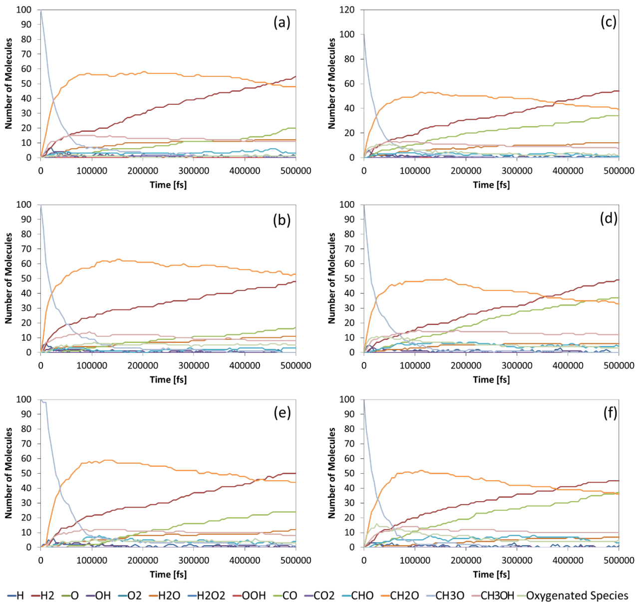
Figure 50. Number of oxygen containing molecules over time for the reactions of the nascent soot structures and methoxyl radicals. The results have been averaged over the three calculations performed at each condition. The corresponding calculations contain 100 methoxyl radicals and (a) all ADLH species without sidechains, (b) all ADLH species with sidechains, (c) all APPH species without sidechains, (d) all APPH species with sidechains, (e) all AALH species without sidechains and (f) all AALH species with sidechains.
