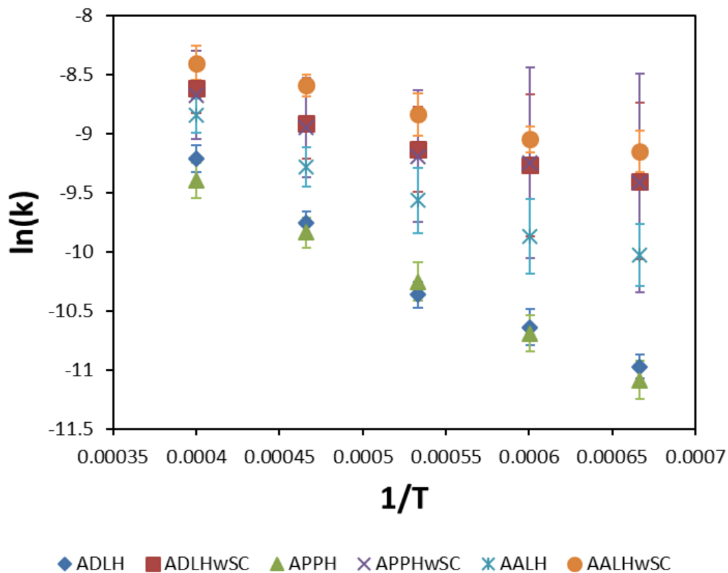
Figure 55. Natural logarithm of the fitted kinetic rate constant over the inverse temperature, for all differentiated species and a temperature range between 1500 K and 2500 K. The addition of “wSC” to the different structural groups denotes the presence of sidechains in the species of the structural group.
