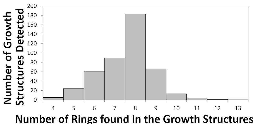
Figure 29. Bar diagram of the number of detected growth structures for all calculations at all temperatures, equivalence ratios and fuel mixtures over the number of pericondensed rings found in the structure.
