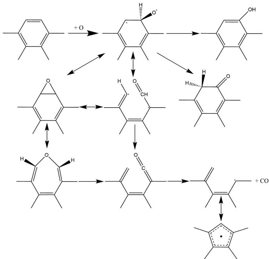
Figure 45. Detected reaction pathways for the addition of atomic oxygen to free edge sites of aromatic hydrocarbons.
