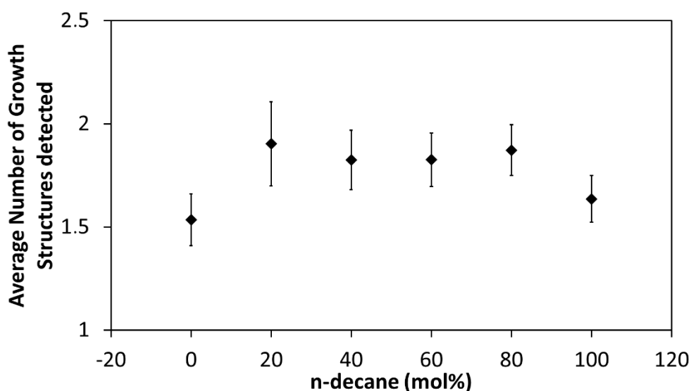
Figure 32. Number of all detected growth structures through bond formation as a function of n -decane mol fraction in the fuel mixture. The number of structures is averaged for all temperatures and equivalence ratios and distinguished by fuel mixture. The vertical bars represent error bars.
