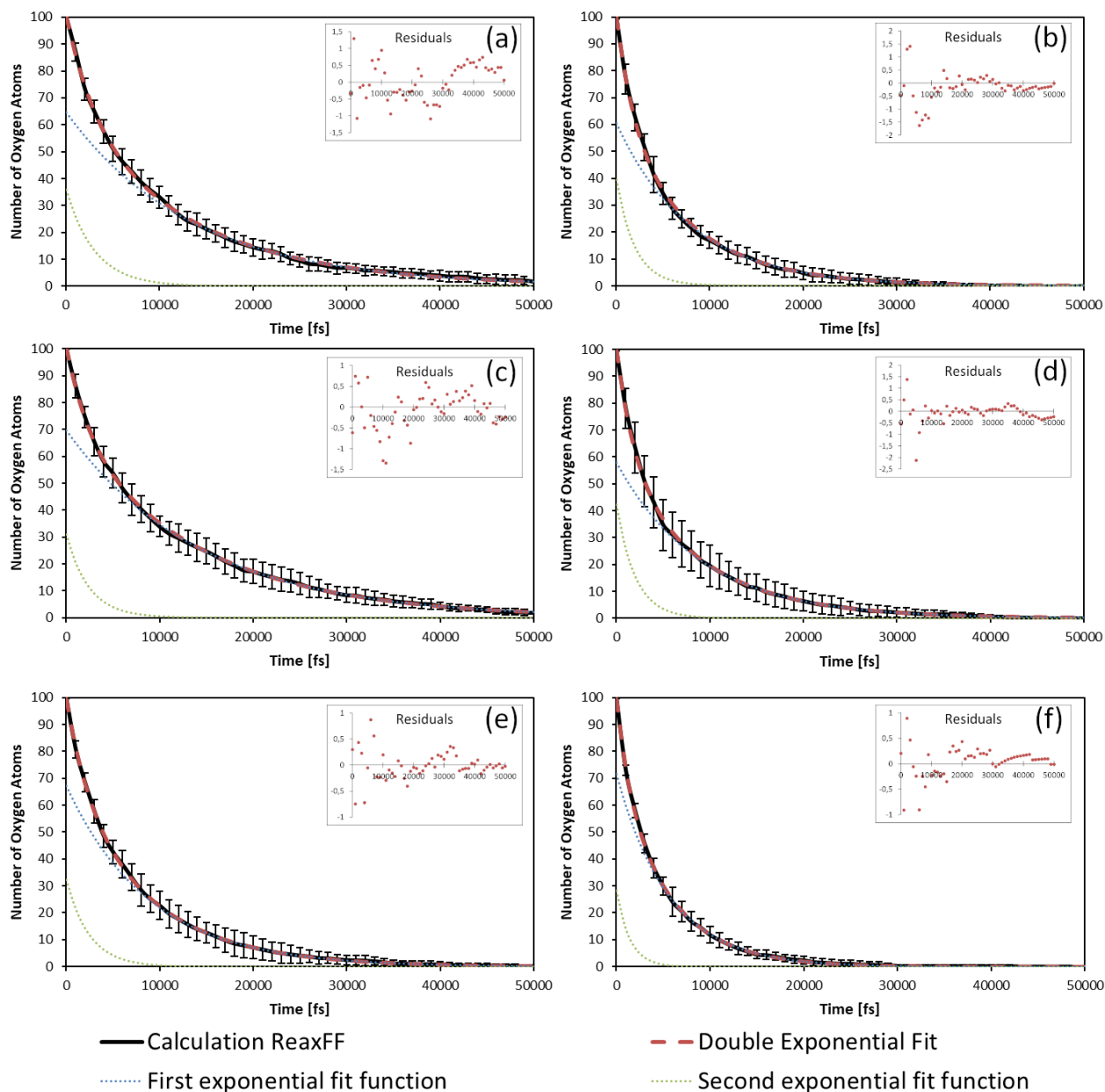
Figure 56. Number of atomic oxygen radicals over time (black) for (a) all ADLH species without sidechains, (b) all ADLH species with sidechains, (c) all APPH species without sidechains, (d) all APPH species with sidechains, (e) all AALH species without sidechains and (f) all AALH species with sidechains. The dashed red line gives the double exponential fit of the consumption of atomic oxygen during the calculation, with the two single exponential functions displayed as dotted blue and dotted green line. The residuals of the fit are given in the upper right corner of each graph.
