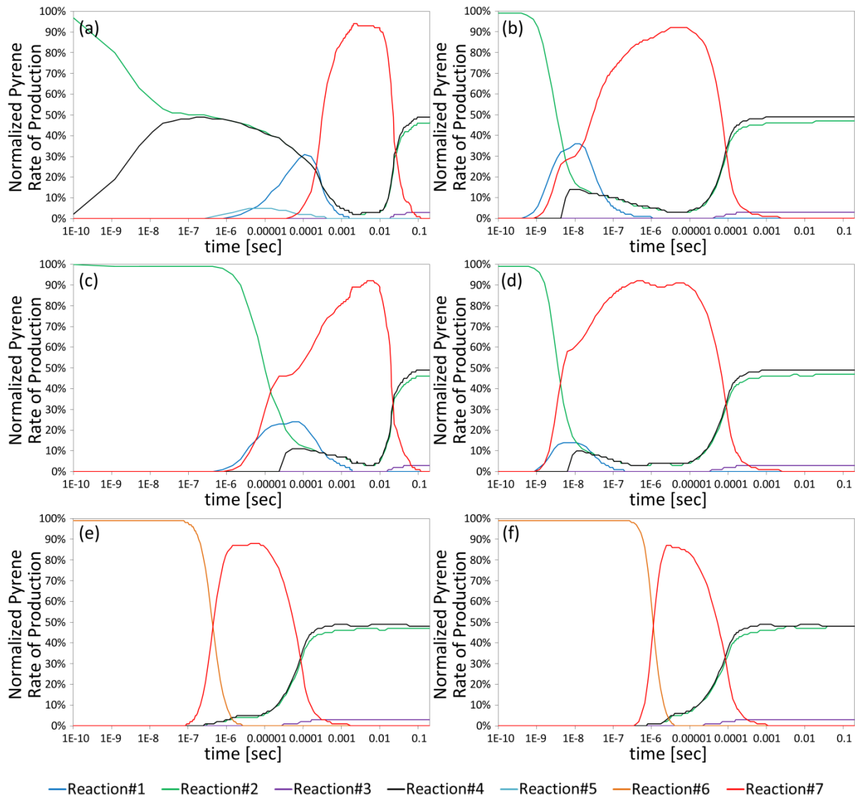
Figure 17. Percentage contribution to the positive ROP of pyrene by each reaction detected to contribute to the growth of pyrene. The numbering of the reactions follows the numbering shown in Table 12. The chosen conditions depicted are taken at an equivalence ratio for 3.5, a temperature of 2000K and a fuel mixture of (a) 100 mol% n-decane, (b) 80 mol% n-decane and 20 mol% toluene, (c) 60 mol% n-decane and 40 mol% toluene, (d) 40 mol% n-decane and 60 mol% toluene, (e) 20 mol% n-decane and 80 mol% toluene, and (f) 100 mol% toluene, to show the impact of fuel composition on the percentage contribution of each reaction. Reactions not shown in one of the graphs did not exceed 1% with respect to the total pyrene ROP.
