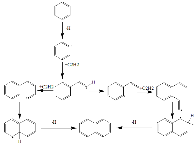
Figure 2. H-abstraction-carbon-addition mechanism for the growth of the second aromatic ring.
