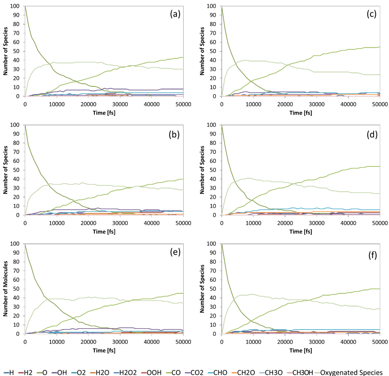
Figure 43. Number of oxygen containing molecules over time for the reactions of the nascent soot structures and atomic oxygen. The results have been averaged over the three calculations performed at each condition. The corresponding calculations contain 100 atomic oxygen radicals and (a) all ADLH species without sidechains, (b) all ADLH species with sidechains, (c) all APPH species without sidechains, (d) all APPH species with sidechains, (e) all AALH species without sidechains and (f) all AALH species with sidechains.
