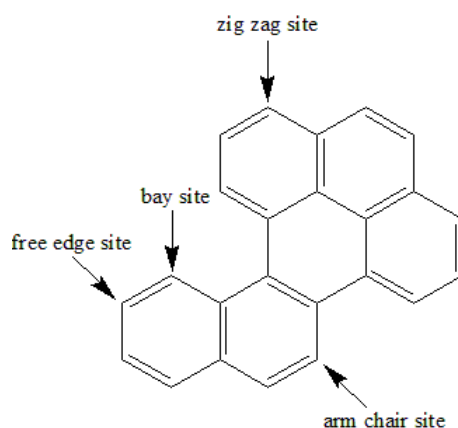
Figure 3. Different H-abstraction sites of PAHs.
