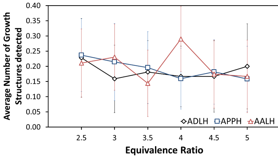
Figure 34. Number of detected growth structures through bond formation with different structural features plotted as a function of the equivalence ratio. The number of structures of each structural group are averaged for all temperatures and fuel mixtures and distinguished by equivalence ratio. The vertical bars represent error bars.
