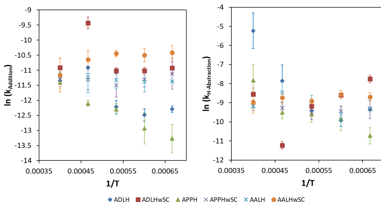
Figure 59. Natural logarithm of the fitted kinetic rate constant of hydroxyl consumption of the first exponential function of the double exponential fits (left) and the second exponential function of the double exponential fit (right) over the inverse temperature, for all differentiated species and a temperature range between 1500 K and 2500 K. The addition of “wSC” to the different structural groups denotes the presence of sidechains in the species of the structural group.
