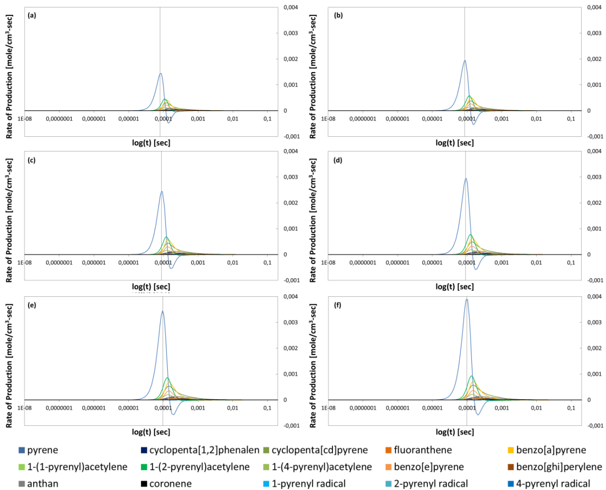
Figure 6. Rates of production of the extracted PAH (shown in Figure 9) over the simulation time for the Chemkin calculations performed with a temperature of 1600K and a fuel mixture of 0 mol% n-decane and 100 mol% toluene, and equivalence ratios of (a) 2.5, (b) 3, (c) 3.5, (d) 4, (e) 4.5, and (f) 5.
