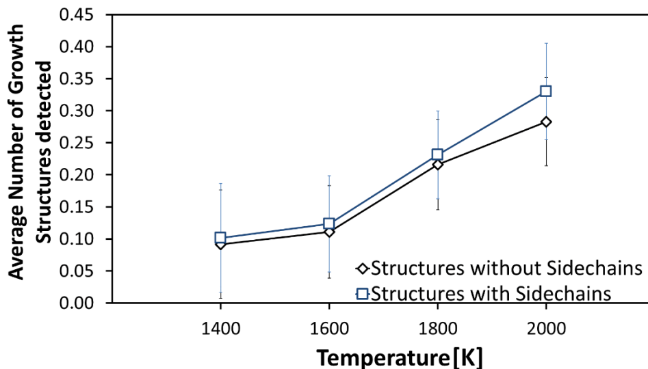
Figure 38. Number of detected growth structures through bond formation with and without sidechains plotted as a function of the temperature. The number of structures of each structural group are averaged for all equivalence ratios and fuel mixtures and distinguished by temperature. The vertical bars represent error bars.
