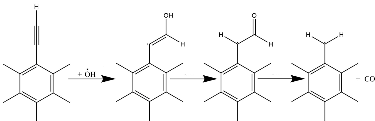
Figure 48. Detected reaction pathway for the addition of hydroxyl radicals to terminal sidechain carbon.
