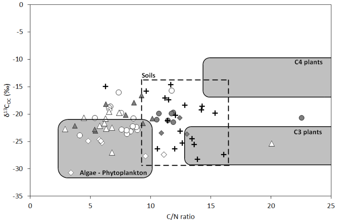
Figure III.7 : Relation between C/N ratio and isotopic composition of particulate (open markers), sediment (filled markers) and soil (crosses) organic carbon for the Nyando (circles), the Lufilyo (diamonds) and the Tukela (triangles) catchments.
