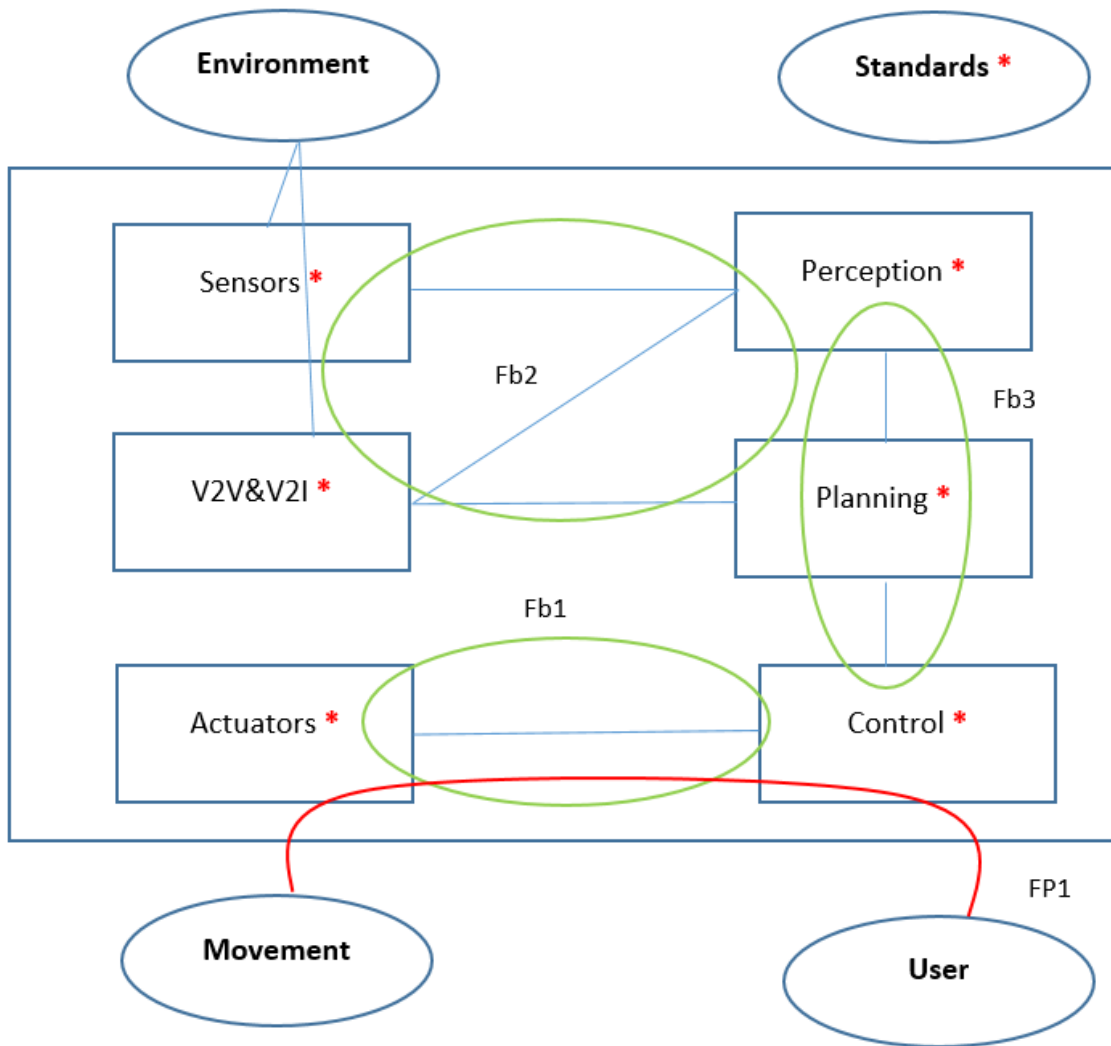
Figure 3-6 Global functional block diagram for CAV
