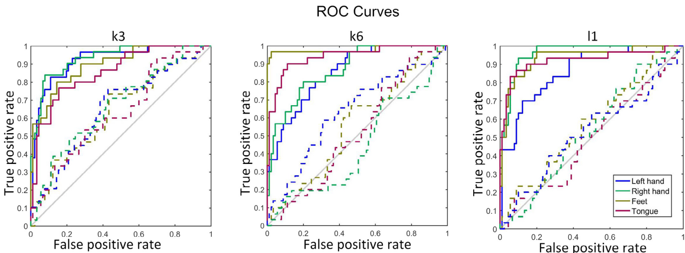
Fig. 5. ROC curves for our method (MTFS, solid lines) in comparison to using the broad band, full length data (dashed lines).
