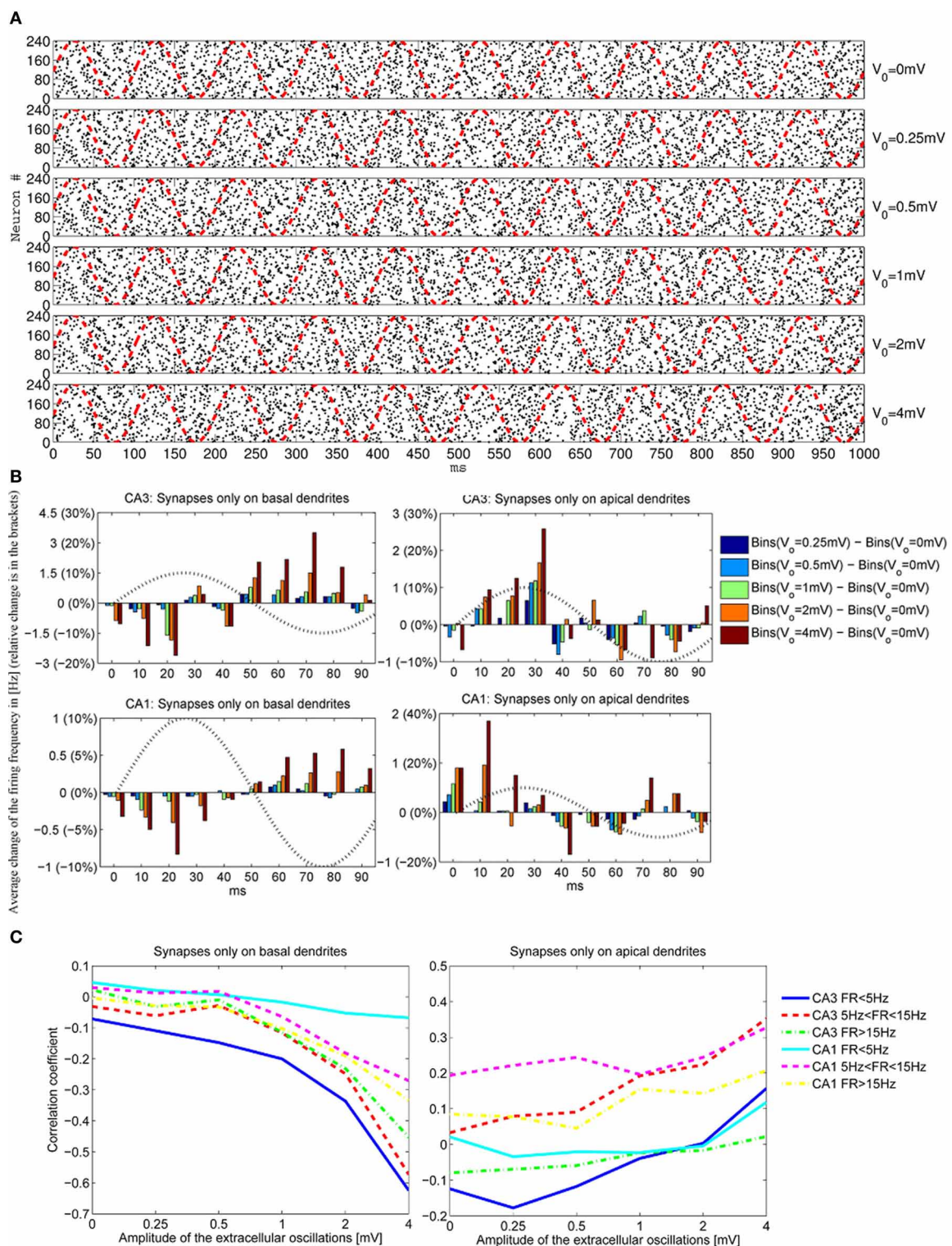
FIGURE 7 | (A) The raster plots showing firing times of CA3 neurons for different amplitudes of the extracellular oscillations, V_o = 0, 0.25, 0.5, 1, 2 and 4\text{mV} , across 48 iterations for 5 morphologies, resulting in 240 spike trains. The phase of the extracellular oscillations is given with red dashed lines. (B) The average (across all 240 iterations) difference between the firing frequencies with and without the extracellular oscillations. Additionally, an observation of 1 s for each
