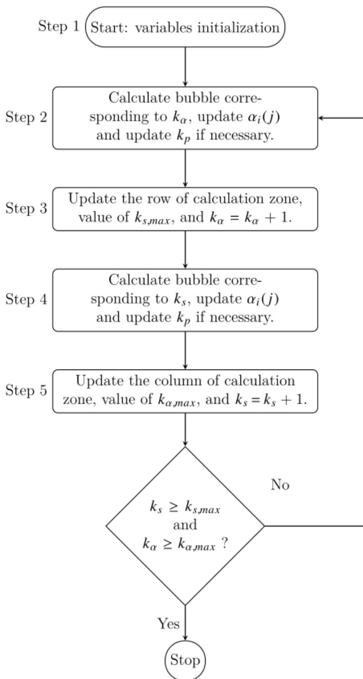
Figure 5.8: Flow chart of the proposed simplified min-sum processing algorithm.
