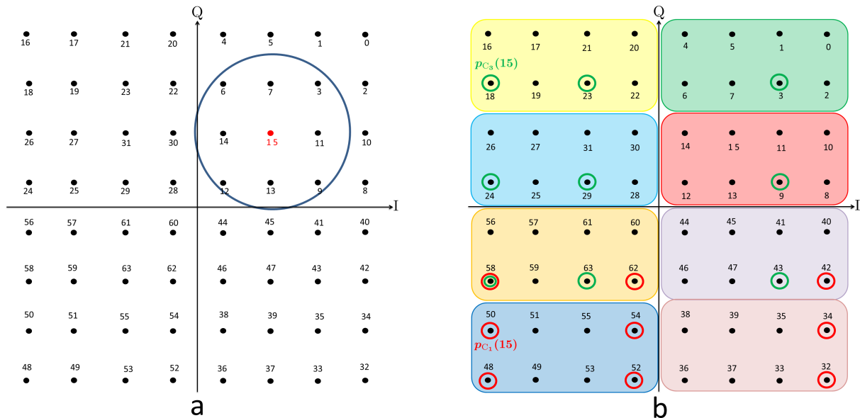
Figure 3.16: (a) Example of a transmitted systematic symbol (15) with its neighborings competing symbols in the 64-QAM constellation. (b) Resulting parity symbols for the systematic competing symbols of (a), for code C_1 (red circles) and code C_3 (green circles).
