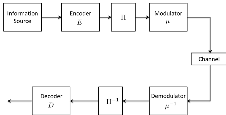
Figure 1.4: Block diagram of a transmission with Coded Modulation (CM) or Bit Interleaved Coded Modulation (BICM).
