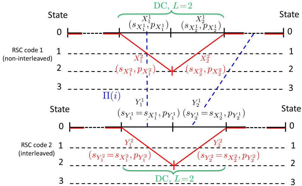
Figure 4.2: Example of competing DC sequences of length L = 2 in the trellises of both RSC codes of a NB-TC over GF(4).
