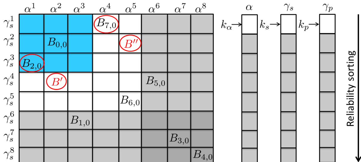
Figure 5.7: Example of sorting table used for the computation of \alpha_i(0) with Eq. (5.12) for q = 8 . All B(j', 0) values, j' = 0 \dots q - 1 are placed in different rows and columns. Min-sum processing is performed with radius R = 3 , k_{s,\max} = k_{\alpha,\max} = n_m = 5 . Illustration of Steps 2 and 3 (resp. Steps 4 and 5) for k_\alpha = 1 (resp. for k_s = 1 ), and illustration of sorted vectors \alpha , \gamma_s and \gamma_p .
