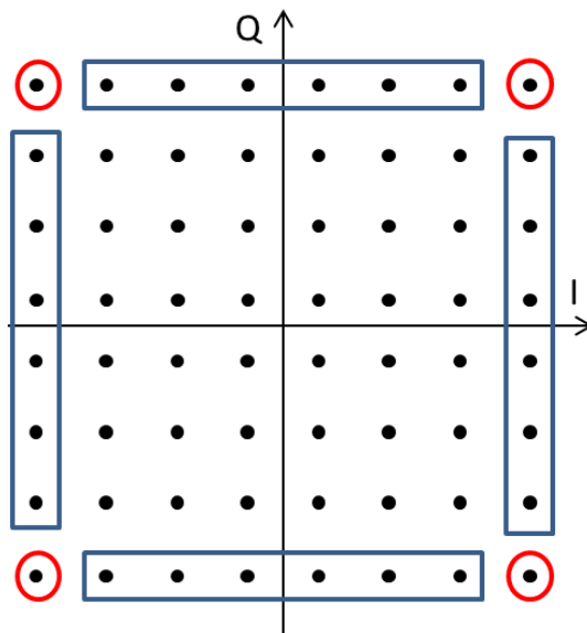
Figure 4.4: 64-QAM constellation with different protection levels for symbols.
