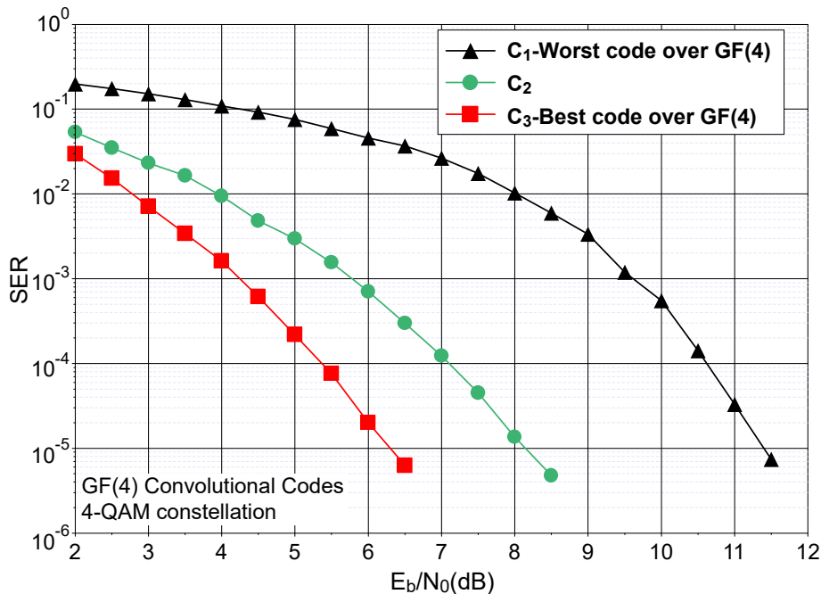
Figure 2.12: Performance comparison of rate-1/2 convolutional codes over GF(4) in terms of symbol error rates in AWGN channel.
