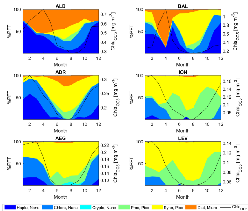
Figure A2.9: Monthly Climatology of dominant PFT frequency alongside the Chla OC5 at the Alboran, Balearic, Adriatic, Ionian, Aegean and Levantine basins
