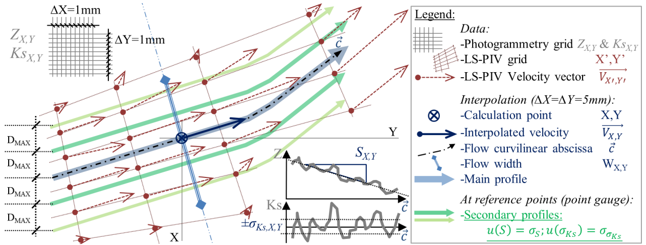
Figure 6.9 – Sketch of the friction law parameters extraction algorithm: extraction of the flow slope S_{X,Y} and roughness standard deviation \sigma_{K_{X,Y}} along curvilinear profiles following the flow direction defined by LS-PIV velocity data. Main profile defined parallel to the main stream line passing by X,Y and additional uncertainty measurements at reference points (underlined steps).
