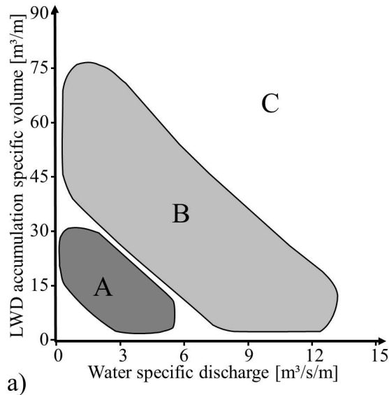
A: Net dams B: V-shaped sectional dams with piles C: Other structures, e.g.: -additional inclined rakes upstream of slot dams - « Austrian type »: integrated structure with multiple inclinations upstream of large slot dams
