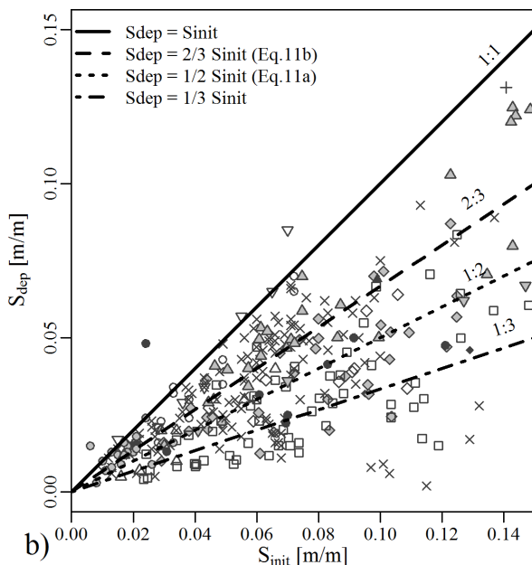
Figure 2.12 – Comparison of the deposition slope and the initial channel slope on a data set with 456 field measurements: a) within the complete range and b) zoom on the slopes < 0.15. Confirmation of the nearly systematic relation S_{dep} \leq S_{init} (Numbers between brackets are the number of data of each reference)
