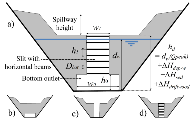
Figure 2.3 – Definition of shape parameters for water stage-discharge equation; example of a) a slit dam with horizontal beams and a slot as the bottom outlet, b) a slot dam, c) a slit dam and d) a slit dam with horizontal beams (adapted from Zollinger, 1983, with permission)
