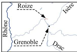
Figure 4.2 – Location of the Roize catchment and main geomorphology and structures, indication of catchment and sub-catchment area, lower and top elevation, roughness index (Melton, 1965), outlet bed slope, bed-surface grain size and channel width
