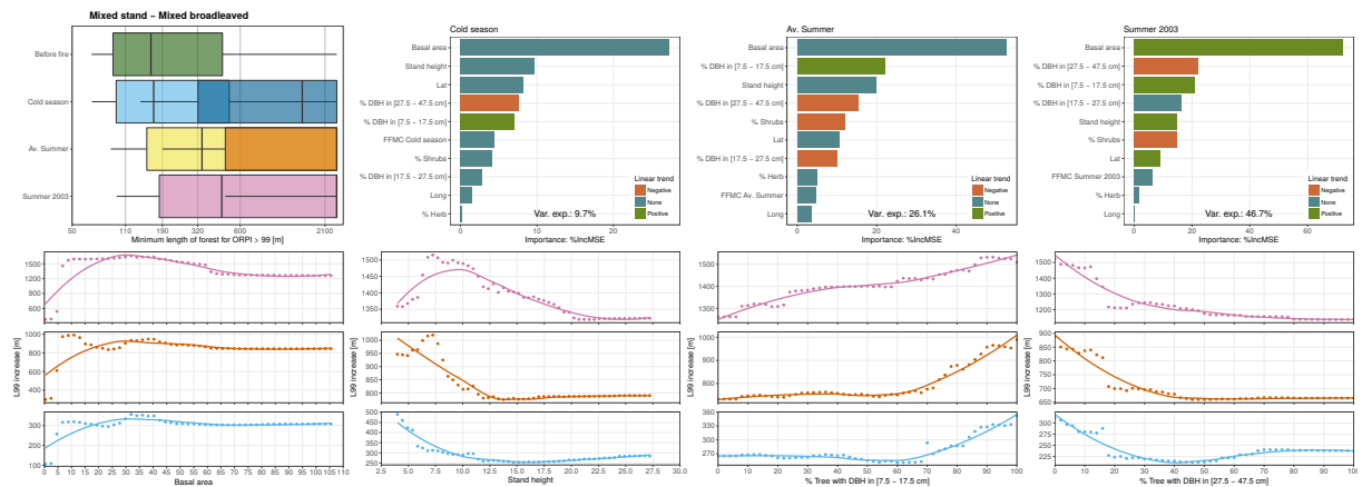
FIGURE C.16 – Result of regression forest for mixed stands of broadleaved species.
