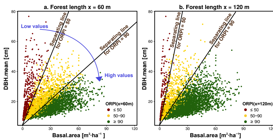
FIGURE 3.3 – Illustration of the clockwise motion of ORPI values for a rock volume of 1 \text{ m}^3 at forest lengths x=60 \text{ m} (a.) and x=120 \text{ m} (b.). Points are coloured according to ORPI(x) . The separating lines between plots were ORPI(x) < 90 (or 50 ) and plots were ORPI(x) \geq 90 (or 50 ) are shown. (Figure adapted from Dupire et al. (2016a))
