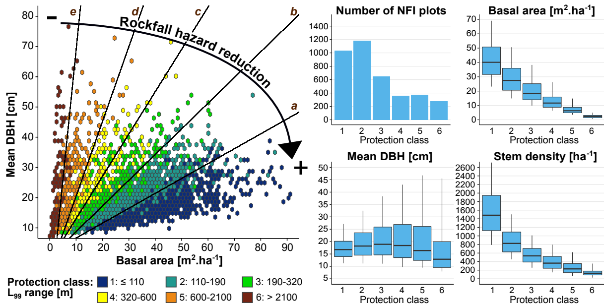
FIGURE 3.5 – Classification with the separating lines method (Dupire et al., 2016a) with a rock volume of 1 \text{ m}^3 . For a better visualization, NFI plots were grouped by hexagonal pixels, the colour represents the average value of the L_{99} of all the NFI plots contained in the pixel. The number of NFI plots per class and the distribution of the basal area, mean DBH and stem density are also shown.
