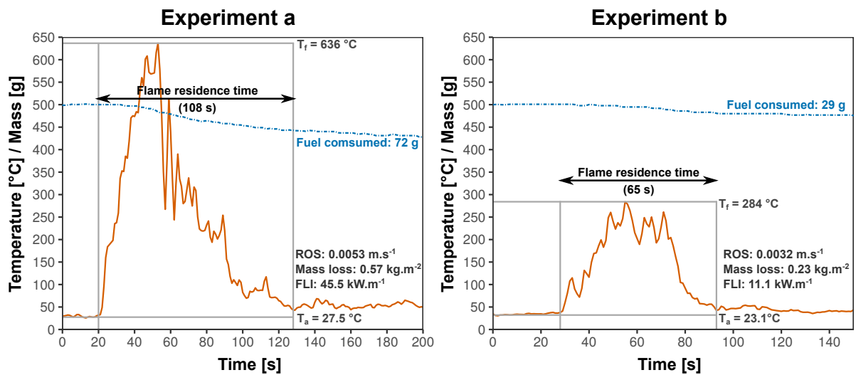
FIGURE 3.4 – Examples of temperature (orange solid line) and mass (dashed blue line) profiles measured along time during two different litter flammability experiments.
