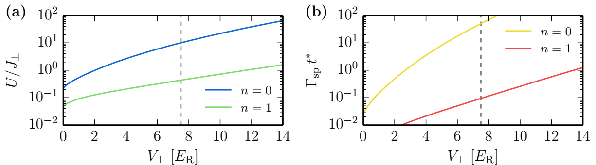
Figure 4.21: Figures of merit for the validity of the model presented in Section 4.3 for atoms in the fundamental band n = 0 and atoms in the first excited energy level n = 1 . In both curves the vertical gray dashed line denote the depth above which the first excited band is bound. (a) Ratio U/J_{\perp} . (b) Time scale \Gamma_{\text{sp}} t^* .
