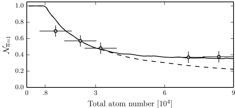
Figure 3.7: Normalised population \mathcal{N}_{\bar{n}=1} in the shell with unit filling fraction as a function of total initial atom number in the lattice. Open symbols show the measurements using the asymptotic value of the total population after many Rabi oscillations as presented in Figure 3.6b. The dashed line is the prediction from our loading model without three-body losses. The solid line accounts phenomenologically for three-body recombination processes which prevent sites with triple occupancy. Figure adapted from Bouganne et al. (2017).
