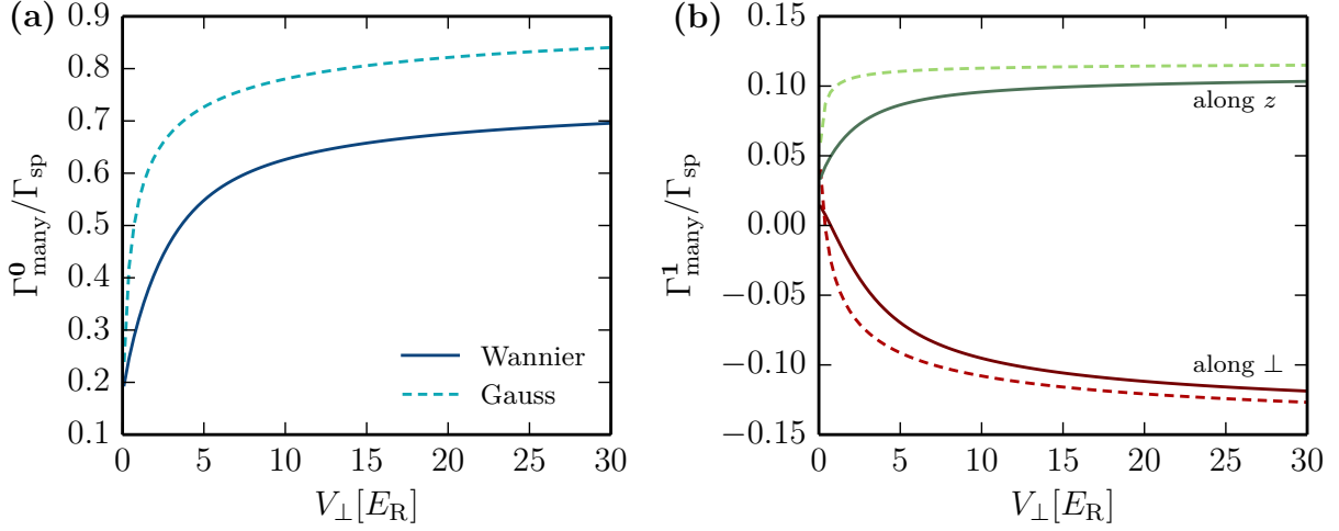
Figure 5.12: Two-body collective contribution \Gamma_{\text{many}}^i to the spontaneous emission rate in units of the single-particle spontaneous emission rate \Gamma_{\text{sp}} , for various horizontal lattice depth V_{\perp} . The vertical lattice depth is V_{0,z} = 27 E_R . Solid lines show the numerical computation using Wannier wavefunctions. Dashed lines shows the analytical expression for a Gaussian ansatz. (a) On-site rate \Gamma_{\text{many}}^0 . (b) Nearest-neighbour rate \Gamma_{\text{many}}^1 for nearest-neighbour along the vertical z direction and along the horizontal \perp direction.
