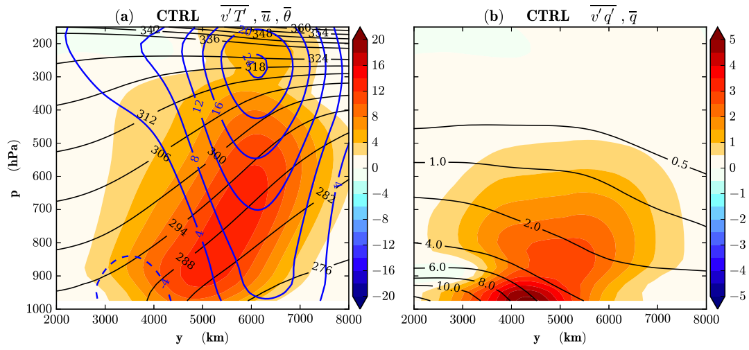
FIG. 3. Storm-track properties of the CTRL experiment. (a) Zonal wind (blue contours, in m s -1 ), 2-10 days filtered meridional flux of temperature (shadings, in K m s -1 ) and potential temperature (black contours, in K). (b) Specific humidity (contours, in g kg -1 ) and (2-10 days filtered) meridional flux of specific humidity (shadings, in g kg -1 m s -1 ).
