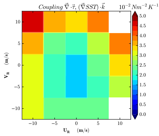
FIG. 10. Regression coefficient of wind stress divergence and downwind SST gradient anomalies as a function of the large-scale background wind at 10 meters, in 10^{-2} \text{ N/m}^2/\text{K} .
