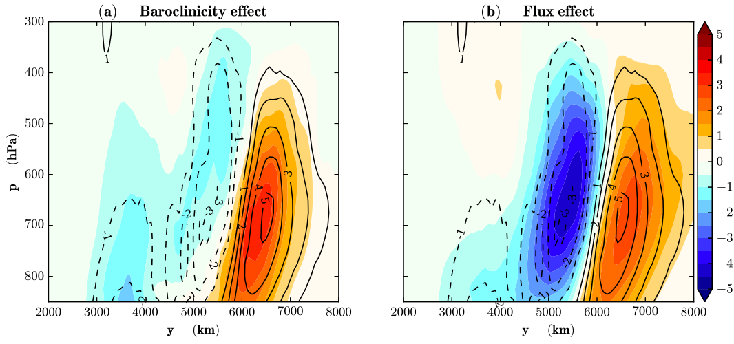
FIG. 11. Decomposition of the EDDY-CTRL difference between the contribution to baroclinic conversion of (a) change of Eady growth rate at a constant heat flux and (b) change of heat flux at constant Eady growth rate. Contours represent the total baroclinic conversion in the 2-10 days band. All terms are in \text{m}^2 \text{s}^{-2} \text{day}^{-1} .
