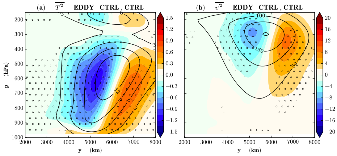
FIG. 7. Same as Fig. 5, but for zonal and time average of (a) \langle T'T' \rangle (in \text{K}^2 ) and (b) \langle v'v' \rangle (in \text{m}^2\text{s}^{-2} ). Regions with significant variance differences are shaded with black dots.
