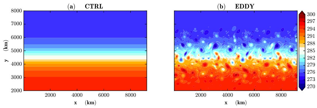
FIG. 1. SST fields (in K). (a) CTRL and (b) EDDY experiments.
