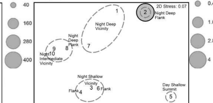
Figure 4.7 Bubble plot overlays of the MDS ordination representing the relative abundance of common (c) deep dwelling, (d) and seamount flank associated species. Trawl stations are numbered 1 to 10 on the bubble plots and dotted lines denote the 42% similarity clusters. The larger the bubble, the greater the number of individuals captured at that trawl station.
