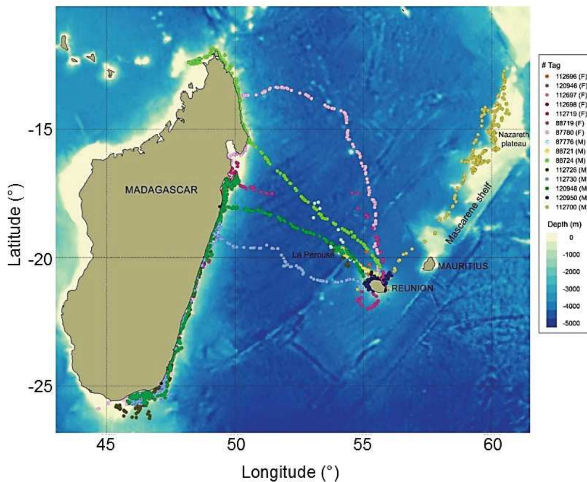
Figure 1.11 Received Argos locations from humpback whales tagged in R union in 2013 (F: Female, M: Male). Male humpback whales engaged in localized behaviour in R union Island, La P erouse seamount, St Brandon Shoal and Madagascar, while females engaged in localized behaviour at R union Island and Ile Sainte-Marie (Source: Dulau et al., 2017).
