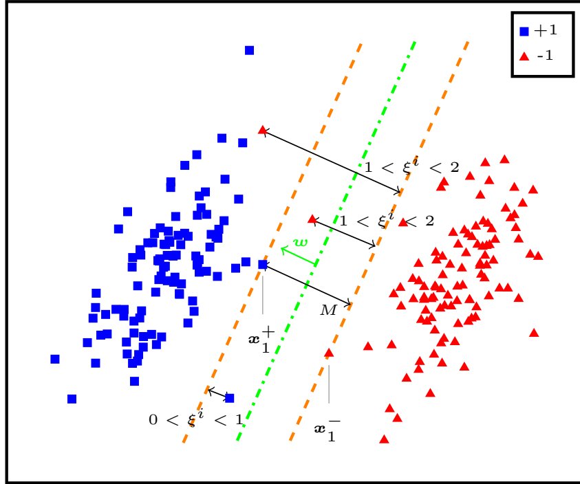
Figure B.2: Illustration of a soft margin SVM. The orange lines ( resp. green line) correspond to the support hyperplanes ( resp. separator). Dataset points are allowed to be inside the margin and even in the other side of the separator. It helps fit a natively linear classifier in a non linearly separable case.
