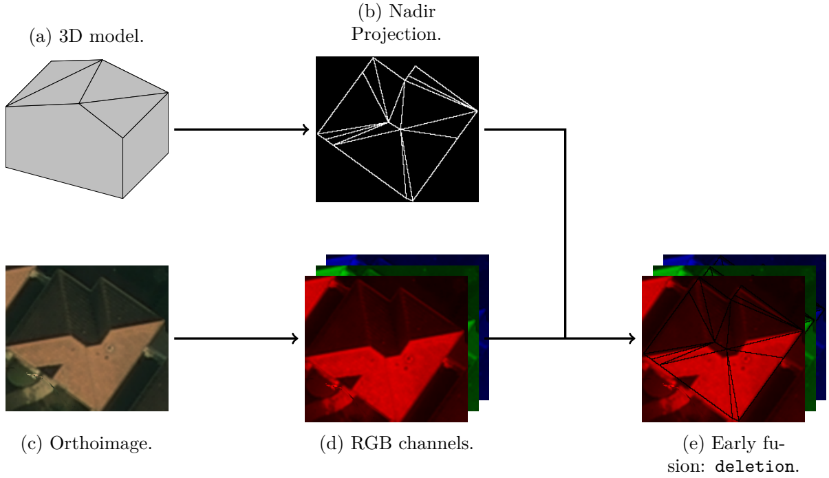
Figure 6.6: Illustration of the early fusion scheme denoted deletion . Pixels that intersect the edges of the nadir projection of the model are blackened.
