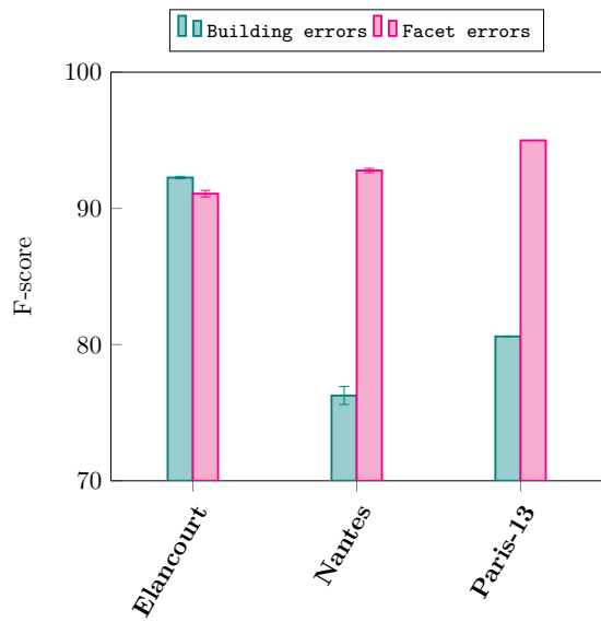
(a) Test scores for classifiers trained on the same zone.
