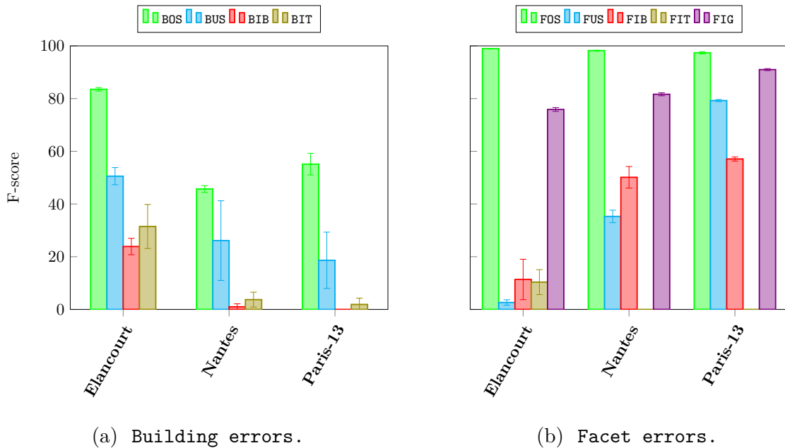
Figure 5.9: Visualizing mean F-score and standard deviation for the feature ablation study. Details are reported in Table C.3.
