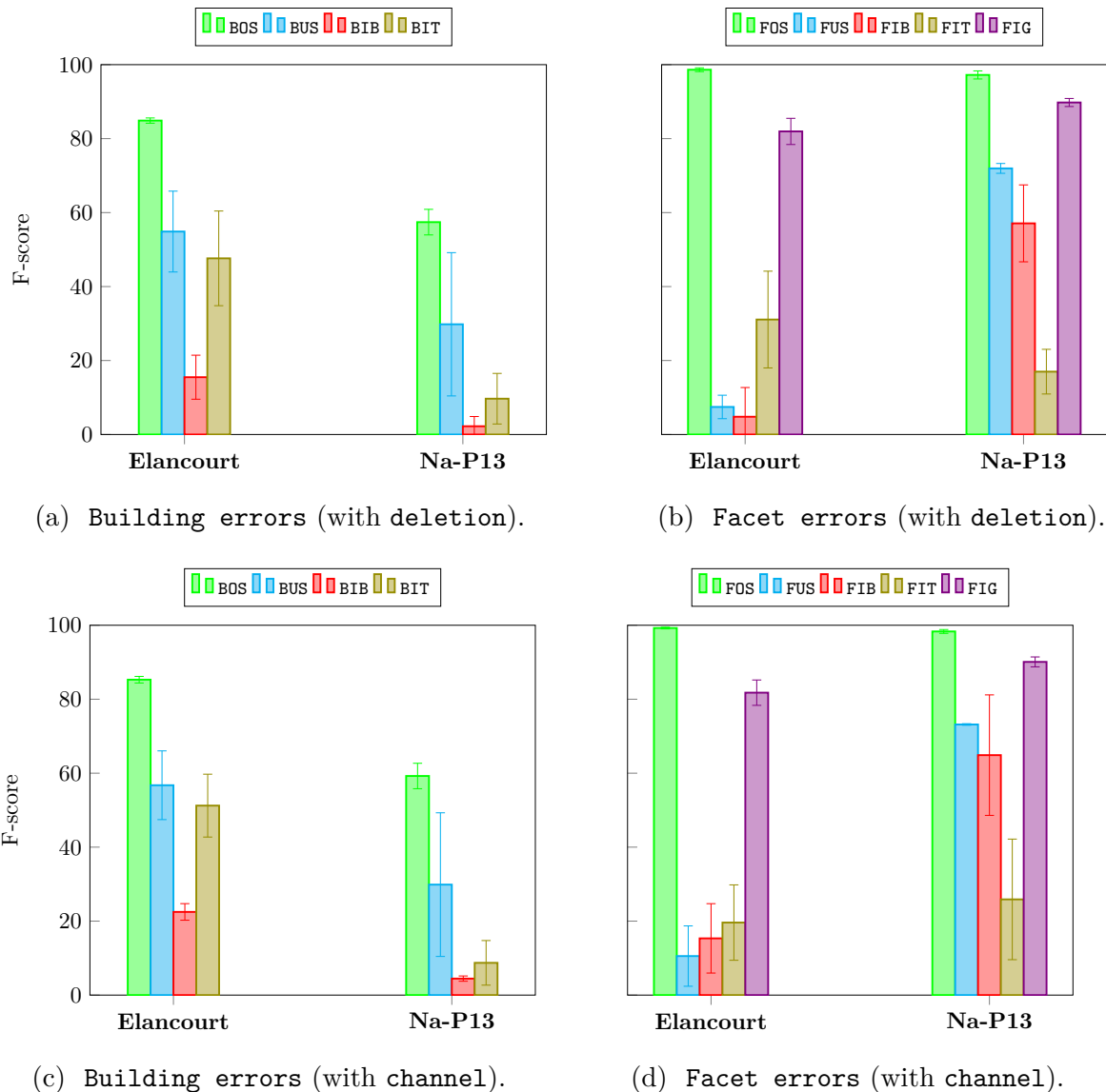
Figure 7.5: Mean F-score and standard deviation obtained with an RF based on ScatNet features. This is a vizualization of scores recorder in Table C.25.
