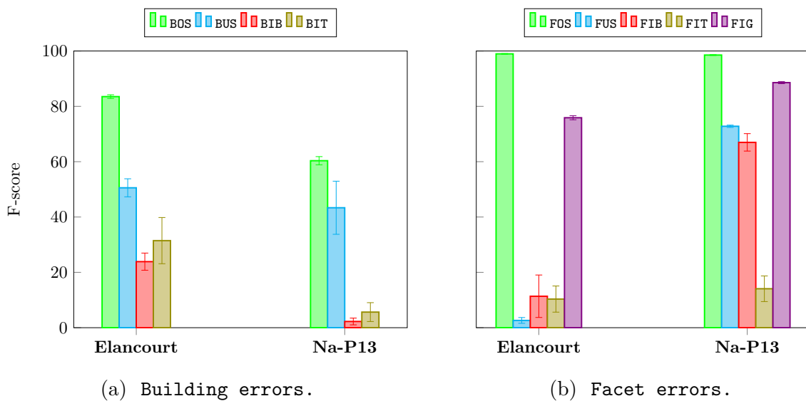
Figure 7.2: Mean F-score and standard deviation obtained with an RF using baseline features.
