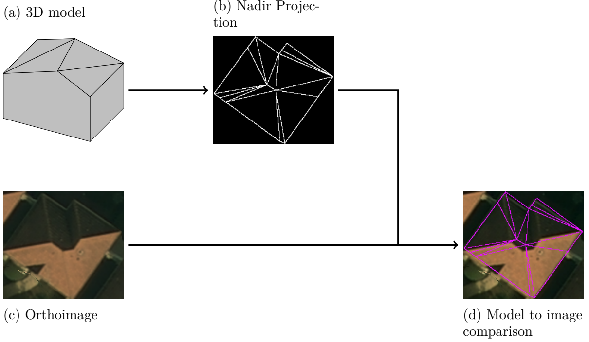
Figure 4.3: Nadir projection of 3D models to image comparison. The input model is projected in the nadir direction. It is then superposed on the orthoimage and compared to it.
