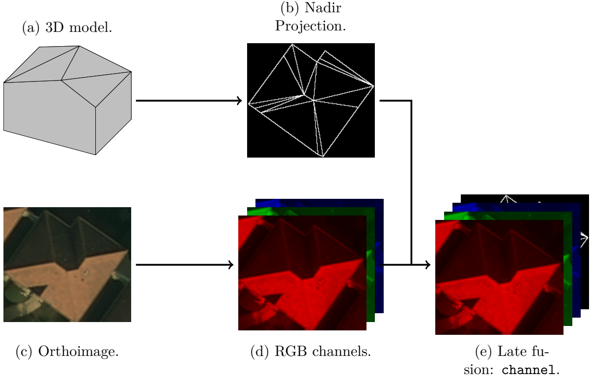
Figure 6.7: Illustration of the late fusion scheme denoted channel . The mask indicating the pixels that intersect the edges of the nadir projection of the model is added as a fourth channel.
