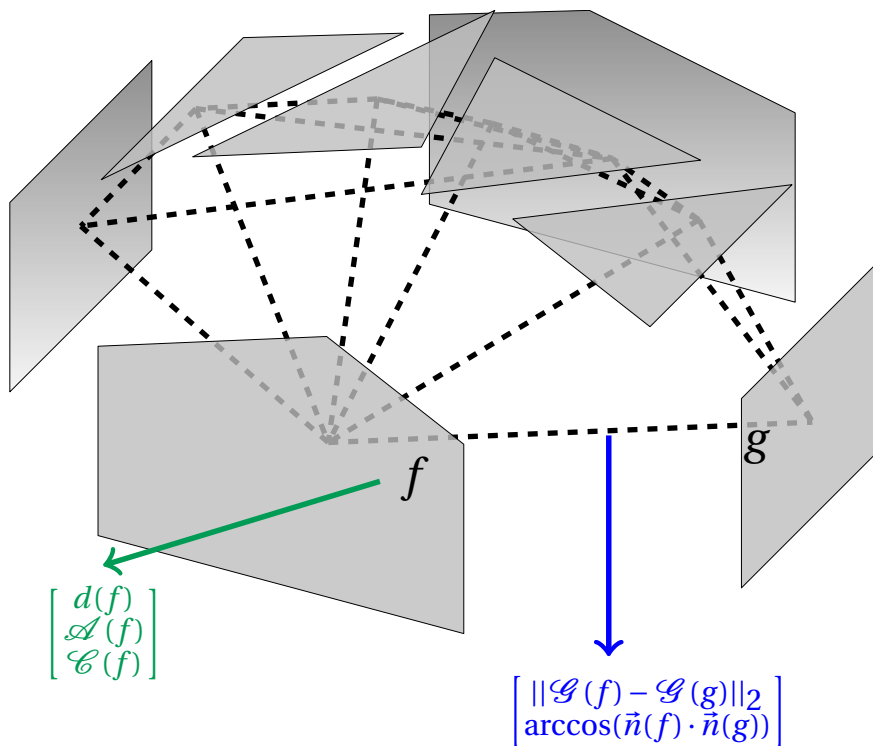
Figure 4.1: Computed geometric attributes represented on the dual graph, for facets f and g . The green vector groups the node (facet) attributes while the blue one shows the edge features.
