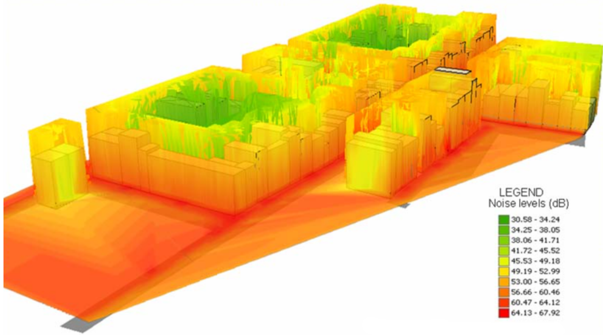
Figure 1.4: Example of noise propagation simulation study using 3D city models. Image taken from (Kurakula et al., 2007).
