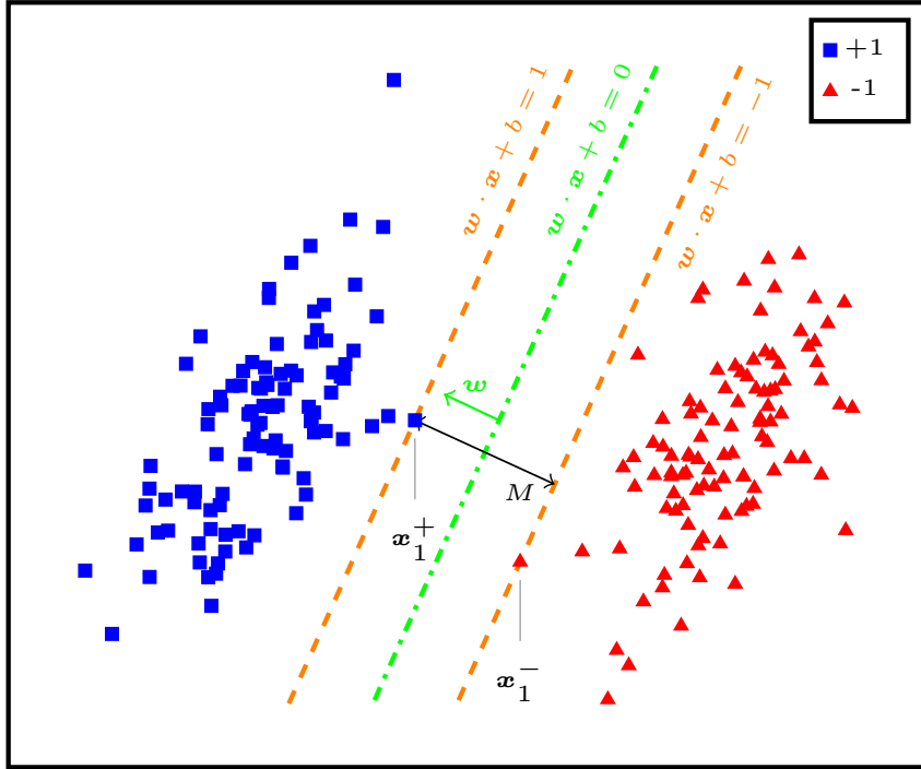
Figure B.1: Illustration of the hard-margin SVM. A hyperplane separator in \mathbb{R}^2 corresponds to a line. In this case, n_{psp} = n_{nsp} = 1 . The support lines are plotted in orange. M is the margin.
