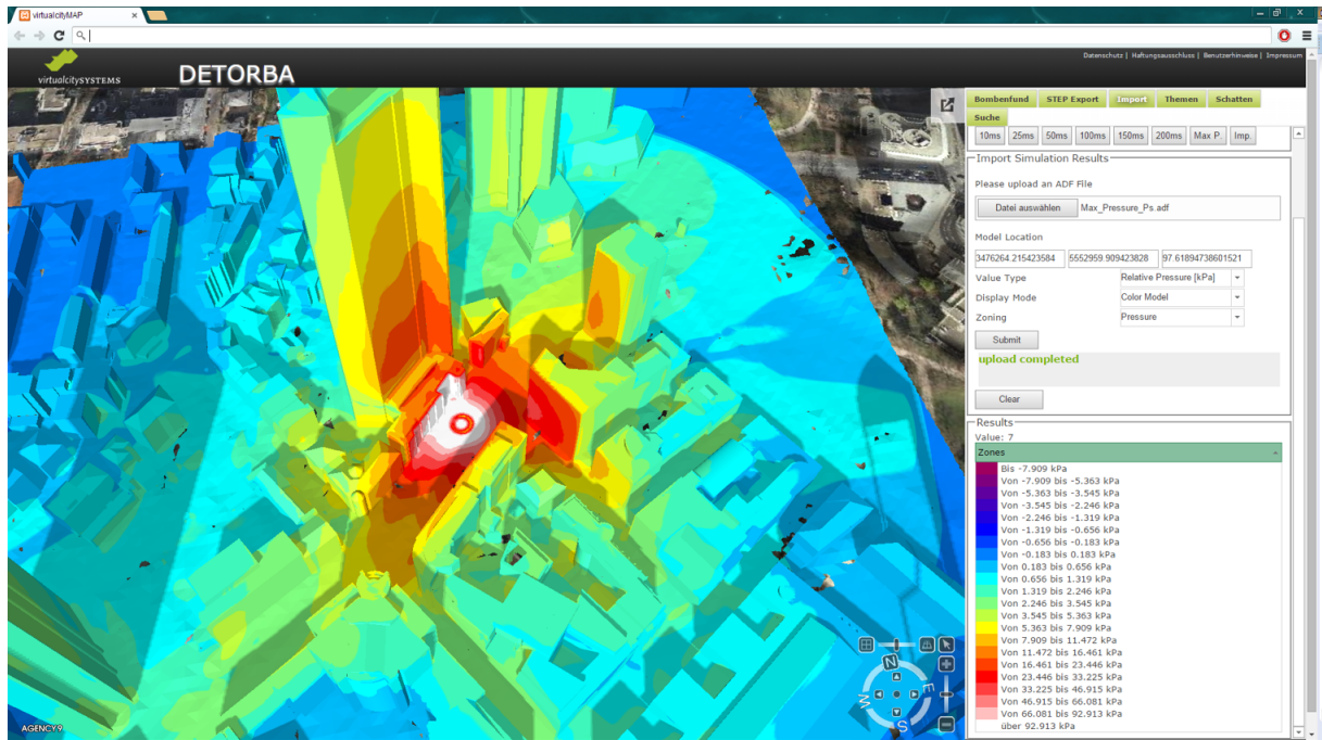
Figure 1.8: Explosion simulation in urban environments using 3D building models. Image taken from (Biljecki et al., 2015b).
