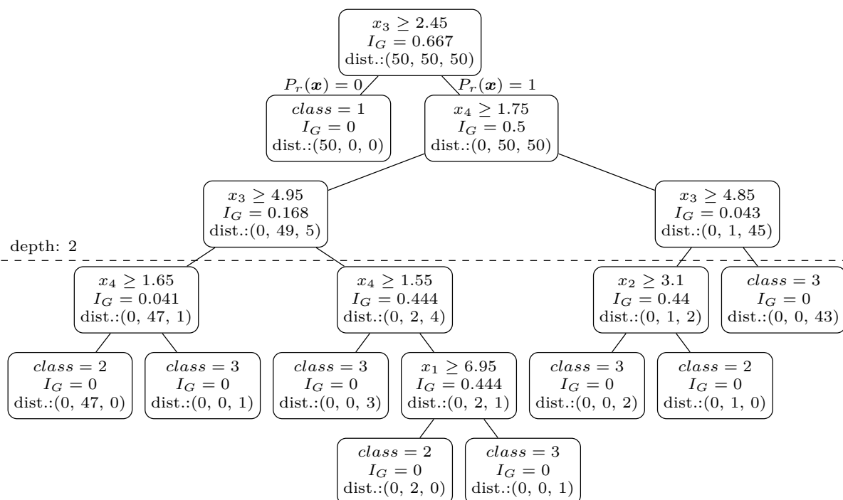
Figure B.4: A visualization of a decision tree classifier learned using I_G Gini index over the iris dataset (Fisher, 1936). Three classes are possible. Each non leaf node states a thresholding condition. For a leaf, its class is presented instead. “dist.”stands for distribution of classes in each node. The whole decision tree overfits to the data with a 100 % overall accuracy ratio. However, when cut at depth 2, the overall accuracy ratio does not drop noticeably (96 %).
