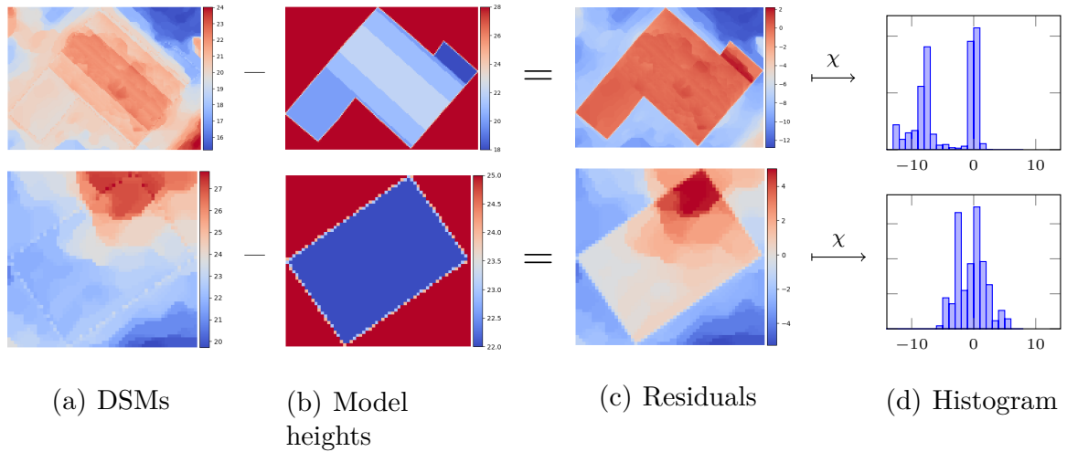
Figure 4.2: Illustration of the baseline for height based features. First, residuals (cf. Figure 4.2c) are computed by subtracting the model height maps (cf. Figure 4.2b) from the DSMs (cf. Figure 4.2a). Histograms are then computed out of these residuals and taken as feature vectors as shown in Figure 4.2d.
