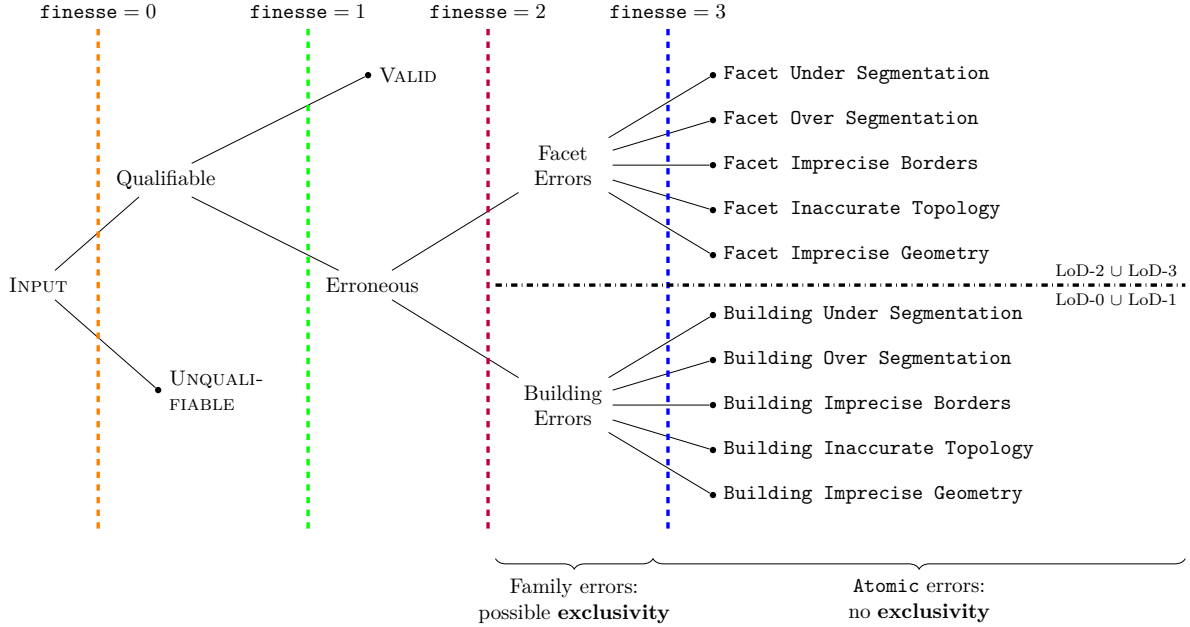
Figure 3.1: The proposed taxonomy structure. In our case of VHR overhead image modeling, only two family errors are depicted. At finesse level 2, hierarchization is possible: an exclusivity parameter can thus act. However, it is not the case at the atomic errors level since they are independent.
