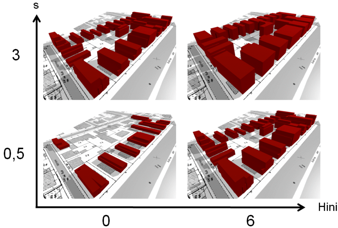
Figure 1.2: Example of 3D urban scene simulated based on known urban norms. Results obtained using the SimPLU3D tool developed by Brasebin et al. (2017). Different parameter values (building surface s and initial height Hini ) result in different urban scenery. Urban planners can assess the projected urban density of future districts for better decision making. Image taken from the SimPLU3D website (Brasebin et al., 2014–2019).
