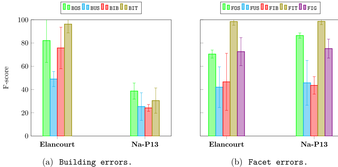
Figure 7.3: Mean F-score and standard deviation obtained with an SVM using baseline features.
