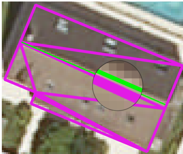
Figure 3.15: Nadir projection of an erroneous building superposed on the corresponding orthoimage showing a FIB error. The real location of the edge is shown in green.
