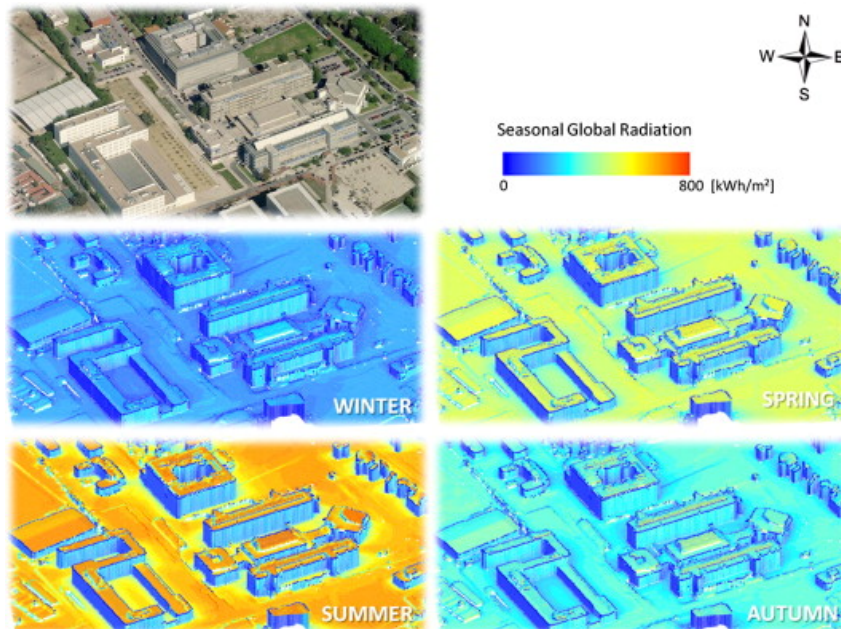
Figure 1.5: Solar potential estimation using 3D building models. The slope, orientation and dimensions of roofs are determinant factors in computing solar irradiation. Image taken from (Redweik et al., 2013).
