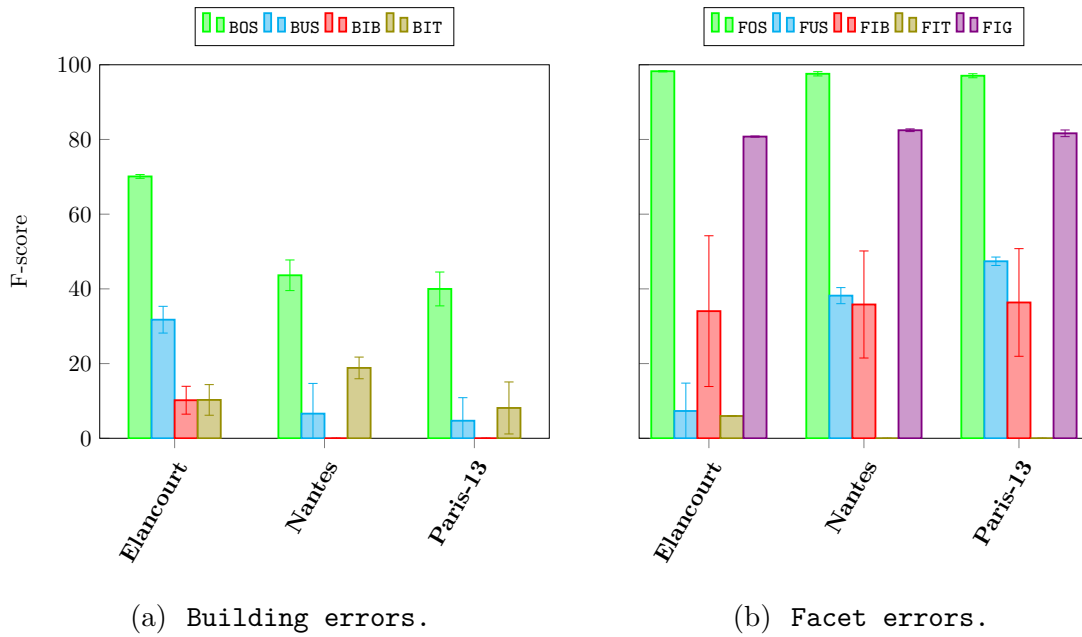
Figure 5.14: Mean F-score and standard deviation for the generalization study per test zone. These are also provided in Table C.9.
