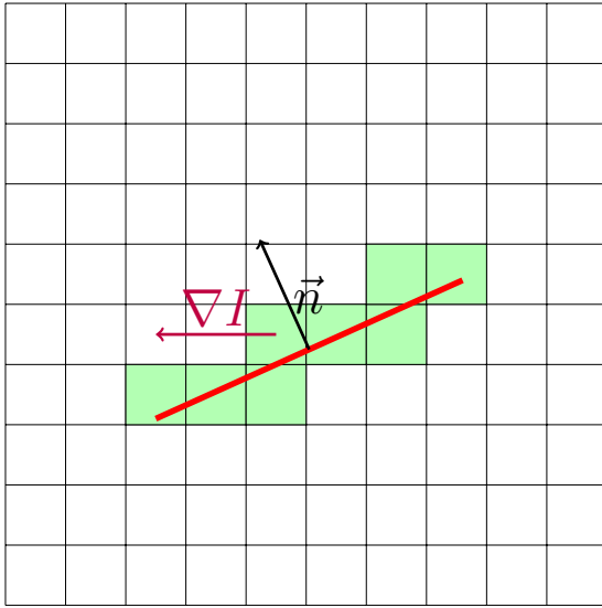
(a) Local gradients (in purple), on intersecting pixels (in green), are compared to the edge (in red) normal (in black).
