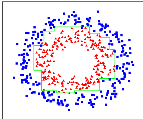
(a) Decision tree separator
