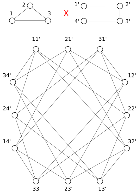
Figure 6.5: Depiction of a direct product (bottom) of two graphs (top). Nodes adjacent in the direct product graph G_\times correspond to adjacent nodes in both graphs. Image taken from (Vishwanathan et al., 2010).
