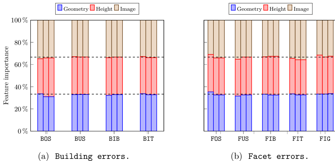
Figure 5.10: Modality importance computed by stacking single feature importances retrieved from the RF classifier. The first ( resp. second and third) column represents Elancourt ( resp. Nantes and Paris-13 ).
