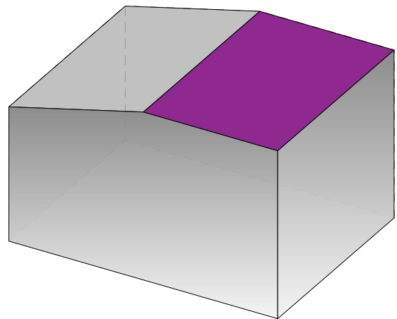
(b) 3D model with a FIG error. The facet in purple has a wrong slope: It is flat instead of being sloped.
