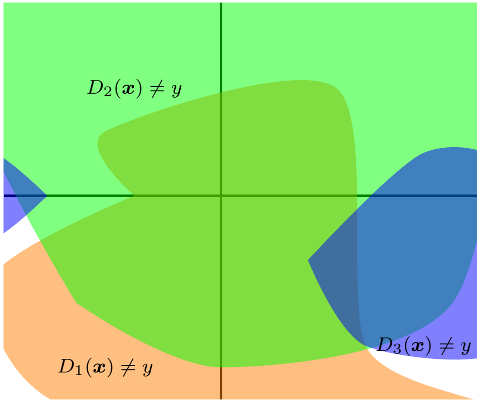
Figure B.6: Illustration of the principle of ensemble methods. For each decision function \forall l = 1, 2, 3 D_l , is represented the set where the each classifier fails F(D_l) \leftarrow \{(\mathbf{x}, y) \in \prod_{i=1}^d \mathcal{X}_i \times \{1, 2, \dots, C\} : D_l(\mathbf{x}) \neq y\} . In the case of unweighed bagging, the aggregated classifier will fail when more than half of the classifiers fail. In this case, the set F(D_{\text{bagging}}) is the union of intersections of two different F(D_l) : F(D_{\text{bagging}}) = \bigcup_{l \neq p} F(D_l) \cap F(D_p) . In this case where classifiers are diverse, the aggregated one fails less frequently than each single one.
