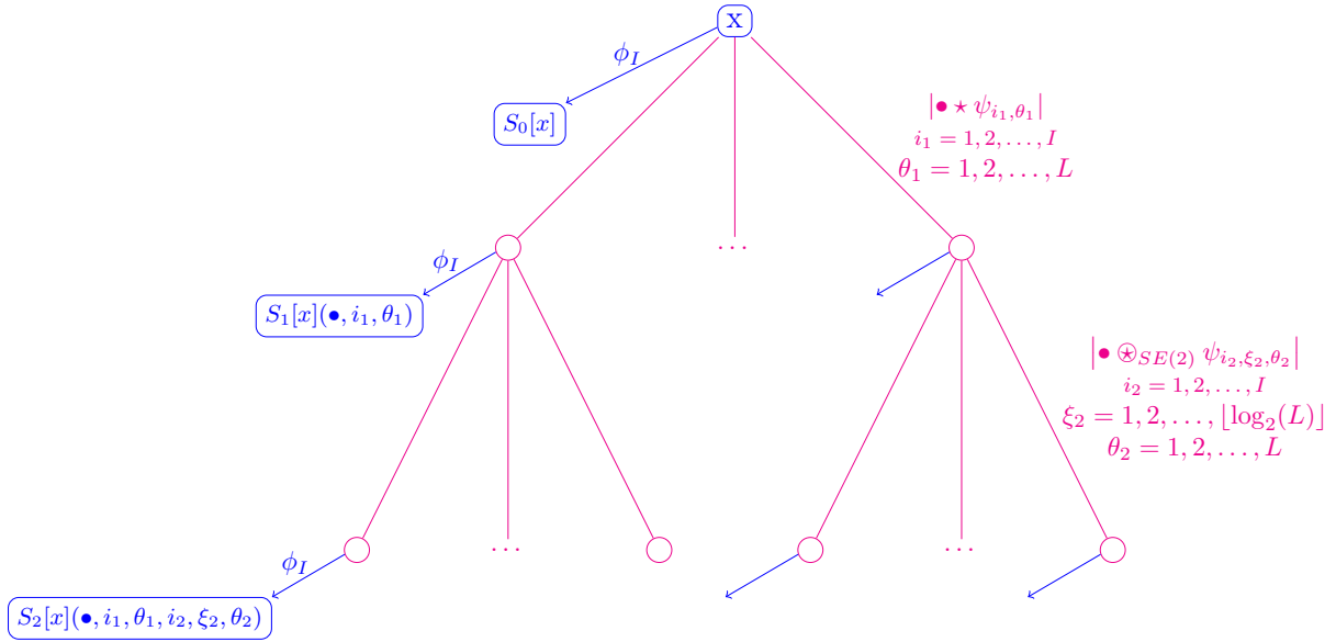
Figure 6.4: Illustration of a ScatNet. At each level are computed convolutions with a filter bank followed by a modulus operator. The scattering coefficients are obtained then by a low-pass filter (in blue). In practice, scattering coefficients are only computed for increasing scale paths up to level 2.
