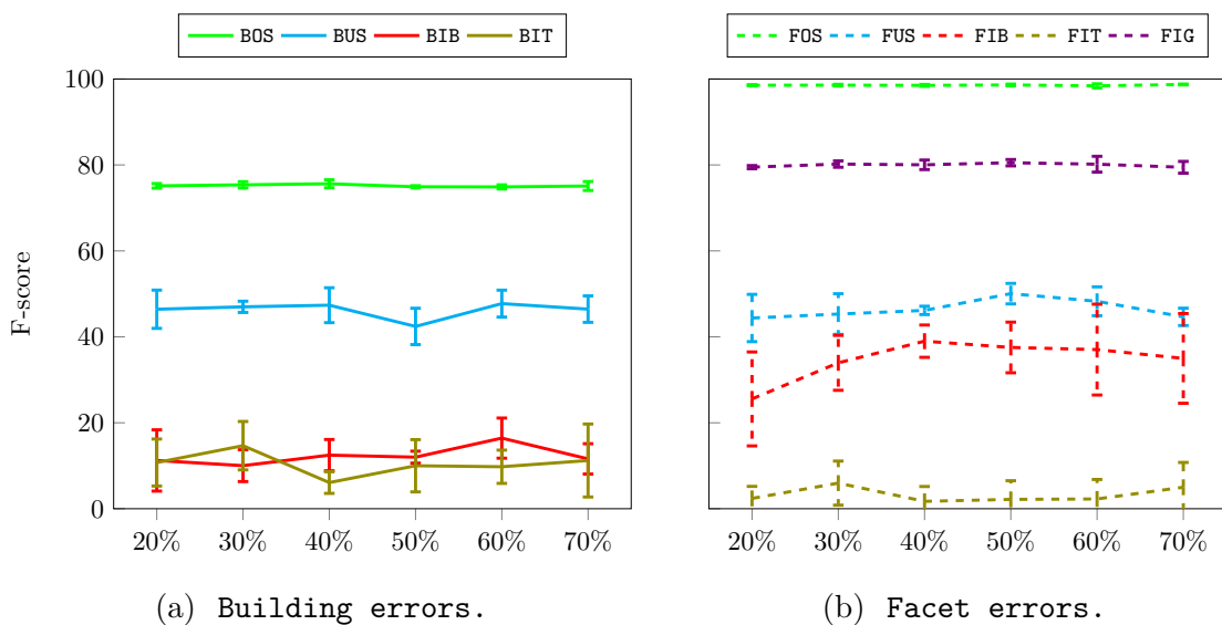
Figure 5.15: Mean F-score and standard deviation for the representativeness experiments depending on the training set size.
