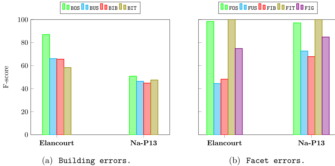
Figure 7.9: F-score obtained with an SVM using graph kernels features.
