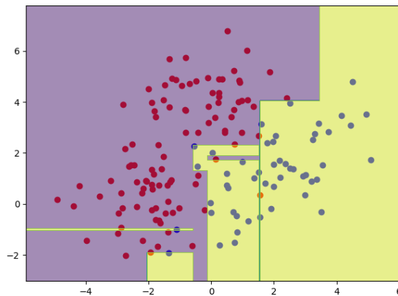
Figure B.5: Visualization of a decision tree separator trained over generated data in a two dimensional feature space. The separator is composed exclusively of horizontal and vertical lines. We can also see how the decision tree overfits by adding narrow splits to accomodate lone points surrounded by others with an opposite class.
