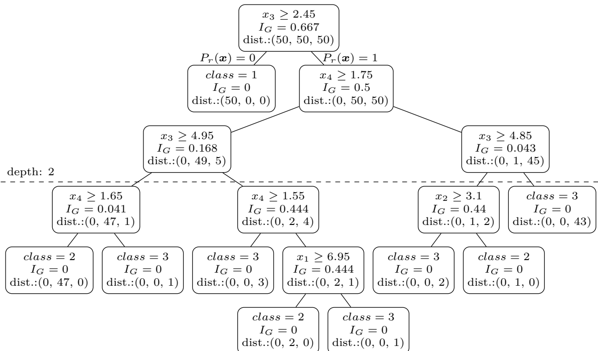
Figure B.4: A visualization of a decision tree classifier learned using I_G Gini index over the iris dataset (Fisher, 1936). Three classes are possible. Each non leaf node states a thresholding condition. For a leaf, its class is presented instead. “dist.”stands for distribution of classes in each node. The whole decision tree overfits to the data with a 100 % overall accuracy ratio. However, when cut at depth 2, the overall accuracy ratio does not drop noticeably (96 %).
