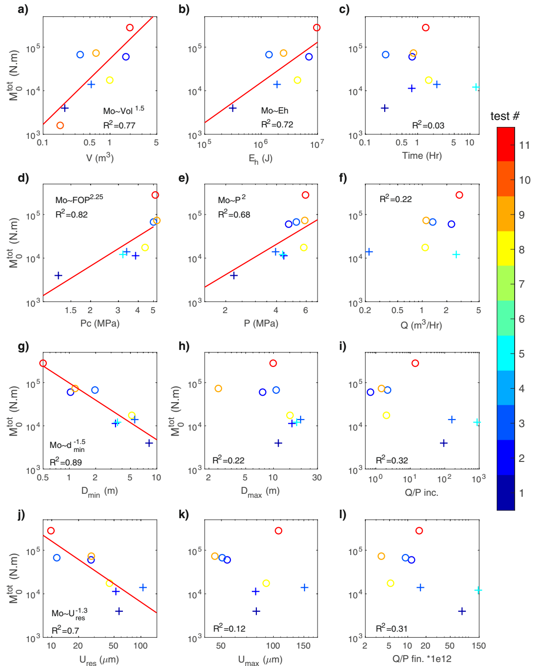
Figure 3. Released seismic moment and monitoring parameters. Total released seismic moment versus (a) Injected volume V . (b) Hydraulic energy E_h . (c) Injection duration time. (d) Critical Pressure P_c . (e) Maximum injection pressure P . (f) Maximum flowrate Q . (g) Minimal hypocentral distance from the injection D_{min} . (h) Maximal hypocentral distance from the injection D_{max} . (i) Ratio of the final over the initial Flowrate-Pressure ratio Q/P_{inc} (i.e. proxy for increase of permeability). (j) Residual displacement at the injection U_{res} . (k) Maximum displacement at the injection U_{max} . (l) Final Flowrate over Pressure ratio, i.e. proxy for final permeability Q/P_{fin} . Colourscale refers to the test number in either Rustrel (“o” symbols) or Tournemire (“+” symbols) experiments. Red lines show the best fitting lines for which R^2 is greater than 0.6.
