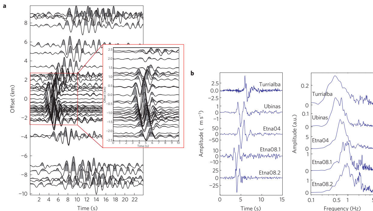
Figure 1 | Illustration of short-duration long-period events and strong propagation path effects. a, Spatial distribution of the long-period wavefield for family 1, 2008 Mount Etna field data. Each seismic trace is a stack of \sim 60 events in the family. Events are located beneath the summit at depths < 800 m. Normalized vertical component traces are plotted as a function of the station's distance from the volcano summit. b, Left panel, shallow pulse-like long-period events (vertical component) detected on near-summit stations at Turrialba Costa Rica (2009); Ubinas, Peru (2009) and two different time periods on Mount Etna (2004 and 2008, family 1 and 2); right panel, amplitude spectra for the data shown in the left panel.
