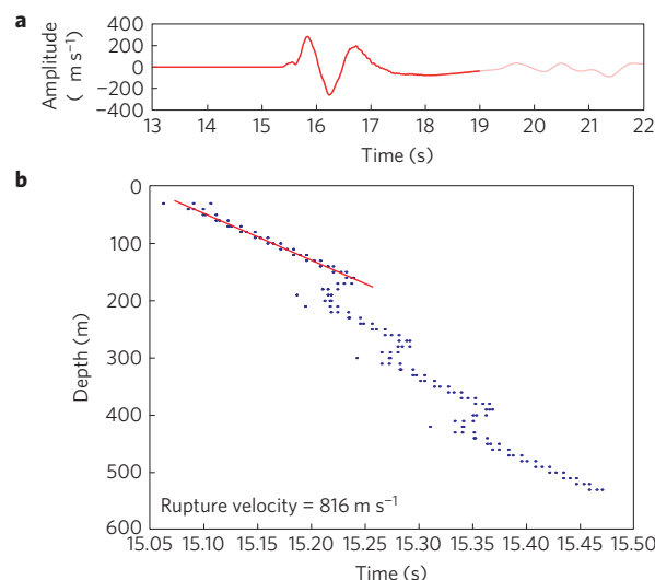
Figure 3 | 2D molecular dynamic simulations of rupture propagation.
