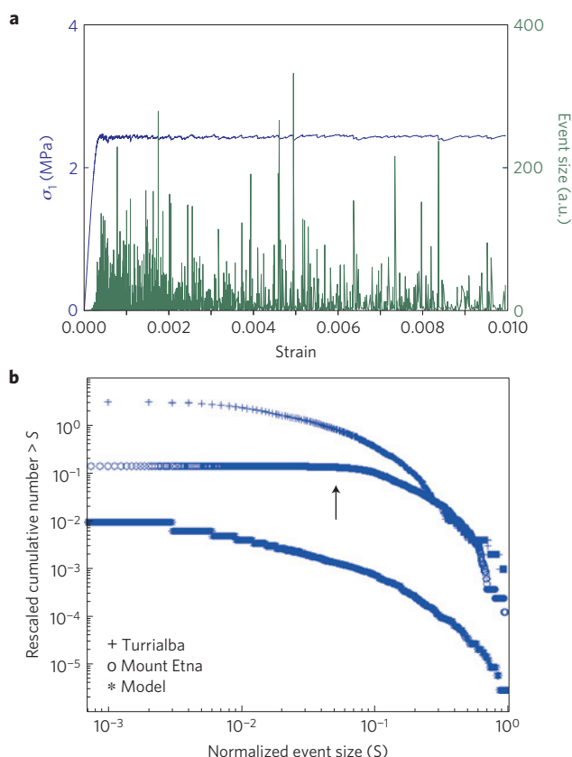
Figure 4 | Simulated seismicity in a weak volcanic upper edifice.
