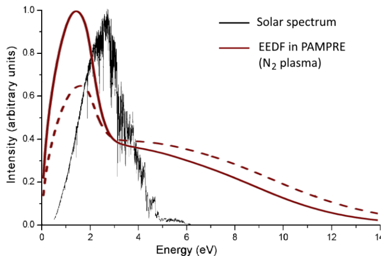
Figure I.4-8: Comparison of the solar spectrum to the modelled Electron Energy Distribution Function (EEDF) of a pure N 2 discharge in PAMPRE at 1 mbar (solid line) and 0.5 mbar (dashed line). From Alves et al. (2012) and Szopa et al. (2006).
