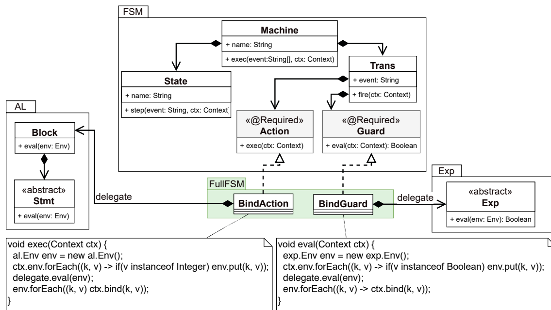
Figure 4.8 – Composing the FSM language module with an action language module and an expression language module. For the sake of conciseness, only excerpts of these modules are depicted here
