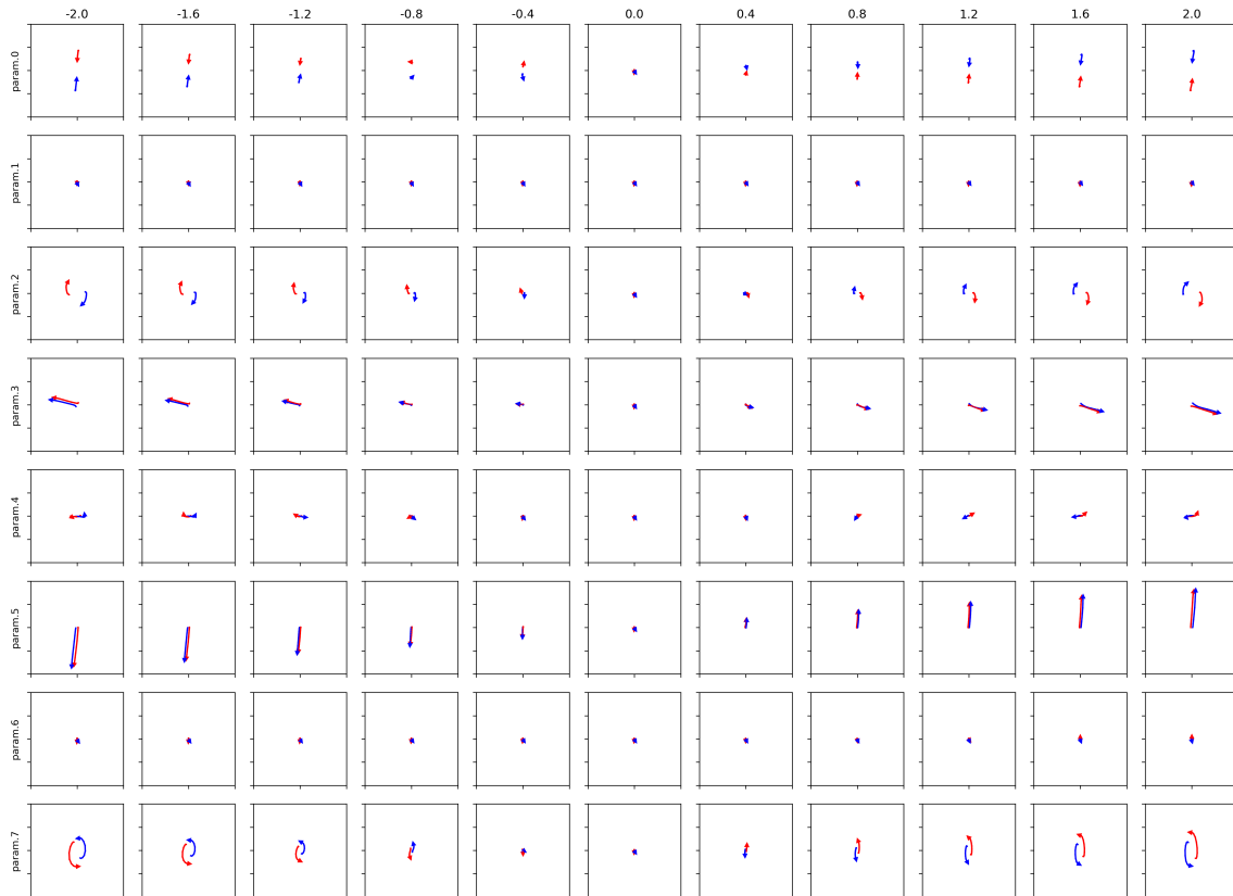
Figure 5.3 – Navigating the latent space learned by the VAE by displaying gestures generated using different codes z . We set the default code to all zeros (middle column). We then change the values of one variable at a time in the range [-2, 2] . So, any code used in this graph will have at most one non-zero value. Lines correspond to different modified latent variables (dim=8). Columns correspond to different values.
