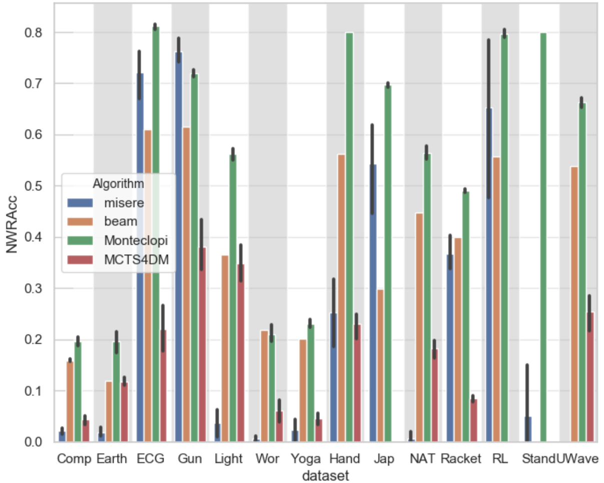
Figure 5.2: Mean NWRAcc of top-5 patterns with different algorithms. Bar errors represent the 95% confidence intervals
