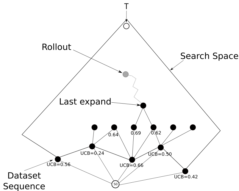
Figure 4.3: MCTSExtent Principle.
