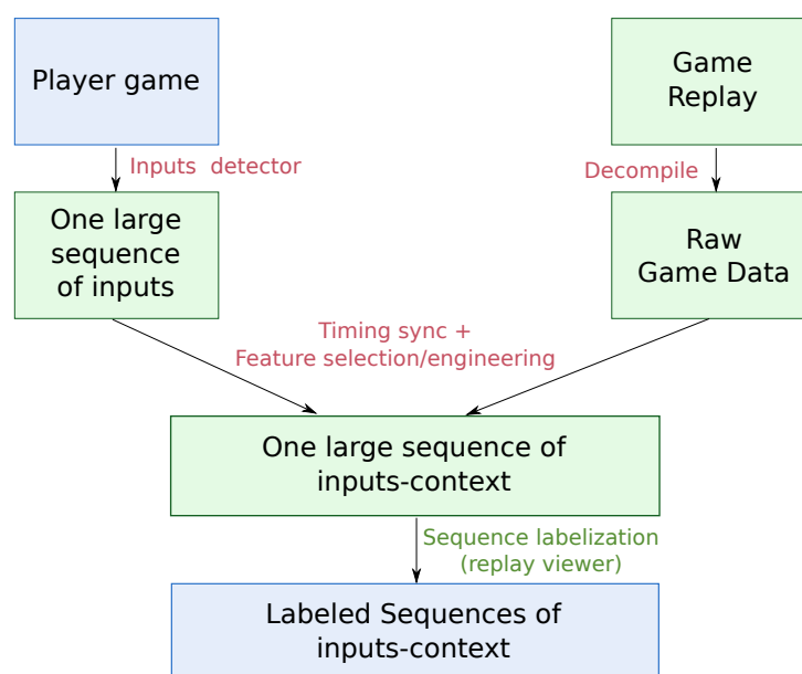
Figure 6.3: Data augmentation
