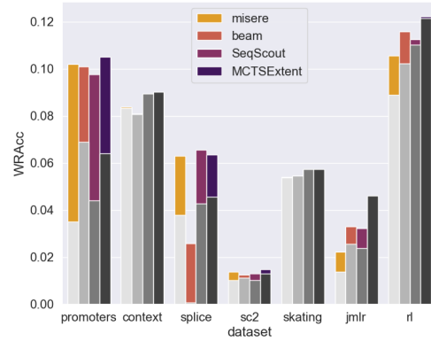
Figure 4.23: Added value of local optima search for 3,000 iterations
