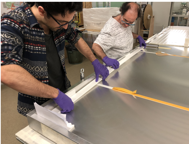
Figure 5.7: Picture of the installation of a scintillator bar inside the aluminum frame. Beforehand, double-sided adhesive stripes are laid out on top of the composite panels two on each side of the module. The protection on the other side of the adhesive stripes are removed as the scintillator bars are installed in the frames.
