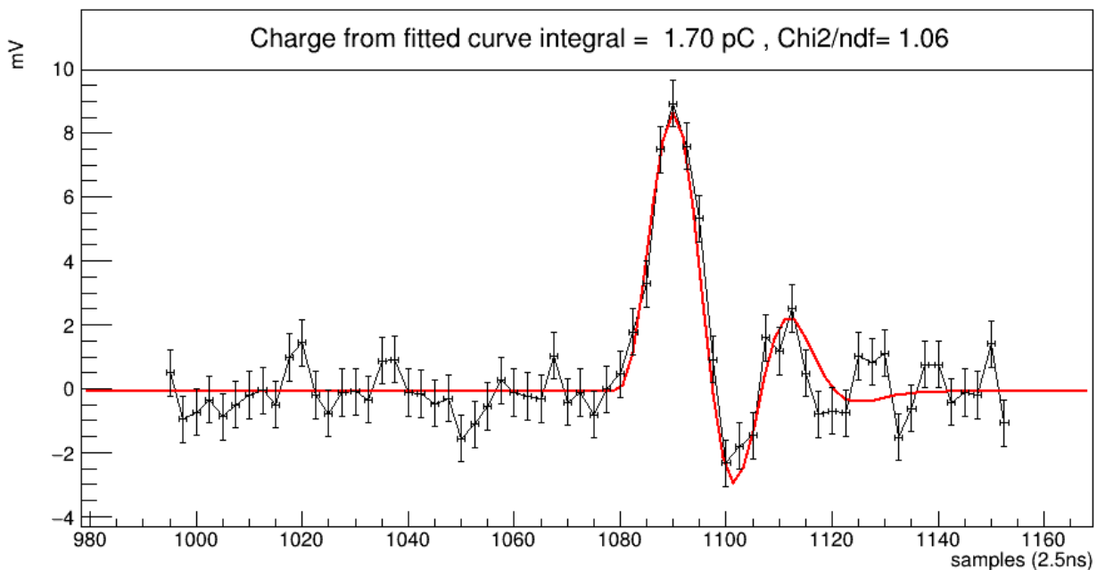
Figure 5.14: Example of a SPE peak fit. This particular pulse was taken from a LED-pulse run.
