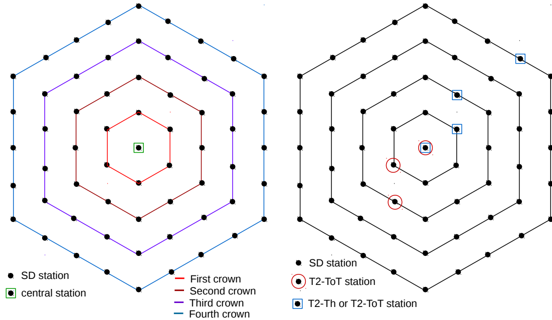
Figure 4.5: Scheme of the SD stations crowns. On the left, the crowns from first to fourth, centered on a central SD station, are represented. On the right, examples of the T3 main trigger geometrical conditions are shown.
