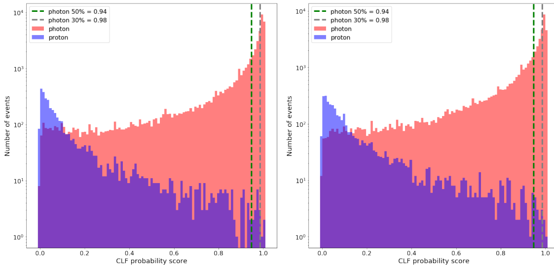
Figure 7.10: Distributions of the classifiers probability scores assigned to the MC-simulations. On the left, the probabilities are those assigned with the ML-observables and on the right, the ones assigned with the analytical observables. Only events not part of the training dataset are included in these histograms. In blue and red are respectively the MC-protons and MC-photons. The green dashed line corresponds to the median of the photon distribution (i.e. 50% signal efficiency), the grey dashed line corresponds to the 30% signal efficiency line.
