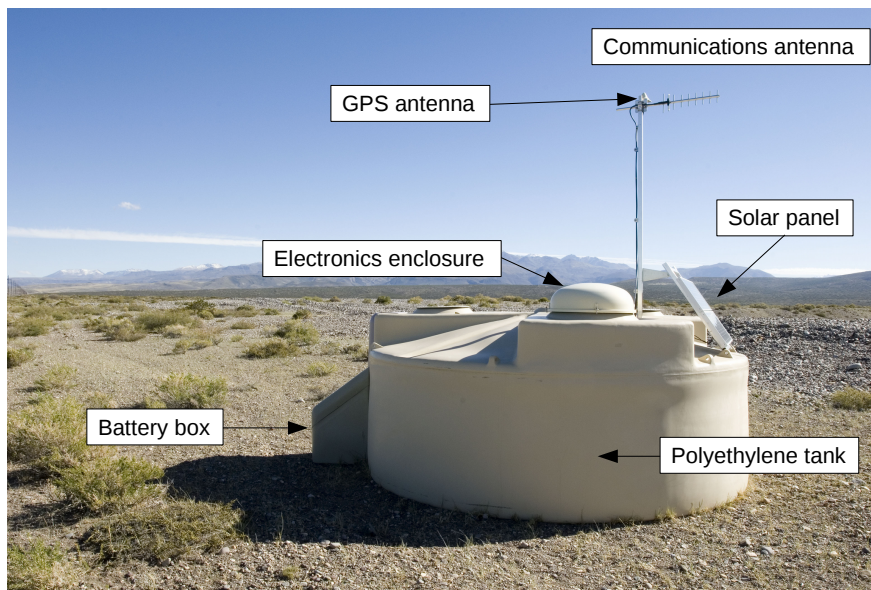
Figure 4.1: Picture of a Water Cherenkov Detector in the pampa, with annotations indicating the main elements.
