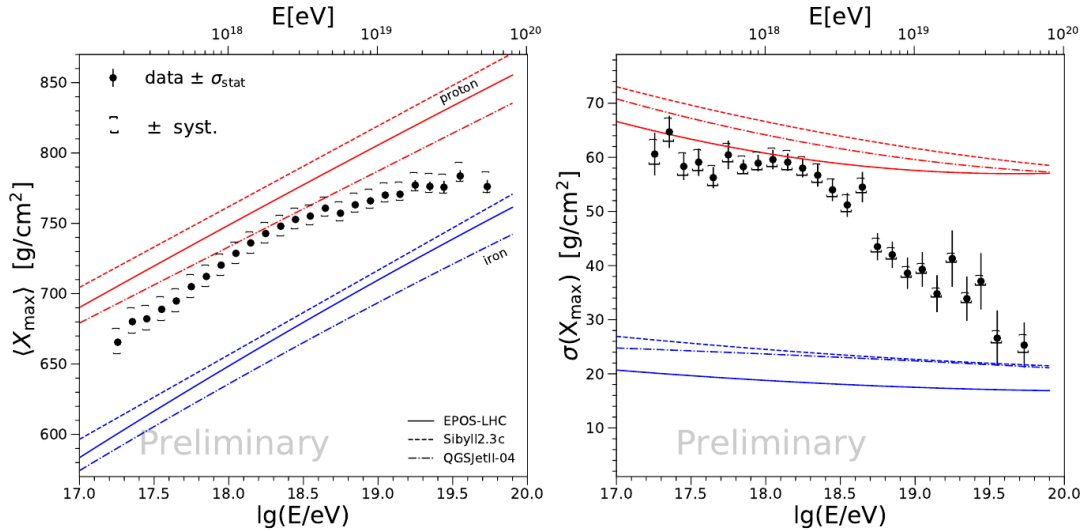
Figure 4.13: Evolution as a function of energy of the primaries mass sensitive observables, \langle X_{max} \rangle (left) and \sigma(X_{max}) (right). The predictions from proton and iron primaries are represented by red and blue lines respectively, for hadronic models EPOS-LHC, QGSJetII-04 and Sybill 2.3c. From [147]
