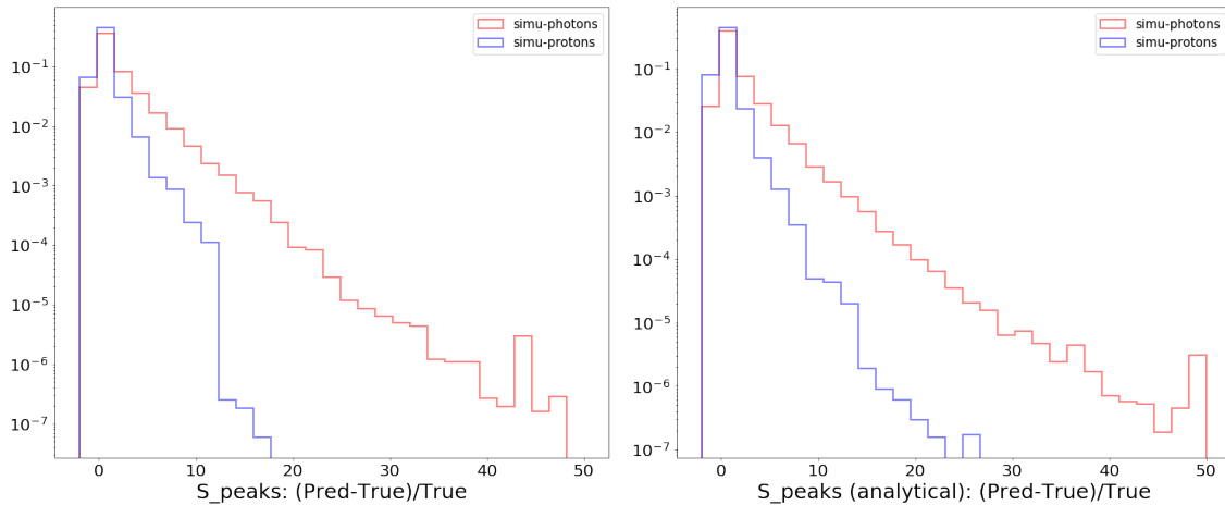
Figure 7.6: Normalized distributions of the relative error of S_{peaks} for protons (blue) and photons (red). Left: ML models. Right: Analytical models.
