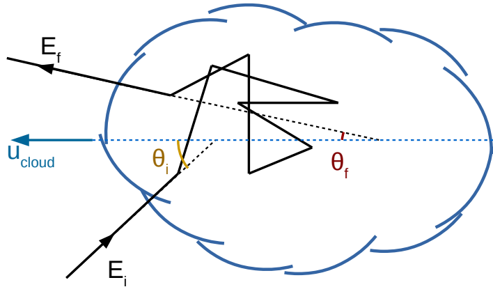
Figure 2.2: Illustration of the second-order Fermi acceleration process.
