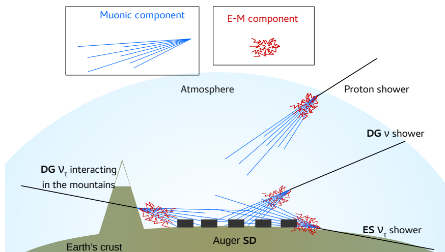
Figure 4.16: Scheme of the neutrino channels
