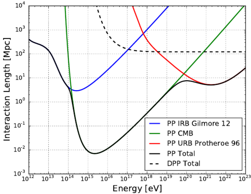
Figure 2.8: Interaction lengths \lambda for photons interacting with E.M. background as a function of photon energy. The relevant processes are represented individually, pair production (solid lines) and double pair production (dashed line) as a photon energy. The pair production process is further separated into the contributions of each type of photon fields, infrared background (IRB - in blue), cosmic microwave background (CMB - in green) and radio background (URB - in red). From [72].
