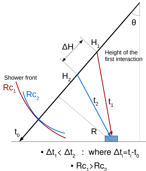
Figure 6.1: Illustration of the geometrical effects involved in the Radius of Curvature calculation.
