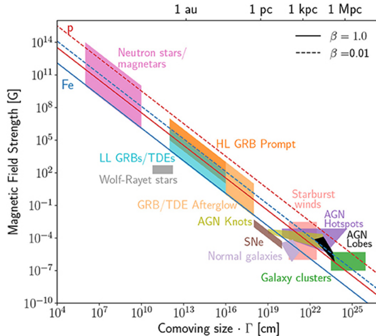
Figure 2.4: Hillas diagram, showing the source classes as a function of their characteristic size R , the product of the comoving size and the Lorentz factor \Gamma of the flow, and their magnetic field strength B . Following relation 2.9, the lines indicate the BR product beyond which the confinement of CRs with energy 10^{20} eV is possible. The continuous (dashed) lines indicate the values for protons, in red and for iron, in blue, for outflows with velocity \beta_{sh} = 1 ( \beta_{sh} = 0.01 ). To be viable, a source must be in the upper-right region of the plot. The figure is taken from [45], more details on the sources can be found in it and in the references therein.
