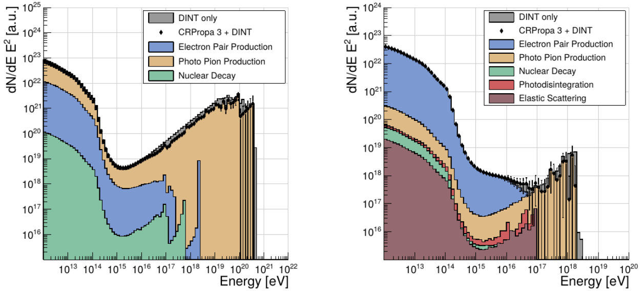
Figure 2.7: Distributions as a function of energy of the secondary photons produced by the interactions of UHECRs during their propagation (from CRPropa simulations). The photon flux is scaled by E^2 , and it corresponds to the secondary photons produced by 10^4 primaries (left: proton, right: iron) drawn from a dN/dE \propto E^{-1} distribution, between 10^{18} eV and 10^{21} eV. The primaries are produced from uniformly distributed sources located between 3 and 1000 Mpc from the observer. The black dots show the total photon flux while the individual-process contributions are color-coded. From [72].
