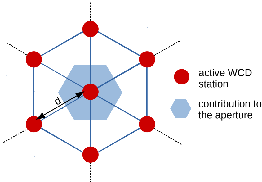
Figure 4.11: Scheme of an hexagon cell. The aperture of each active hexagon cell of the SD is represented as the light blue area.
