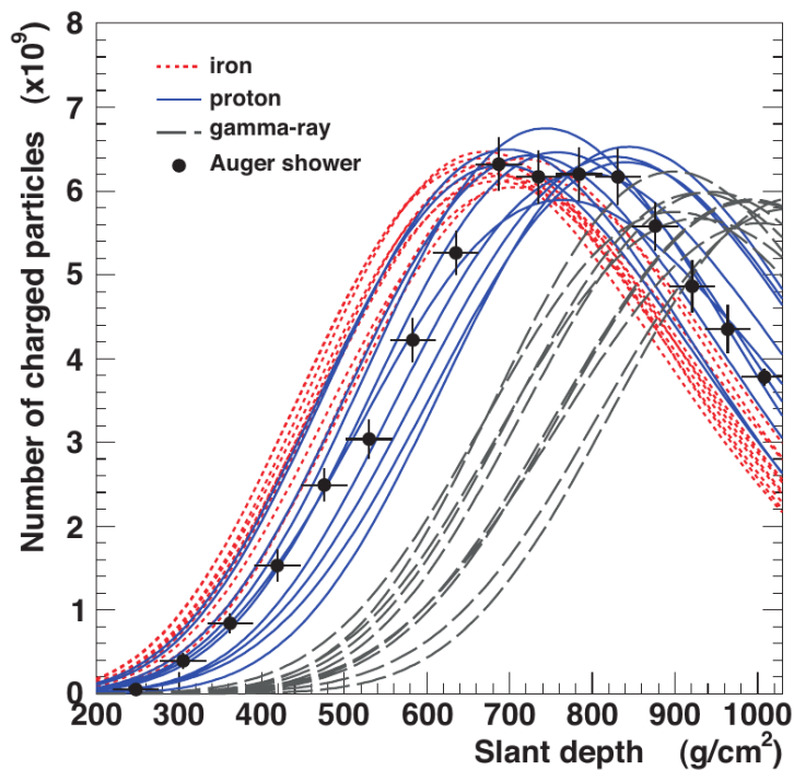
Figure 3.5: Longitudinal profiles of 10 proton-, iron- and photon-induced showers of energy E_0 = 10^{19} eV simulated with Sibyll. The data points in black show the longitudinal development of a shower observed with the Pierre Auger Observatory at approximately the same energy. From [99].
