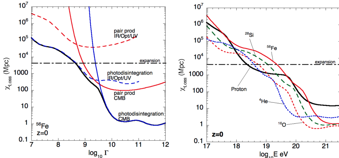
Figure 2.6: Left: Evolution of the energy loss length for an UHE iron at redshift z = 0 as a function of its Lorentz factor \Gamma . The photodisintegration (in blue) and the pair production mechanism (in red) are represented for interactions with the IR/opt/UV background photons (dashed curve) and for CMB photons (continuous curve). Right: Evolution of the energy loss length for UHECRs of various nuclear masses at redshift z = 0 as a function of their energy. The curves are drawn for z=1,4,16,28,56 . From [73].
