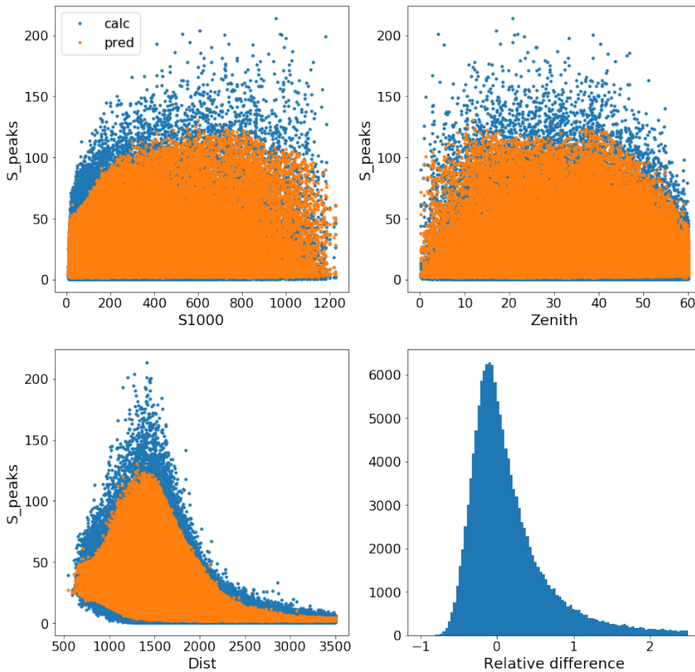
Figure 7.4: Distributions of calculated values (in blue) and predicted values using the KNR algorithm (in orange) of S_{peaks} for MC-protons. From top to bottom and left to right, the figures represents: the distributions of the S_{peaks} values as a function of (1) S_{1000} , (2) \theta and (3) r . The bottom-right figure (4) represents the relative difference between the S_{peaks} values calculated and the ones predicted by the regressor.
