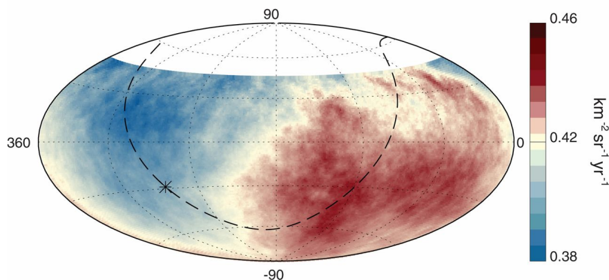
Figure 4.15: Sky map in equatorial coordinates of the UHECRs flux above 8 \times 10^{18} eV in a Hammer projection, smoothed with a 45^\circ top-hat function. The colormap indicates the intensity of the flux. The dashed line indicate the galactic plane and the asterisk indicates the galactic center. From [74].
