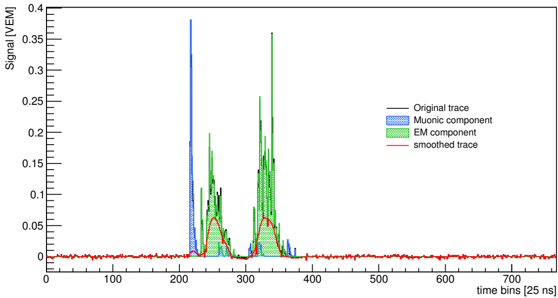
Figure 6.17: The smoothing process applied on a simulated VEM trace, with the muonic and EM components highlighted in different colors.
