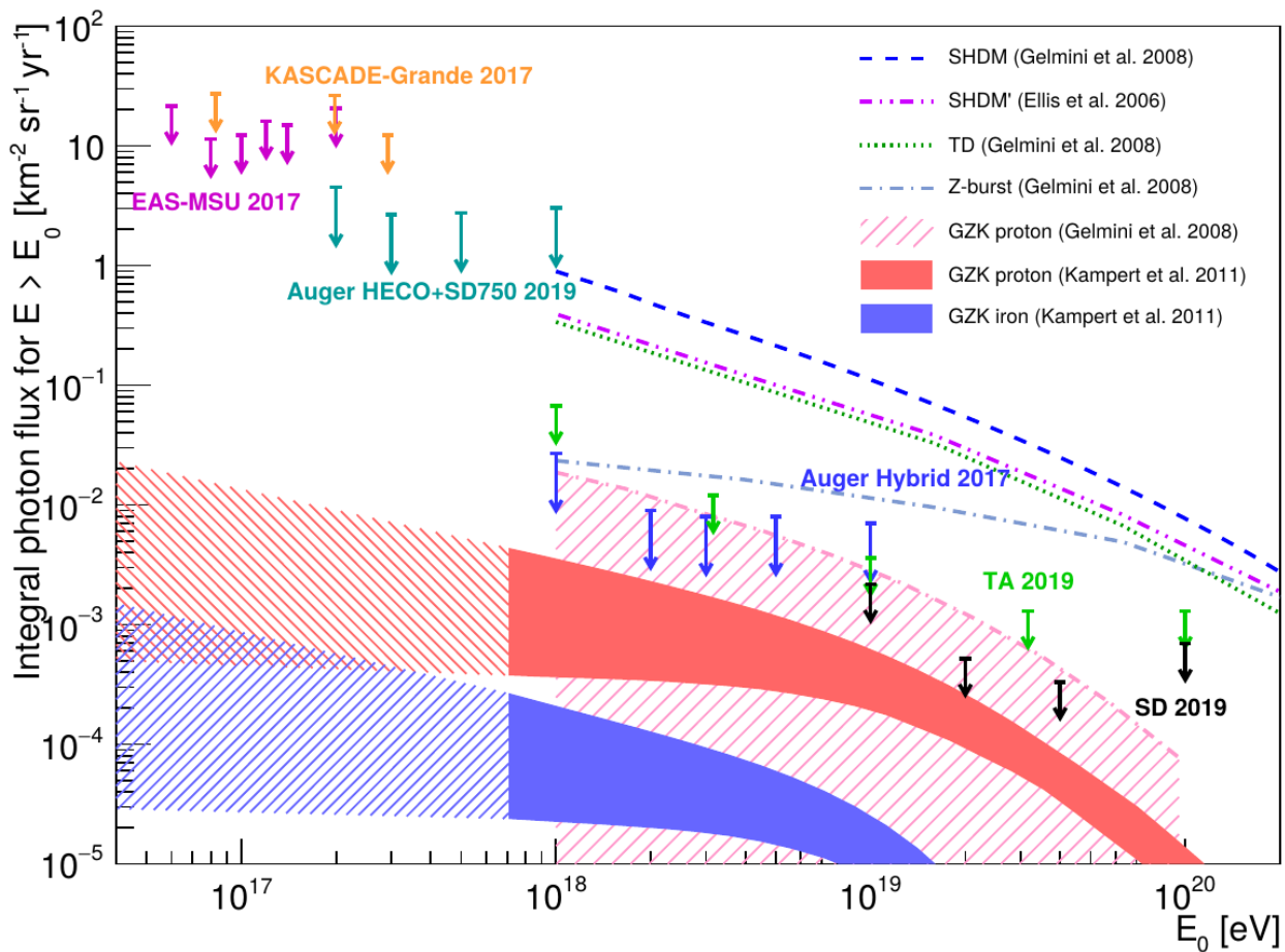
Figure 6.13: The latest results of the Auger searches (hybrid, hybrid with 750m array, SD) are shown, as well as the limits obtained by EAS-MSU [198], KASCADE-Grande [199] and TA [192]). The predicted flux from top-down scenarios and GZK process are also shown (see [195] and references therein) Taken from [195]
