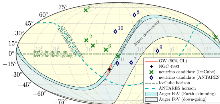
Figure 4.18: Skymap in equatorial coordinates during the GW170817 event. The expected localization of the BNS event and its host galaxy are shown, as well as the neutrino candidates within \pm 500 s of the merger and the horizons of the ANTARES and IceCube experiments. The Pierre Auger Observatory fields of view in the ES and DG channels are also depicted. [157] and references therein.
