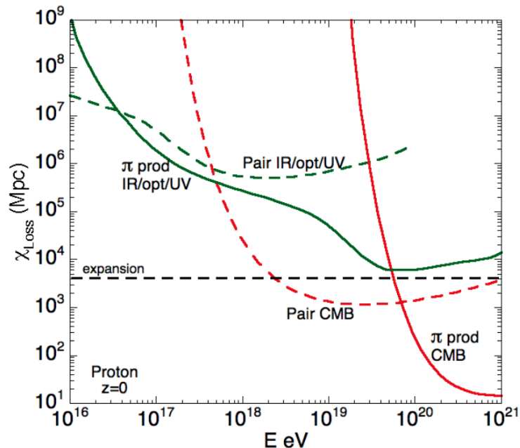
Figure 2.5: Evolution of the energy loss length for an UHE proton at redshift z = 0 as a function of its energy. Three processes are represented, the adiabatic expansion of the universe (black dashed horizontal line), the pair production mechanism (dashed curves) and the pion photo-production mechanism (continuous curves). The pair production and pion photo-production mechanism are drawn for interactions of the proton with CMB photons (in red) and for other sources of background photons (IR/opt/UV) (in green). From [73].
