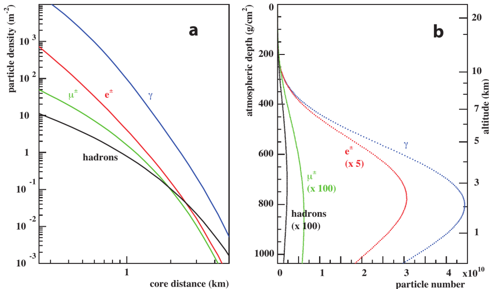
Figure 3.3: Average lateral (a) and longitudinal (b) profiles of vertical showers induced by a proton of energy E_0 = 10^{19} eV simulated with CORSIKA [98]. The number of particles at ground (a) is calculated at depth X = 870 \text{ g}\cdot\text{cm}^{-2} which corresponds to the average ground-level for the Pierre Auger Observatory. From [99].
