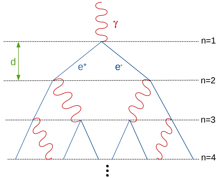
Figure 3.1: Scheme of the first four splits in an EM cascade. Redrawn following [95].
