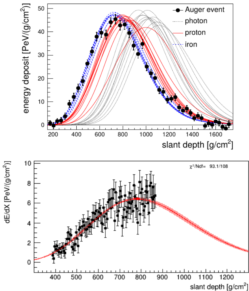
Figure 7.13: Top: Examples of longitudinal development profiles for MC-simulations of iron, proton and photon primaries. For hadronic primaries the maximum of dE/dX is expected below \sim 820 \text{ g.cm}^{-2} , while for photons it is expected around or above 900 \text{ g.cm}^{-2} . Bottom: Longitudinal development profile of event 7426428 measured with a FD telescope located Los Morados. This distribution of the dE/dX values as a function of the slant depth matches the hadronic-induced showers expectations from MC-simulations, with a maximum slightly below \sim 800 \text{ g.cm}^{-2} .
