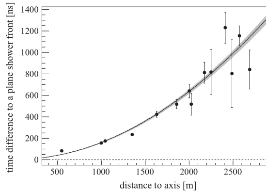
Figure 4.8: Geometrical reconstruction of a shower. As the stations get further away from the core, the time-difference between the expected start time from a planar shower front and the measured one gets larger. From [133].
