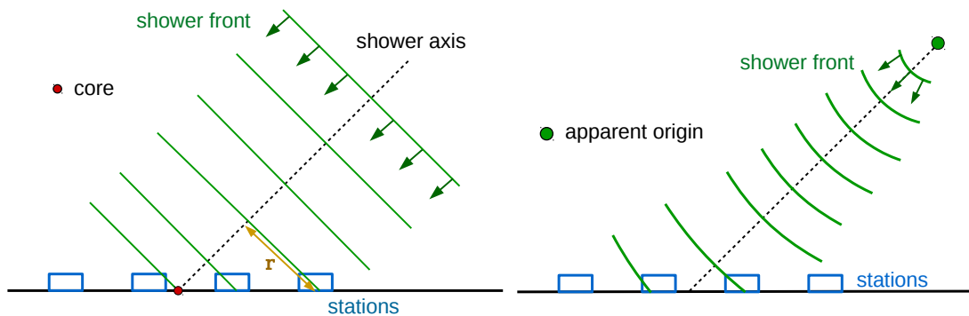
Figure 4.7: Scheme of the shower front estimation. Left: the first seed reconstruction performs a planar shower front fit on the individual stations. The distance of a station to the shower axis ( r ) is represented. Right: representation of a spheric shower front.
