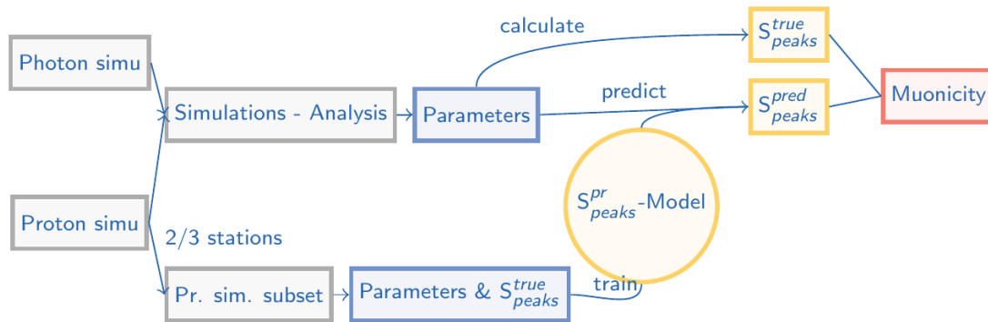
Figure 7.7: Scheme of the observable reconstruction procedure, example of the Muonicity observable.
