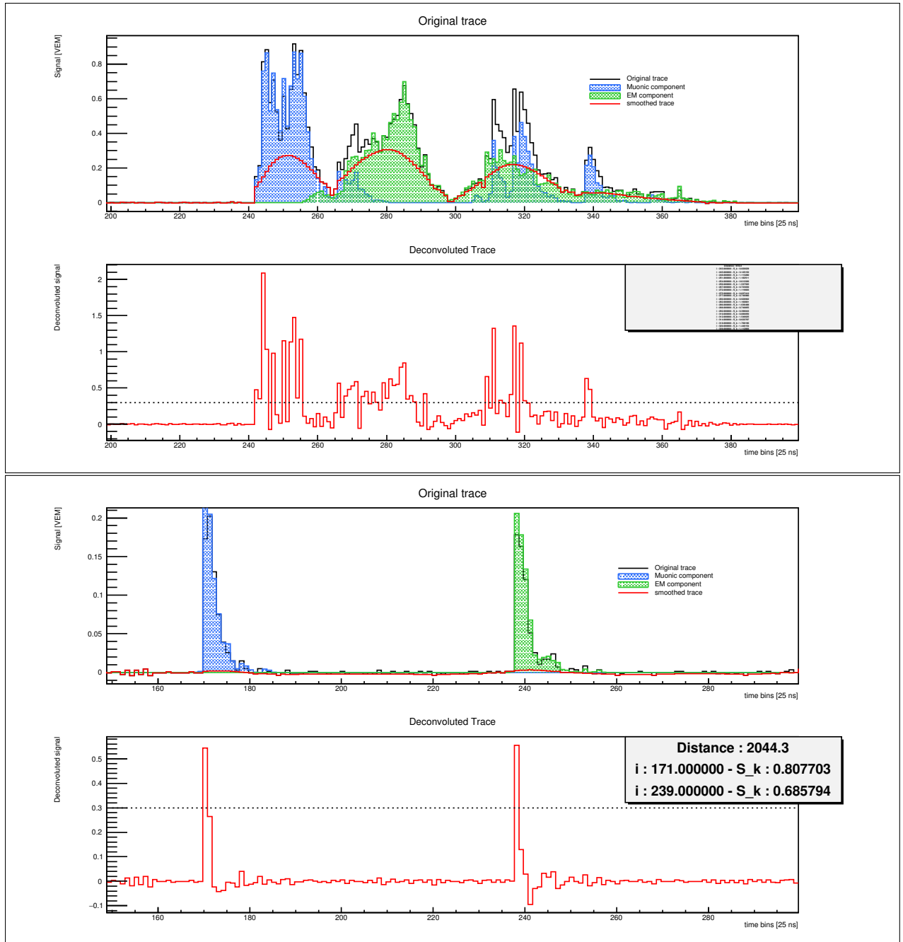
Figure 7.1: Examples of “bad” traces for the Muonicity and Smoothing methods. In both frames, the original VEM traces are shown above the deconvoluted traces, calculated using the Muonicity method, while the smoothed traces (calculated according to the Smoothing method) are drawn over the VEM traces, in red. The dotted line in the deconvoluted traces represent the S_{min} value above which a bin is considered a peak by the Muonicity method. The frame on the top-right of the deconvoluted traces indicates the bin-number and the S_k value of the deconvoluted peaks selected by the Muonicity method. Top: the VEM trace shows a crowded trace, where the muon signals are bundled together and the Muonicity method is unable to properly separate the muon peaks. Bottom: in this VEM trace, around bin 240, a photon produces a “muon-like” peak, and both the Muonicity and the Smoothing methods treat it as a muon signal. One can see that for the top figure, the method does not work as it finds too many peaks compared to the true number of muon peaks.
