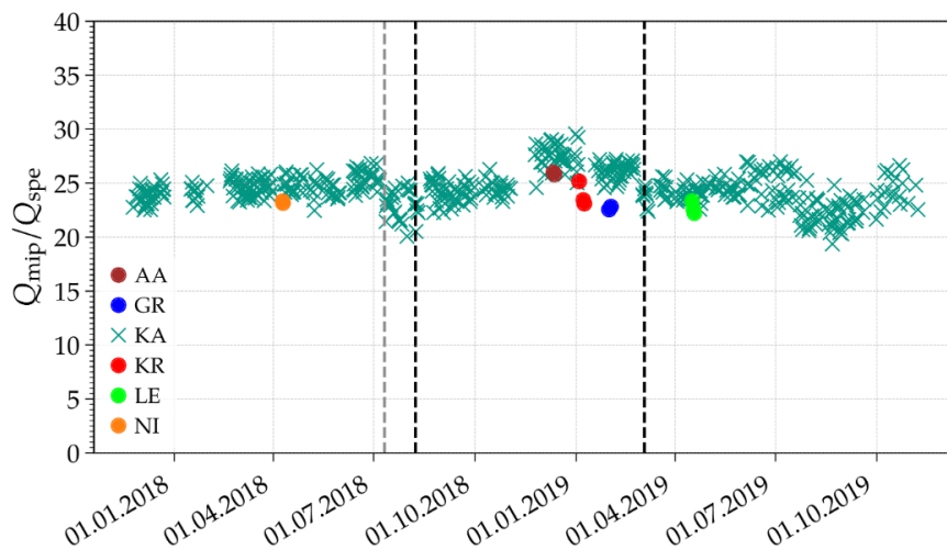
Figure 5.19: SPE per MIP values obtained with the KIT test setup, for SSDs assembled in the several assembly sites.
