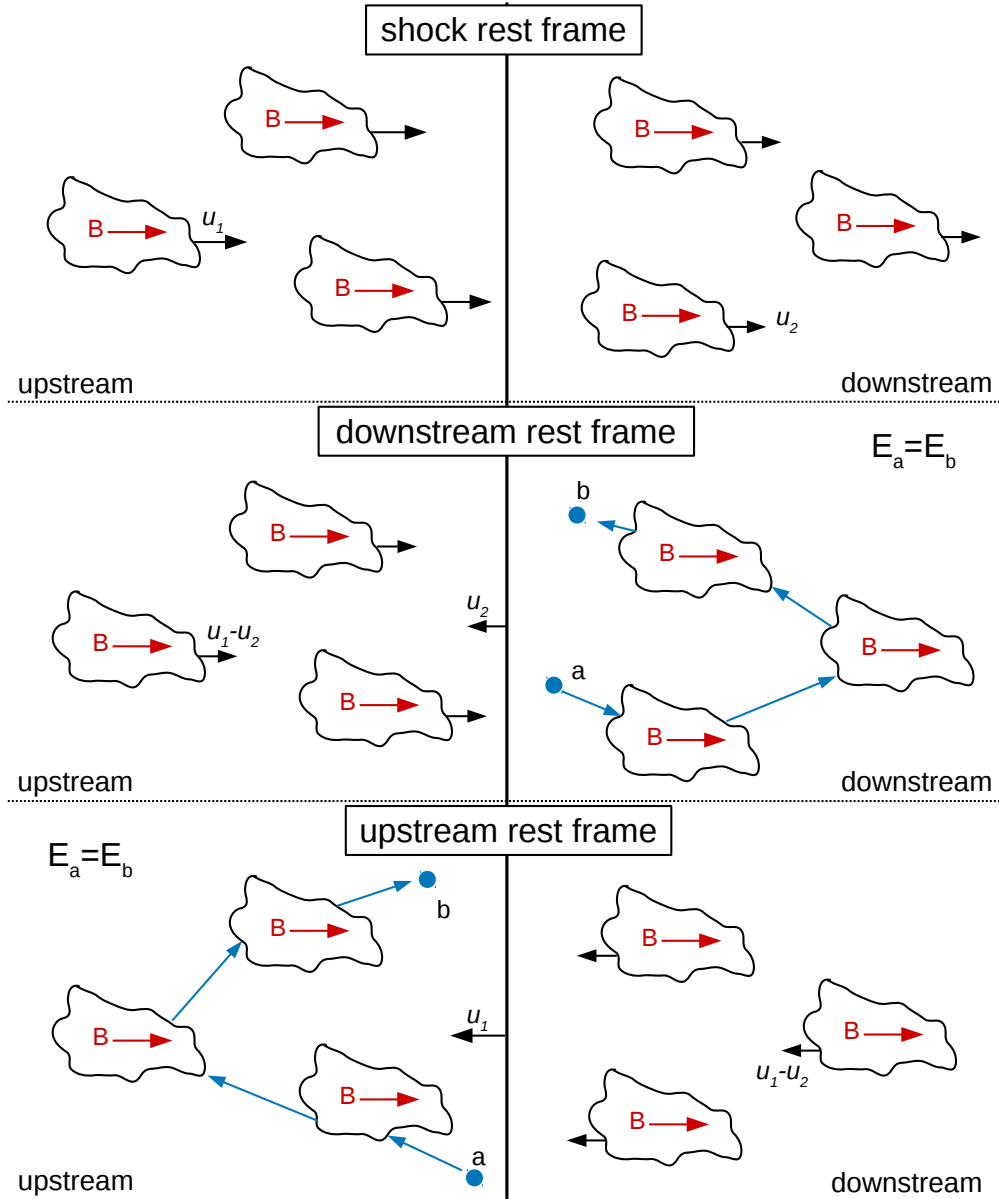
Figure 2.3: Illustration of the first-order Fermi acceleration mechanism.
