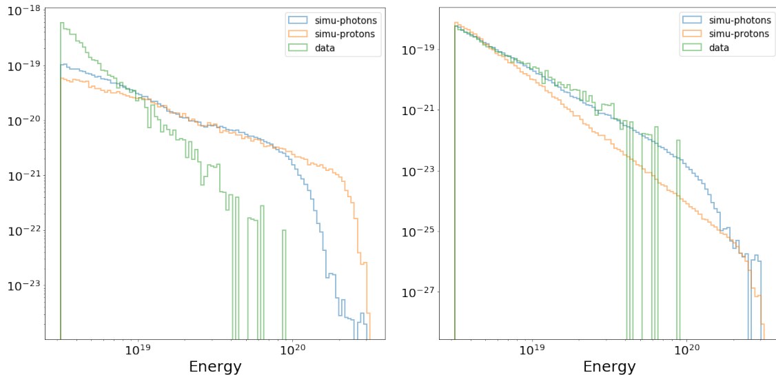
Figure 7.8: Normalized distributions of the reconstructed energies for MC-photons, MC-protons and burn sample events unscaled (left) and with the MC-photons and MC-protons rescaled on a E^{-\gamma} spectrum with \gamma = 3 and \gamma = 2 respectively. To compare the three distributions they had to be normalized to 1, the vertical axis is thus the probability densities estimate.
