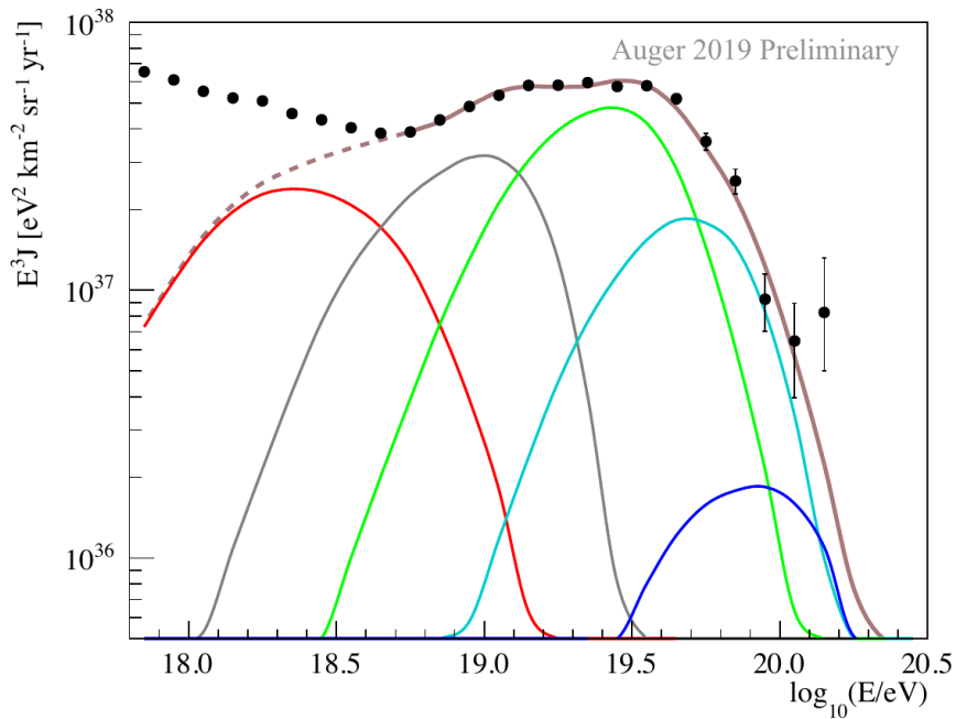
Figure 4.14: The Auger energy spectrum (multiplied by E^3 ) at the top of Earth's atmosphere, fitted with a simulated energy spectrum following the model used in [148]. The simulated energy spectra (colored line) is obtained by performing a combined fit of a simple astrophysical model to the energy spectrum obtained from SD data (black dot) and the values of X_{max} (which are composition-sensitive). The all-particle simulated spectrum (brown line) is the sum of the mass-restricted energy spectra: in red A=1 , in grey 2 \leq A \leq 4 , in green 5 \leq A \leq 22 , in cyan 23 \leq A \leq 38 and in blue A \geq 39 . From [149].
