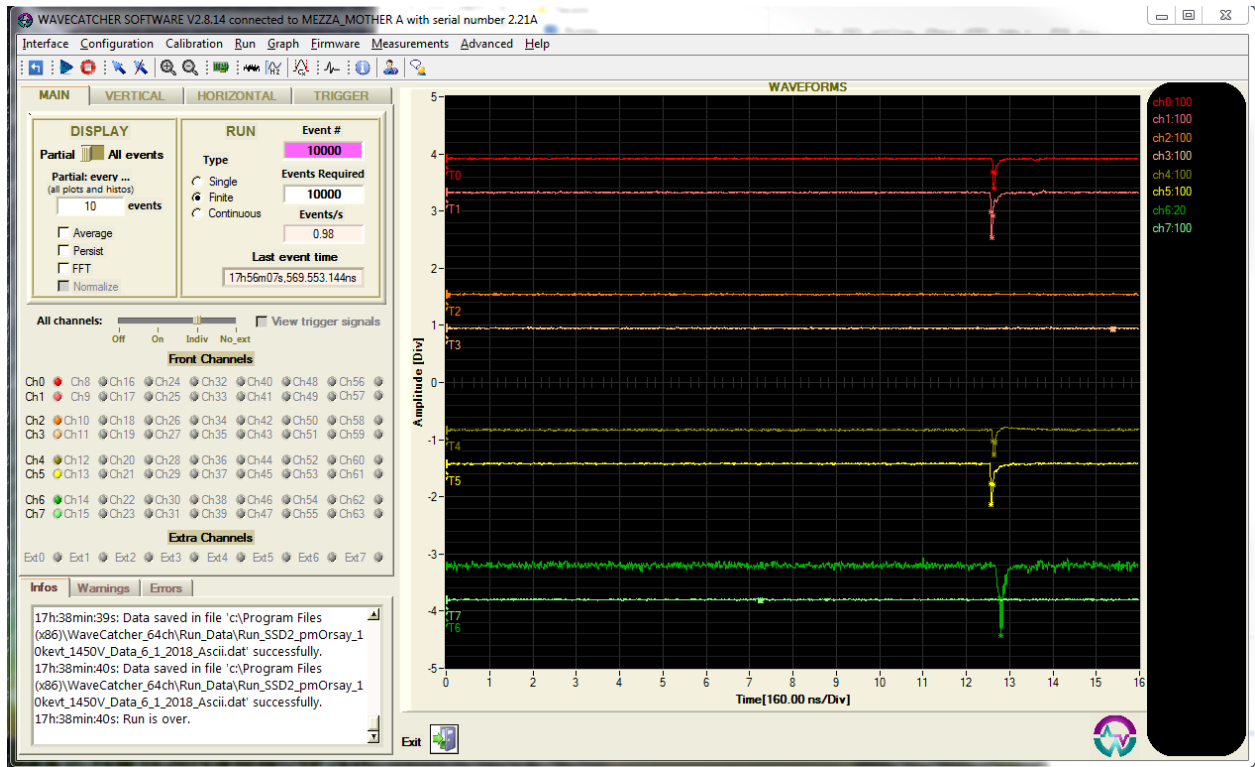
Figure 5.12: A screenshot of the WaveCatcher software, taken during acquisition. This interface allowed us to control that the acquisition was going smoothly and to check for any major lightleaks.
