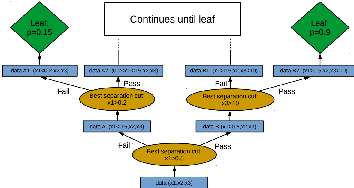
Figure 6.18: Simplified scheme of a decision tree training.
