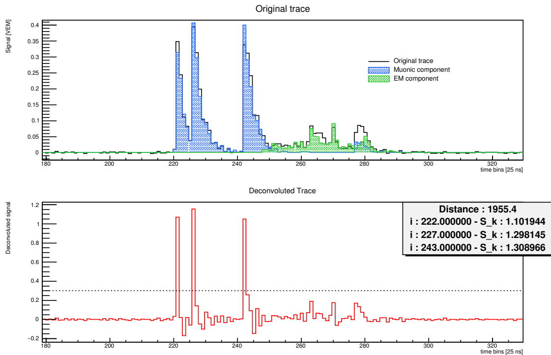
Figure 6.16: The muonicity process applied on a simulated VEM trace, with the muonic and EM components highlighted in different colors.
