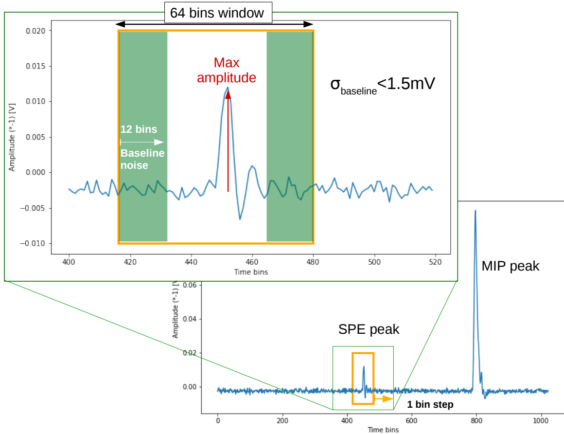
Figure 5.13: Simplified scheme of the sliding window search performed on the traces (see text).
