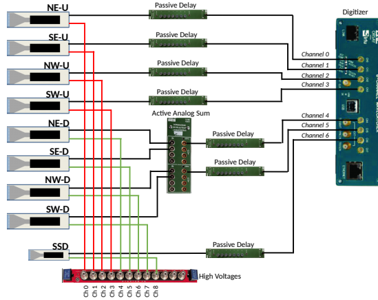
Figure 5.11: Scheme presenting the way the PMTs are read-out with the WaveCatcher digitizer.
