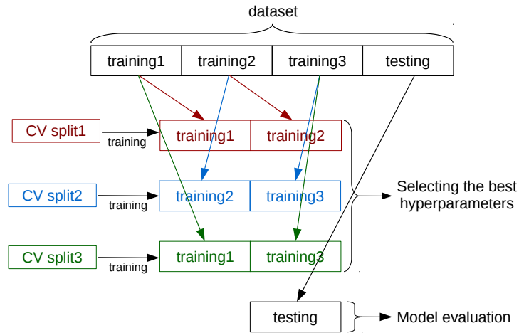
Figure 7.3: Scheme of the cross-validation (CV) process performed on the ML-models to select the best hyperparameters.
