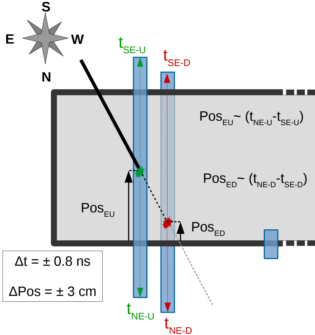
Figure 5.15: Scheme of the procedure to reconstruct the position at which a particle went through the boards to trigger the test bench. The time difference between the signals from both side of a single scintillator bar of the external trigger, can be directly linked to the position of the triggering particle.
