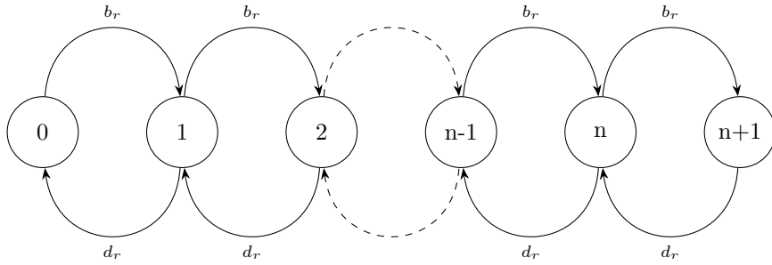
Figure 1.5: Transition between the states in birth and death process
