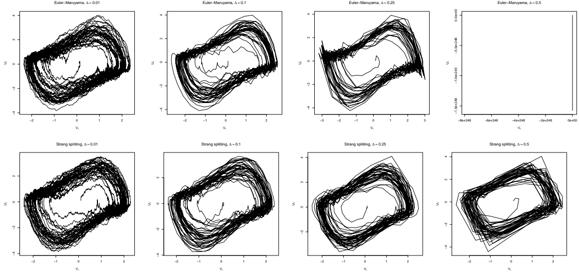
Figure 2.1: Comparison of the performance of the Euler-Maruyama and Strang splitting schemes, applied to the stochastic Van der Pol oscillator (Example 2.1). Parameters used for simulation: \mu = 1, \sigma = 0.5 . Top row: phase portrait of the process, simulated with the Euler-Maruyama approximation, bottom row: phase portrait of the process, simulated with the Strang splitting. Step size \Delta = 0.01, 0.1, 0.25, 0.5 respectively, time interval is [0, 250] , initial values (0.1, 0.1) .
