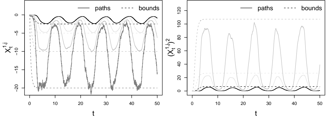
Figure 4.1: First (left panel) and second (right panel) moment bounds with respective trajectories of the inhibitory population k = 1 . The rate function f_2 is given in Section 4.6. The parameters are \eta_1 = 3 , \nu_1 = 2 , N = 20 and p_2 = 1/2 .
