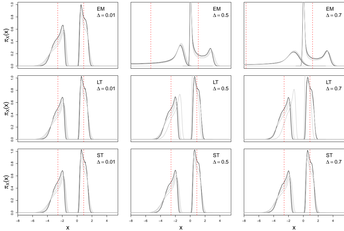
Figure 4.7: Empirical density of the system, simulated with the Euler-Maruyama scheme (top), the Lie-Trotter (middle) and the Strang (bottom) splitting scheme for varying \Delta and T = 10^5 .
