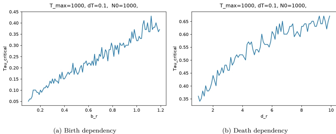
Figure 5.6: Dependency on the threshold for extinction \tau_{ext} with respect to the birth rate b_r and death rate d_r .
