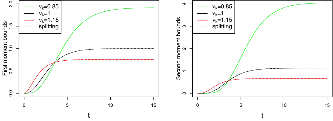
Figure 4.2: First (left panel) and second (right panel) moment bounds of the excitatory population k = 2 for different values of \nu_2 . The moment bounds for the diffusion are in solid lines and the moment bounds for the splitting scheme are in dashed lines. The bound of the rate function is fixed to f_1^{\max} = 1 . The parameters are \eta_2 = 3 , N = 100 , p_1 = 1/2 and the time step \Delta = 0.1 is used.
