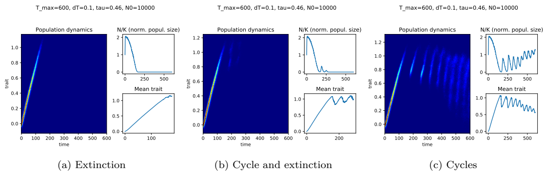
Figure 5.2: Different behaviors for \tau_0 = 0.46 (and the other parameters as in Figure 5.1).
