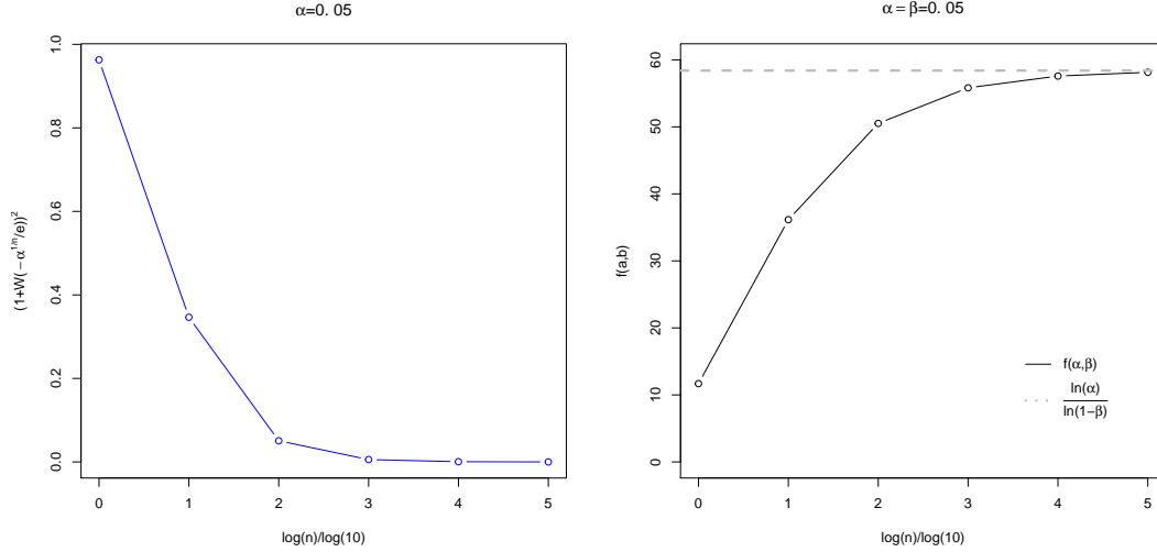
Figure 7.1: Left panel: evolution of the function \left(1+W\left(-\frac{\alpha^{1/n}}{e}\right)\right)^2 as n grows, for \alpha = 0.05 . Right panel: evolution of the function f(\alpha, \beta) = \left(\frac{1+W\left(-\frac{\alpha^{1/n}}{e}\right)}{1+W\left(-\frac{(1-\beta)^{1/n}}{e}\right)}\right)^2 as n grows and its limit value, for \alpha = \beta = 0.05 .
