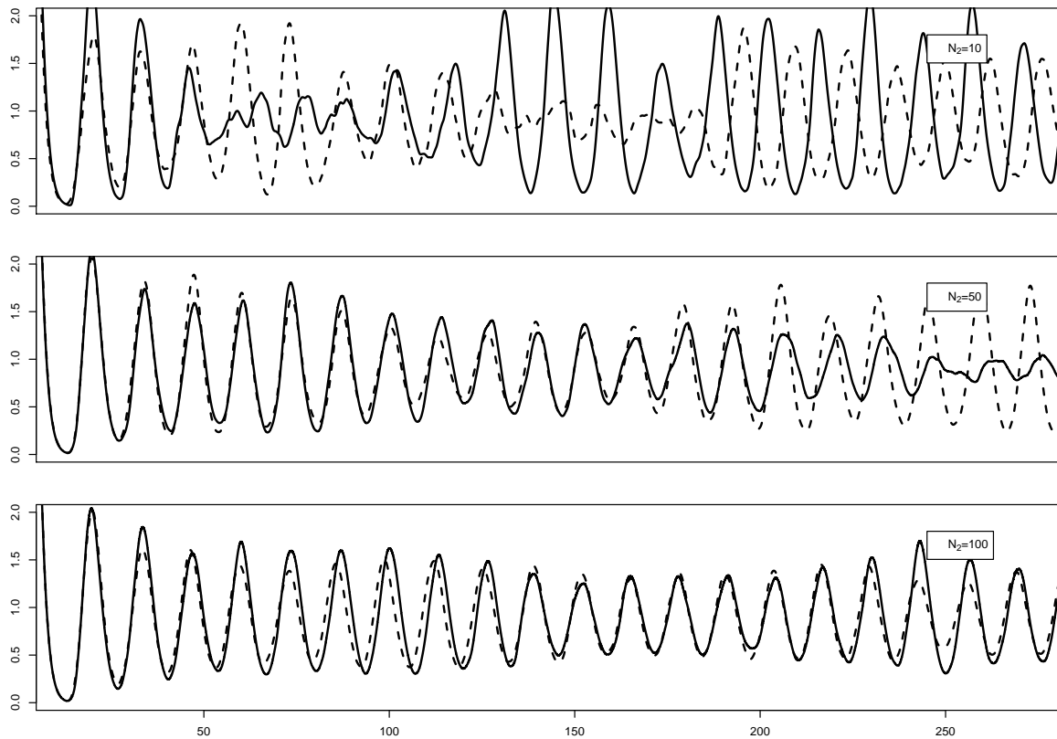
Figure 4.9: Sample trajectories of the PDMP and the diffusion for varying N (excitatory population). Solid line: main variable of \bar{X} , dashed line: main variable of X (simulated with the Strang splitting scheme, using \Delta = 0.01 ).
