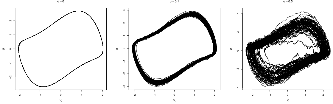
Figure 1.3: Phase portrait of a Van Der Pol oscillator (Example 2.1) under different random perturbation forces.
