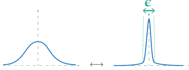
Figure 3.2: Shape of \frac{f}{\rho_\varepsilon} under the time rescaling
