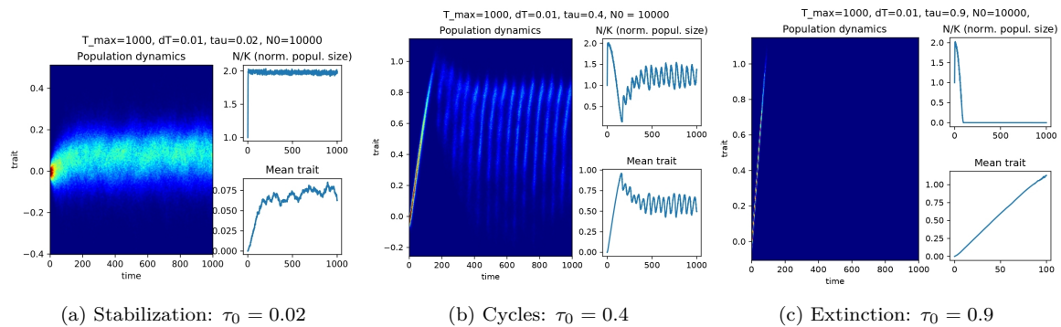
Figure 5.1: Behavior of the population dynamics as the mutation rate \tau_0 is changing, ( b_r = d_r = 1 , \sigma = 10^{-2} , K = 10^4 , \sigma^0 = 10^{-2} , x_{mean}^0 = 0 , N^0 = 10^4 ).
