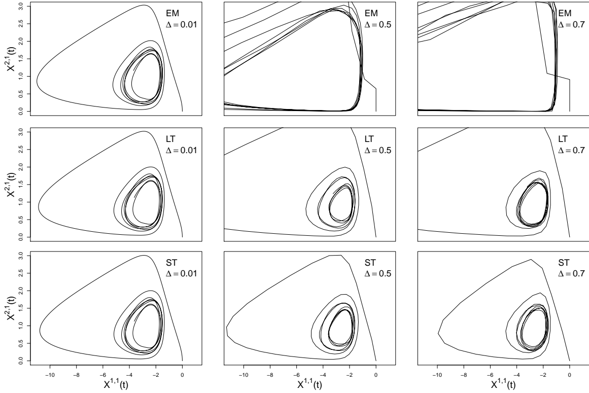
Figure 4.6: Phase portrait of the main variables, simulated with the Euler-Maruyama scheme (top), the Lie-Trotter (middle) and the Strang (bottom) splitting scheme for varying \Delta and x_0 = (0, 0, -3.5, -4, 0, 1.3, 1.1) .
