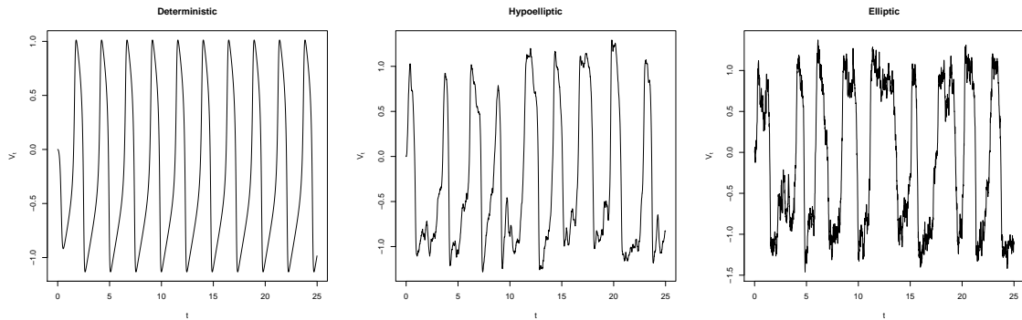
Figure 1.4: Membrane potential V_t of a neuron in a FitzHugh-Nagumo neuronal model in the deterministic, hypoelliptic and elliptic cases.
