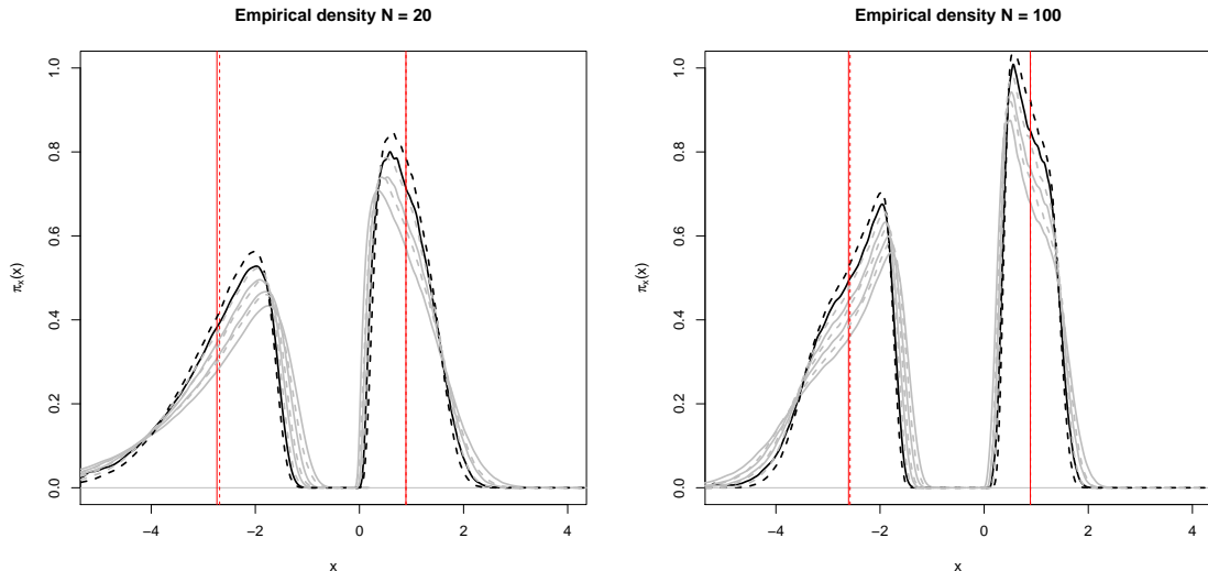
Figure 4.10: Empirical density of the PDMP and the diffusion for N = 20 (left) and N = 100 (right). Solid line: \bar{X} , dashed line: X (simulated with the splitting scheme, \Delta = 0.1 , T = 10^5 ). The red solid and dashed vertical lines denote the mean of the respective main variables.
