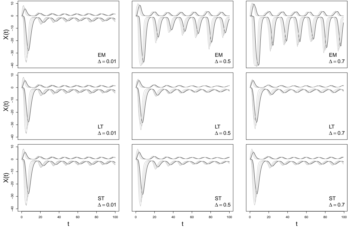
Figure 4.5: Sample trajectories of the system, simulated with the Euler-Maruyama scheme (top), the Lie-Trotter (middle) and the Strang (bottom) splitting scheme for varying \Delta .
