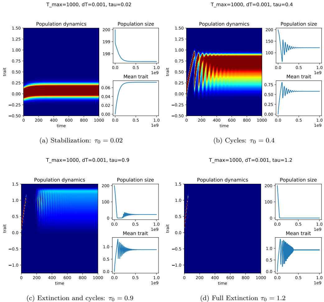
Figure 5.4: Behavior of the population dynamics described by a PDE model as the mutation rate \tau_0 is changing, ( b_r = d_r = 1 , \sigma = 0.01 , \varepsilon = 1 ).
