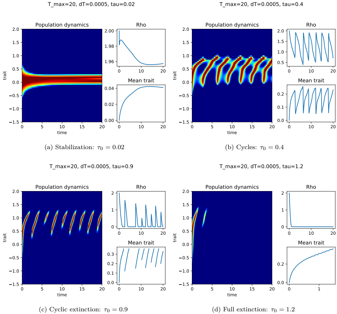
Figure 5.5: Behavior of the population dynamics described by a PDE model for \varepsilon = 0.01 as the mutation rate \tau is changing, ( b_r = d_r = 1, \sigma = 1 ).
