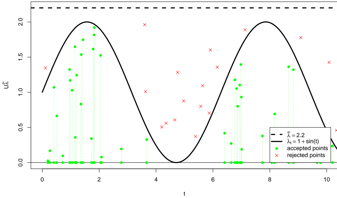
Figure 2.2: Illustration of the acceptance-rejection method: spiking times t_i are generated by law \mathcal{E}(\tilde{\lambda}) and accepted, if U\tilde{\lambda} < \lambda_{t_i} , where U \sim \mathcal{U}([0, 1]) . Plotted points are values of U\tilde{\lambda} at times t_i .
