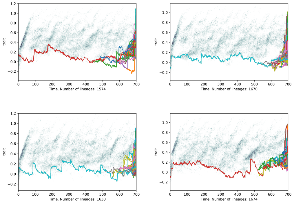
Figure 5.3: Simulations on the stochastic model with lineages. \tau_0 = 0.4 , T_{max} = 700 , dT = 0.1 , K = N_0 = 1000 and other parameters as in Figure 5.1.
