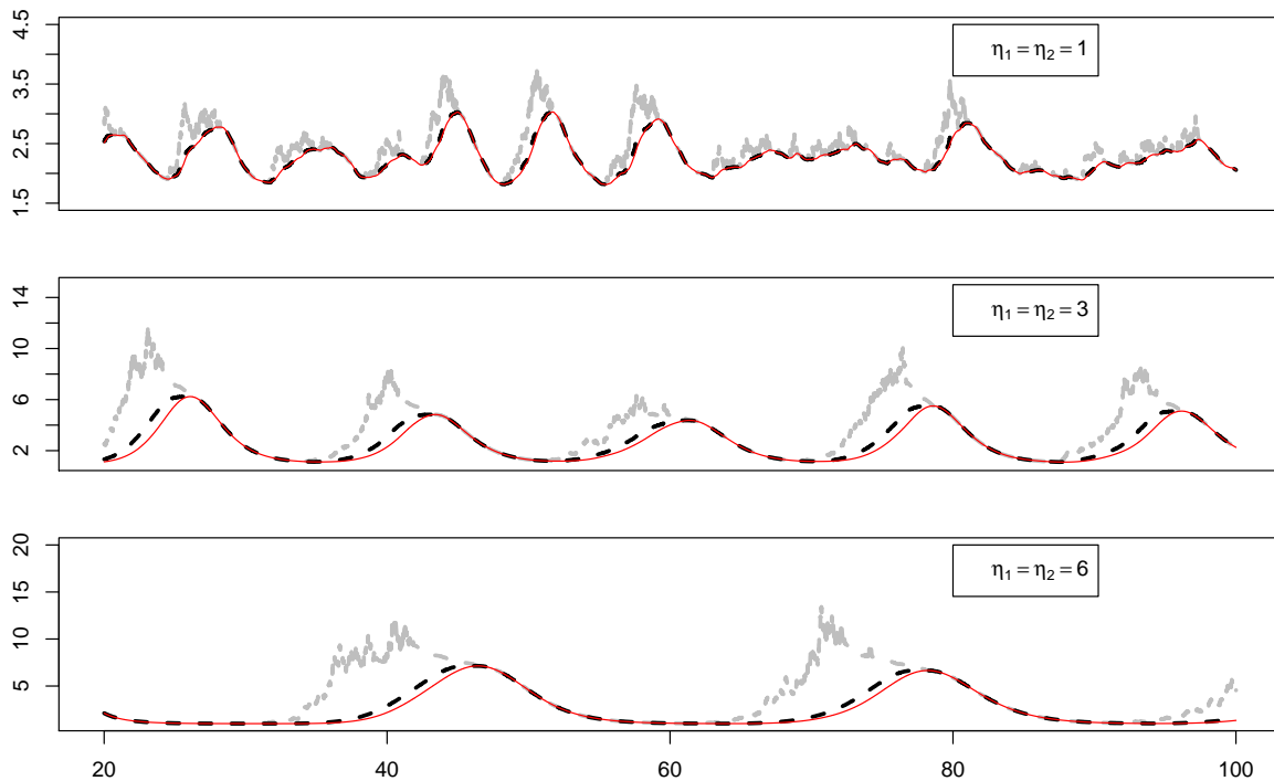
Figure 4.3: Intensity and intensity bounds for the second population (excitatory) t \in [20, 100] . Red solid line: true intensity \lambda_t^2 , black dash line: \tilde{f}_2^{\tilde{\Delta}}(\bar{X}_t) , grey dash line: \tilde{f}_2(\bar{X}_t) . Intensity functions f_1 and f_2 are given by (4.24), \nu_1 = \nu_2 = 0.9 , N_1 = N_2 = 50 .
