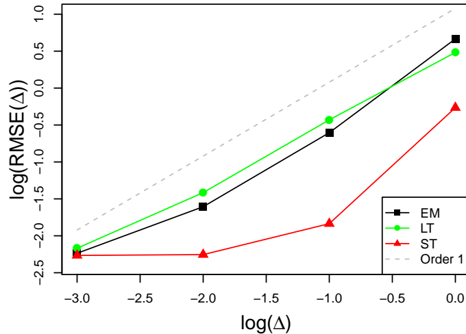
Figure 4.4: Mean-square order of convergence. The reference solution is obtained with the Euler-Maruyama method and the small time step \Delta = 10^{-4} . The numerical solutions are calculated for \Delta = 10^{-3}, 10^{-2}, 10^{-1}, 10^0 . The log is with base 10, t^* = 1 and M = 10^3 .
