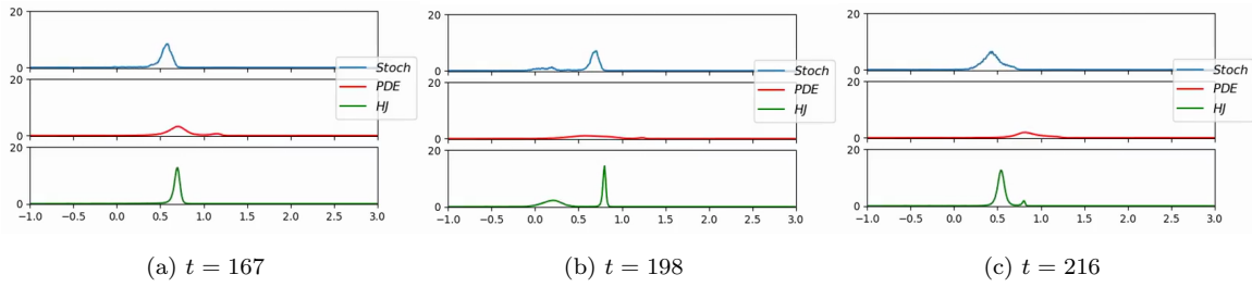
Figure 5.7: Comparison of numerical simulations between the different models. \tau_0 = 0.4 , \varepsilon = 0.1 , \delta = 0.001 and other parameters as in Figure 5.1. Blue line stands for the stochastic model, red line: for a PDE, green — for a Hamilton-Jacobi PDE
