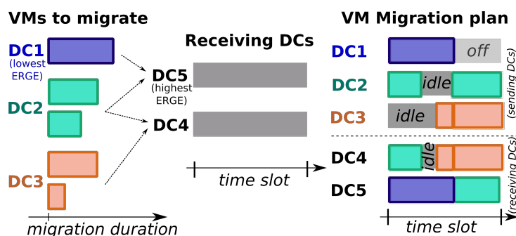
Figure IV.8 – Example of VM migrations with 5 data centers
