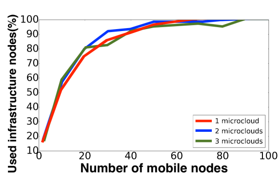
Figure III.7 – Utilization of the network
