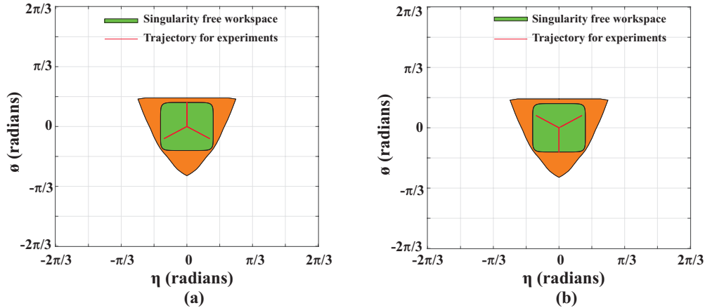
Figure 4.6 – Trace of the desired input trajectories chosen for the (a) one spring pull and (b) two springs pull experiments within the workspace of the tensegrity mechanism
