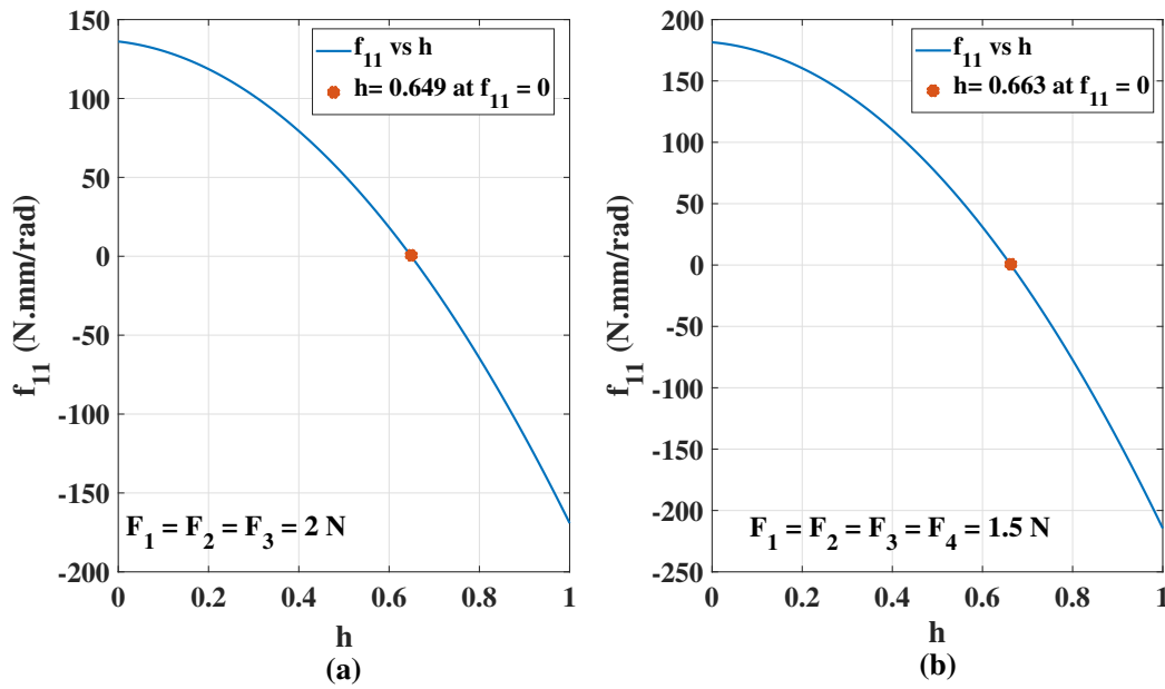
Figure 3.22 – Optimum value of h at spring stiffness of 0.75 N/mm for the (a) 3-SPS-U and (b) 4-SPS-U mechanisms under the presence of external forces
