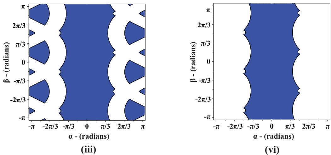
Figure 3.7 – Results obtained by CAD algorithm from Maple with representation of (i),(ii),(iii): Feasible and non-feasible solutions and (iv),(v),(vi): Extraction of geometrical workspaces around the home-pose for the three case study postures
