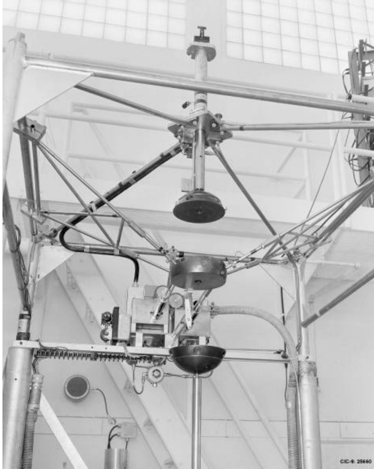
FIGURE 2.1 – Godiva device in scrambled position [10].
