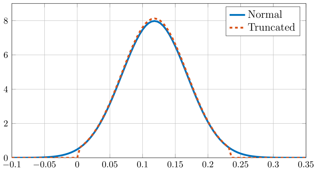
Figure 4.9: Distribution of \alpha .
