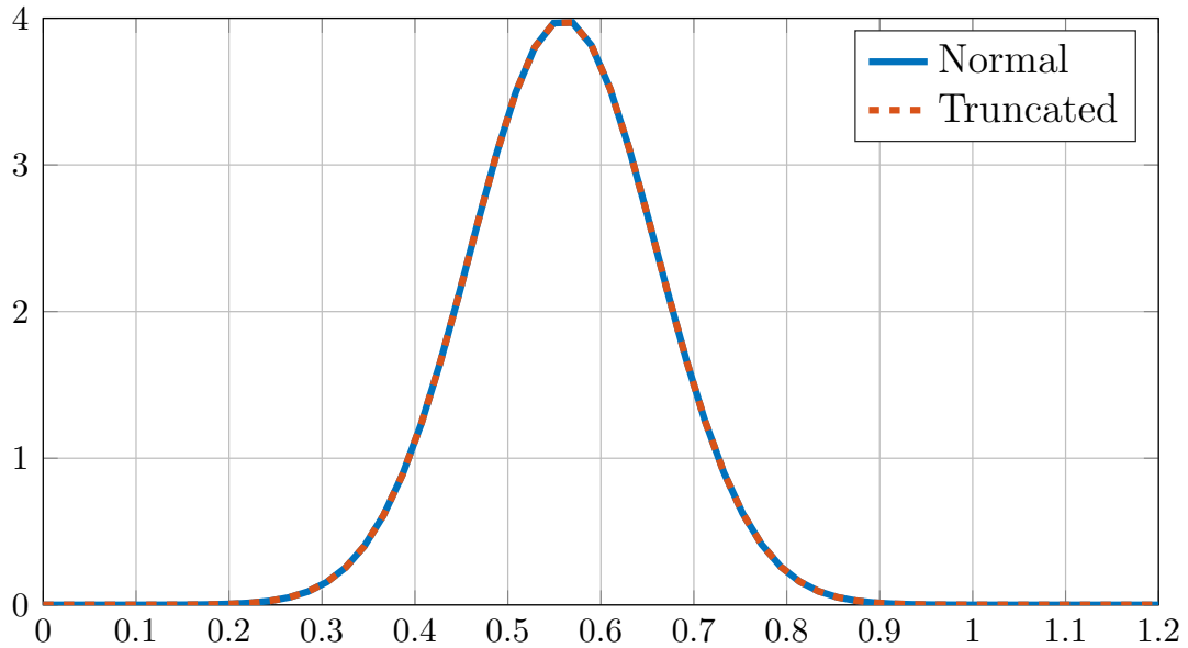
Figure 4.8: Distribution of \mu_C .
