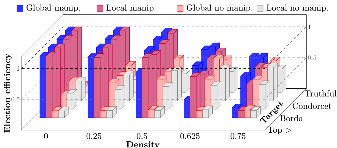
Figure 5.10: Algorithm 5.2 in local and global poll-confident BBR_p -dynamics where p = (5, \dots, 5) for different densities of network
