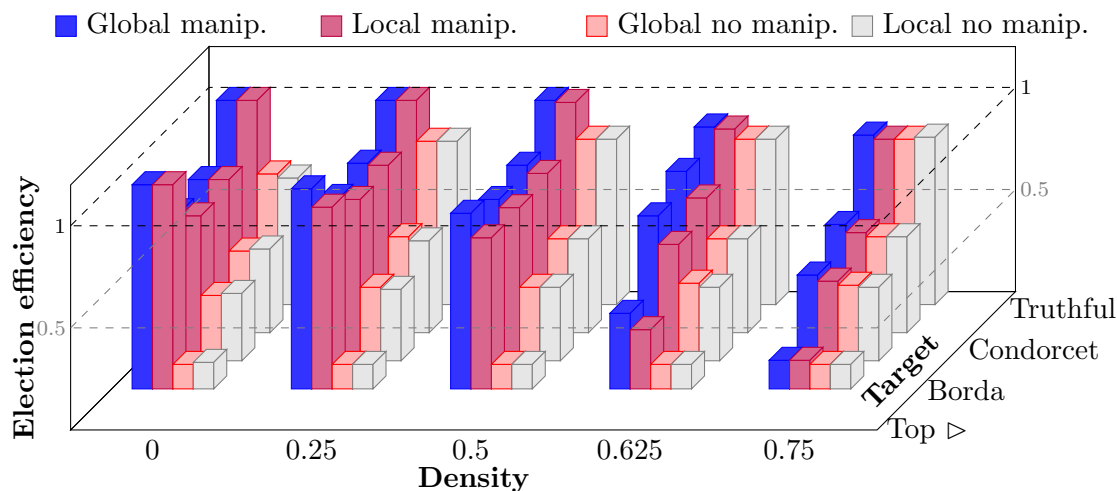
Figure 5.9: Algorithm 5.2 in local and global poll-confident BBR_p -dynamics where p = (1, \dots, 1) for different densities of network
