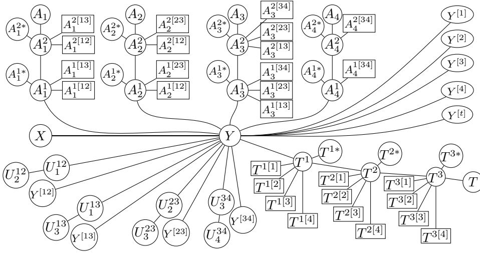
Figure 3.4: Graph construction for an instance of CLIQUE with vertices \mathcal{V} = \{1, 2, 3, 4\} and k = 3 . The edges are: \{1, 2\} , \{1, 3\} , \{2, 3\} and \{3, 4\} .
