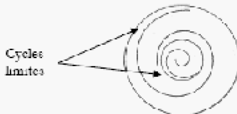
Figure tirée de [POINCARÉ, H., 1882a], p. 59
