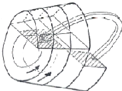
Fig. 15 Nontrivial reinjection between different portions of a 3-dimensional flow. Example of a generalized (three-dimensional) paper model.
