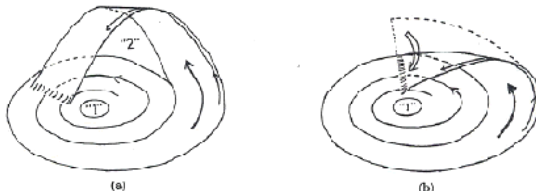
Figure 3. (a) "Paper-sheet model" of the flow of Figure 1. (b) Prototype. "1", "2" = allowed holes - (---) mixing line
