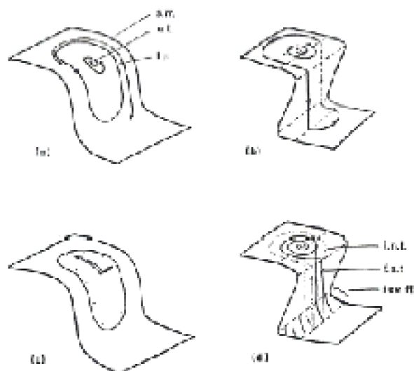
Fig. 1. Main trajectory-set flow of a universal circuit. a) Nearly linear mode. b) Relaxation mode. c) Analogous "Soft Wash" (after Salvador Dalí's synonymous painting, 1933). d) Chase-producing mode (see text). s.m. = slow manifold, u.f. = unstable focus, l.c. = limit cycle, the intermediate part of slow manifold in (b) and (d) is unstable, l.s.t. = "first switched trajectory", l.m.t. = "last nonswitched trajectory", rev.H. = reversed direction of flow "downstairs".
