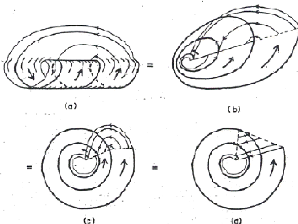
Figure 10. Three views of the same paper-sheet flow of Figure 9c, taken from three different perspectives, proving equivalence to the flow of Figure 3b. a = Figure 9c; d = Figure 3b; b, c = intermediate stages
