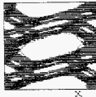
Fig. 5.2 The same as in fig. 5.1 except K=1.0 ( q=10^6 ).
