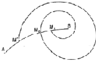
Figure tirée de [POINCARÉ, H., 1882a], p. 45
