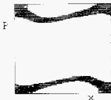
Fig. 5.1 Phase map of system (5.2): K=0.9q ; q=2 ; P_0=0.000000^{\circ} ; X_0=0.000000^{\circ} ; n=10^4 ; resolution: 128 \times 128 bits.
