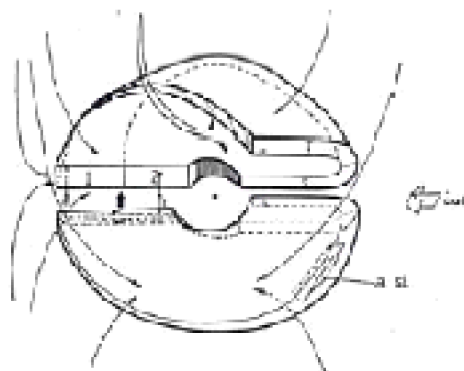
Fig. 9. The "three-dimensional blender". (Cf. Fig. 8a.) — = Trajectories entering the structure from the outside; 1, 2 = half cross-sections (demonstrating the 'mixing transformation' that occurs); a = entry point of some arbitrarily chosen trajectory; r = centre point of the same trajectory after one cycle; † = 'bounces map'; a.s. = allowed slit
