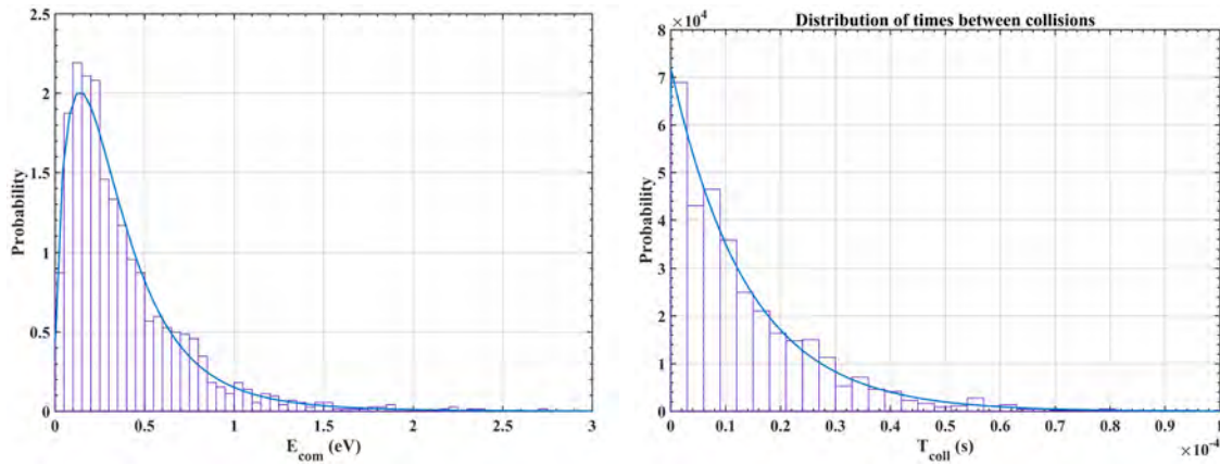
Figure 5.6 Calculated distributions of E_{\text{com}} and the time between collisions, T_{\text{coll}} , for a DE at 200 mV and 10^{-3} mbar of Ar buffer gas pressure.
