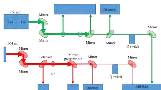
Figure 2.6 Laser scheme and picture of the optical table.
