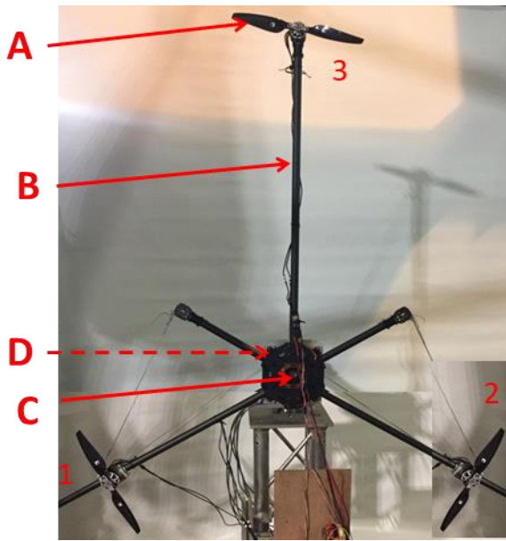
Figure 56: Multi-actuators test bench. The actuators are numbered 1, 2 and 3.
