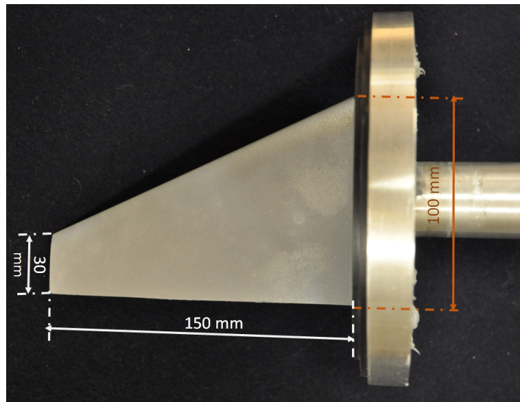
FIGURE 2.6 – POM hydrofoil
