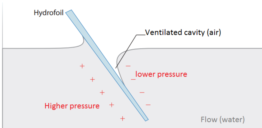
FIGURE 1.15 – Ventilation phenomenon [101]
