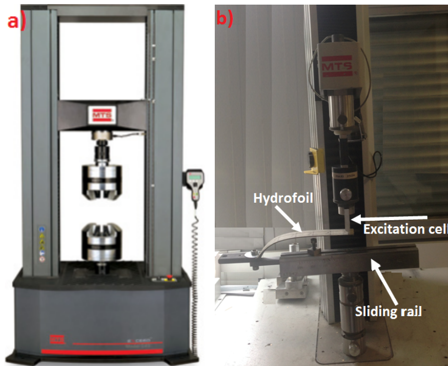
FIGURE 2.7 – a) Tensile test bench. b) Adaption of the bench for bending tests.
