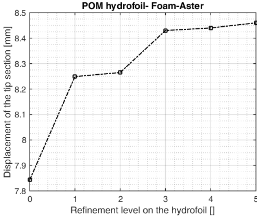
FIGURE 5.4 – Evolution of the displacement at the tip of the hydrofoil with the refinement around the foil in the fluid domain. Re = 7 \times 10^5 and \alpha = 10^\circ .
