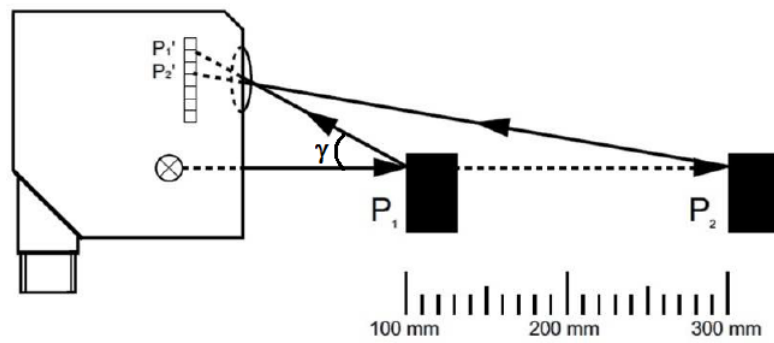
FIGURE 2.18 – Laser principle.
