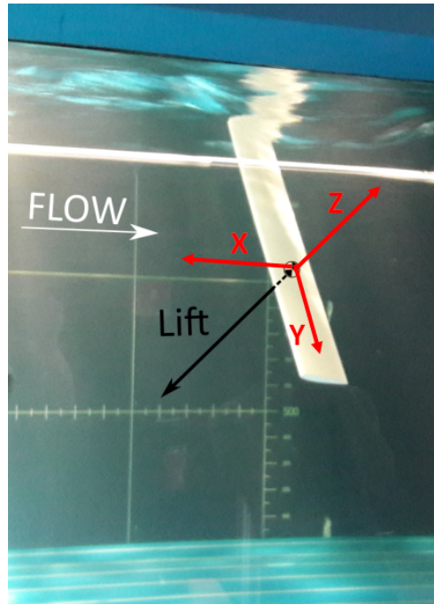
FIGURE 2.53 – Picture of the hydrofoil tested in IFREMER Lorient flume at 0.9ms and \text{AoA} = -9^\circ , from the observation window.
