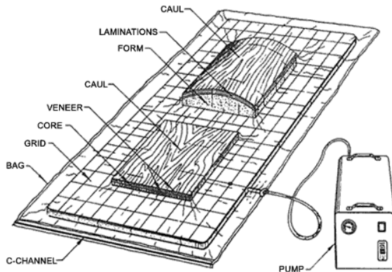
FIGURE 2.32 – Vacuum press.
