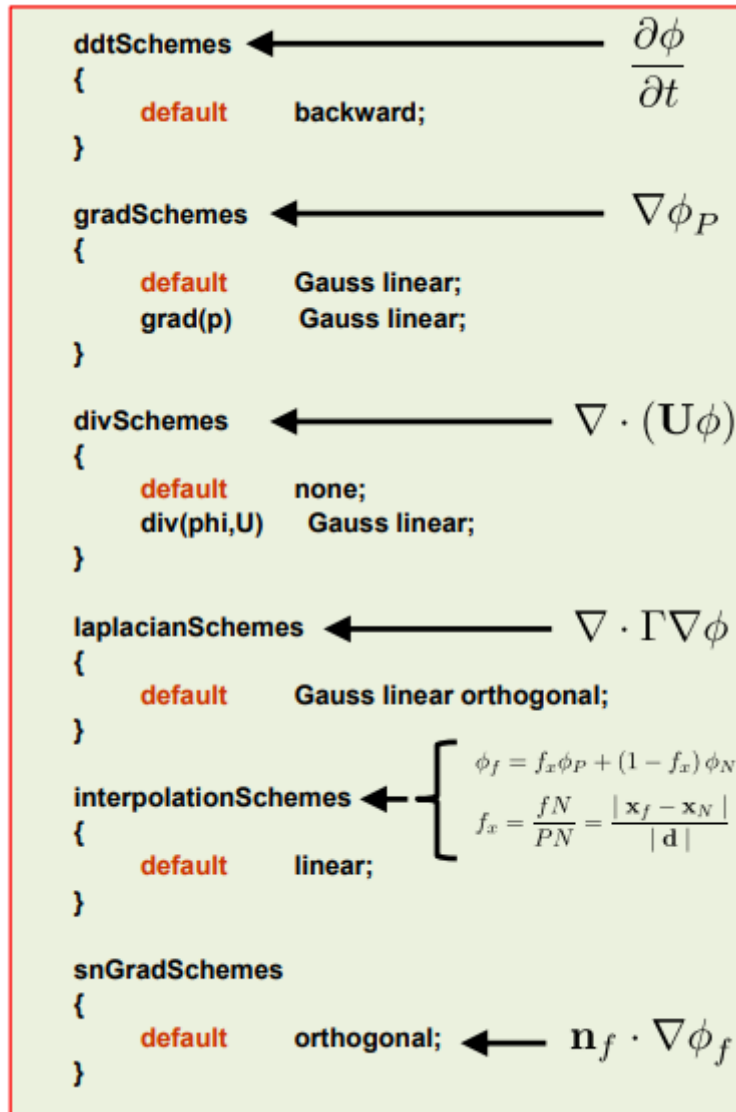
FIGURE 3.17 – Discretization schemes chosen for the simulations of OpenFOAM in the present work.
