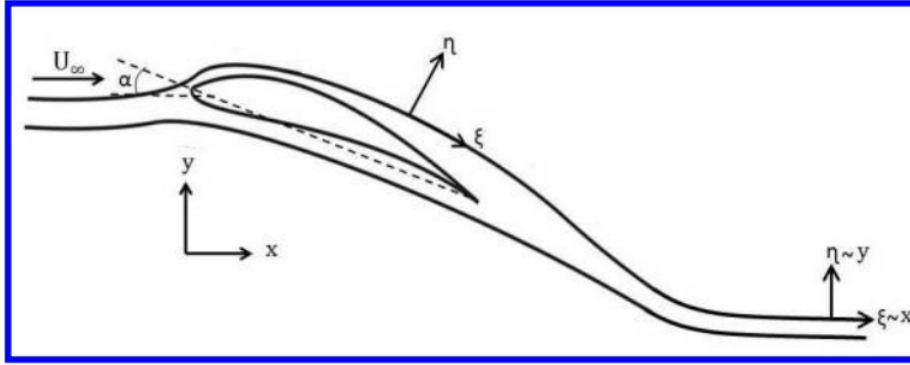
FIGURE 3.8 – Cartesian (x, y) and Streamwise (\xi, \eta) directions on an airfoil. U_\infty is the stream flow and \alpha is the angle of attack. [104]
