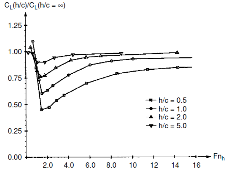
FIGURE 3.9 – Lift coefficient with the submerged Froude number Fn_h [49]
