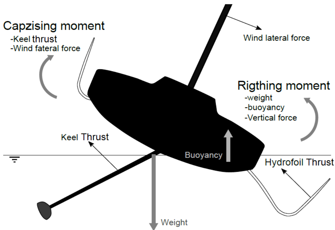
FIGURE 1.1 – Equilibrium of a modern 60 Imoca foiling yacht. Inspired from VPLP [122].
