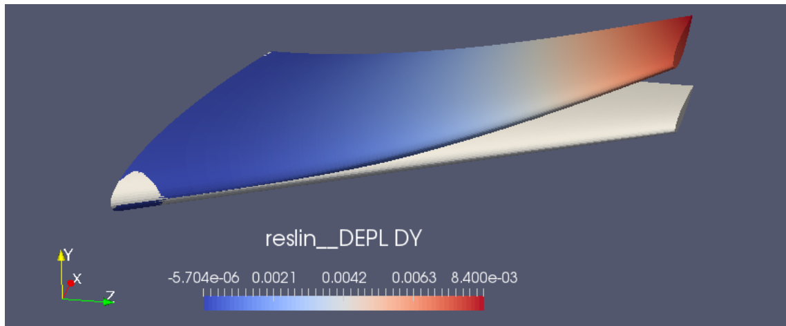
FIGURE 5.12 – Displacement of the POM hydrofoil after a FSI simulation for \alpha = 10^\circ .
