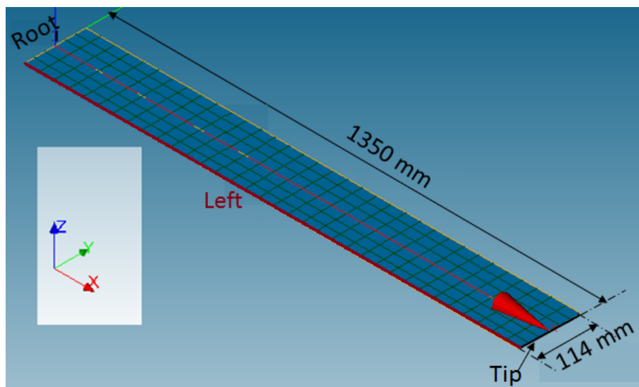
FIGURE 5.17 – Geometry of the plate used for BTC analysis with Code_Aster, 1350 \times 114 \times 17.1\text{ mm}^3 .
