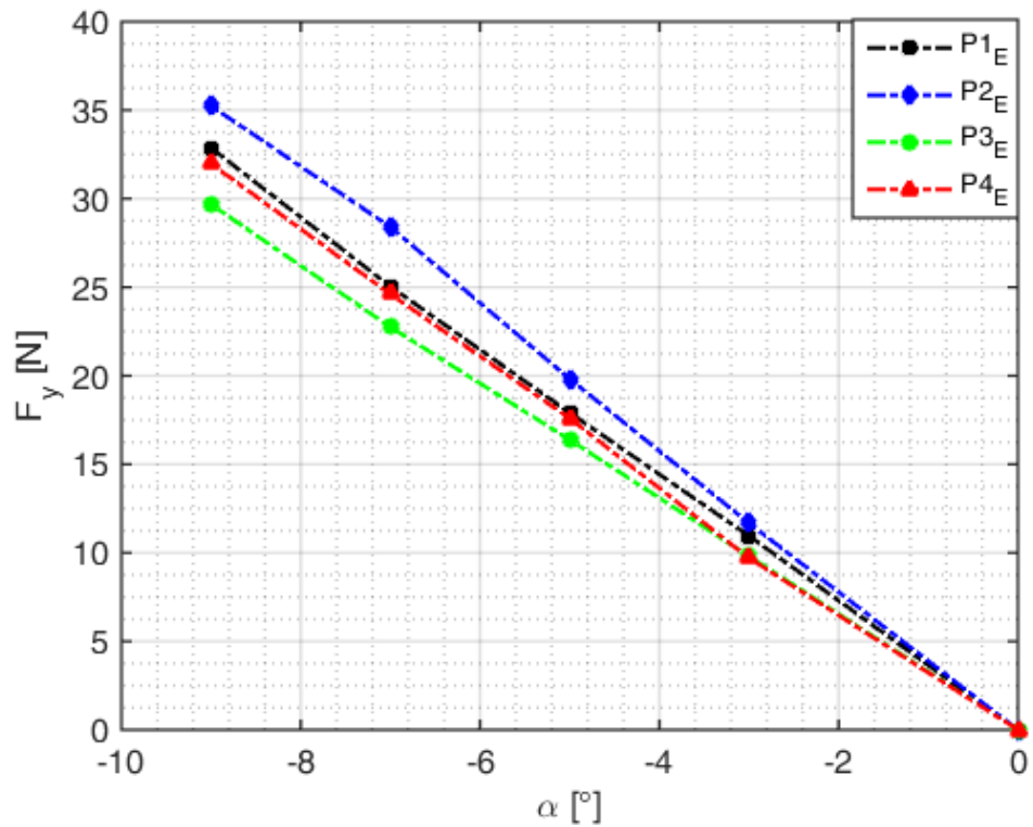
FIGURE 4.36 – Projection on Y axis of the lift force measured on the composite hydrofoils, U = 0.9\text{ m/s} .
