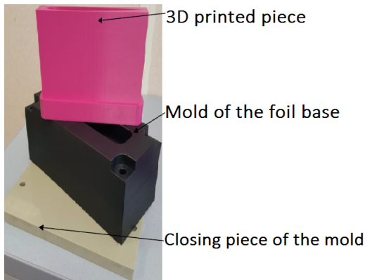
FIGURE 2.35 – Setup of Foil base 's molding
