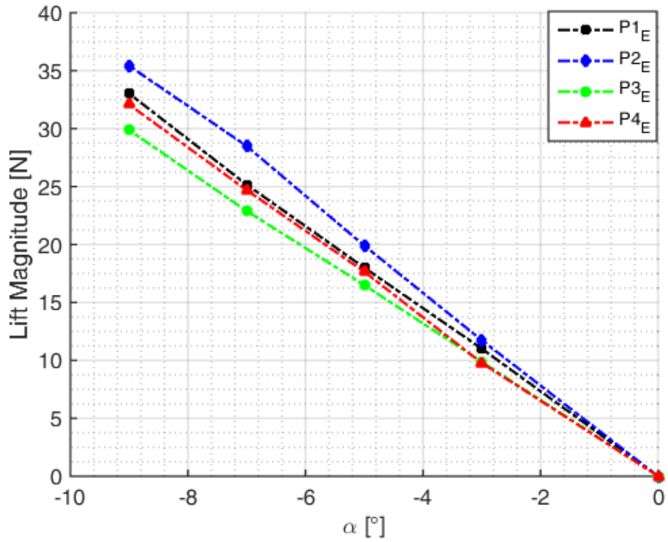
FIGURE 4.35 – Lift force measured on the composite hydrofoils, U = 0.9\text{ m/s} .
