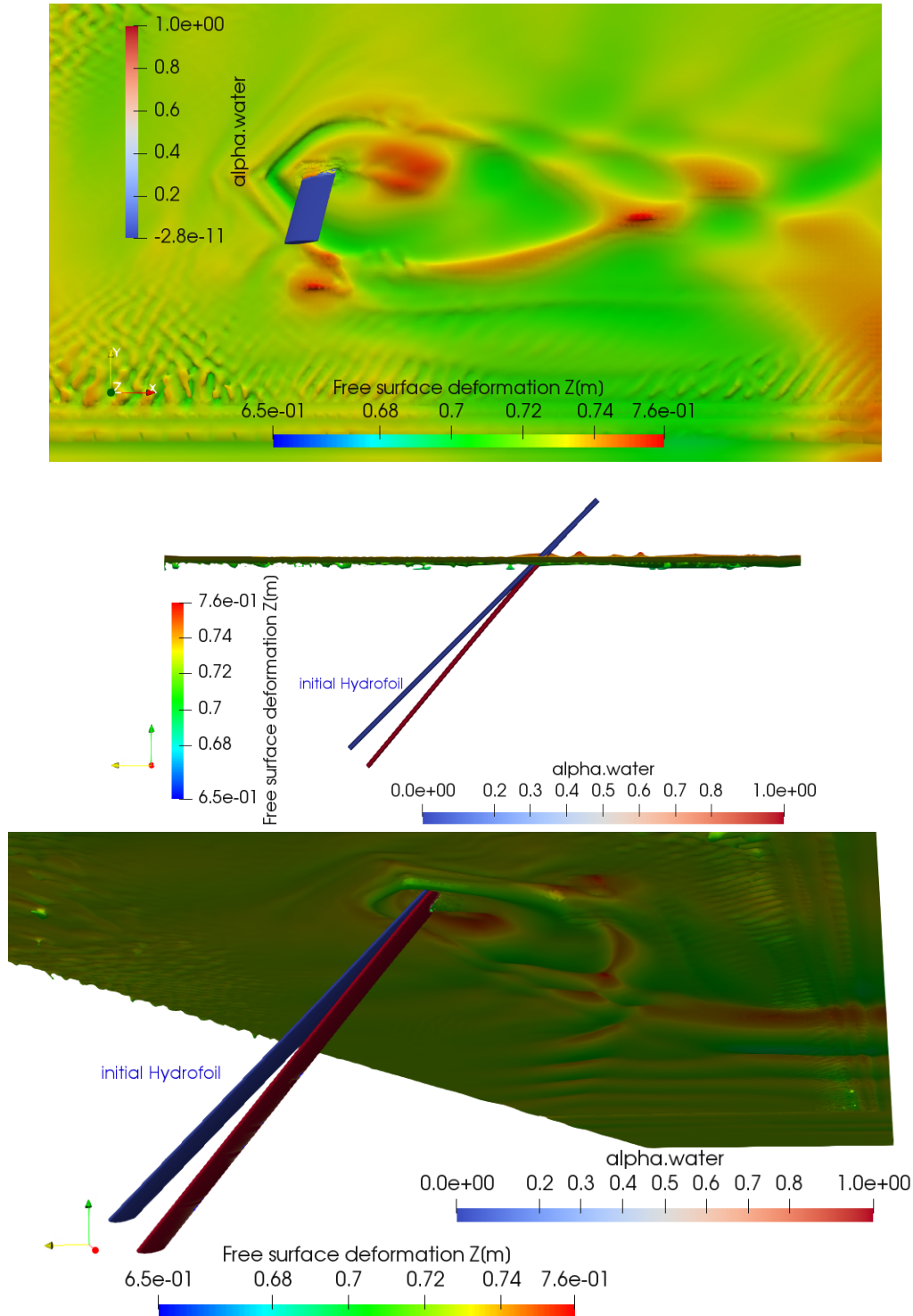
FIGURE 5.38 – Visualisation of the free surface deformation for the hydrofoil P2, including the initial geometry \alpha = 7^\circ and U=0.9m/s .
