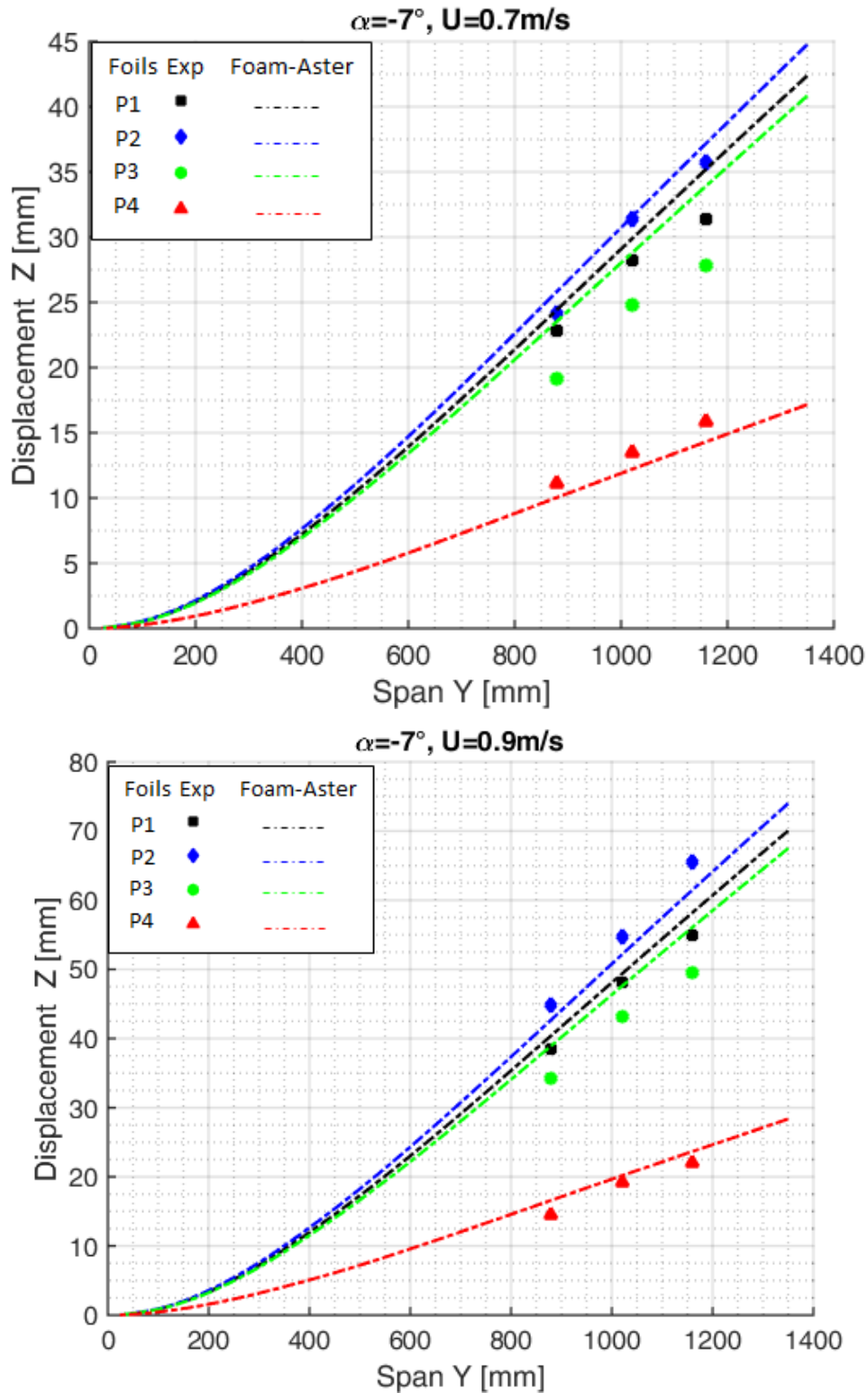
FIGURE 5.35 – Validation of Foam-Aster : Normal displacements of all the hydrofoils, \alpha = -7^\circ , U = 0.7 \text{ m/s} and U = 0.9 \text{ m/s} .
