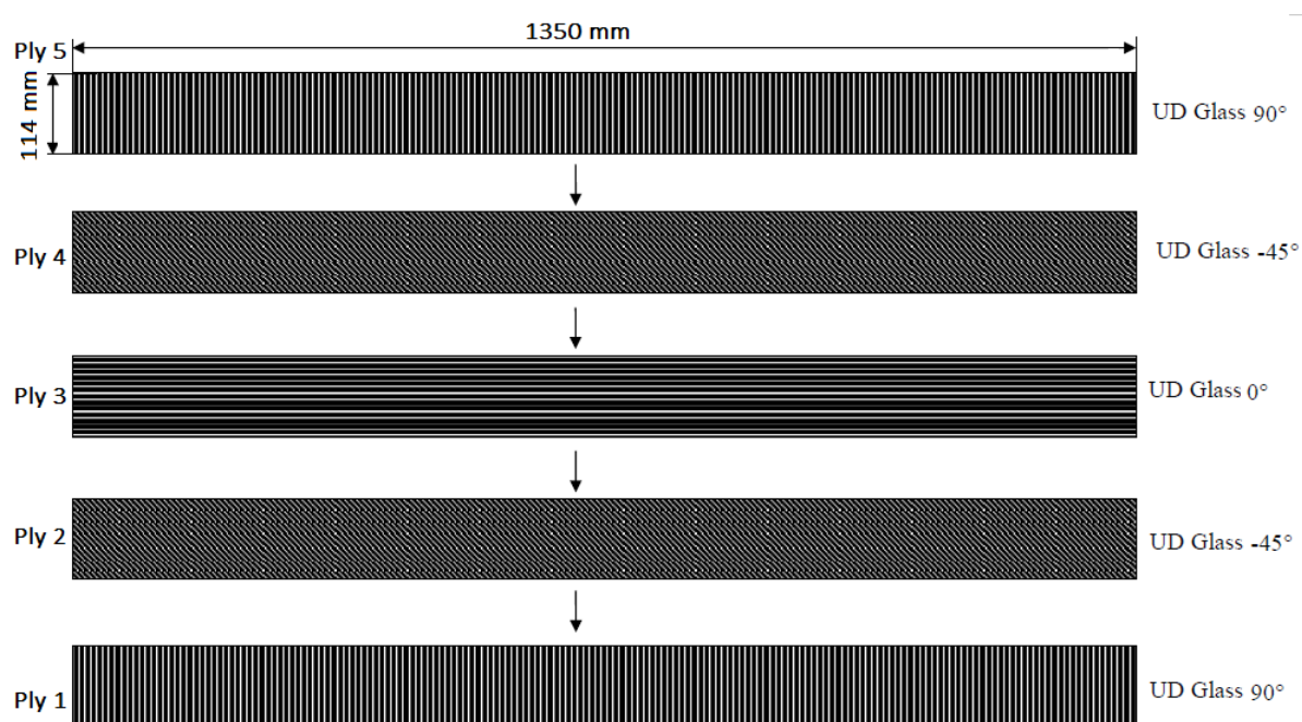
FIGURE B.5 – Orientation of the lies in the layup P_3 .
