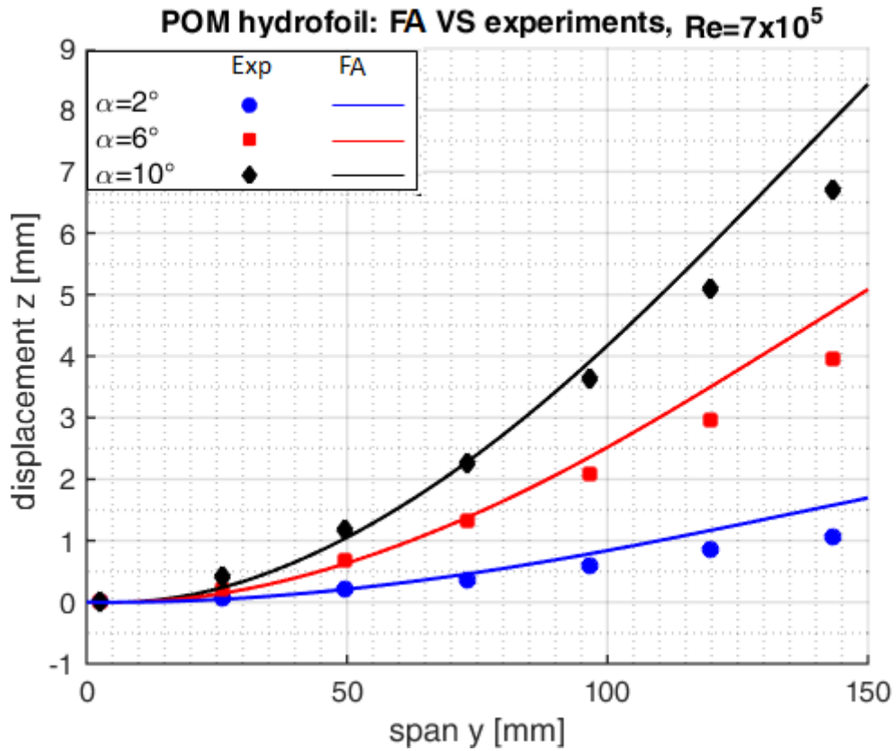
FIGURE 5.11 – Foam-Aster VS experiments : displacements of the POM hydrofoil Re = 7 \times 10^5 .
