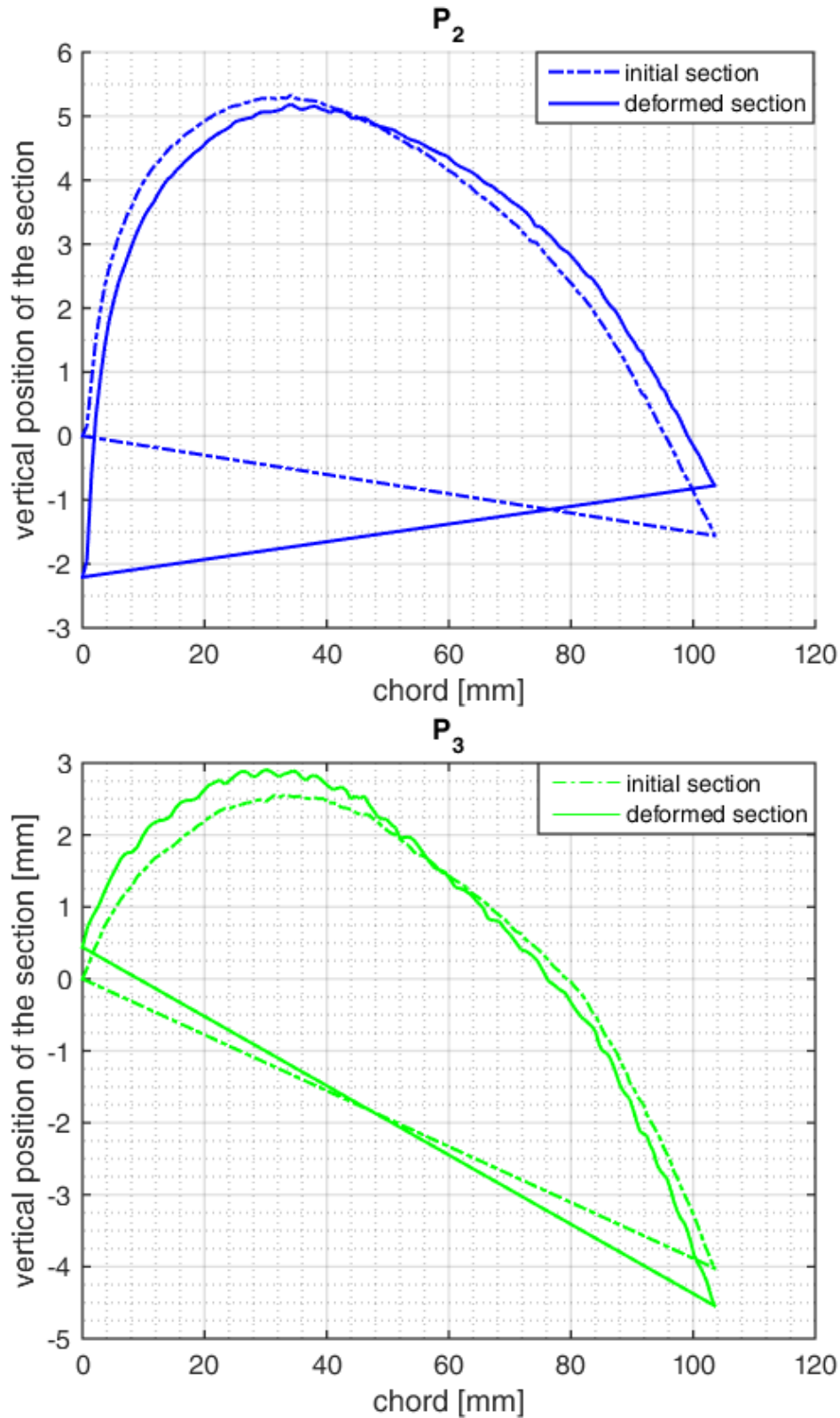
FIGURE 4.32 – Bend twist angle measured for P_2 on the section S_2 and P_3 on the section S_1 , with M_1 loading
