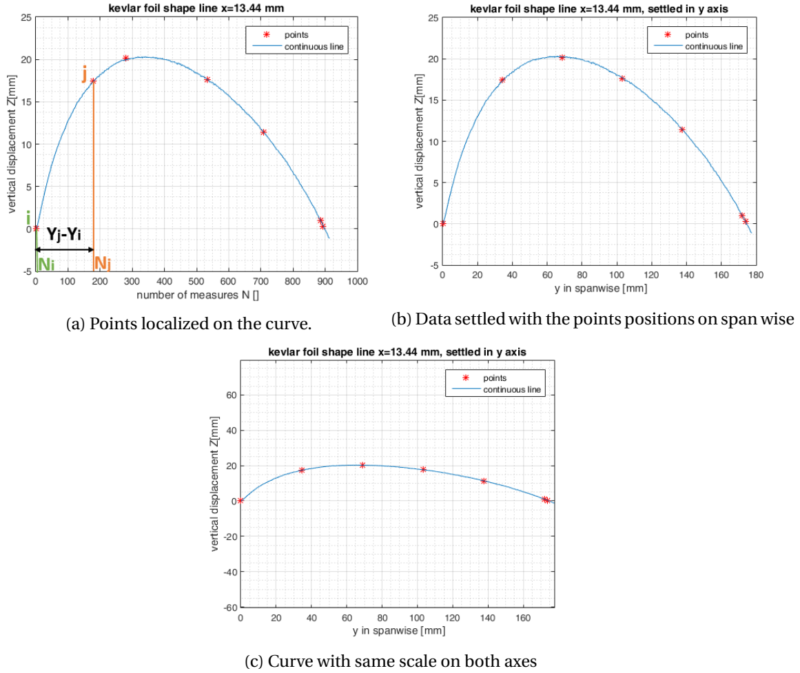
FIGURE 2.57 – Example of post processing of displacement recorded during the hydrodynamic tests : kevlar hydrofoil \alpha = 5.5^\circ at V = 0 \text{ m/s}
