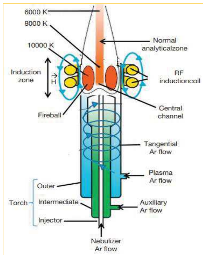
Figure 8. Inductively Coupled Plasma and torch schematic (Fernández-Sánchez, 2018)
