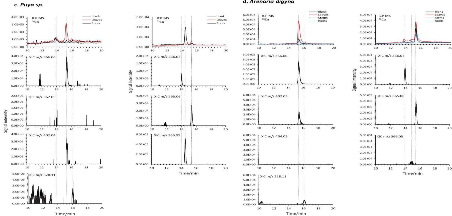
Figure 5. HILIC-ICP/ESI MS speciation of water soluble Cu and Zn species in the leaves, stems, and roots extract of Nicotiana thyrsiflora , Hypericum laricifolium , Puya sp. and Arenaria digyna .
