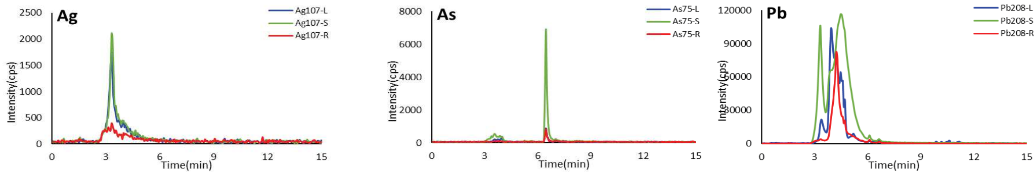
Figure 3. SEC-ICP MS fractionation of the water soluble species of Ag, As, and Pb leaves (blue lines), stems (green lines), and roots (red lines) of Nicotiana thyrsoiflora , Hypericum laricifolium , Puya sp. , and Arenaria digyna
