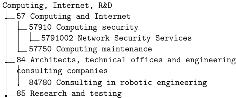
Figure 3.6: KOMPASS example.
