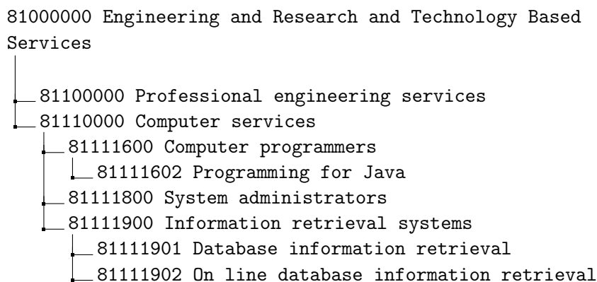
Figure 3.5: UNSPSC example.
