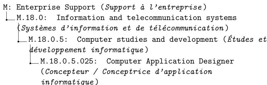
Figure 3.2: ROME example.
