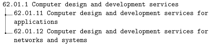
Figure 3.7: CPF example.
