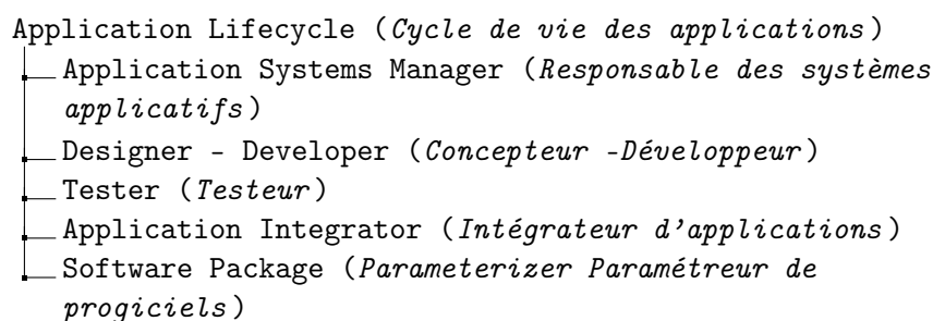
Figure 3.3: CIGREF example.
