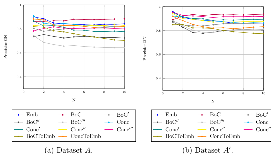
Figure 6.1: Precision@N.
