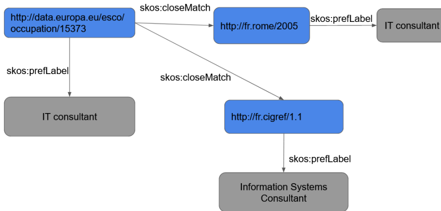
Figure 3.10: Alignment example between ESCO, ROME, and Cigref.
