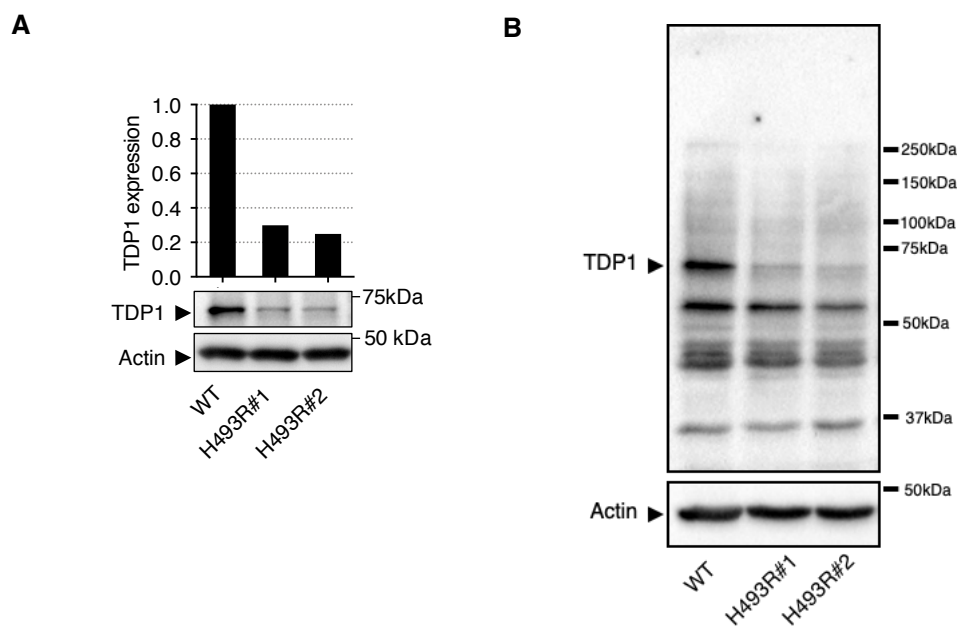
Figure 24. Validation at the protein level of the U2OS H493R TDP1. (A and B) WB analysis of TDP1 levels. Whole cell protein extracts were immunoblotted against TDP1. Actin was used as loading control; (A) Quantification of TDP1 levels relative to actin.
