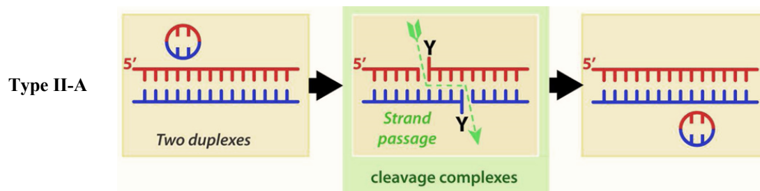
Figure 2: Catalytic mechanisms of type IIA DNA topoisomerases. Type IIA enzymes act by strand passage with double-strand break. Adapted from (Pommier, 2013).
