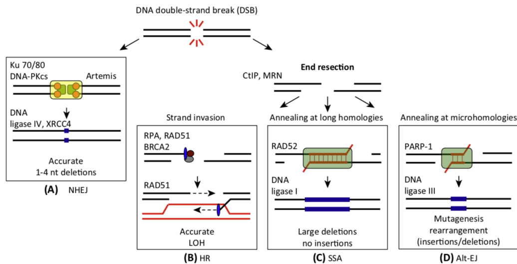
Figure 6: DSBs repair mechanisms. (A) NHEJ; (B) HR; (C) SSA; (D) Alt-EJ. Adapted from (Ceccaldi, Rondinelli and D'Andrea, 2016).
