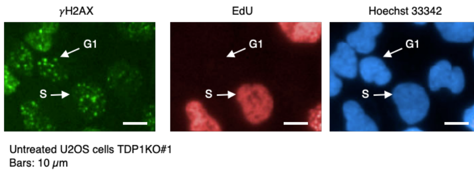
Figure 25. Immunofluorescence microscopy images of untreated cells. U2OS TDP1KO cells untreated incubated with 10 \mu M EdU for 30 min, co-stained for \gamma H2AX (green), and Hoechst33342 (blue). The G1-phase cells are labeled as G1 and the S-phase cells as S. Bars:10 \mu m.
