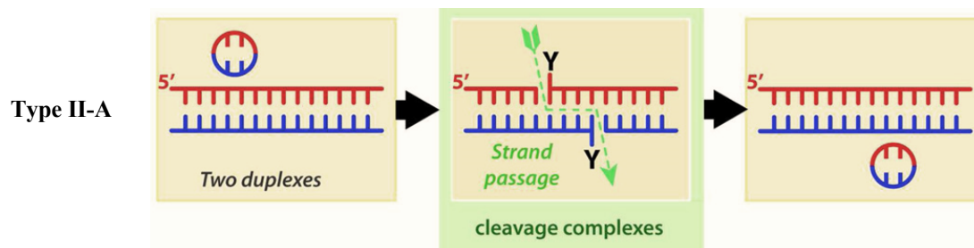
Figure 2: Catalytic mechanisms of type IIA DNA topoisomerases. Type IIA enzymes act by strand passage with double-strand break. Adapted from (Pommier, 2013).
