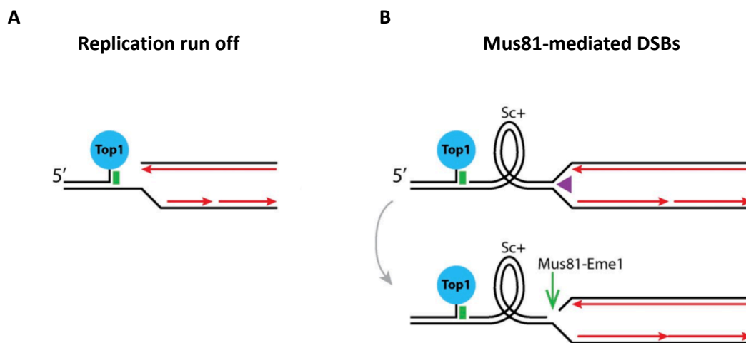
Figure 5: Mechanisms of production of replication coupled DSBs (RC-DSBs) by TOP1cc. (A) Replication run off. (B) Mus81-Eme1 cleavage of the stalled replication fork. Adapted from (Regairaz et al. , 2011).
