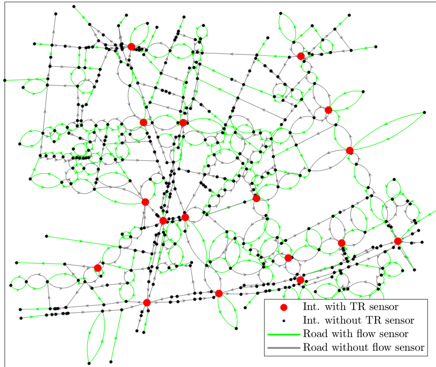
Figure 2.10: Particular configuration of sensors, using 17 TR sensors and 337 flow sensors.
