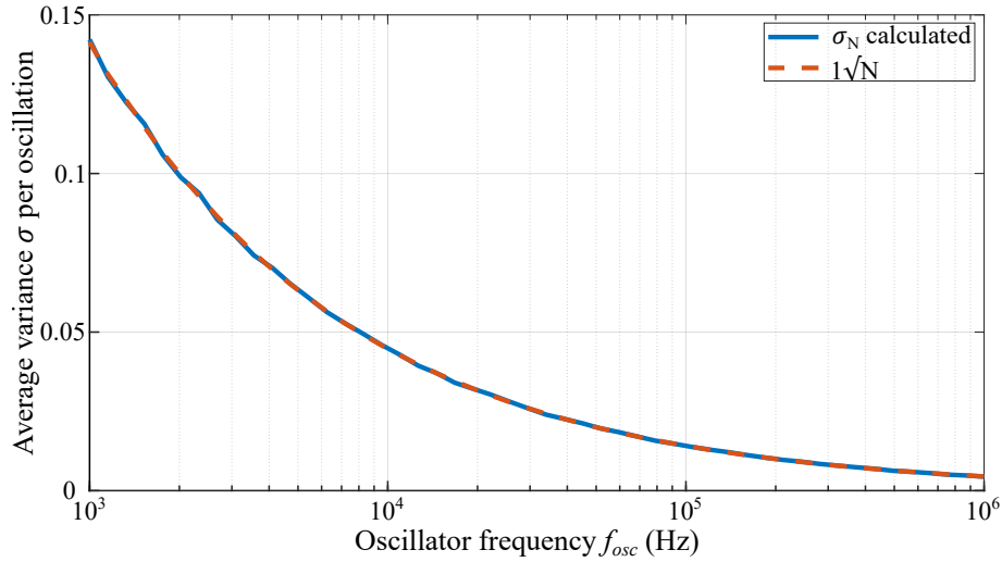
Figure 5.5: Accumulated random jitter as a function of frequency for a fix duration of 50 ms
