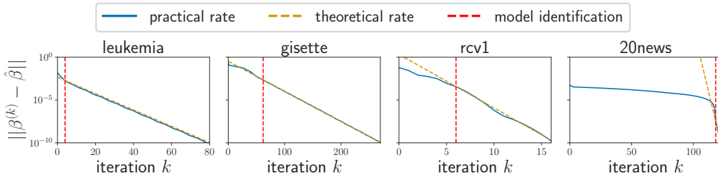
Figure 2.3 – Support vector machine, linear convergence. Distance to optimum, \|\beta^{(k)} - \hat{\beta}\| , as a function of the number of iterations k , on 4 different datasets: leukemia , gisette , rcv1 and 20news .
