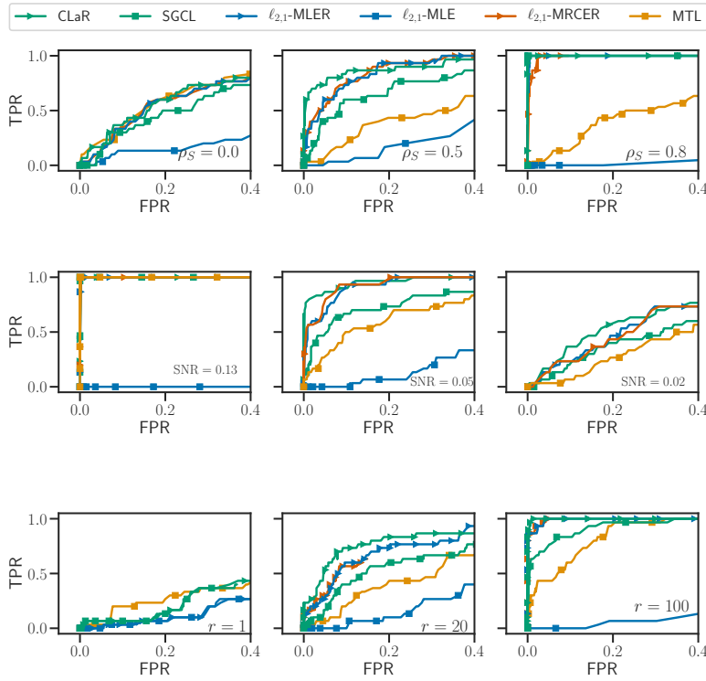
Figure 5.1 – Influence of noise structure. ROC curves of support recovery ( \rho_X = 0.6 , \text{SNR} = 0.03 , r = 20 ) for different \rho_S values.
