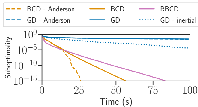
Figure 3.11 – Group Lasso, suboptimality. Suboptimality as a function of time for the group Lasso on the Leukemia dataset, \lambda = \lambda_{\max}/100 . Groups are artificially taken as consecutive blocks of 5 features.
