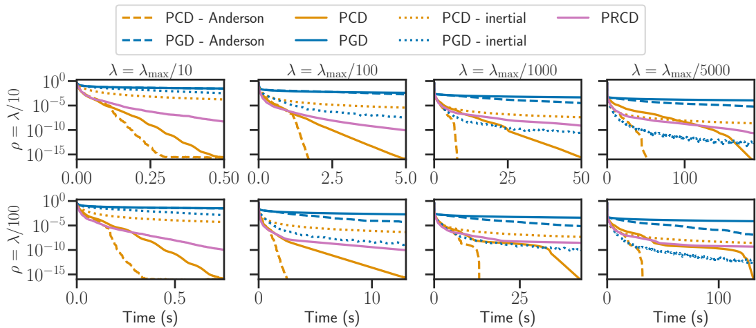
Figure 3.9 – Enet, suboptimality. Suboptimality as a function of time for the elastic net on Leukemia dataset, for multiple values of \lambda and \rho .
