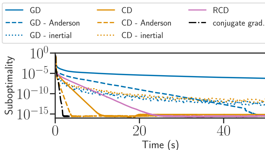
Figure 3.1 – Suboptimality along time for a quadratic problem on the 5000 first features of the rcv1 dataset. GD: gradient descent, CD: cyclic coordinate descent, RCD: randomized coordinate descent.
