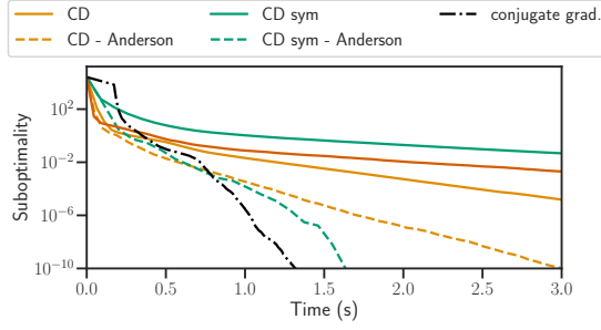
Figure 3.4 – OLS, rcv1 . Suboptimality as a function of time on the 5000 first columns of the dataset rcv1 .
