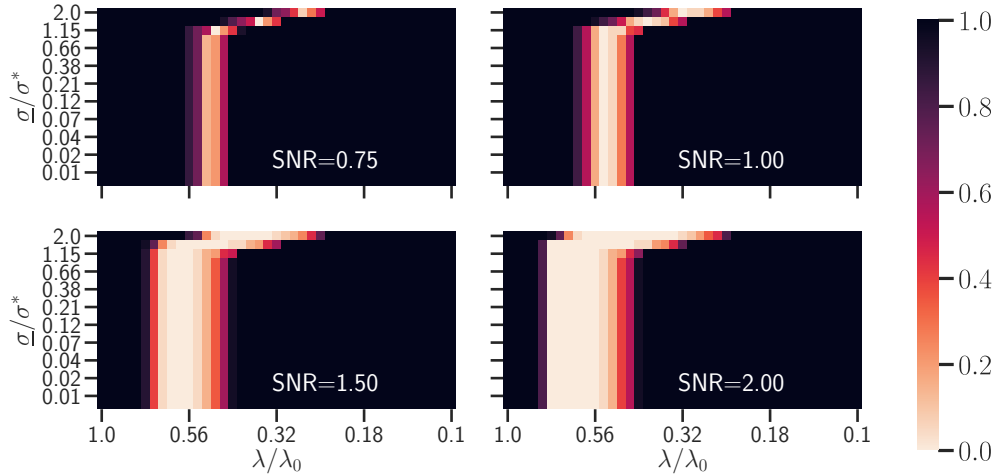
Figure 4.3 – (Synthetic data, n = 50 , p = 1000 , T = 20 ) Hard recovery loss for different values of SNR for the multitask SCL.
