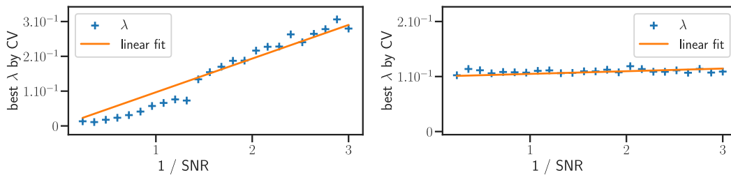
Figure 4.1 – Lasso (left) and square-root Lasso (right) optimal regularization parameters \lambda determined by cross validation on prediction error (blue), as a function of the noise level on simulated values of y . As indicated by theory, the Lasso’s optimal \lambda grows linearly with the noise level, while it remains constant for the square-root Lasso.
