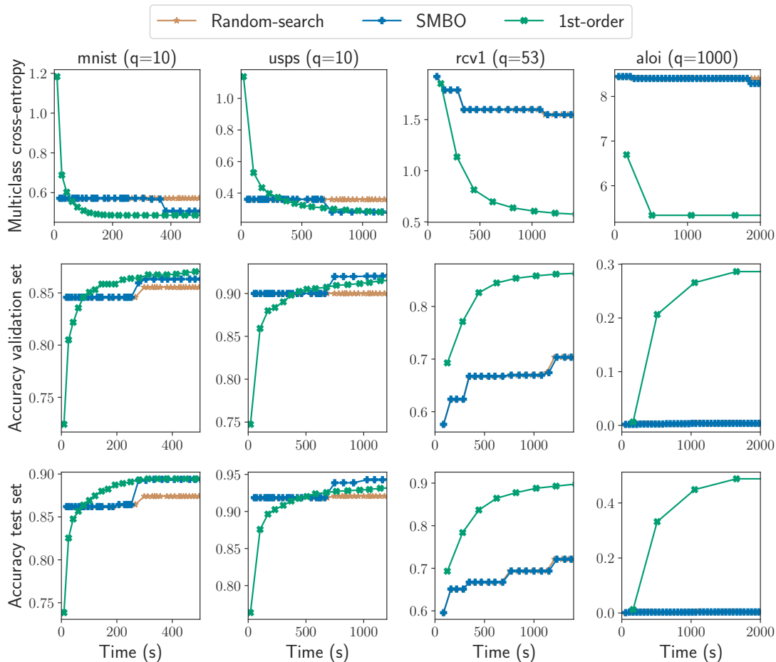
Figure 6.6 – Multiclass sparse logistic regression hold-out, time comparison (# classes hyperparameters). Multiclass cross-entropy (top), accuracy on the validation set (middle), and accuracy on the test set (bottom) as a function of time on mnist , usps ( q = 10 classes), rcv1 ( q = 53 classes), aloi ( q = 1000 classes).
