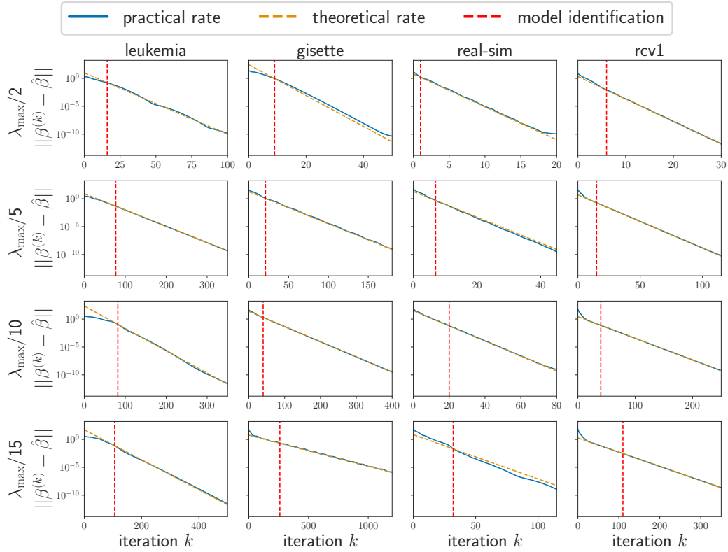
Figure 2.1 – Lasso, linear convergence. Distance to optimum, \|\beta^{(k)} - \hat{\beta}\| , as a function of the number of iterations k , on 4 different datasets: leukemia , gisette , rcv1 , and real-sim .
