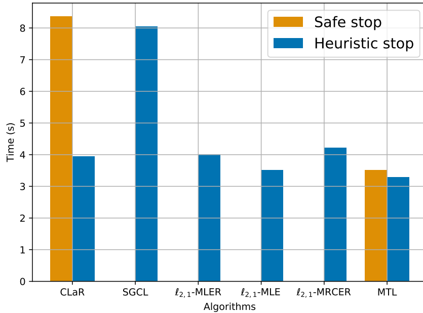
Figure 5.14 – Time comparison, real data, n = 102 , p = 7498 , T = 54 , r = 56 Time for each algorithm to produce Figure 5.6.
