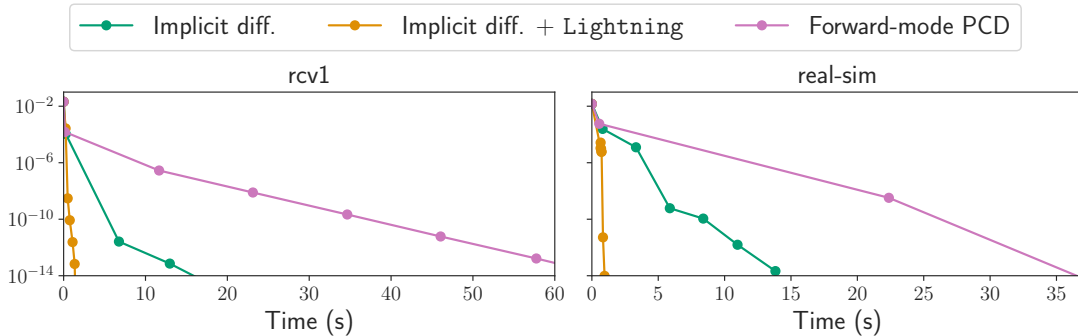
Figure 6.3 – SVM with hold-out criterion: absolute difference between the exact hypergradient (using \hat{\beta} ) and the iterate hypergradient (using \beta^{(k)} ) of the SVM as a function of time. “Implicit diff. + Lightning” uses Lightning (Blondel and Pedregosa, 2016), instead of our proximal coordinate descent implementation.
