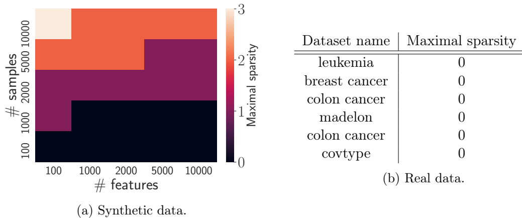
Figure 1.5 – Maximal sparsity that can theoretically be recovered assuming mutual incoherence in Equation (1.7) is displayed for multiple values of number of samples and number of features (left), and for multiple real-life datasets (right). For the synthetic data, entries of the design matrix X are drawn i.i.d. following a Gaussian distribution of mean 0 and variance 1. Real datasets are taken from libsvm (Chang and Lin, 2011) 2 .
