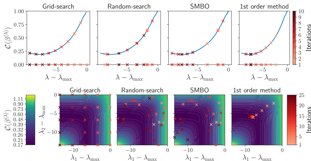
Figure 6.1 – 5-fold cross-validation error \mathcal{C}(\beta^{(\lambda)}) : (top) Lasso CV error with respect to \lambda for multiple hyperparameter optimization methods on the real-sim dataset, and (bottom) elastic net CV error with respect to \lambda_1 and \lambda_2 on the rcv1 dataset. Crosses represent the 10 (top) or 25 (bottom) first error evaluations for each method.
