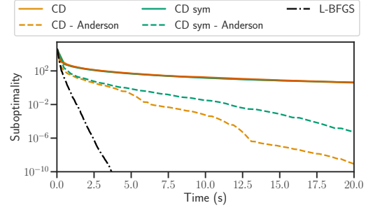
Figure 3.5 – \ell_2 -regularized logistic regression, real-sim . Suboptimality as a function of time on the 2000 first features of the real-sim dataset, Tikhonov strength set so that \kappa = 10^5 .
