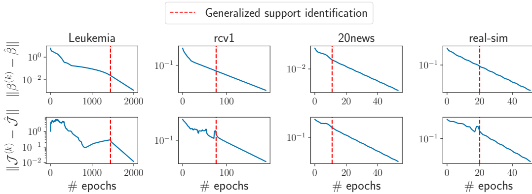
Figure 6.3 – Local linear convergence of the Jacobian for the Lasso. Distance to optimum for the coefficients \beta (top) and the Jacobian \mathcal{J} (bottom) of the forward-mode differentiation of proximal coordinate descent (Algorithm 6.3) on multiple datasets.
