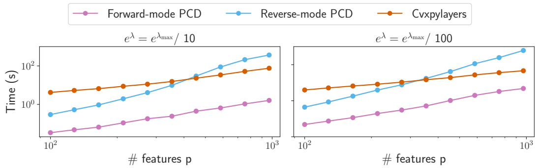
Figure 6.1 – Lasso with hold-out criterion: time comparison on the gina dataset to compute a single hypergradient as a function of the number of features, for two values of \lambda , e^\lambda = e^{\lambda_{\max}}/10 (left) and e^\lambda = e^{\lambda_{\max}}/100 (right).
