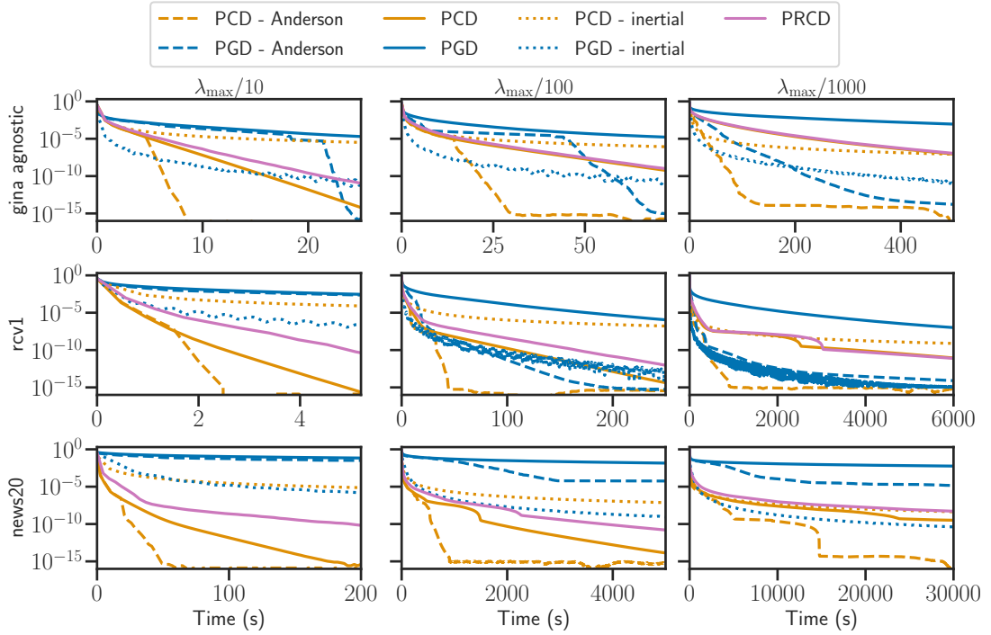
Figure 3.10 – \ell_1 -regularised logistic regression, suboptimality. Suboptimality as a function of time for \ell_1 -regularized logistic regression on multiple datasets and values of \lambda .
