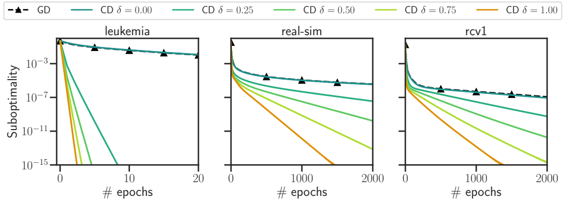
Figure 1.8 – Influence of stepsizes for cyclic coordinate descent, OLS. Suboptimality f(\beta^{(k)}) - f(\hat{\beta}) as a function of the number of epochs to solve a least squares problem on multiple datasets from libsvm : leukemia , real-sim and rcv1 . Gradient descent is compared against coordinate descent with step sizes \gamma_j = \delta/L_j + (1 - \delta)/L , for multiple values of \delta .
