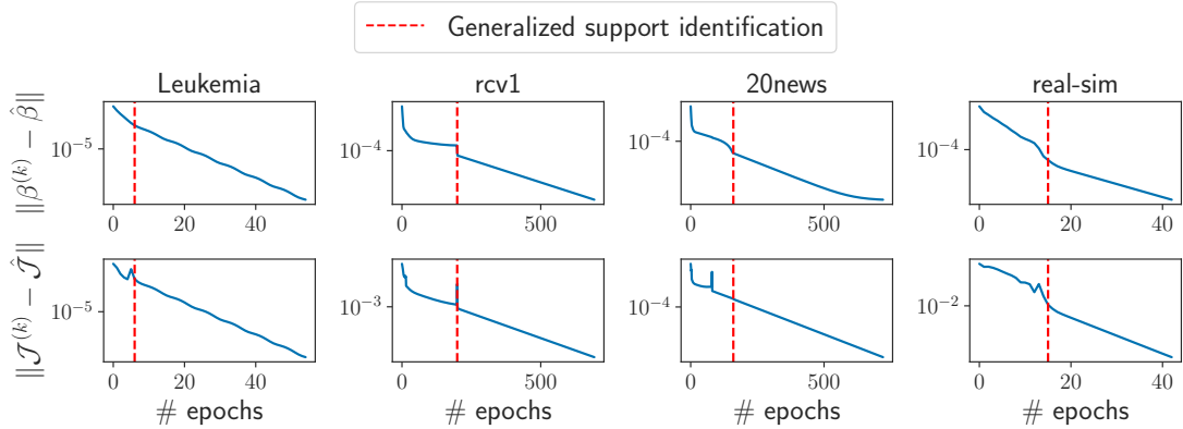
Figure 6.2 – Local linear convergence of the Jacobian for the SVM. Distance to optimum for the coefficients \beta (top) and the Jacobian \mathcal{J} (bottom) of the forward-mode differentiation of proximal coordinate descent (Algorithm 6.3) on multiple datasets. One epoch corresponds to one pass over the data, i.e. , one iteration with proximal gradient descent.
