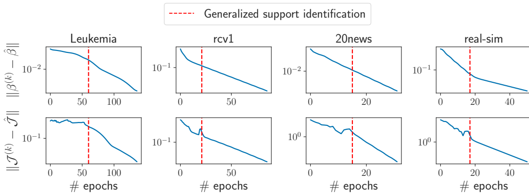
Figure 6.4 – Local linear convergence of the Jacobian for sparse logistic regression. Distance to optimum for the coefficients \beta (top) and the Jacobian \mathcal{J} (bottom) of the forward-mode differentiation of proximal coordinate descent (Algorithm 6.3) on multiple datasets.
