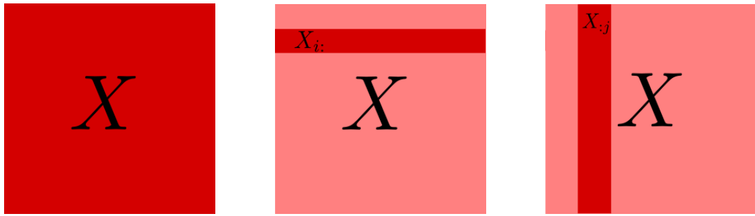
Figure 1.7 – Matrix storage. For coordinate descent (right), one needs to access efficiently successively each column X_{:j} of X \in \mathbb{R}^{n \times p} . On the opposite, when applying Kaczmarz or SGD (middle), one needs to access efficient each line X_{i:} of X .
