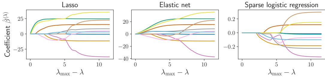
Figure 6.1 – Regularization paths (coefficient values as a function of \lambda ), on the diabetes and breast cancer datasets for the Lasso, the elastic net and sparse logistic regression. This illustrates the weak differentiability of the paths. We used diabetes for the Lasso and the elastic net, and the 10 first features of breast cancer for the sparse logistic regression.
