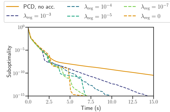
Figure 3.7 – Influence of \lambda_{\text{reg}} , sparse logistic regression, rcv1 . Influence of the regularization amount when solving a sparse logistic regression using Anderson extrapolation with proximal coordinate descent (PCD) on the rcv1 dataset, K = 5 , \lambda = \lambda_{\text{max}}/30 .
