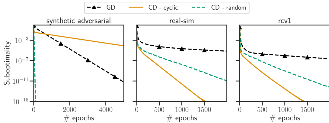
Figure 1.9 – Cyclic against random coordinate descent. Suboptimality as a function of the number of epochs to solve a least squares problems. Gradient descent is compared against random and cyclic coordinate descent.
