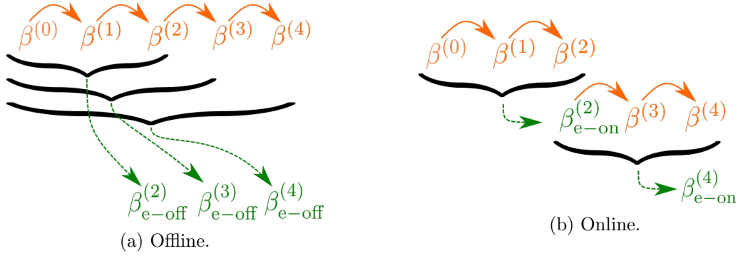
Figure 3.2 – Illustrations of offline (left) and online (right) Anderson extrapolation.
