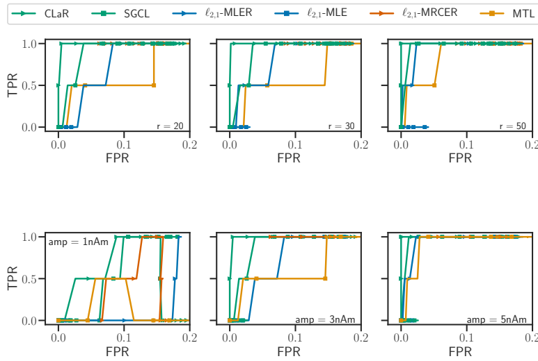
Figure 5.4 – Influence of the number of repetitions. ROC curves with empirical X and S and simulated B^* ( \text{amp} = 2\text{ nA.m} ), for different number of repetitions.
