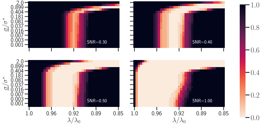
Figure 4.5 – (Synthetic data, n = 150 , p = 500 , T = 100 ) Hard recovery loss for different values of SNR for the SGCL.
