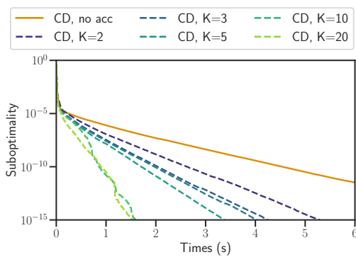
Figure 3.6 – Influence of K , quadratic, rcv1 . Influence of the number of iterates K used to perform Anderson extrapolation with coordinate descent (CD) on a quadratic with the rcv1 dataset (2000 first columns).
