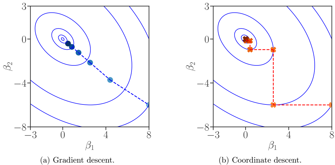
Figure 1.6 – Five iterations of gradient descent (left in blue) and cyclic coordinate descent (right in red) to minimize the quadratic function f(\beta_1, \beta_2) = 7\beta_1^2 + 6\beta_1\beta_2 + 8\beta_2^2 . Contour lines of the function f are in blue. Each algorithm starts at point (8, -6) and converges toward the minimizer (0, 0) . The darker the point, the larger the iteration number. From a computational point of view, two updates of coordinate descent are equivalent to one update of gradient descent (see Algorithm 1.4 ).
