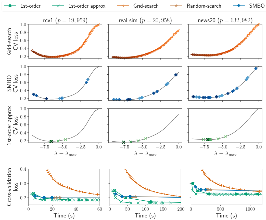
Figure 6.4 – Lasso with cross-validation criterion: cross-validation loss as a function of \lambda (black line, top) and as a function of time (bottom). Lighter markers correspond to earlier iterations of the algorithm.
