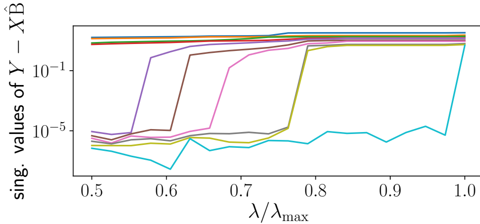
Figure 4.2 – Singular values of the residuals Y - X\hat{B} of the multivariate square-root Lasso ( n = 10, T = 20, p = 30 ), as a function of \lambda . The observation matrix Y is full rank, but the residuals are rank deficient even for high values of the regularization parameter, invalidating the classical assumptions needed for statistical analysis.
