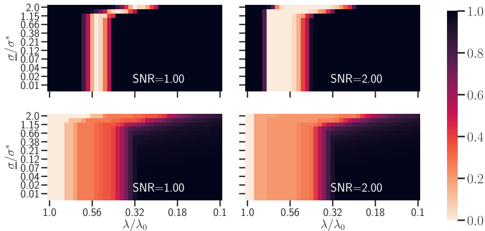
Figure 4.4 – (Synthetic data, n = 50 , p = 1000 , T = 20 ) Hard recovery loss (top) and percent of non-zeros coefficients (bottom) for different values of SNR: SNR = 1 (left), SNR = 2 (right) for the multitask SCL.
