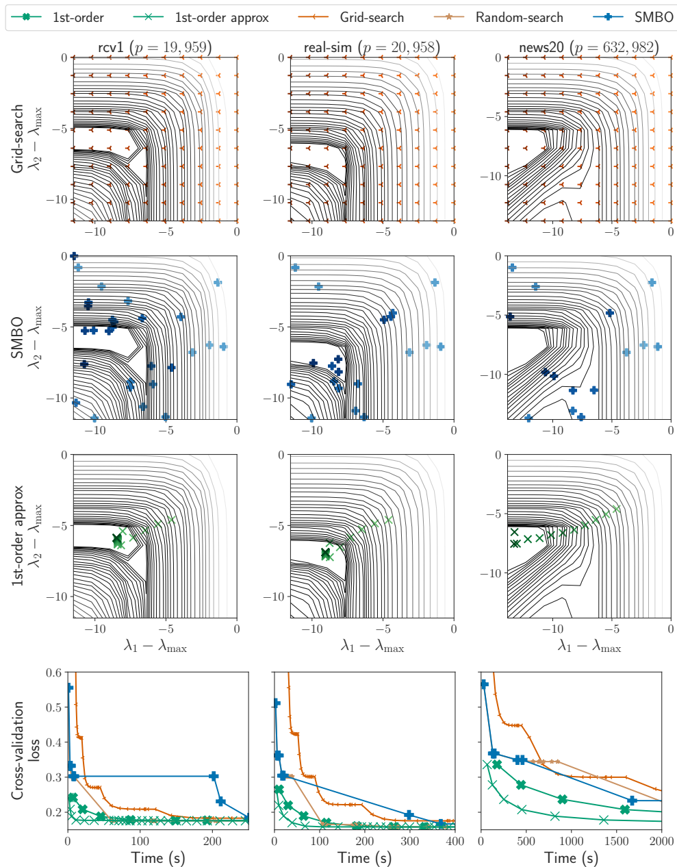
Figure 6.5 – Elastic net cross-validation, time comparison (2 hyperparameters) . Level sets of the cross-validation loss (black lines, top) and cross-validation loss as a function of time (bottom) on rcv1 , real-sim and news20 datasets.
