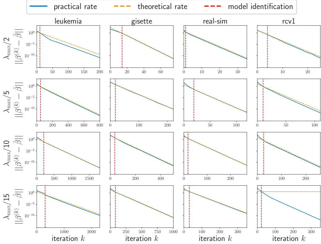
Figure 2.2 – Sparse logistic regression, linear convergence. Distance to optimum, \|\beta^{(k)} - \hat{\beta}\| , as a function of the number of iterations k , on 4 different datasets: leukemia , gisette , rcv1 , and real-sim .
