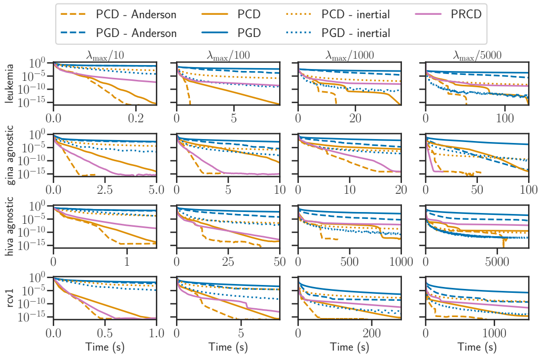
Figure 3.8 – Lasso, suboptimality. Suboptimality as a function of time for the Lasso on multiple datasets and values of \lambda .
