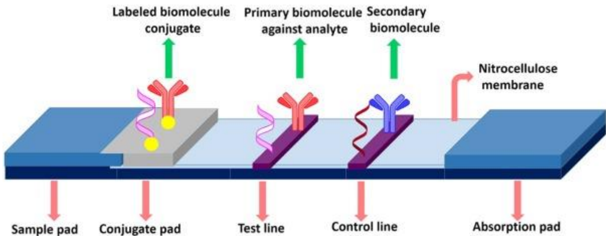
Figure 25: Lateral flow assay method [88].
