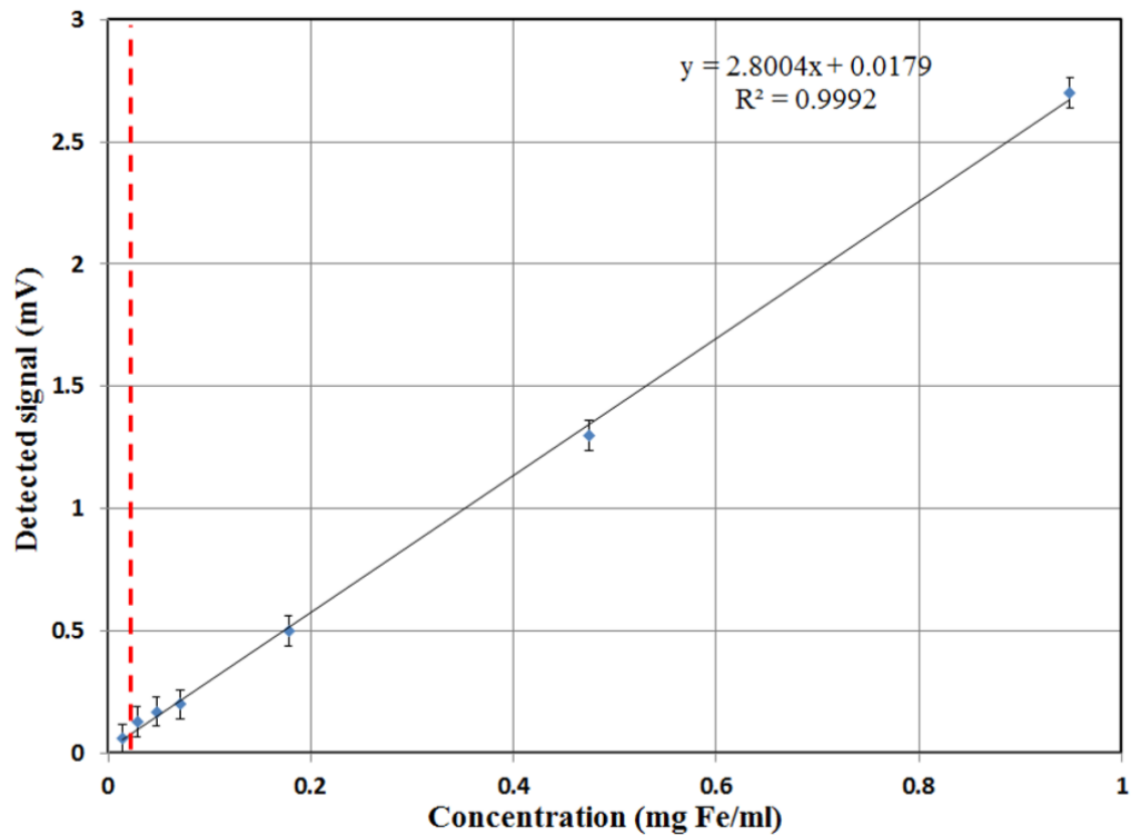
Figure 58: Magnetic response signal f_1+2f_2 as a function of the mass concentration of 20 nm iron oxide ( Fe_2O_3 ) nanoparticles. The red dotted line indicates the limit of detection at about 0.015 mg/mL or 15 mg/L for these measurements.
