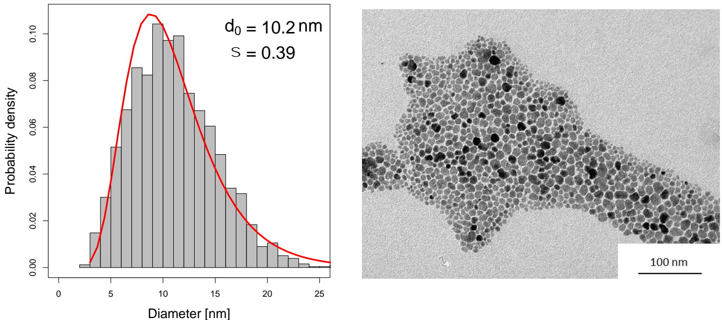
Figure 59: (Left) Particle size distribution (PSD) of the CoFe-20nm. The parameter d_0 is the mass-median-diameter of the SPN (average particle diameter by mass) and \sigma is the standard deviation. (Right) TEM image of CoFe-20nm nanoparticles.
