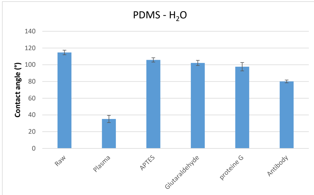
Figure 98: Water contact angle on pristine PDMS, after the plasma \text{O}_2 treatment, after APTES grafting, after the glutaraldehyde adding, the protein G and finally after putting the antibodies on top of the formed chemical chain.
