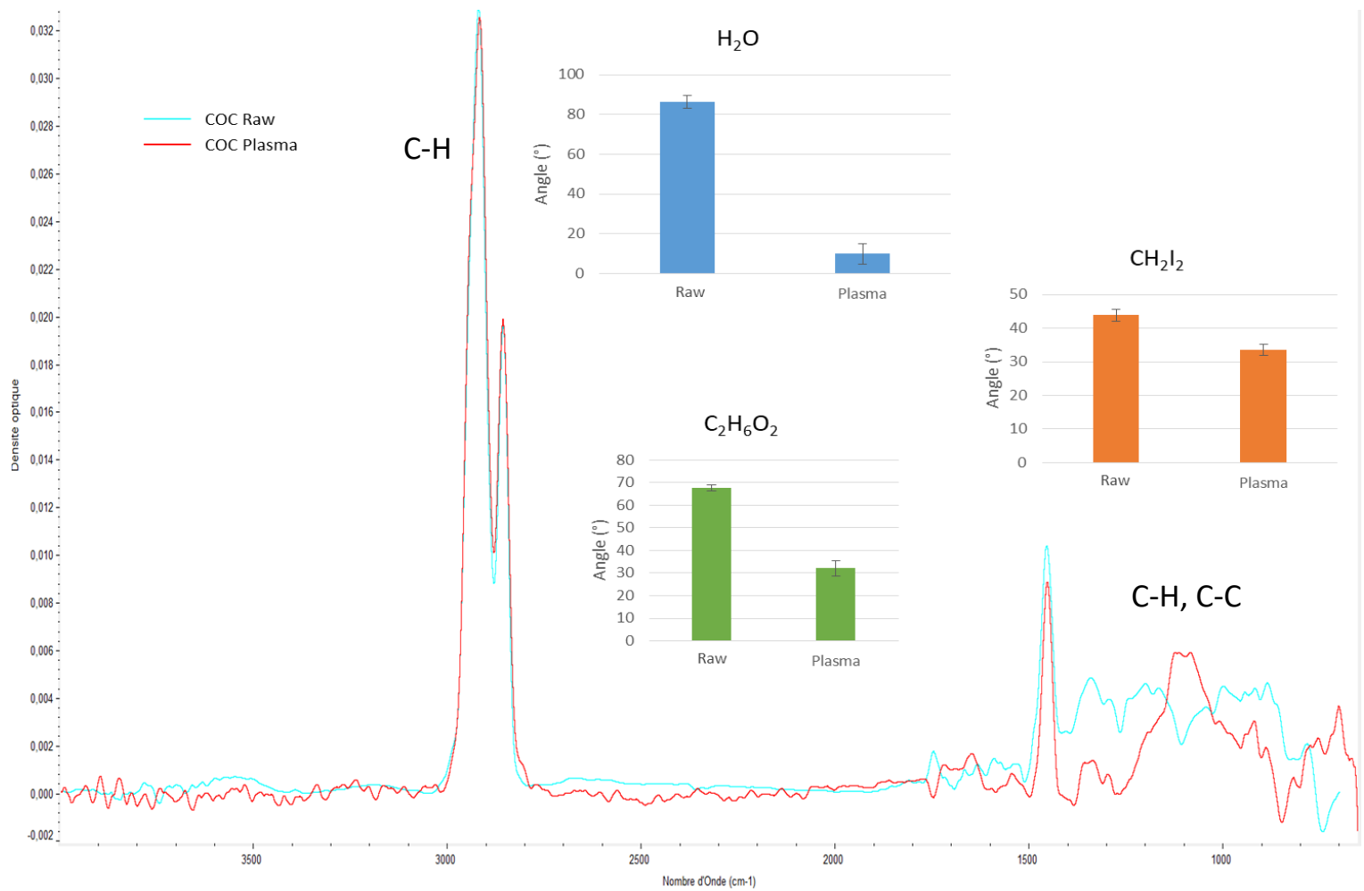
Figure 105: Comparison of infrared ATR-FTIR spectra and contact angles after and before the plasma treatment of COC surfaces.
