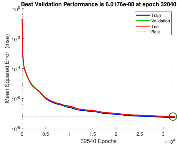
(a) 2L-FANN
