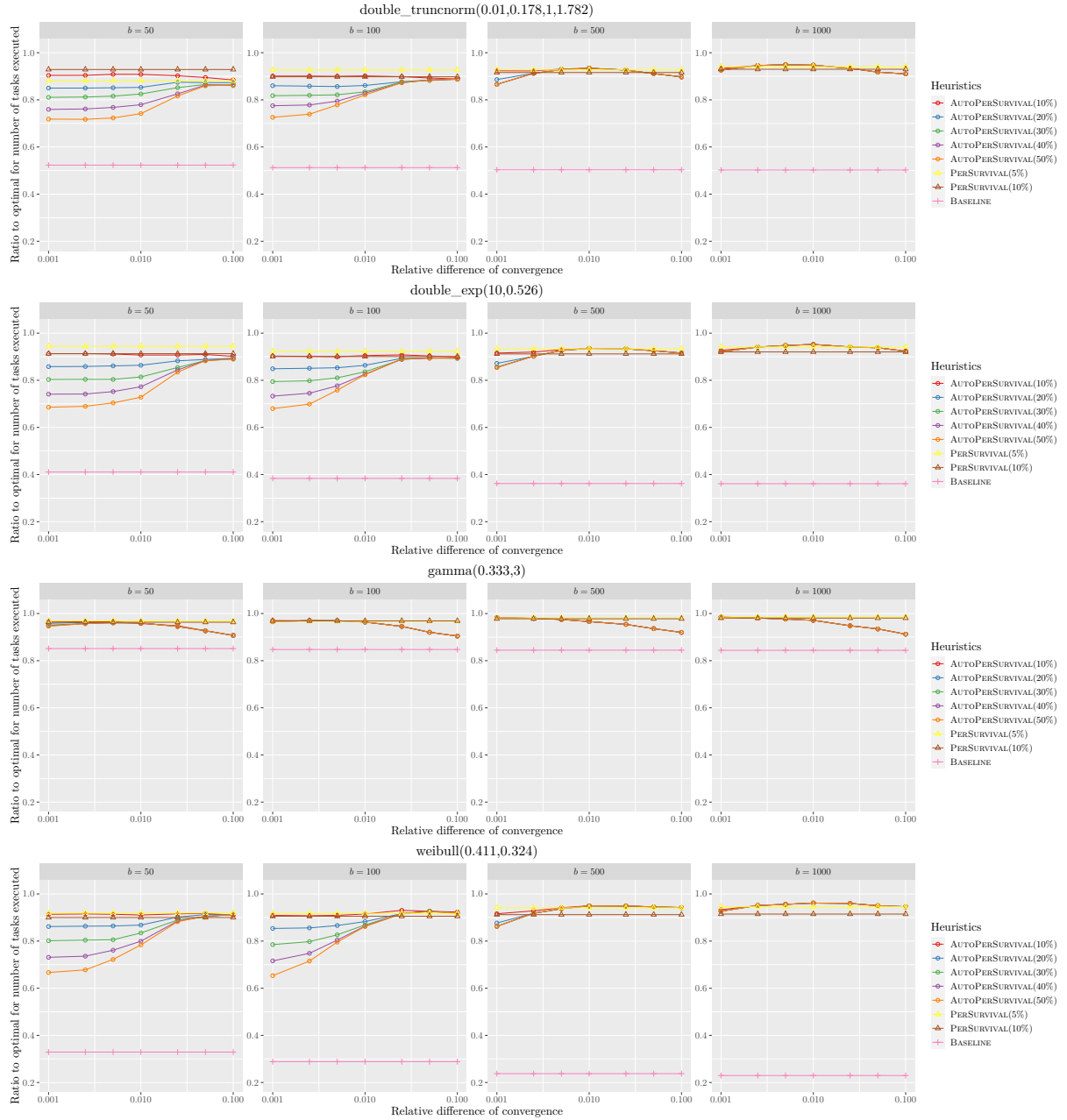
Figure 3.9: Number of successfully executed tasks for each distribution using AUTOBERSURVIVAL (different p_{max} when varying \epsilon ) and PERSURVIVAL (different p ) (3/3).
