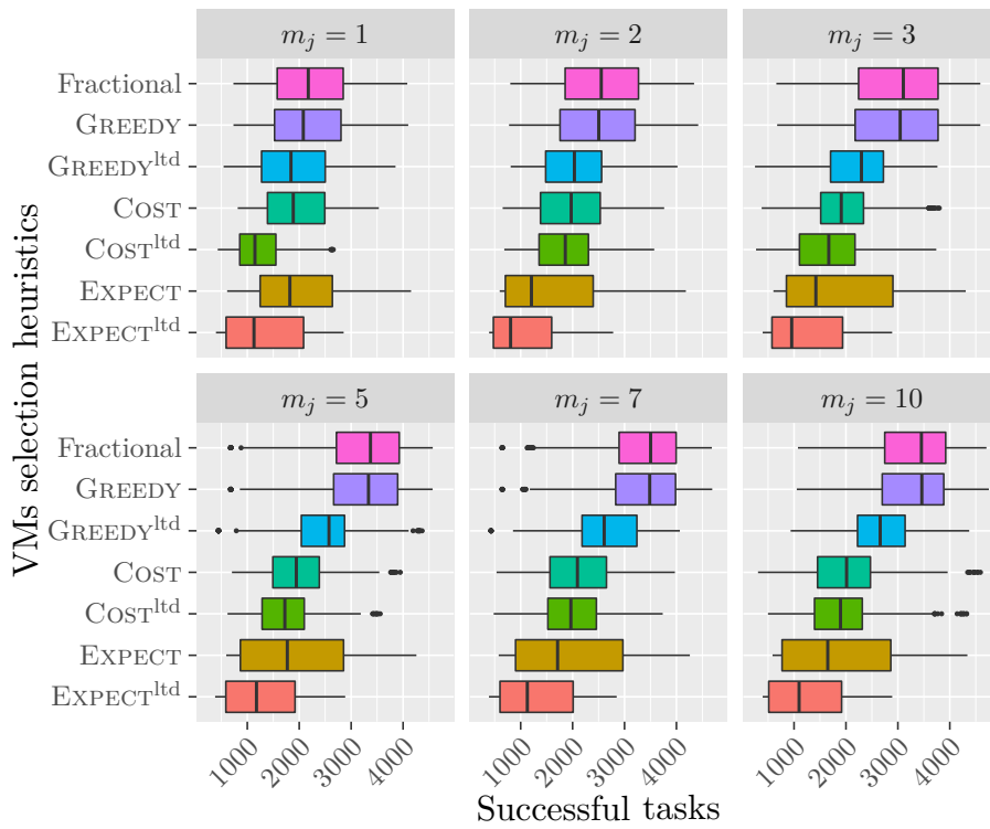
Figure 2.4: Number of successfully executed tasks of different methods to choose VMs when interrupting tasks with heuristic OPTRATIO. Each of the 100 platforms is generated with m_j = 1, 2, 3, 5, 7, 10 , M = 6, 12, 18, 30, 42, 60 , c_j = s_j and is used 10 times with b = 630 and d \approx 13.2 ( K \approx 47.8 ). Execution times follow lognormal distributions with x_{CV} = 3 .
