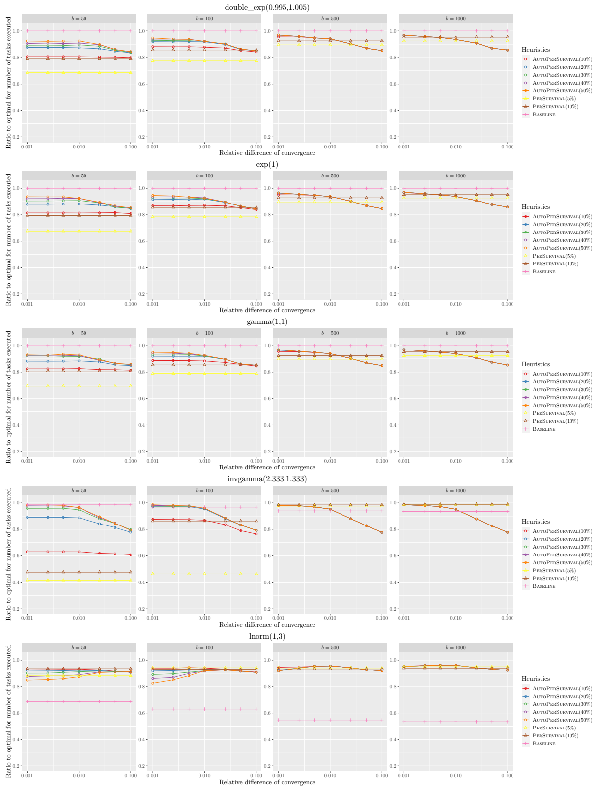
Figure 3.8: Number of successfully executed tasks for each distribution using AUTO PERSURVIVAL (different p_{max} when varying \epsilon ) and PERSURVIVAL (different p ) (2/3).
