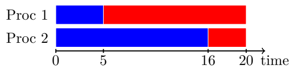
Figure 3.1: Toy example with two processors, two successfully completed tasks (in blue) and two not-yet-completed tasks (in red) at time 20.
