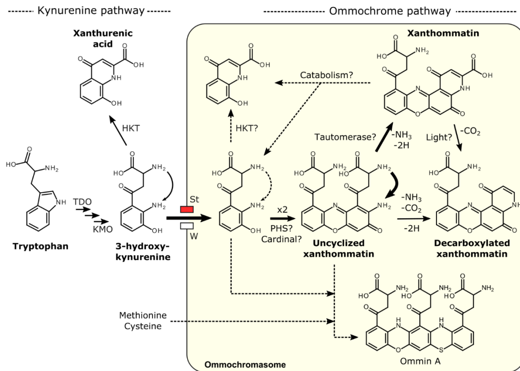
Figure 4-8. Proposed biosynthetic pathway of ommochromes through the formation of uncyclized xanthommatin in ommochromosomes.
