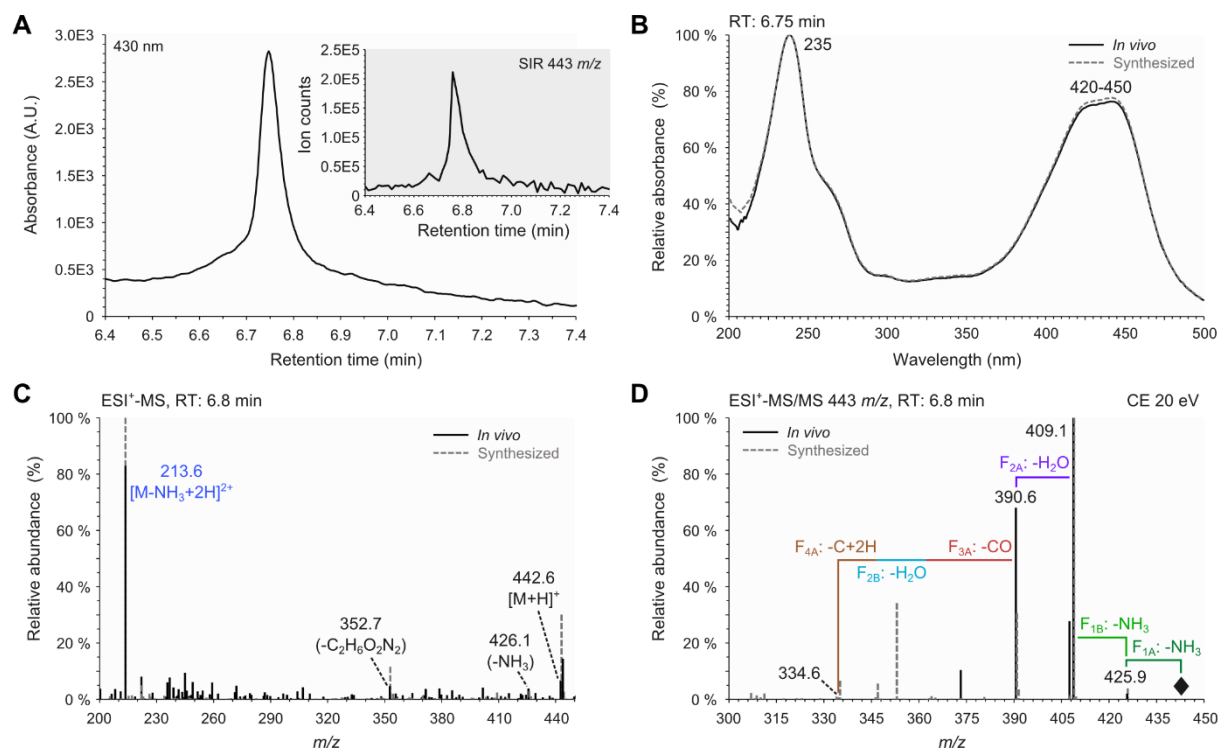
Figure S4-6. Analytical characterization of uncyclized xanthommatin in methanolic extracts of housefly eyes.
