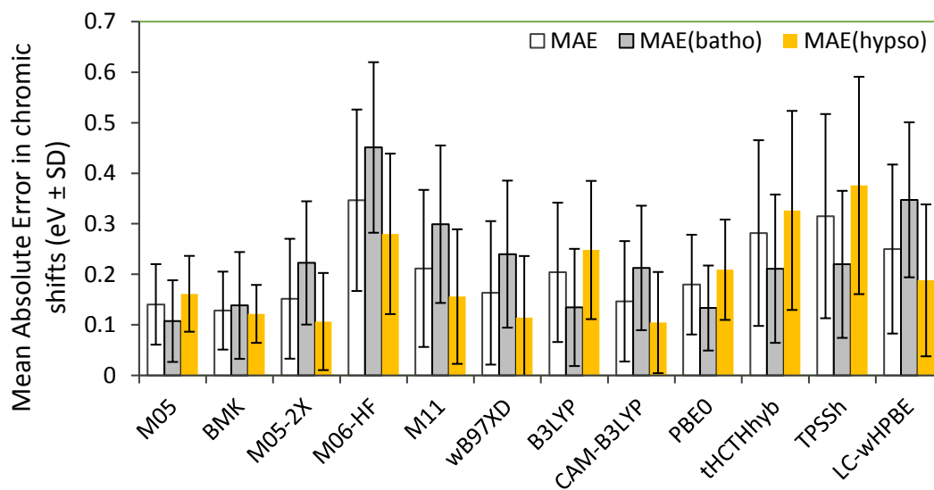
Figure S5-5. Mean absolute error (MAE) in computed vertical chromic shifts of phenoxazinones/phenoxazines pairs for a series of functionals.
