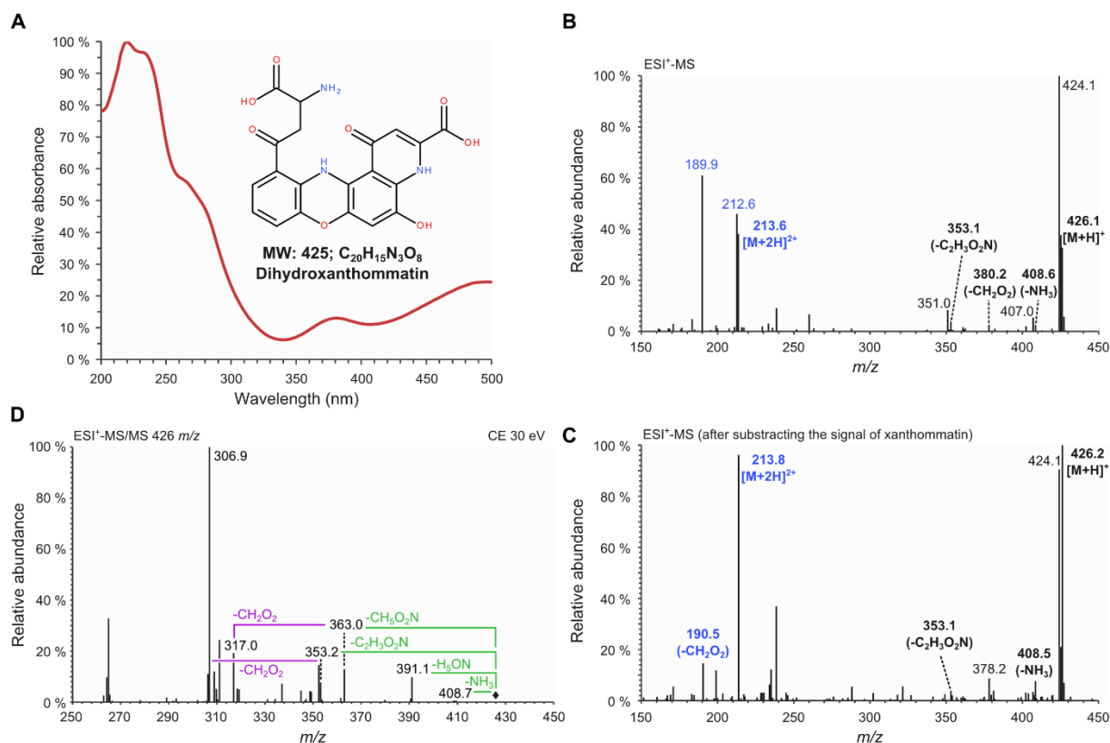
Figure S4-5. Analytical characterization of dihydroxanthommatin.
