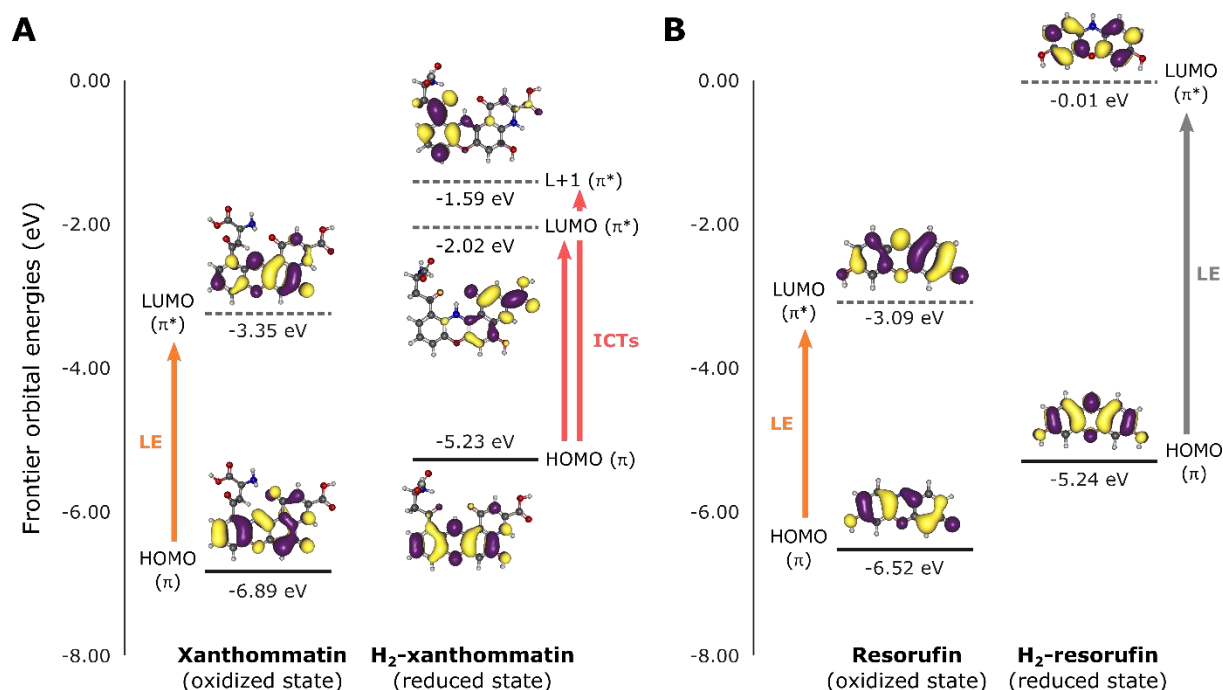
Figure 5-6. Orbital diagrams of the bathochromic ommochrome pair xanthommatin/dihydroxanthommatin and the hypsochromic pair resorufin/dihydroresorufin.
