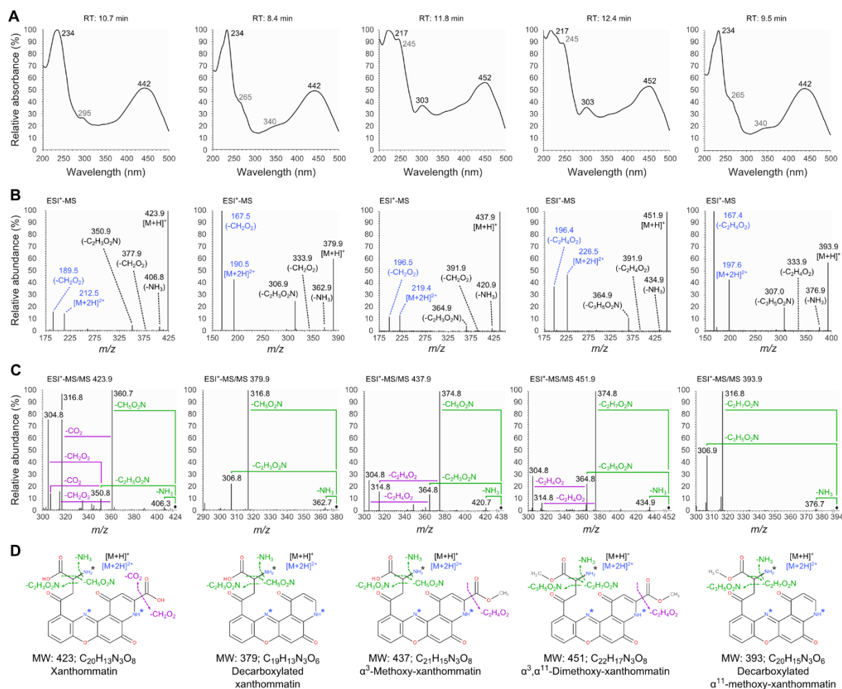
Figure 4-3. Absorbance- and mass spectrometry-assisted elucidation of the structure of the five major ommatins detected after incubation in acidified methanol.
