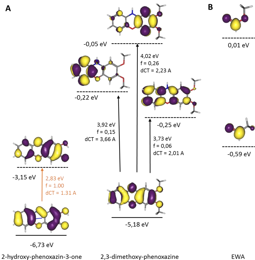
Figure S5-11. Molecular orbital diagrams of unsubstituted 2-hydro-phenoxazine-3-one, 2,3-dimethoxy-phenoxazine and of two electron-withdrawing auxochromes (EWA).
