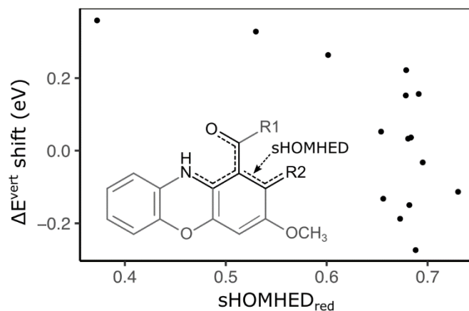
Figure S5-7. Comparison of computed chromic shifts ( \Delta E^{\text{vert}} shift) of phenoxazinone/phenoxazine pairs with the s\text{HOMHED} values of corresponding reduced phenoxazines (red).
