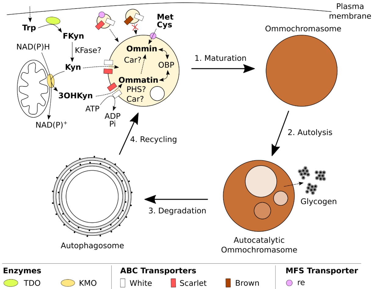
Figure 3-6. Putative model for the formation and recycling of ommochromosomes and ommochromes.
