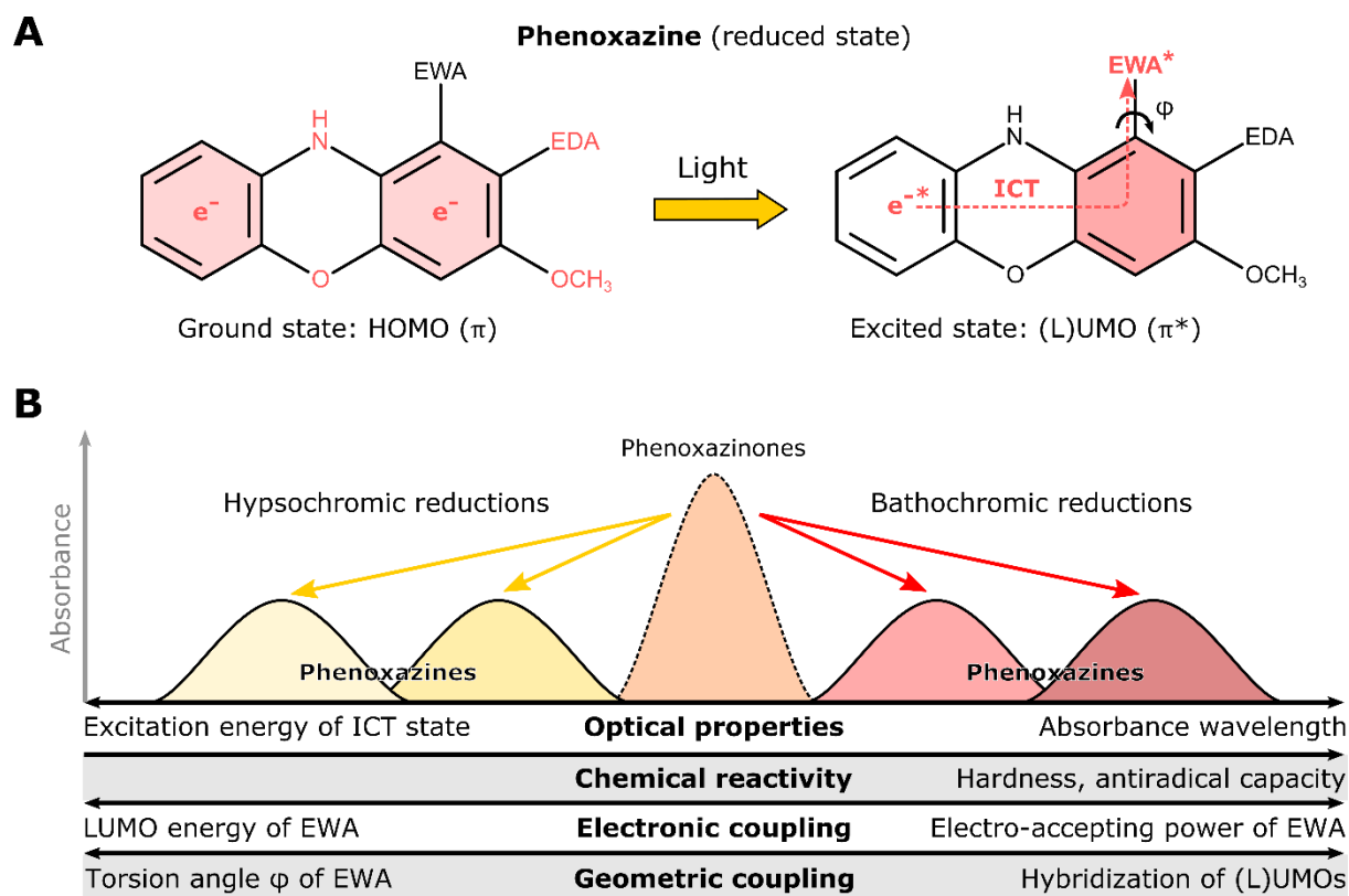
Figure 5-7. Model of the effect of geometric and electronic couplings on chromic shifts and chemical behaviors of phenoxazinone/phenoxazine pairs upon reduction.
