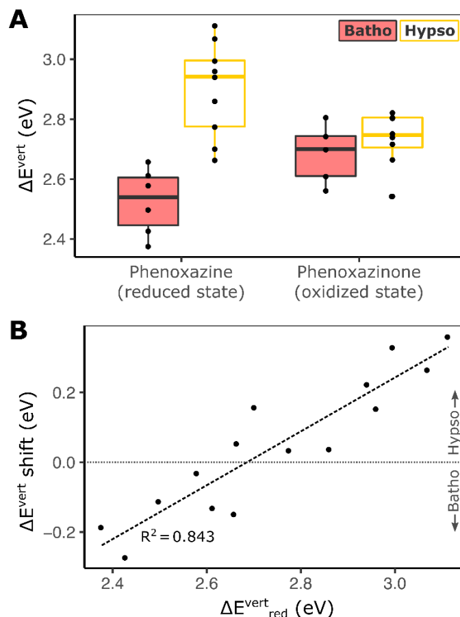
Figure 5-3. Relationship between computed vertical excitation energies ( \Delta E^{vert} ) chromic shifts of phenoxazinone/phenoxazine pairs.
