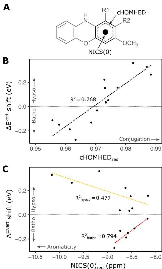
Figure 5-2. Computed vertical chromic shifts ( \Delta E^{\text{vert}} shift) of phenoxazinone/phenoxazine pairs as a function of two aromaticity indexes (A), cHOMHED (B) and NICS(0) (C), of phenoxazines.
