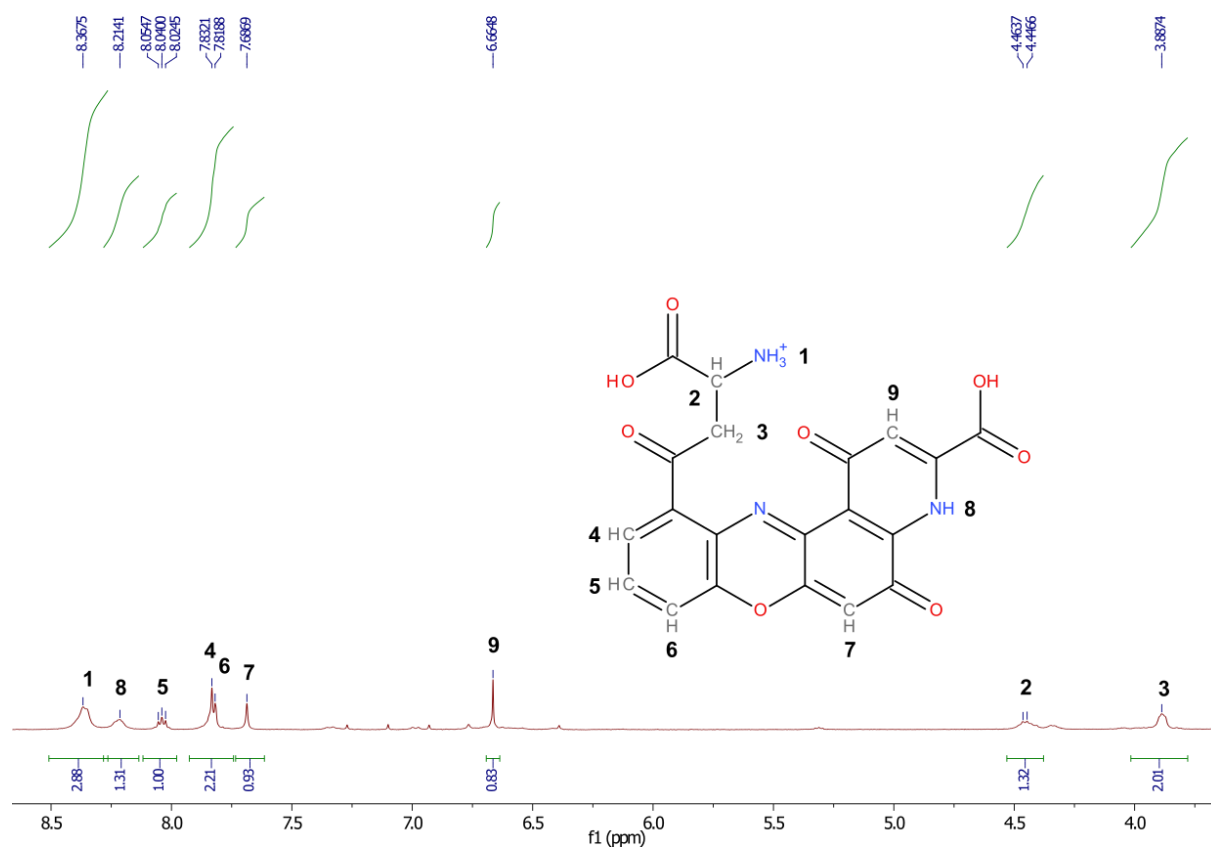
Figure S4-1. 1 H-NMR spectrum of synthesized xanthommatin in acidic DMSO.
