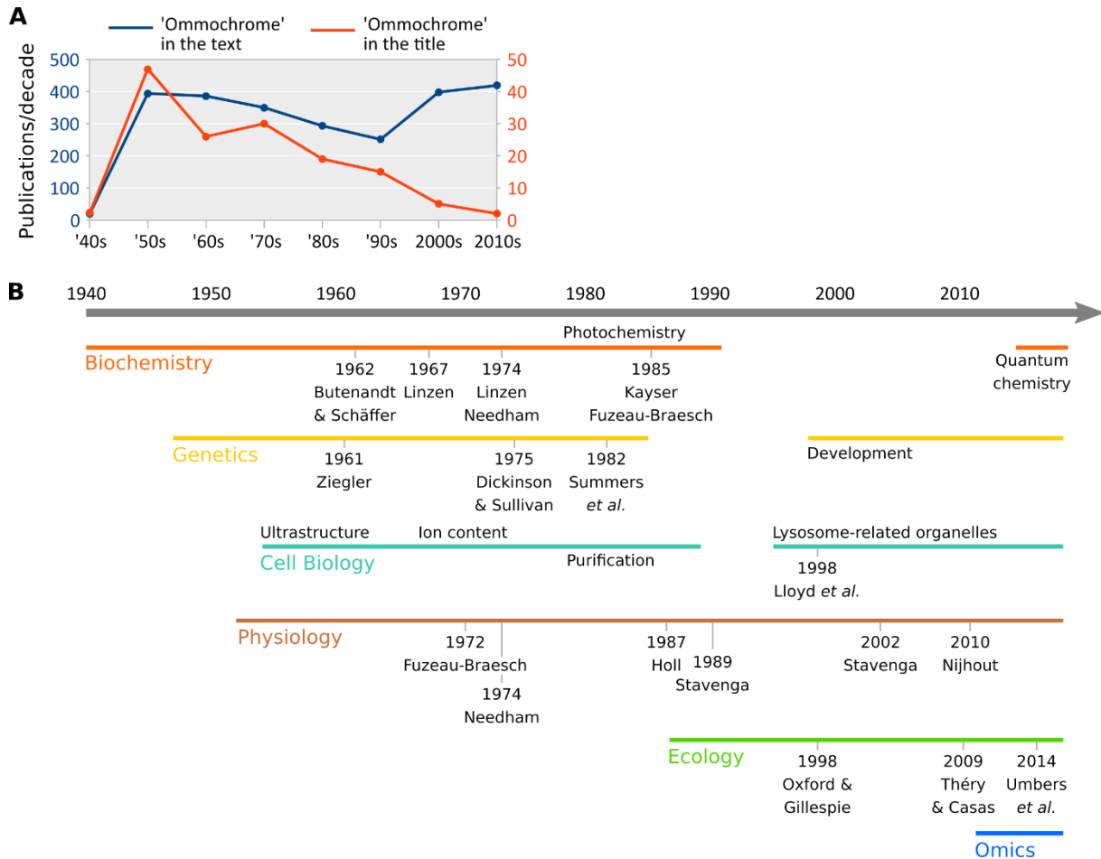
Figure 3-2. History of ommochrome study.
