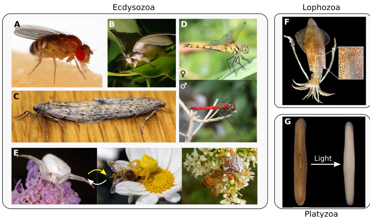
Figure 3-1. Examples of protostomes that produce ommochromes.
