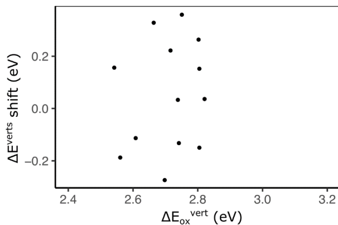
Figure S5-8. Comparison of computed chromic shifts ( \Delta E^{\text{vert}} shift) of phenoxazinone/phenoxazine pairs with the vertical excitation energies of corresponding oxidized phenoxazinones ( \Delta E_{\text{ox}}^{\text{vert}} ).
