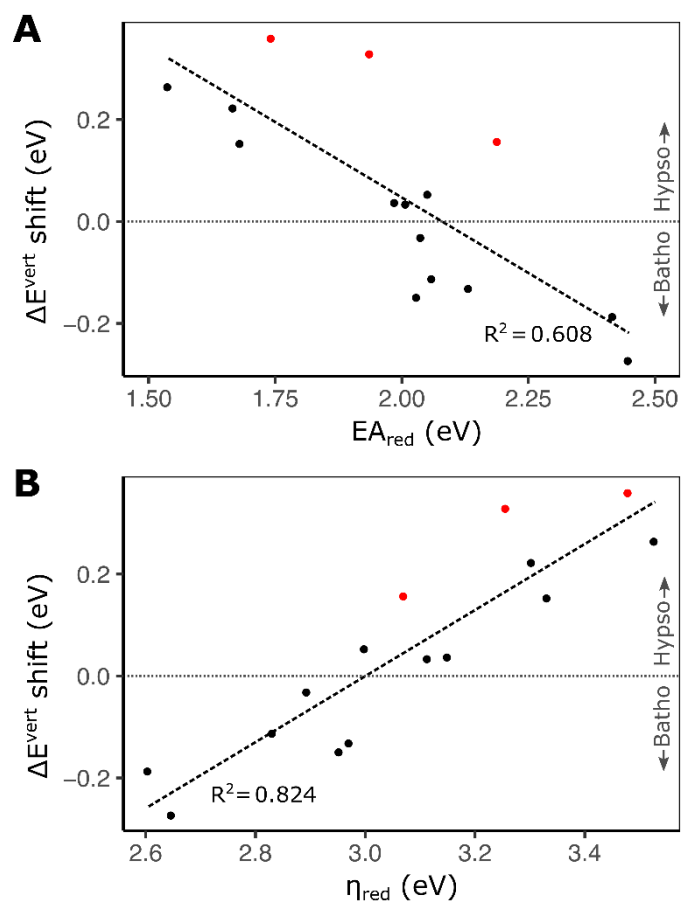
Figure 5-4. Comparison of chromic shifts ( \Delta E^{\text{vert}} \text{ shift} ) of phenoxazinone/phenoxazine pairs with electron affinity (EA, A) and chemical hardness ( \eta , B) of phenoxazines.
