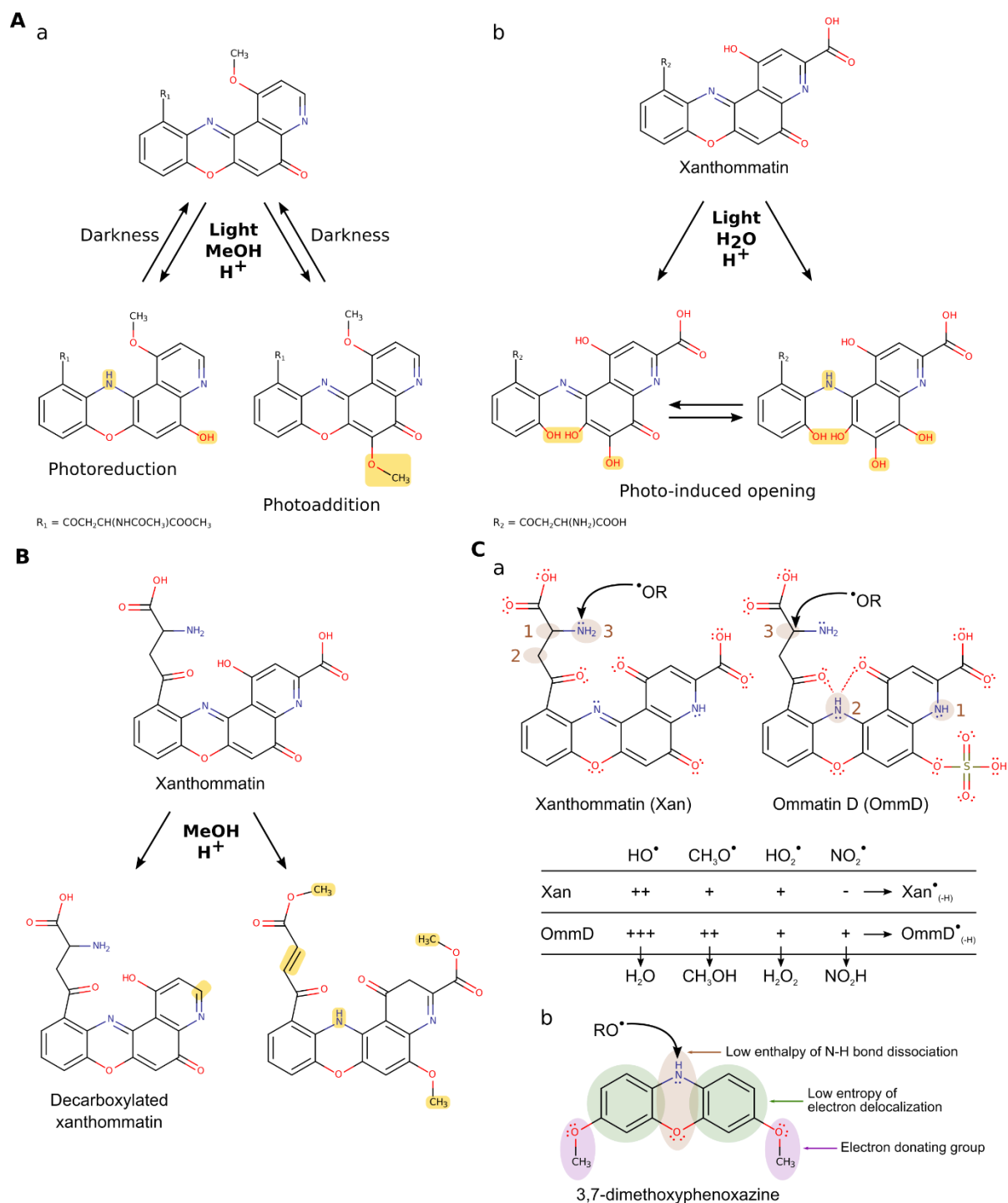
Figure 3-4. The reactivity of ommochromes and related compounds.
