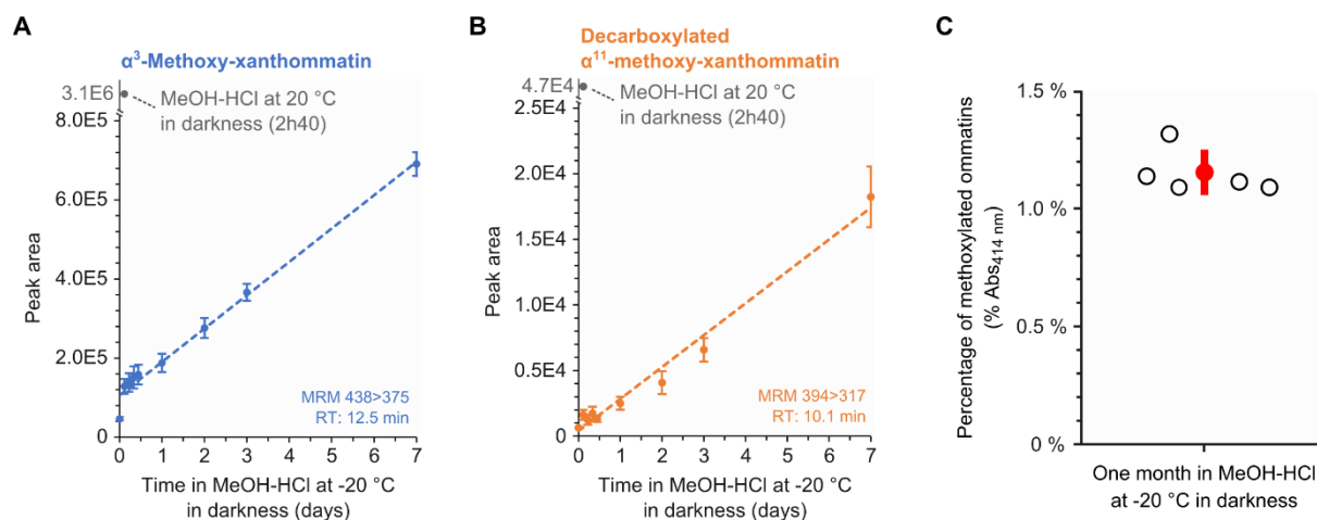
Figure S4-4. Slow methoxylations of synthesized ommatins in acidified methanol at -20 °C in darkness.
