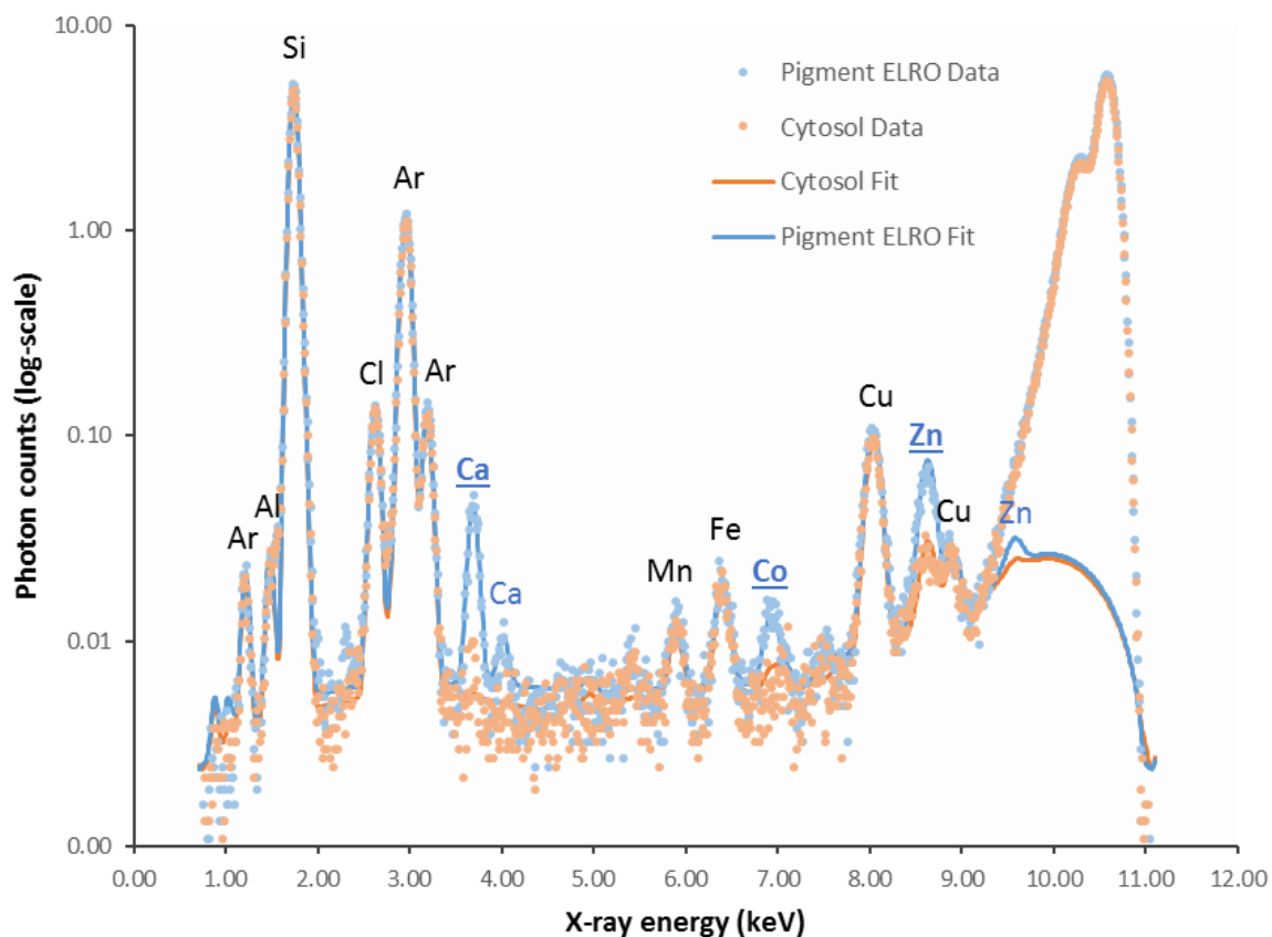
Figure S6-3. Recorded Synchrotron X-ray spectra of two intracellular regions within the same cell.
