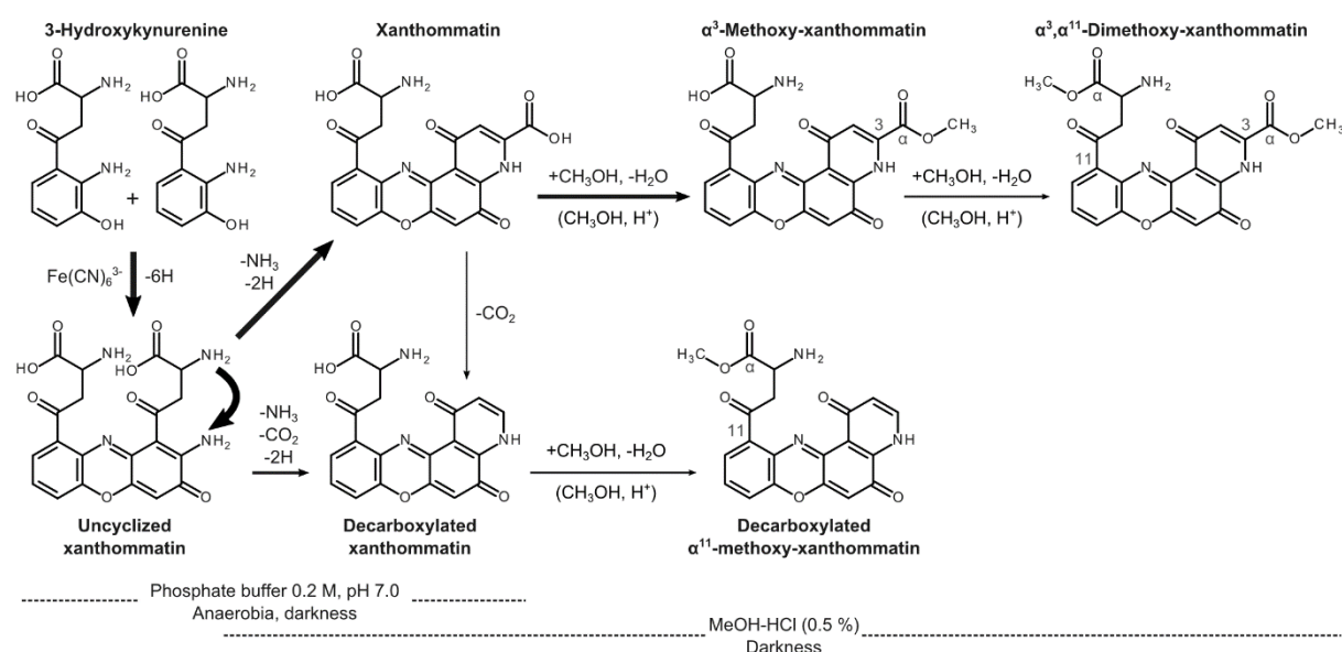
Figure 4-7. In vitro formation and alteration of ommatins.
