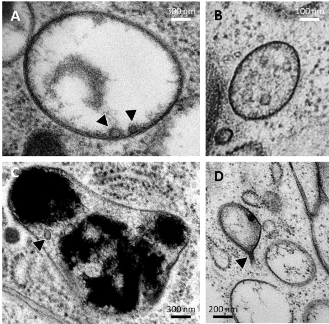
Figure S6-2. Intraluminal vesicles and membrane tubulations of pigment organelles.
