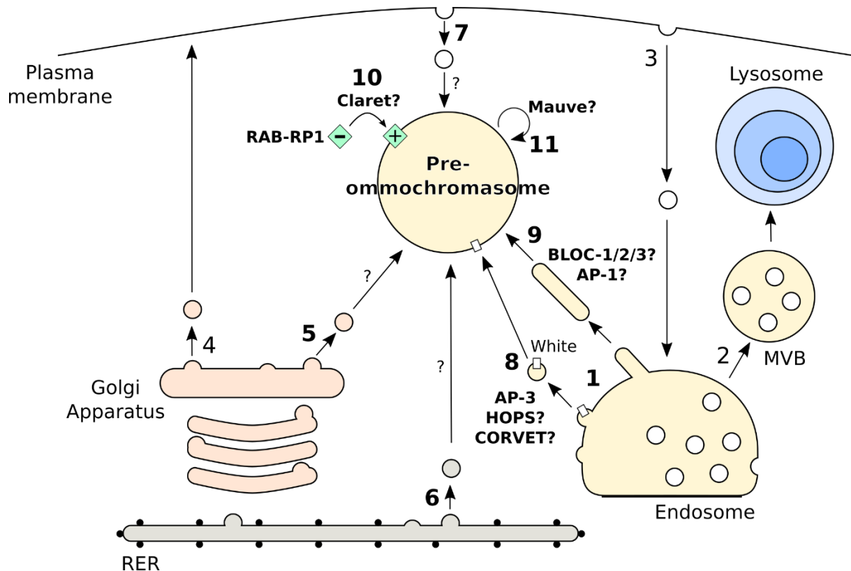
Figure 3-5. Putative scheme of ommochromasome biogenesis.
