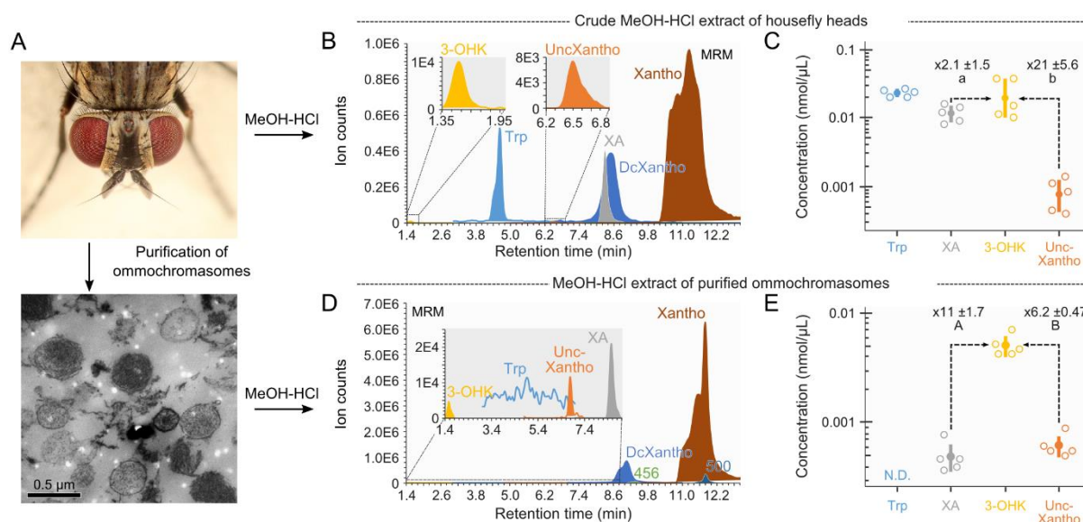
Figure 4-6. Biological localization of uncyclized xanthommatin and tryptophan→ommochrome metabolites from housefly eyes.
