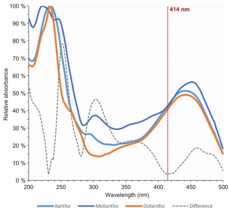
Figure S4-3. Determination of the wavelength at which ommatins absorb light equivalently.
