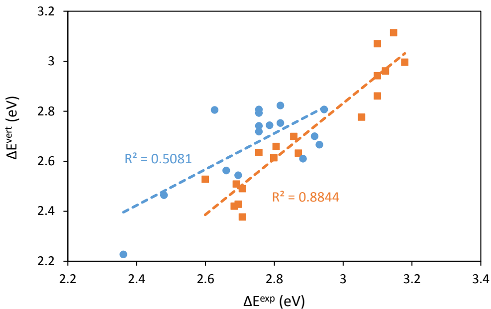
Figure S5-4. Comparison of M05-computed vertical excitation energies ( \Delta E^{\text{vert}} ) with experimental maximum excitation energies ( \Delta E^{\text{exp}} ).
