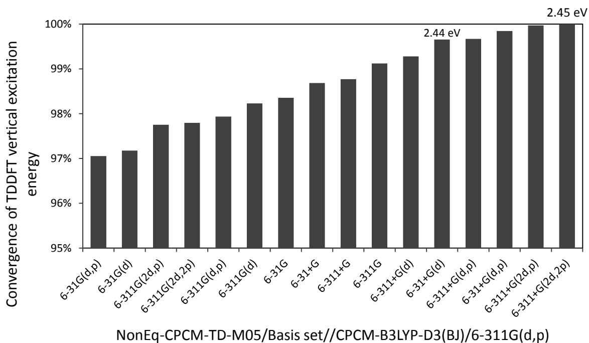
Figure S5-2. Basis-set dependence of the first vertical excitation energy computed for the 2-amino-7-methoxy-phenoxazine-3-one molecule.
