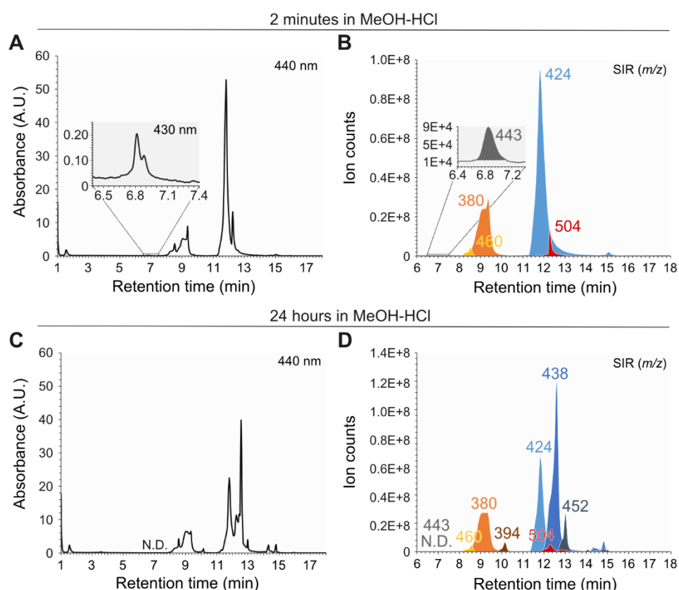
Figure 4-2. Chromatographic profiles of synthesized xanthommatin before and after storage in acidified methanol.
