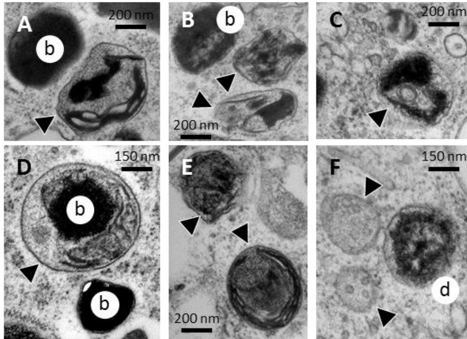
Figure S6-6. Ultrastructural evidence of lysosomal degradation of pigment organelles.
