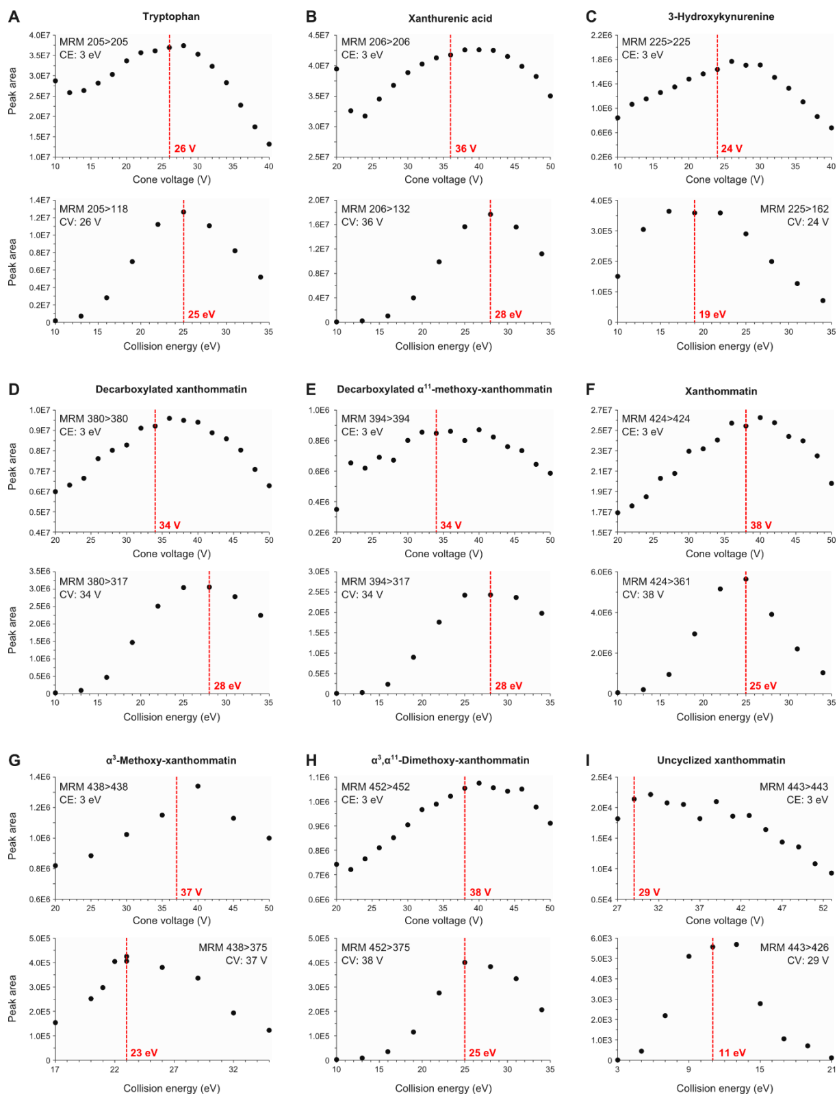
Figure S4-2. Optimization of cone voltages and collision energies for single reaction monitoring of ommochrome-related metabolites.
