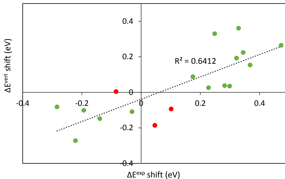
Figure S5-6. Comparison of M05-computed chromic shifts ( \Delta E^{\text{vert}} shift) with experimental shifts ( \Delta E^{\text{exp}} shift) of phenoxazinone/phenoxazine pairs.
