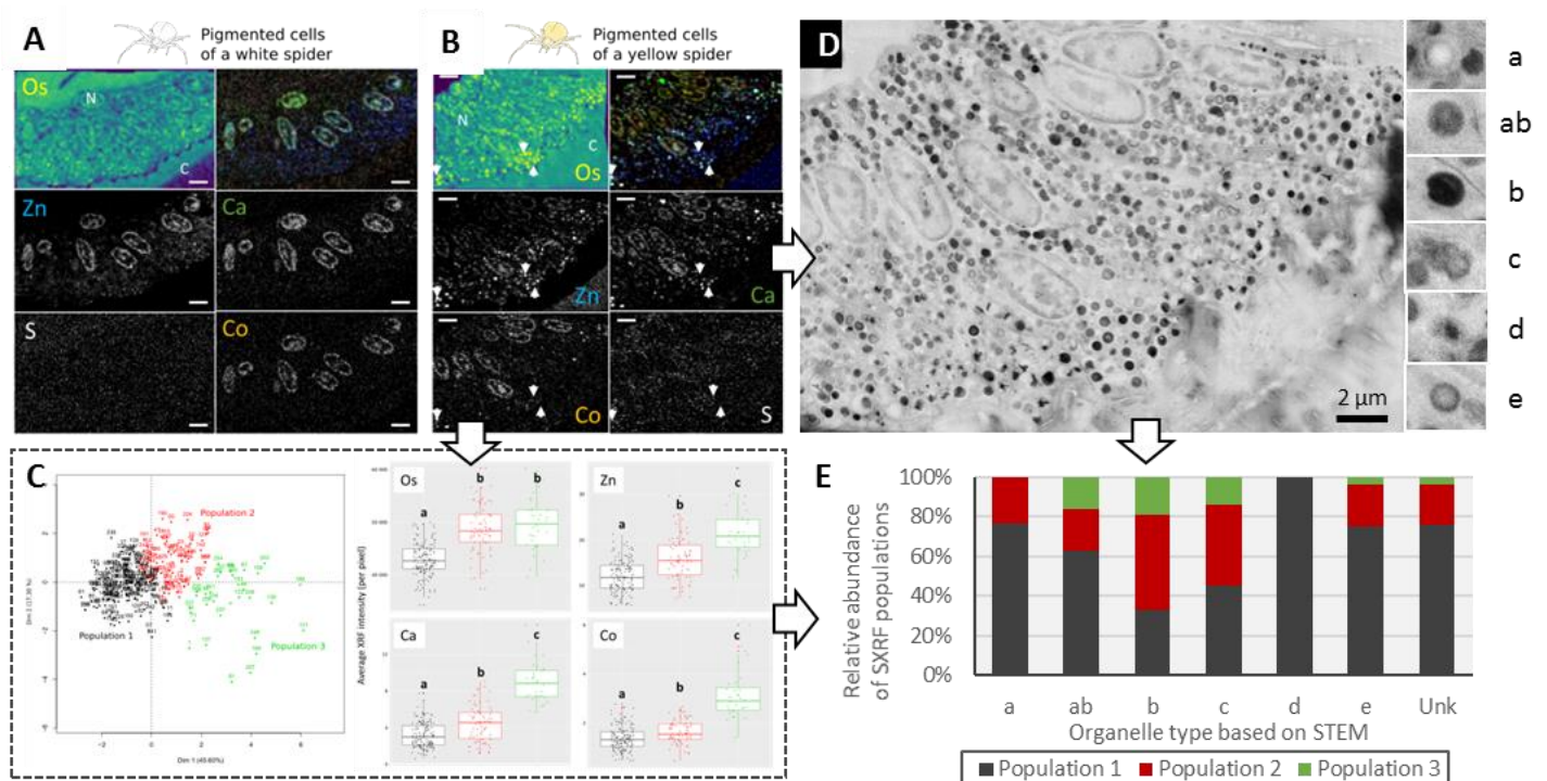
Figure 6-4. Pigment organelles differentially accumulate metals according to coloration and maturation stages.
