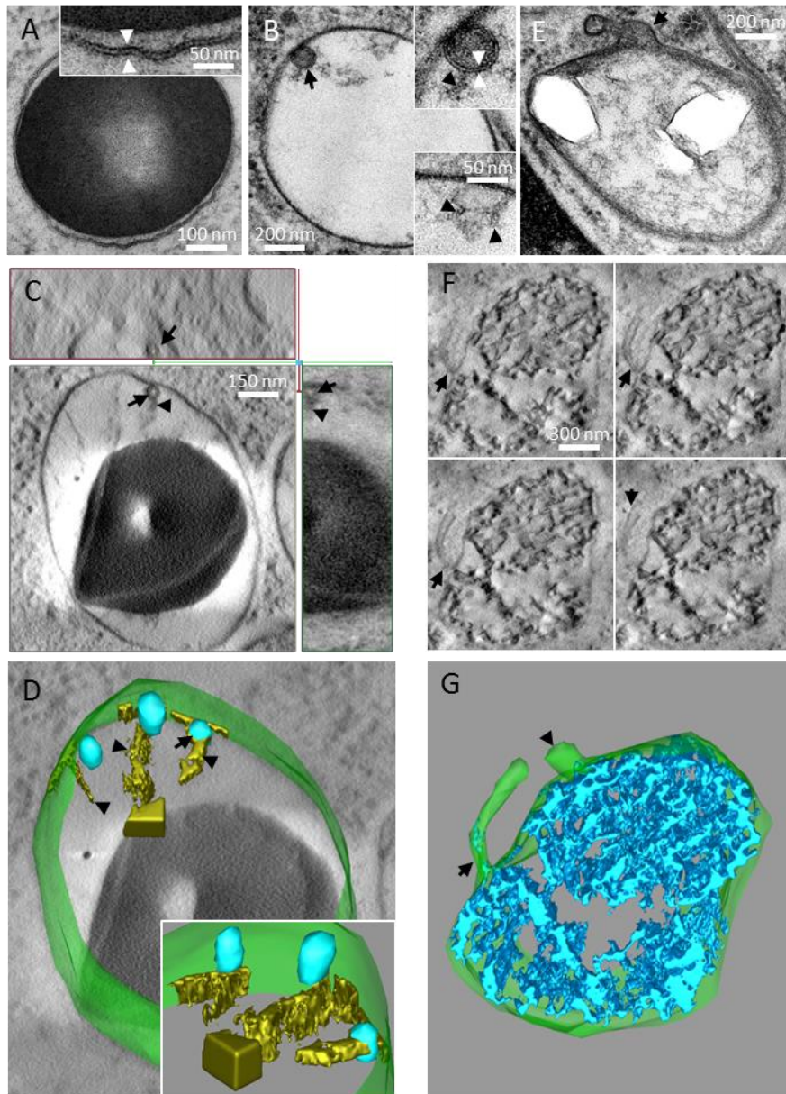
Figure 6-1. High-pressure freezing reveals labile ultrastructural features that relate pigment organelles of crab spiders to endolysosome-related organelles.
