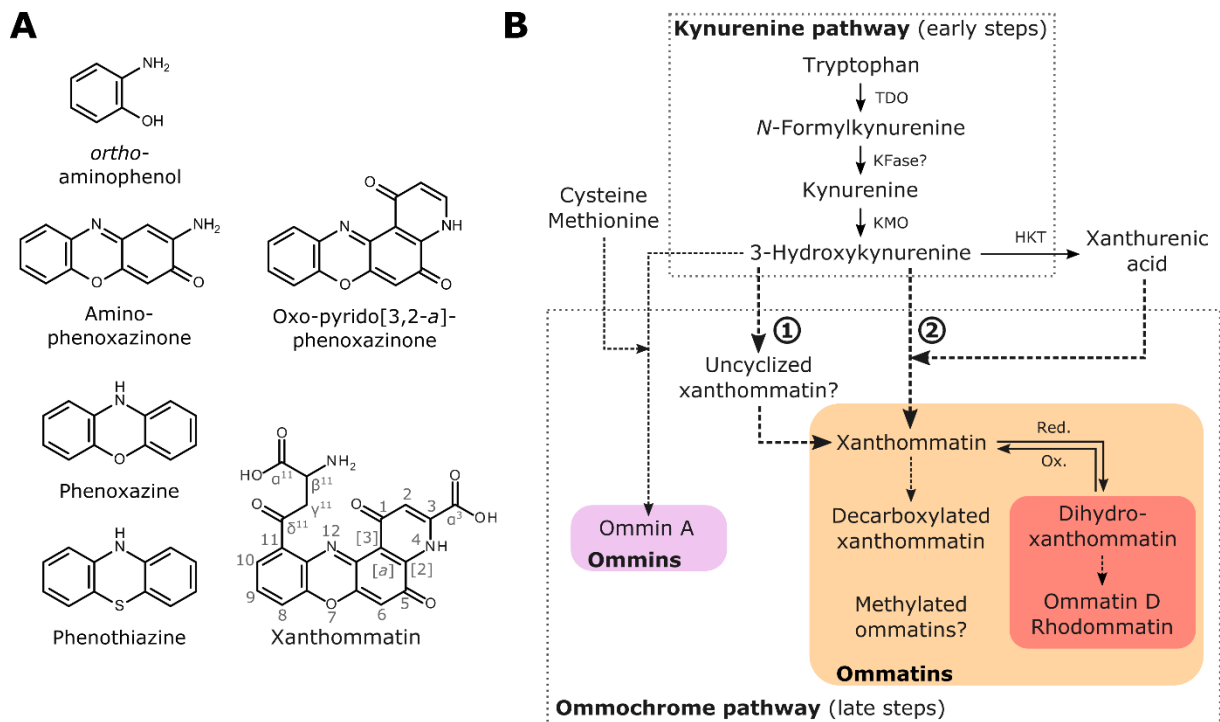
Figure 4-1. Current knowledge of the tryptophan→ommochrome pathway of invertebrates.
