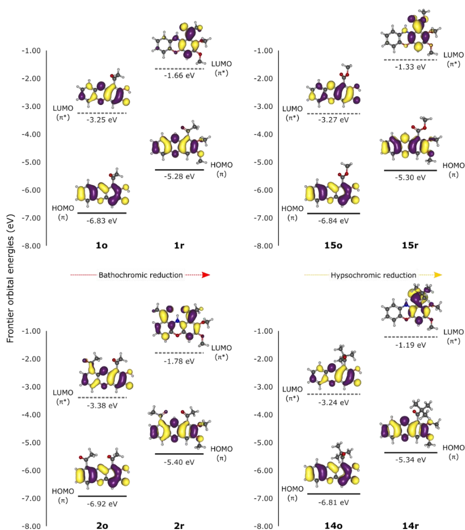
Figure S5-9. Frontier orbital diagrams of two bathochromic phenoxazinone/phenoxazine pairs (1 and 2) and two hypsochromic ones (15 and 14).
