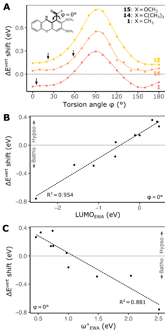
Figure 5-5. Comparison of computed chromic shifts ( \Delta E^{\text{vert}} shift) of phenoxazinone/phenoxazine pairs with geometric (A) and electronic (B-C) properties of electron-withdrawing auxochromes (EWA) in position 1.
