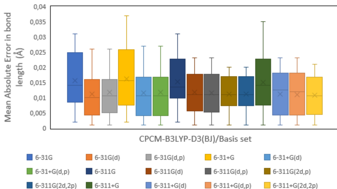
Figure S5-1. Mean absolute errors in computed B3LYP bond lengths of 2-amino-7-methoxy-phenoxazine-3-one as a function of the basis set used.
