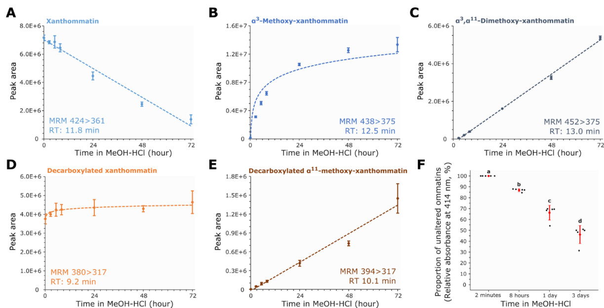
Figure 4-4. Alterations of synthesized ommatins in acidified methanol at 20 °C in darkness.
