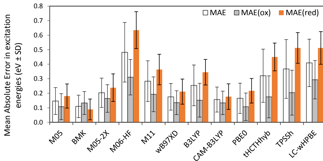
Figure S5-3. Mean absolute errors (MAE) in computed vertical excitation energies of phenoxazinones and phenoxazines for a series of functionals.
