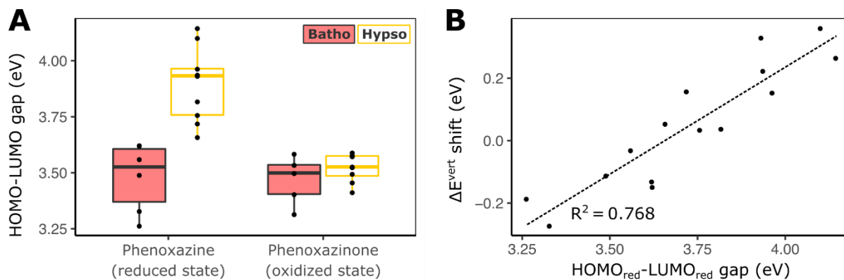
Figure S5-10. Comparison of computed chromic shifts ( \Delta E^{\text{vert}} shift) with HOMO-LUMO gaps of phenoxazinone/phenoxazine pairs.
