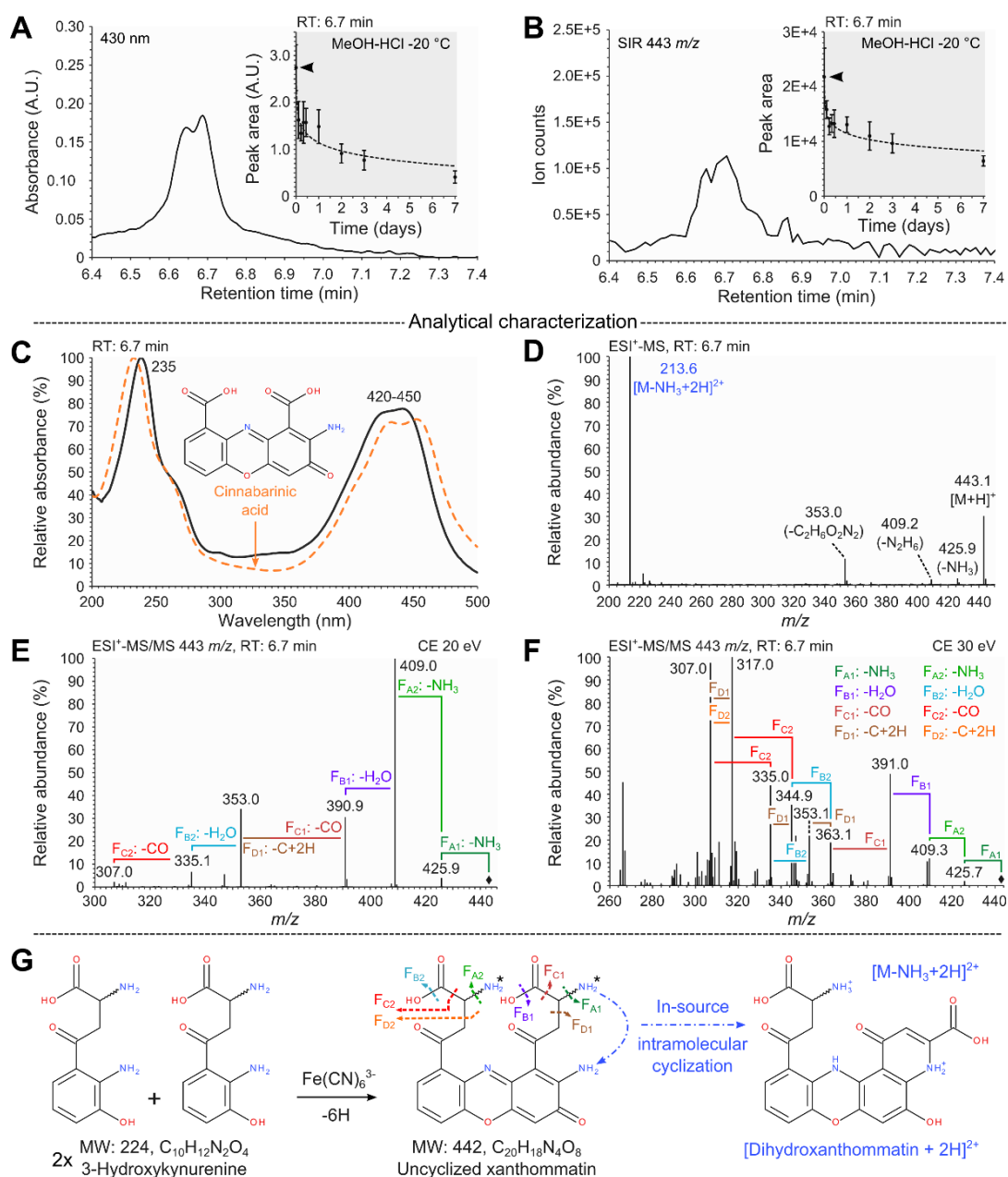
Figure 4-5. Structural elucidation of uncyclized xanthommatin, the labile intermediate in the synthesis of xanthommatin.
