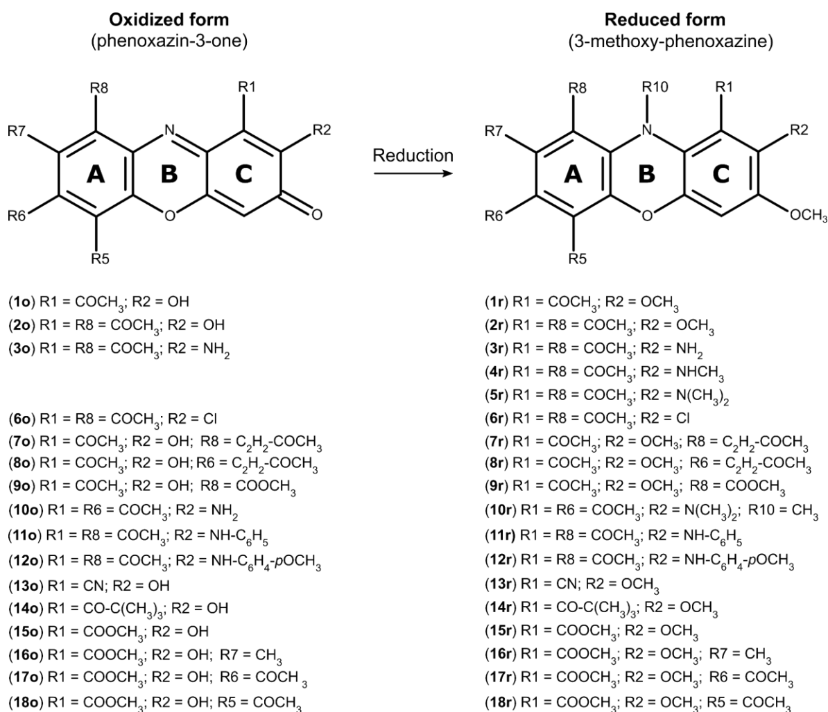
Figure 5-1. Set of substituted phenoxazin-3-ones and 3-methoxy-phenoxazines investigated in this study.
