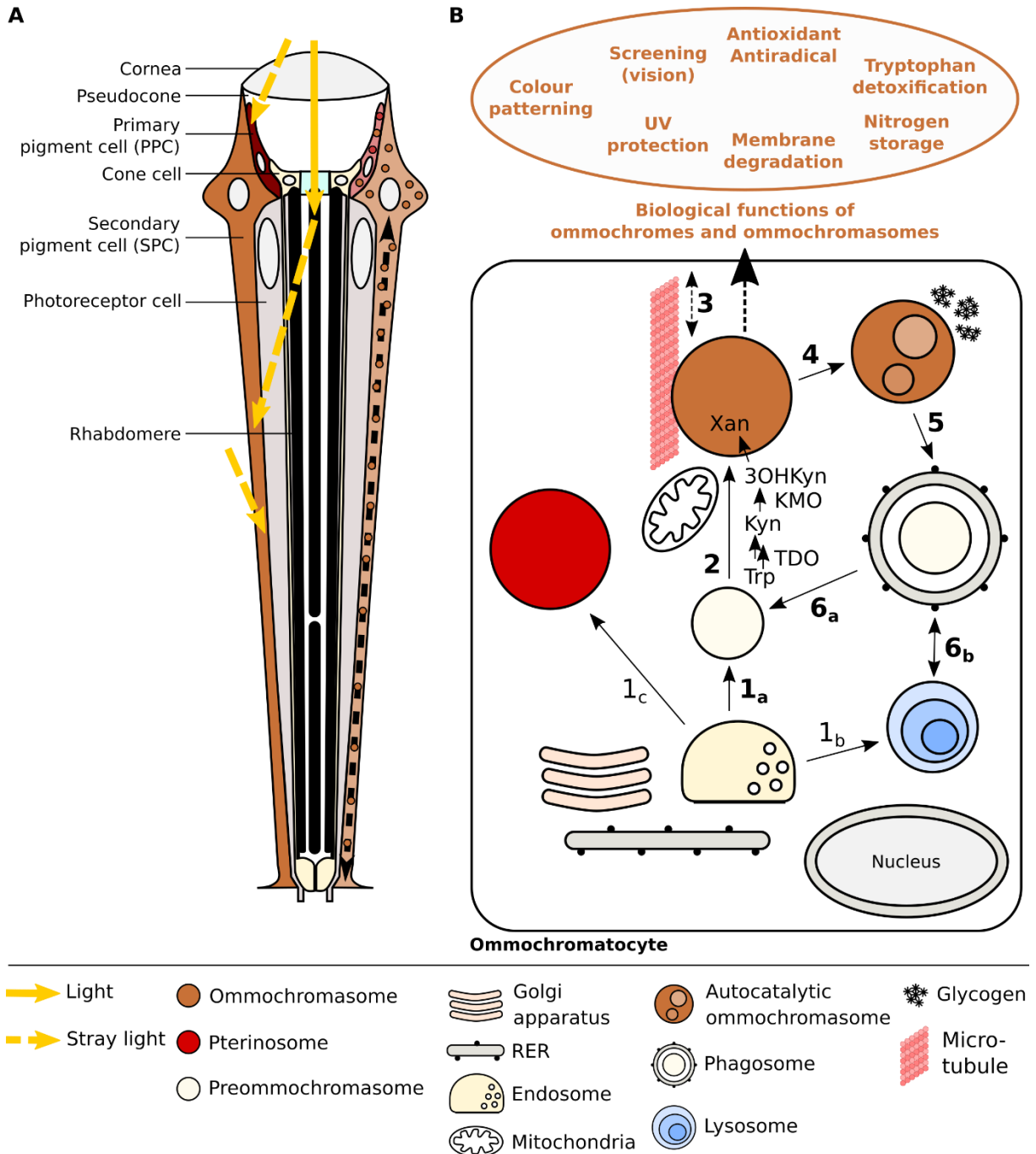
Figure 3-7. Integrated biology of ommochromes and ommochromasomes.
