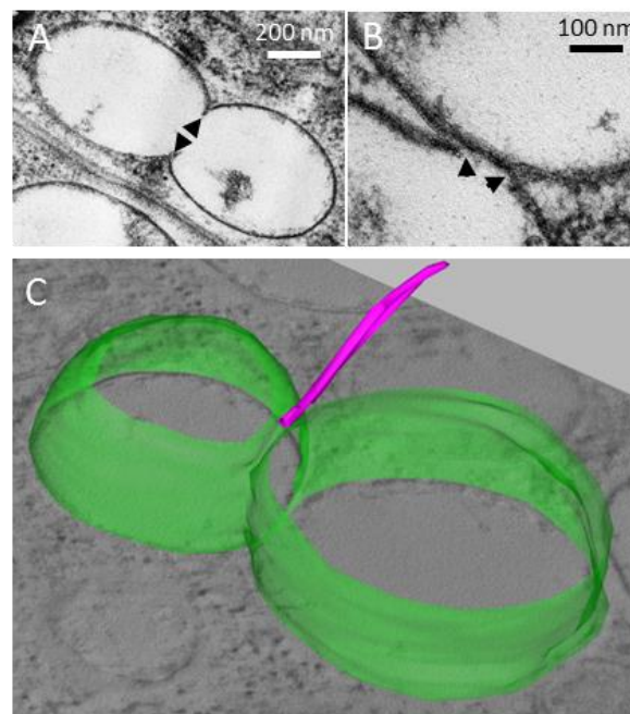
Figure 6-6. Evidence of homotypic fusion events between a-type pigment organelles in white spiders. (A-B) Continuity of limiting membranes (arrowheads) suggest homotypic fusion events between a-type pigment organelles. (C) Three-dimensional reconstruction of fused a-type pigment organelles (green membrane) showing a microtubule (magenta) closely-associated to the fusion site.
