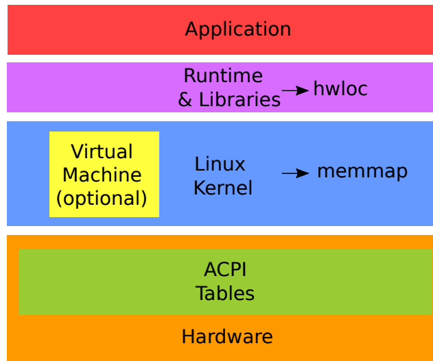
Figure 5.4: Emulation software stack.
