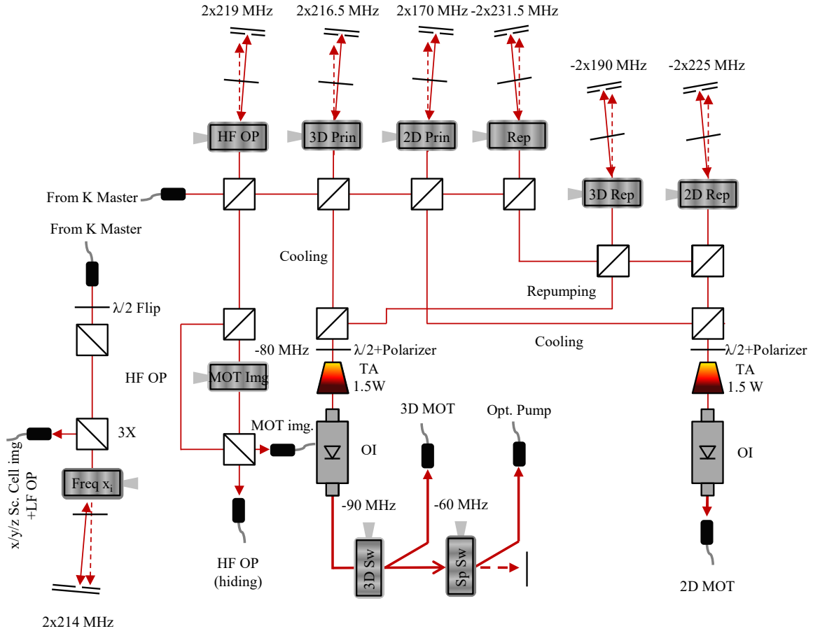
Fig. 2.4 ^{40}\text{K} optical table. Light from the master laser (see fig. 2.3) is split and rerouted towards several double pass AOMs. Light from the principal and the repumper AOMs of the 2D MOT and 3D MOT are overlapped and directed towards the 2D and 3D MOT tapered amplifier respectively. After the amplifiers, the MOTs lights are sent to the main table through single mode optical fibers where they will be used for the 2D-MOT, the 3D-MOT and the optical pumping in the MOT chamber. Optical isolators are placed to avoid damaging the TA chips due to back reflections. After the high field optical pumping AOM, the light is directed towards two fibers: one for the optical pumping at high field in the science cell and one for the MOT imaging. Finally, light from the main D2 laser is also used for the imaging in the science cell. Figure style adapted from [74].
