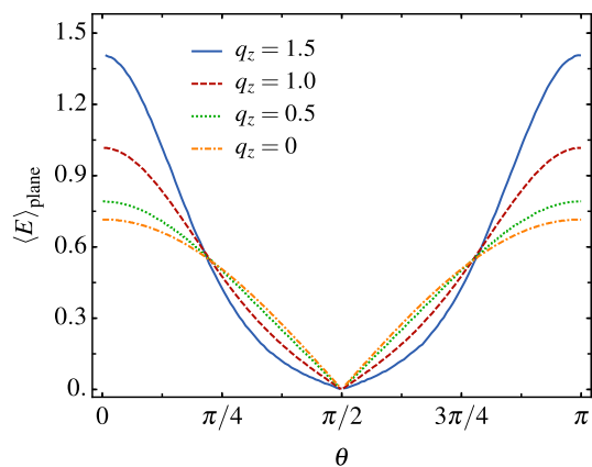
Figure 7. Using Eqs. (33) and (34) to plot \langle E \rangle_{\text{plane}}(\theta) for different values of momentum kick q_z .
