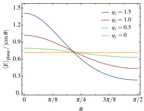
Figure 8. Using Eqs. (33) and (34) to plot \langle E \rangle_{\text{plane}}(\theta)/|\cos \theta| for different values of momentum kick q_z .
