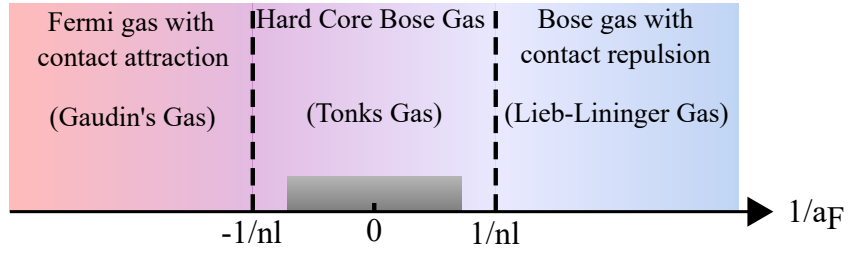
Fig. 4.5 Phase diagram of a 1D Fermi mixture.
