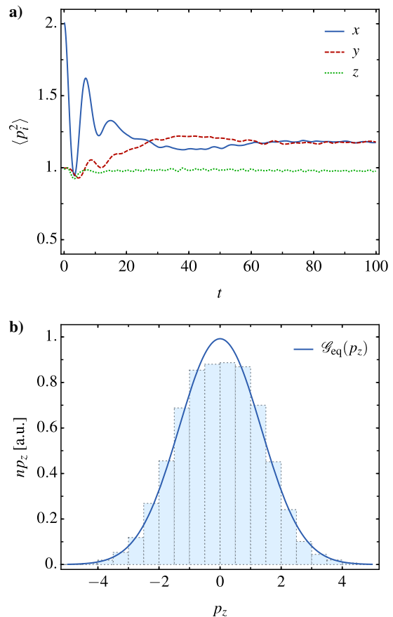
Figure 1. Numerical simulation of the relaxation dynamics in a quadrupole trap. a) Kinetic energy per atom along different directions as a function of time after a kick q = 1 along x at t = 0 . The energies seem to reach a stationary state for t \geq 80 . Along z the average kinetic energy is almost unchanged from its initial value \sim 1 , but along x and y the corresponding values increase by the same amount to a final value of \sim 1.2 . b) Momentum distribution np_z of the steady state. The solid line \mathcal{G}_{\text{eq}} is a Gaussian distribution with the same variance.
