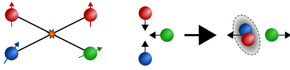
Fig. B.3 Schematic description of two and three body inelastic collisions. For two body inelastic collisions, the two atoms in the entrance channel will collide and flip their spin in the process. During three body collisions, two partners form a molecule and a third partner gather the excess of energy.
