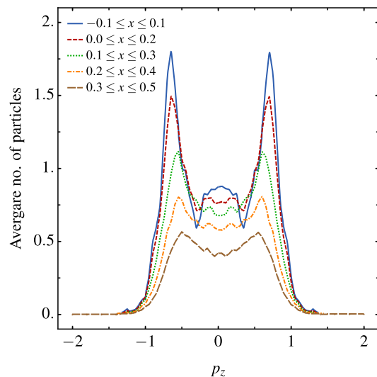
Figure 2. The long time Boltzmann distribution f after a kick along z plotted as a function of p_z keeping all other variables x, y, z, p_x, p_y fixed and for different values of x . To obtain a nonzero number of atoms in the six dimensional volume we considered a narrow region in phase space given by the coordinates in the figure and divided it into bins. We plot the number of atoms in each bin averaged over time. It can be seen that f does not resemble a Gaussian thermal function and that the three peaks feature becomes more prominent for x closer to the center. Similar results are found plotting along all other coordinates.
