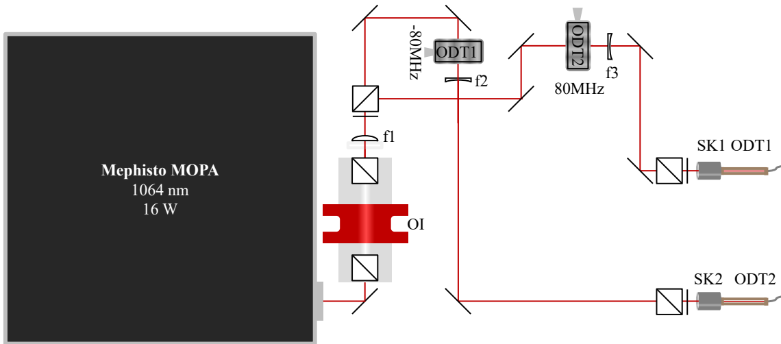
Fig. 3.4 Schematics of the main dipole traps setup. The Mephisto laser (16 W of maximum power) is splitted thanks a polarized beam splitter cube, after being directed to a convex lens f_1 to recollimate the output beam, generating the ODT1 and the ODT2 laser beams. Each beam is then rerouted to an AOM before being sent to a dedicated high power fiber. To prevent any damage of the main laser due to back reflexion, an optical isolator is located right after the Mephisto output. Optical elements: OI (optical isolator) from EO Tech, ODT1 and ODT2 AOMs 80 MHz AOM from Gooch&Housego, model 3080-197, f_1 : 400 mm convex lens from Lambda Research Optics (LRO), model VAR2-R1064-PCX-25.4U-400, f_2 : -300 mm concave lens from LRO, model VAR2-PCC-25.4U-(FL-300)-1064, f_3 : -1000 mm concave lens from LRO, model VAR2-R1064-PCC-25.4U-500, SK1 and SK2: fiber collimator f = 11 mm from Schäfter-Kirchoff, model 60FC-SMA-T-4-A11-03, ODT1 and ODT2 fibers: large mode area high power fibers from NKT Photonics, model LMA-PM-10.
