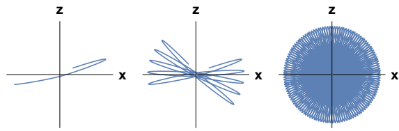
Figure 4. Orbit of atom in a plane with a central potential V(r) = r after increasingly long times from left to right. Since the trajectory never closes, according to Bertrand's theorem, it fills the annular region between r_{\max} and r_{\min} in an isotropic, dense fashion as t \rightarrow \infty .
