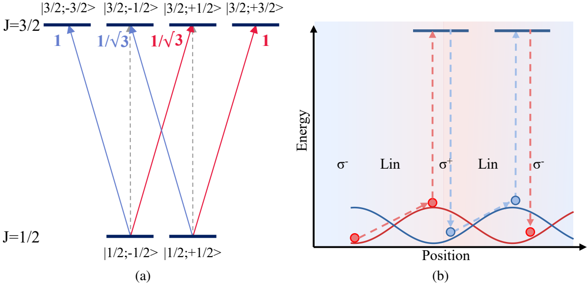
Fig. 2.9 Principle of Sisyphus effect. (a) Atomic level for a transition between the |J = 1/2\rangle and |J = 3/2\rangle levels. The Clebsch-Gordan coefficients for the \sigma^\pm transition, which are different, are indicated. (b) Principle of Sisyphus cooling for a simple J=1/2 ground state. Due to the position dependency of the light polarization, the light shift intensity also varies with the position (because of the difference of the Clebsch-Gordan coefficients). Consequently, the energy of the two sublevels of the groundstate will have a modulation period of \lambda_L/2 . Atoms with a velocity such that v \cdot \gamma_p^{-1} \sim \lambda_L/4 originally in the valley will climb the hill, reach the top, absorb and re-emit a photon, before being transferred to the valley of the other sublevel to climb another hill. Thus on average, atoms travel more uphill than downhill, which lead to the Sisyphus cooling.
