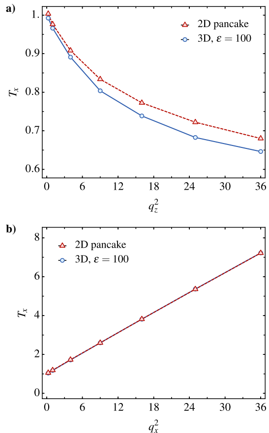
Figure 12. Comparison of the 2D potential given by (56) and the pancake potential. Here \varepsilon = 100 , but larger \varepsilon values produced consistent results. The plots are for \langle p_x^2 \rangle as a function of q_z^2 (top panel), and as a function of q_x^2 (bottom panel). Solid and dashed lines represent guides to the eye. Note that the two potentials give almost identical results for the heating along the kick direction and a small discrepancy for the orthogonal cooling.
