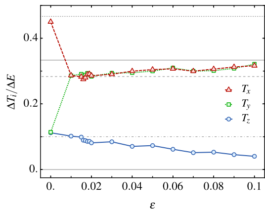
Figure 10. Behavior of the final temperatures \Delta T_i / \Delta E as a function of the anisotropy \varepsilon near the spherical limit after a kick along x . At \varepsilon = 0 , T_z = T_y after which there is a discontinuous change in the temperatures due to the breaking of spherical symmetry along z . Data are obtained by numerical simulation over 100 000 atoms. Dashed, dotted and plain lines correspond to the theoretical expectations of the fully isotropic (39, 40), almost isotropic (38 and 50) and quadrupole geometries, respectively.
