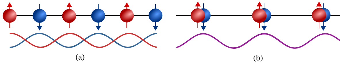
Fig. 4.7 Collective excitations of a 1D system. (Left) For a spin density wave (SDW), one has two waves for the spin up and the spin down component. The two waves are shifted with respect to one another and while the spin modulation is maximum the density is uniform. For a charge wave density (CDW), the two waves are synchronized leading to zero modulation of the spin but a modulation of the density.
