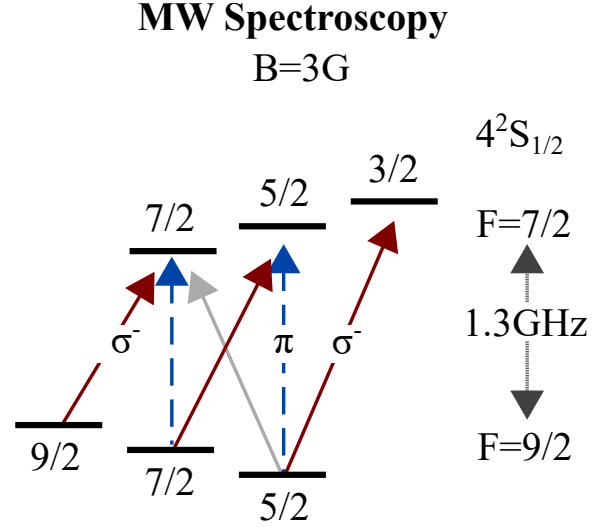
Fig. A.6 Microwave transitions for the positive states of ^{40}\text{K} . MW transitions between the three spin states m_F = 9/2, 7/2 and m_F = 5/2 of the F = 9/2 groundstate manifold and the F = 7/2 upper manifold of the groundstate.
