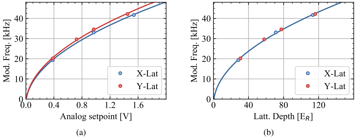
Fig. 6.9 x- and y-lattice calibration. (a) Measured trapping frequencies as a function of the analog setpoint of the optical lattice for both 1D lattices. (b) Evolution of the trapping frequencies as a function of the lattice depth using the harmonic approximation of the band structure.
