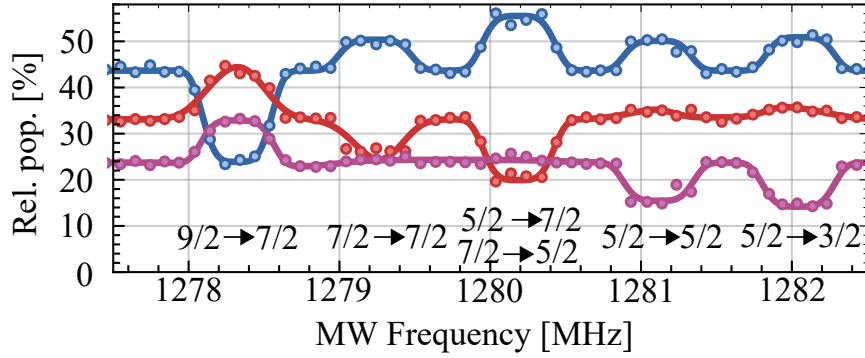
Fig. A.7 Microwave transitions for the positive Zeeman states. After a 10ms sweep the atoms are subjected to the 2\mu\text{s} SG pulse and then imaged via absorption imaging. Prior to imaging atoms were transferred in the m_F = 9/2 Zeeman states with 10\mu\text{s} of optical pumping. By transferring atoms in a zeeman states to the upper manifold its relative population decreases while the other two spins states relative population increases. Solid lines are super-Gaussian fits and act as a guide to the eye.
