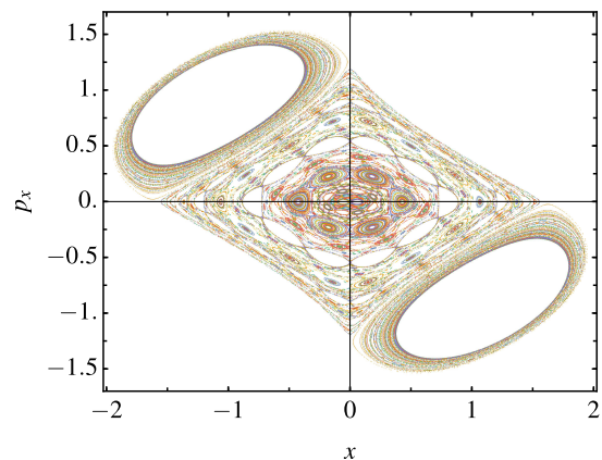
Figure 3. Poincaré map of the quadrupole potential. We study trajectories with the same energy but different initial phase-space coordinates. The values of x and p_x are recorded whenever z = 0 and p_z > 0 . We see the appearance of small islands denoting invariant tori close to which quasi-integrable trajectories evolve, separated by contiguous regions of chaotic dynamics.
