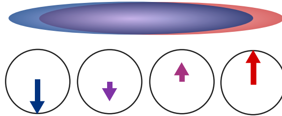
Fig. 4.8 Experimental measurement technique of the longitudinal magnetization. Owing to selective spin imaging the longitudinal magnetization can be easily measured.
