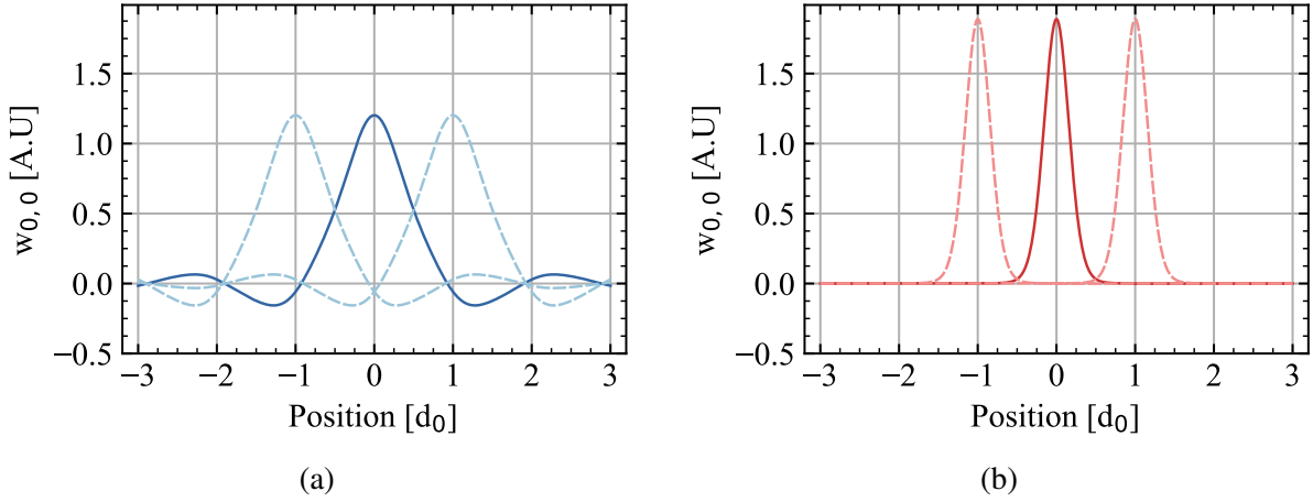
Fig. 5.4 Representation of the Wannier function for the lowest band and a quasi-momentum \hbar q = 0 . (a) Representation of the Wannier function \omega_{0,0}(x) as a function of x/d_0 (blue) as well as \omega_{0,\pm 1}(x) (dashed blue) for V_0 = E_R . The overlap between the Wannier functions is important. (b) Same as (a) for V_0 = 20E_R . The overlap is greatly reduced. When V_0 \geq 4.0E_R , the wannier function can be approximated by the wavefunction of an harmonic oscillator with a precision greater than 97% [220].
