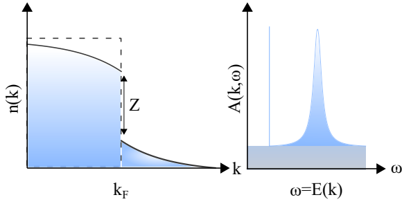
Fig. 4.4 Momentum distribution and spectral response of an ideal Fermi gas (dashed line on the left figure and Dirac peak on the right one) and a Landau liquid. The spectral function of a Fermi liquid consists of an incoherent background with a weight 1 - z_k and the quasi-particle peak with a weight z_k . The width of the peak is proportional to 1/\tau , with \tau being the lifetime of the quasi-particles.
