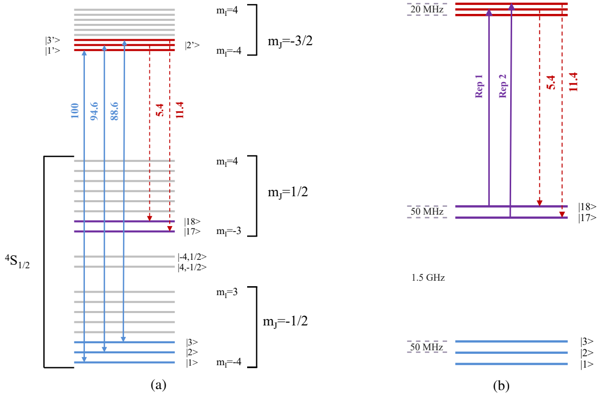
Fig. 3.10 Principle of our high field imaging. (a) Imaging transitions for imaging at the zero crossing (209.9 G) . (b) Repumping transitions at the same magnetic bias field to keep atoms into the imaging transition cycle.
