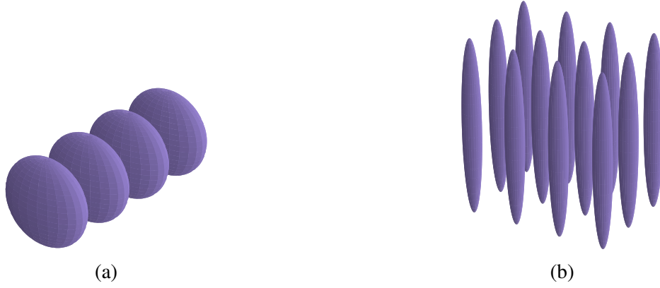
Fig. 5.2 Creation of an optical lattice. Two counter-propagation beams interfere to create a 1D optical lattice (left). When two pair of beams are used a cubic 2D optical lattice can emerge to create an array of elongated micro traps (right). The lattice spacing in both cases is d_0 = \lambda/2 , where \lambda corresponds to the wavelength of the beams.
