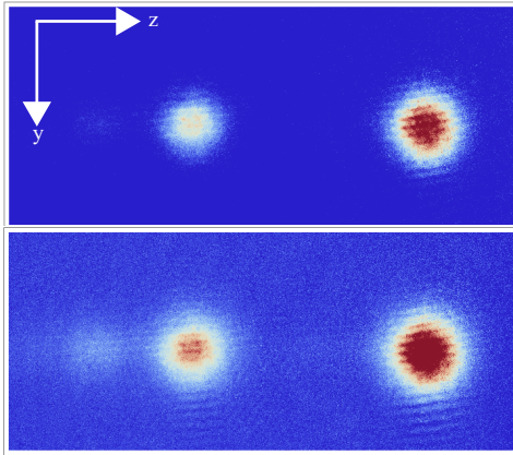
Fig. A.5 SG picture taken along the x-imaging. (Top) In absence of re-pumping the population in m_F = 5/2 is barely visible. (Bottom) Owing to the optical pumping, the spin states ( m_F = 5/2 and m_F = 7/2 ) detectivity increased and one can see the signal of m_F = 5/2 (Left) and m_F = 7/2 (middle) greatly improved while not deteriorating the signal of m_F = 9/2 (right).
