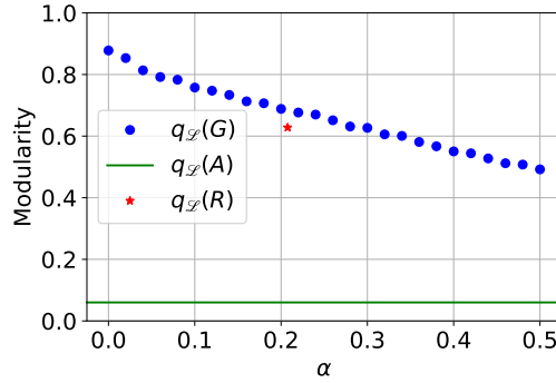
Figure 5.8: Comparison of modularity between our model G , Avin et al. hypergraph A and real co-authorship hypergraph R .
