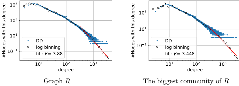
Figure 5.6: A power-law distribution fitted to the degree distributions.
