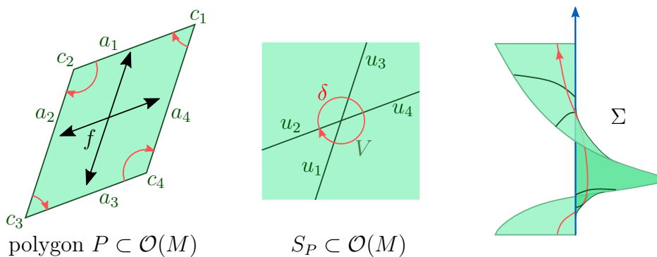
Figure 1.10: Fundamental domain of a ramified partial section.
