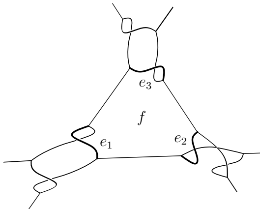
Figure 2.14: Edges used for the slide correction.
