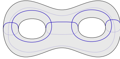
Figure 1.4: Filling geodesic multi-curve on a hyperbolic surface.
