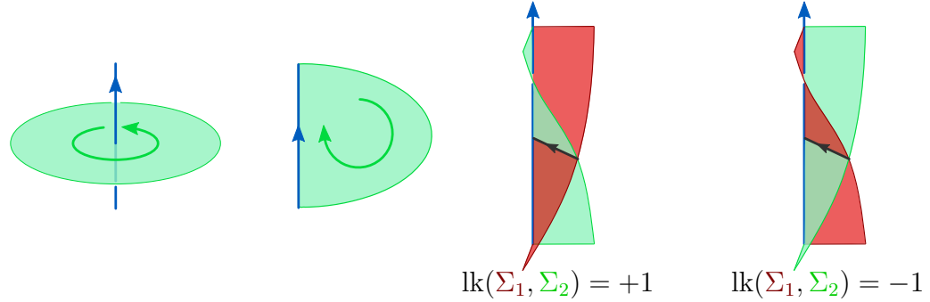
Figure 1.3: Orientation conventions. The flow orients the interior of the surface, which orients its boundary
