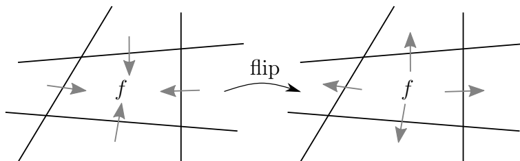
Figure 2.10: A sink face on the left, and a flip.
