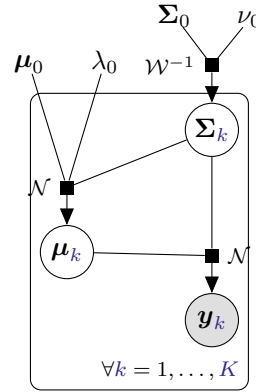
Figure 5.2: Graphical model of the hierarchical structure of the generative model for the vector y_k of peptide intensities in K groups of biological samples, i.e. K experimental conditions.
