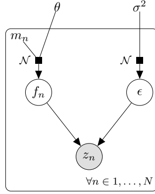
Figure 2.6: Graphical model of dependencies between variables in the Gaussian Process with shared covariance structure model.
