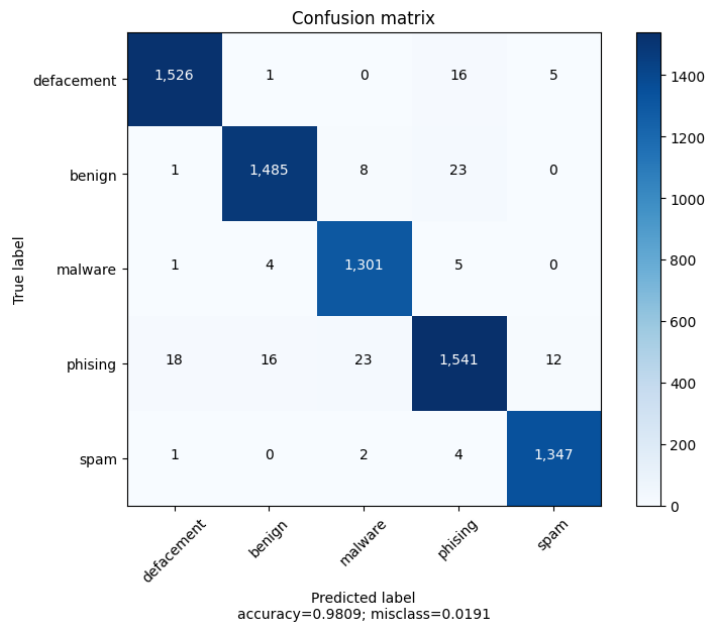
Figure 65: Confusion matrix for Adaboost model on the DB- MALCURL
