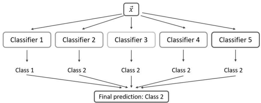
Figure 15: General architecture of the voting classifier [77]
