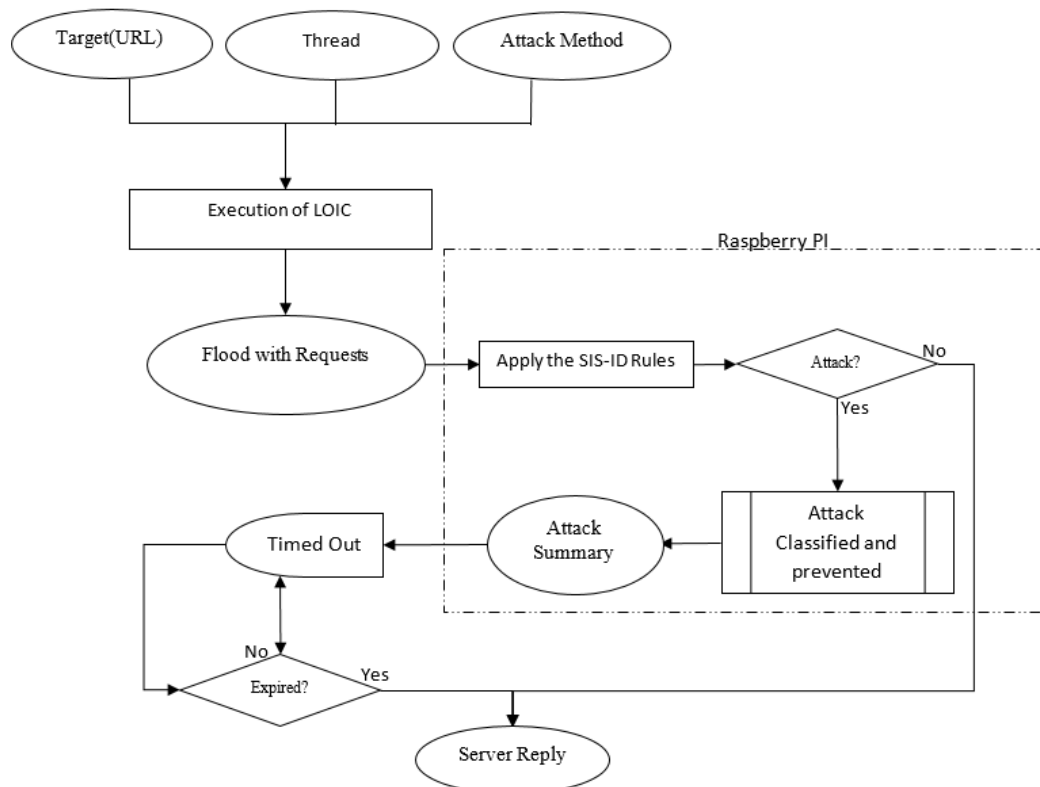
Figure 80: The general architecture of our SIS-ID hardware-based real-time simulation
