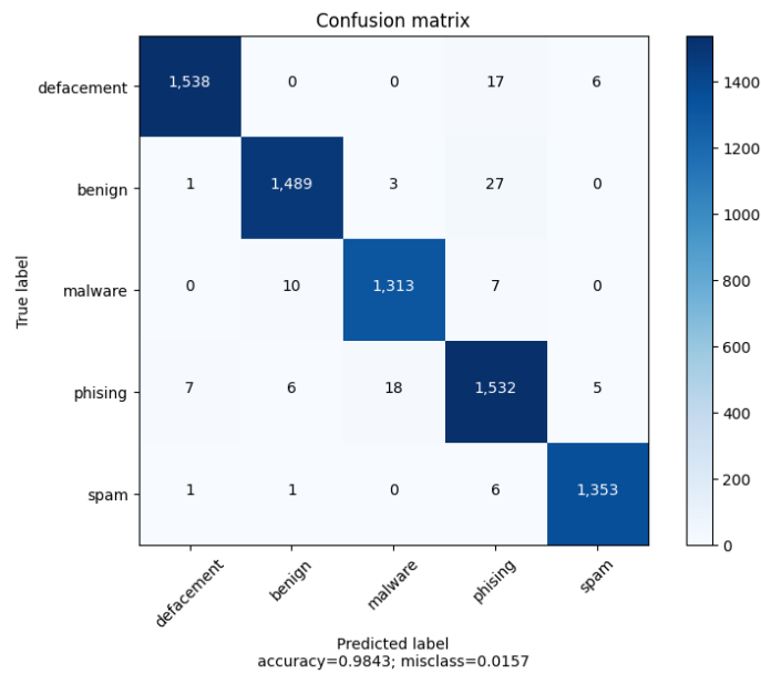
Figure 63: Confusion matrix for XGBoost model on the DB-MALCURL
