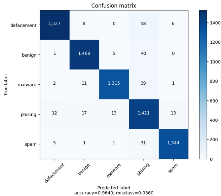
Figure 61: Confusion matrix for KNN model on the DB-MALCURL
