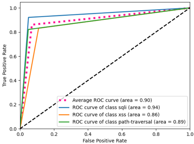
Figure 50: Decision Tree ROC curve
