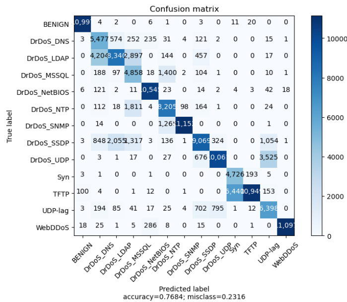
Figure 74: Confusion matrix for Random Forest model on the DB-DDOS
