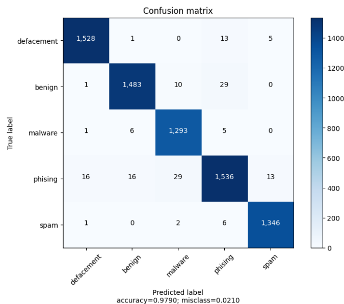
Figure 68: Confusion matrix for Bagging model on the DB-MALCURL
