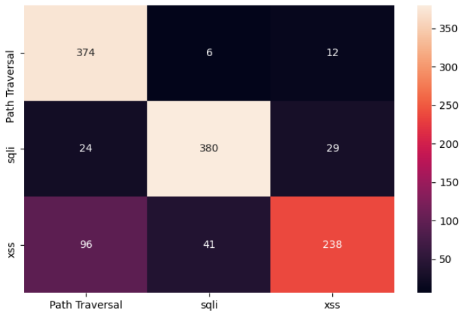
Figure 54: Confusion matrix for the SVM model
