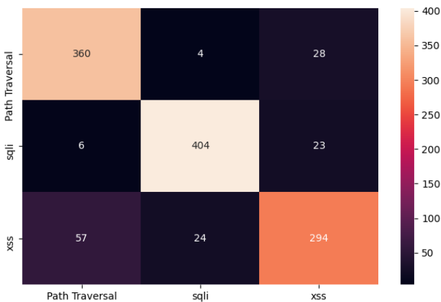
Figure 55: Confusion matrix for the KNN model
