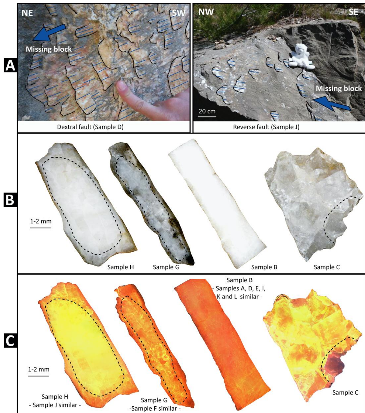
Figure IV-3 - Syn-faulting calcite samples. (a) Examples of analysed tectonic structures and associated slickenfibres calcites. (b) Pictures of syn-faulting calcites with a binocular microscope in reflected light. (c) Cathodoluminescence imaging of corresponding syn-faulting calcites.
